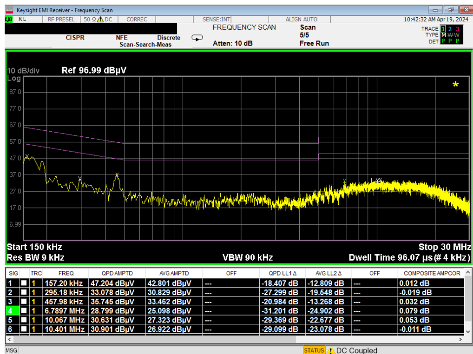
Plot 7-235. Line Conducted Plot with 802.11a UNII Band 2C (N)
