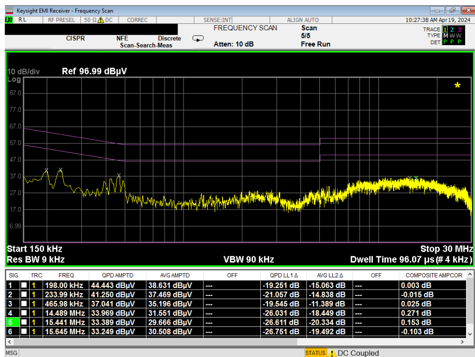
Plot 7-231. Line Conducted Plot with 802.11a UNII Band 1 (N)
