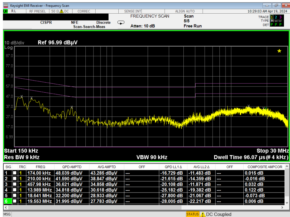
Plot 7-233. Line Conducted Plot with 802.11a UNII Band 2A (N)
