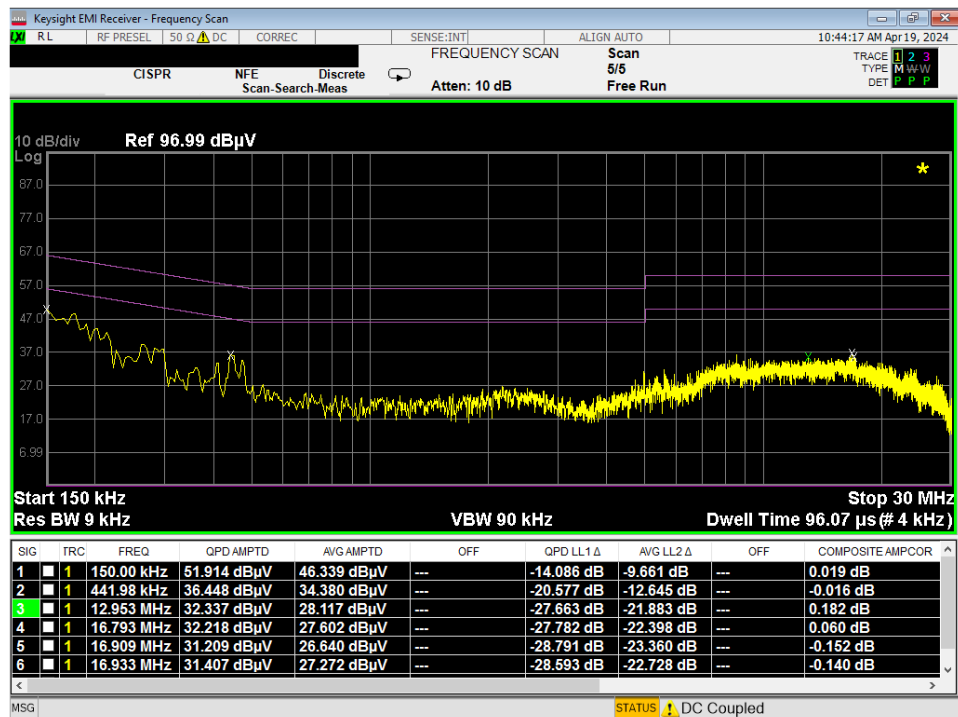
Plot 7-237. Line Conducted Plot with 802.11a UNII Band 3 (N)
