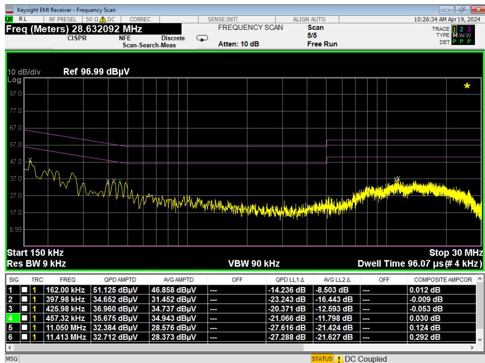
Plot 7-230. Line Conducted Plot with 802.11a UNII Band 1 (L1)
