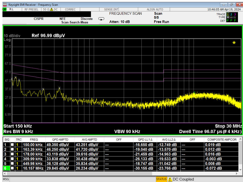
Plot 7-236. Line Conducted Plot with 802.11a UNII Band 3 (L1)
