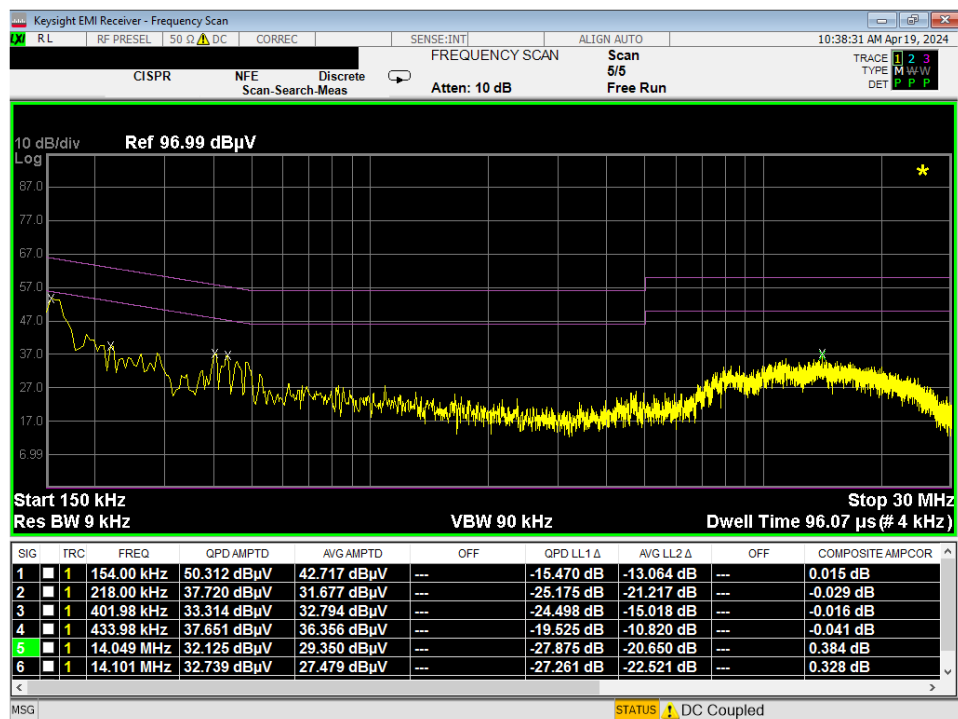
Plot 7-234. Line Conducted Plot with 802.11a UNII Band 2C (L1)
