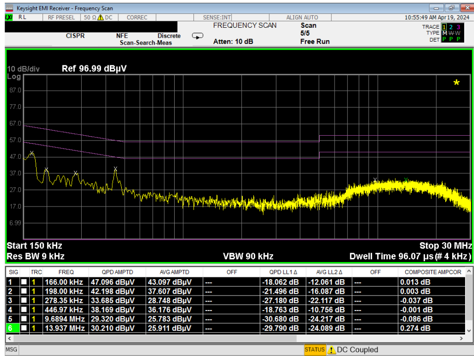
Plot 7-238. Line Conducted Plot with 802.11a UNII Band 4 (L1)
