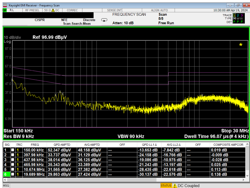
Plot 7-232. Line Conducted Plot with 802.11a UNII Band 2A (L1)
