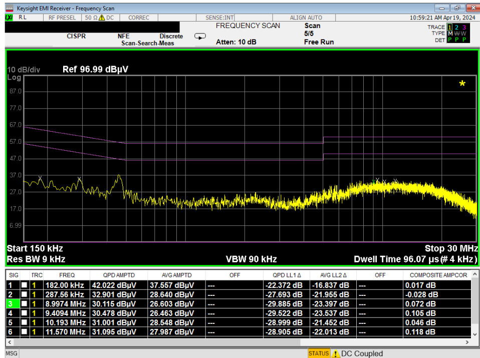
Plot 7-239. Line Conducted Plot with 802.11a UNII Band 4 (N)
