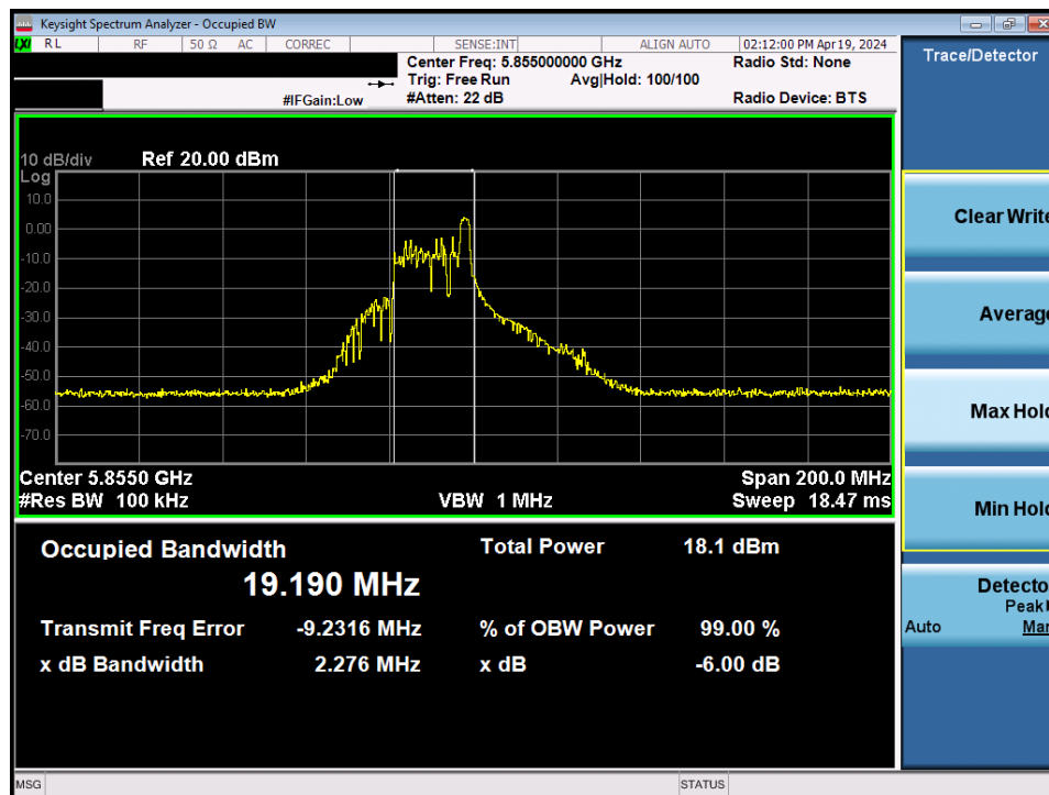
Plot 7-66. 6dB Bandwidth Plot MIMO ANT2 (80MHz BW 802.11be – 26 Tones (UNII Band 3/4) – Ch. 171)
