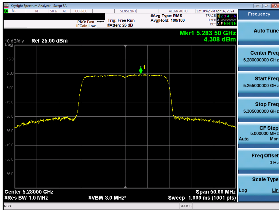
Plot 7-97. Power Spectral Density Plot MIMO ANT1 (20MHz BW 802.11be – 242 Tones (UNII Band 2A) – Ch. 56)
