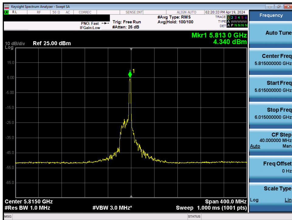
Plot 7-92. Power Spectral Density Plot MIMO ANT1 (160MHz BW 802.11be – 26 Tones (UNII Band 3/4) – Ch. 163)
