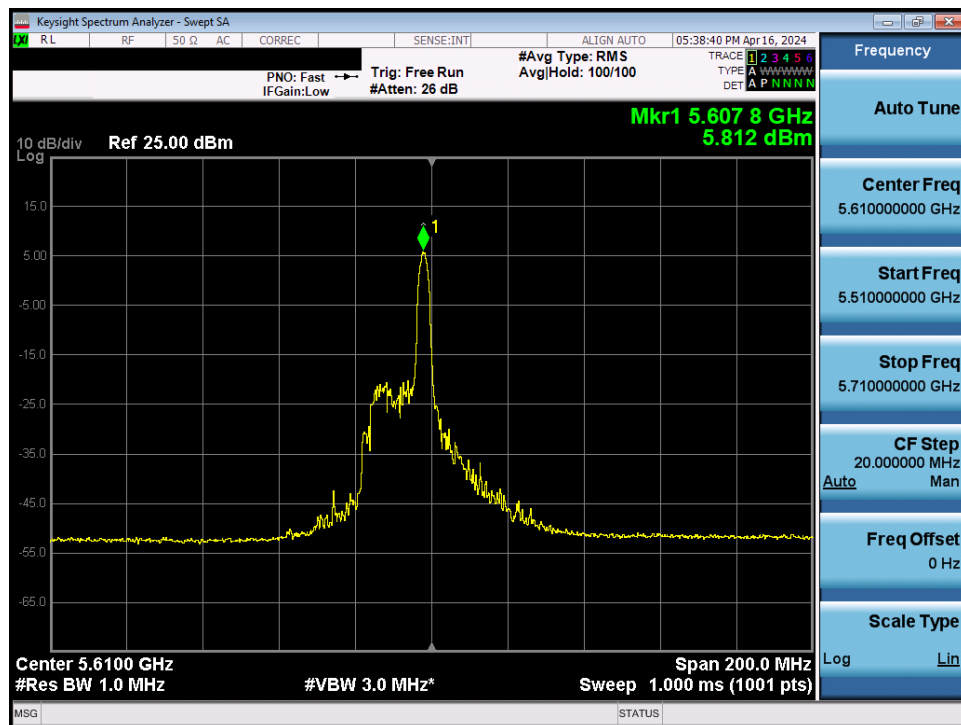
Plot 7-84. Power Spectral Density Plot MIMO ANT1 (80MHz BW 802.11be – 26 Tones (UNII Band 2C) – Ch. 122)
