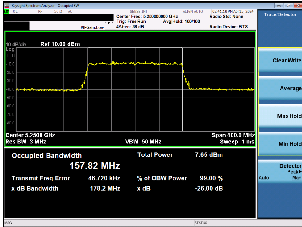
Plot 7-17. 26dB Bandwidth Plot MIMO ANT1 (160MHz BW 802.11be – 2x996 Tones (UNII Band 1/2A) – Ch. 50)
