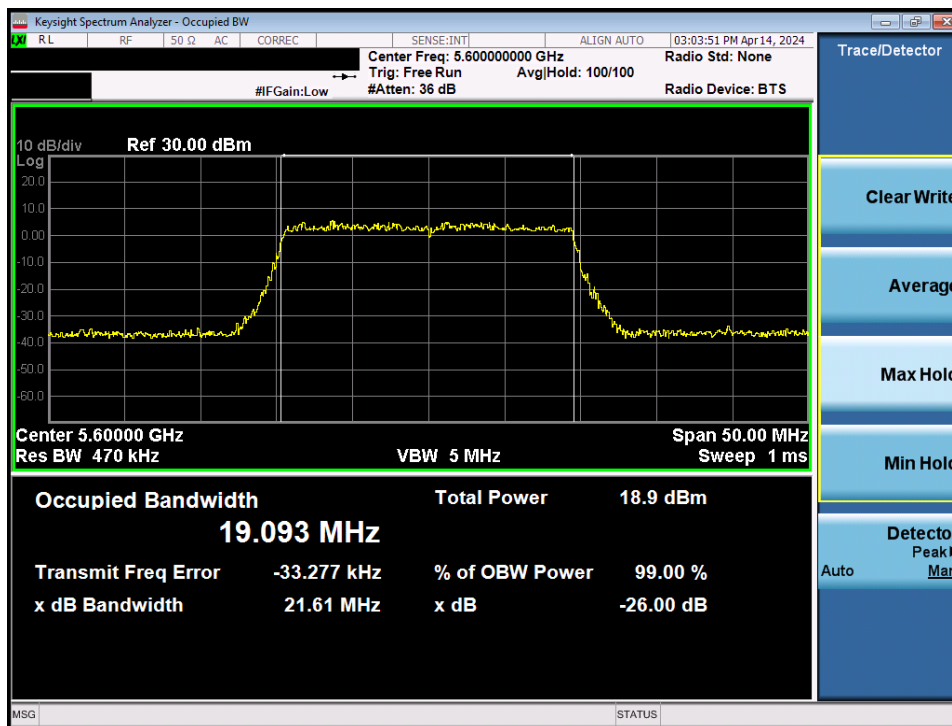
Plot 7-43. 26dB Bandwidth Plot MIMO ANT2 (20MHz BW 802.11be – 242 Tones (UNII Band 2C) – Ch. 120)
