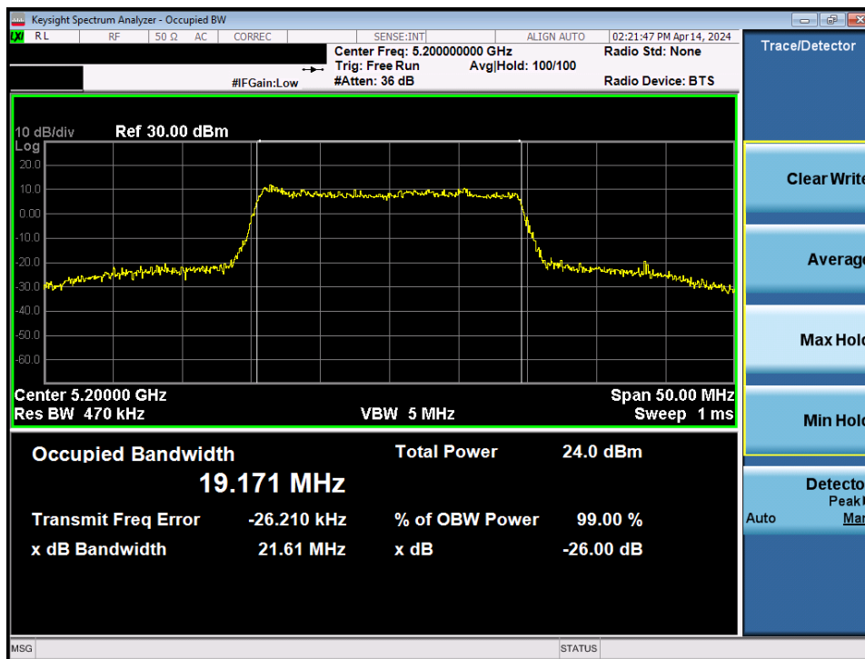
Plot 7-36. 26dB Bandwidth Plot MIMO ANT2 (20MHz BW 802.11be – 242 Tones (UNII Band 1) – Ch. 40)
