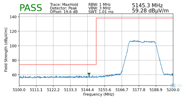
Plot 7-2. Radiated Lower Band Edge Plot MIMO (Peak – UNII Band 1)
