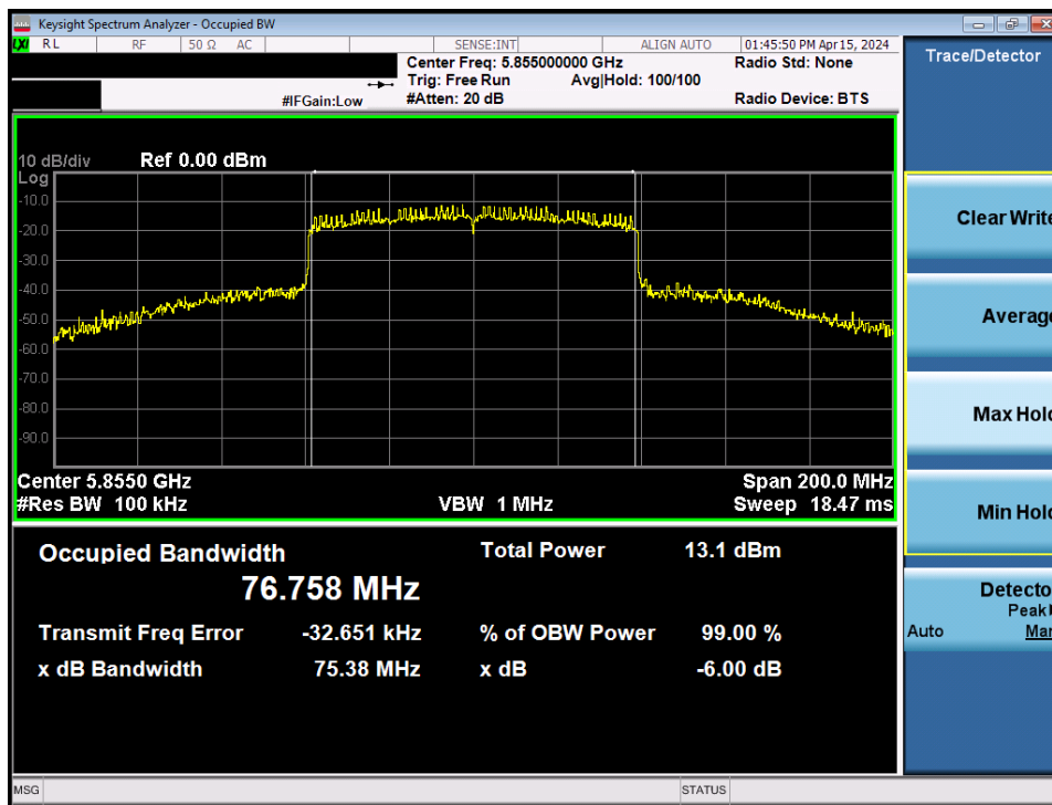
Plot 7-73. 6dB Bandwidth Plot MIMO ANT2 (80MHz BW 802.11be – 996 Tones (UNII Band 3/4) – Ch. 171)
