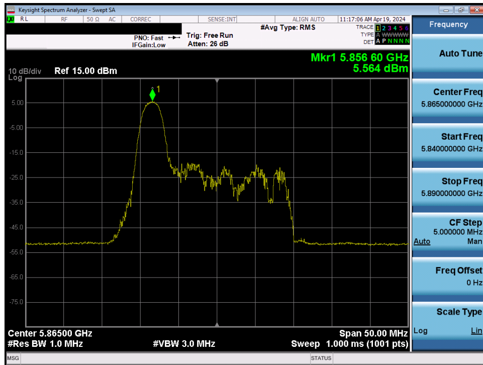
Plot 7-89. Power Spectral Density Plot MIMO ANT1 (20MHz BW 802.11be – 26 Tones (UNII Band 4) – Ch. 173)
