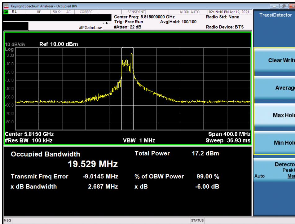
Plot 7-53. 6dB Bandwidth Plot MIMO ANT1 (160MHz BW 802.11be – 26 Tones (UNII Band 3/4) – Ch. 163)
