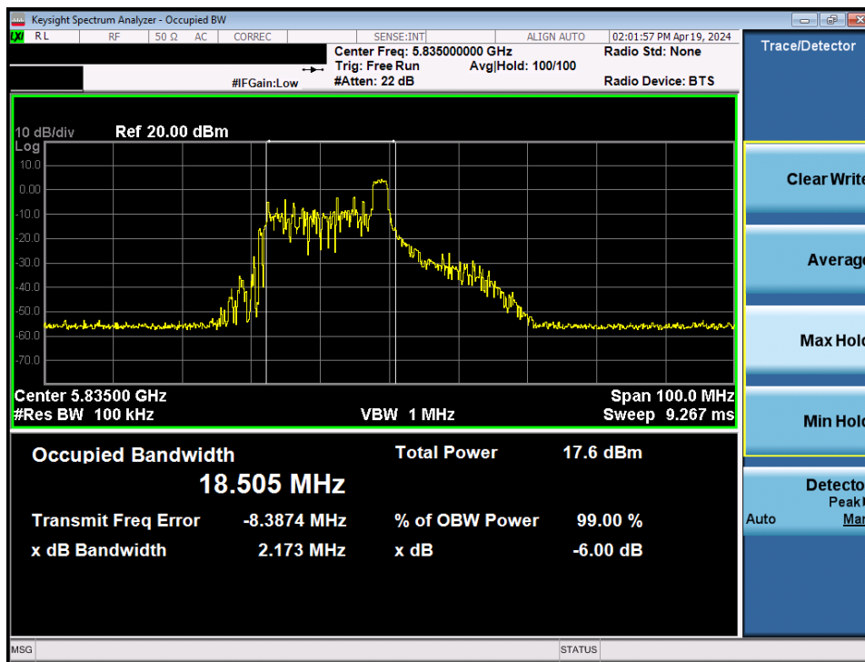
Plot 7-51. 6dB Bandwidth Plot MIMO ANT1 (40MHz BW 802.11be – 26 Tones (UNII Band 3/4) – Ch. 167)
