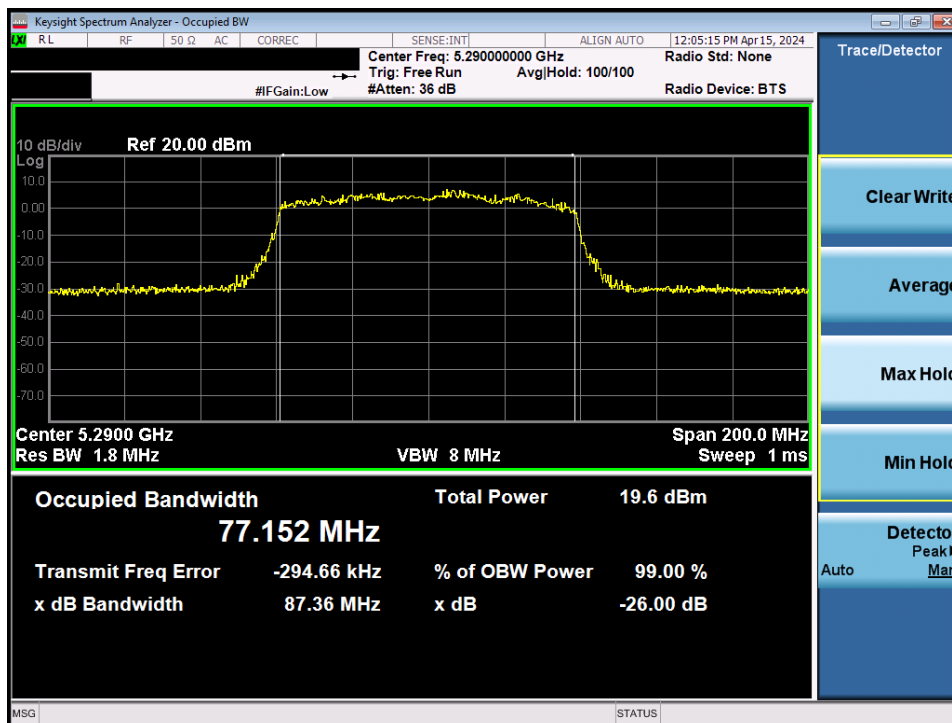
Plot 7-20. 26dB Bandwidth Plot MIMO ANT1 (80MHz BW 802.11be – 996 Tones (UNII Band 2A) – Ch. 58)
