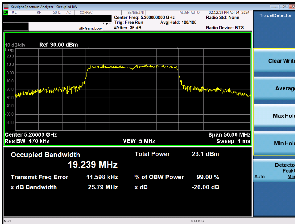
Plot 7-14. 26dB Bandwidth Plot MIMO ANT1 (20MHz BW 802.11be – 242 Tones (UNII Band 1) – Ch. 40)
