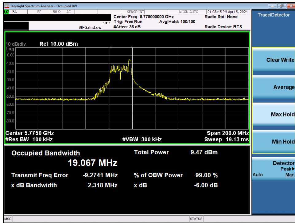
Plot 7-49. 6dB Bandwidth Plot MIMO ANT1 (80MHz BW 802.11be – 26 Tones (UNII Band 3) – Ch. 155)
