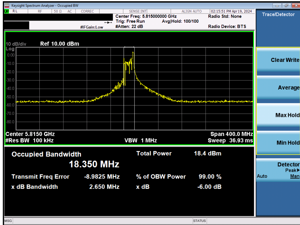
Plot 7-67. 6dB Bandwidth Plot MIMO ANT2 (160MHz BW 802.11be – 26 Tones (UNII Band 3/4) – Ch. 163)
