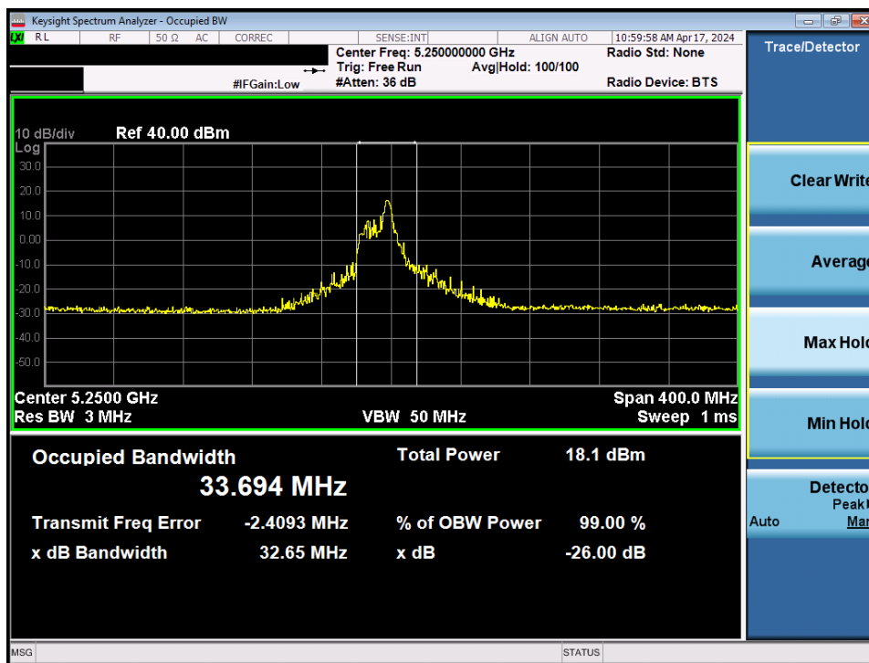
Plot 7-28. 26dB Bandwidth Plot MIMO ANT2 (160MHz BW 802.11be – 26 Tones (UNII Band 1/2A) – Ch. 50)
