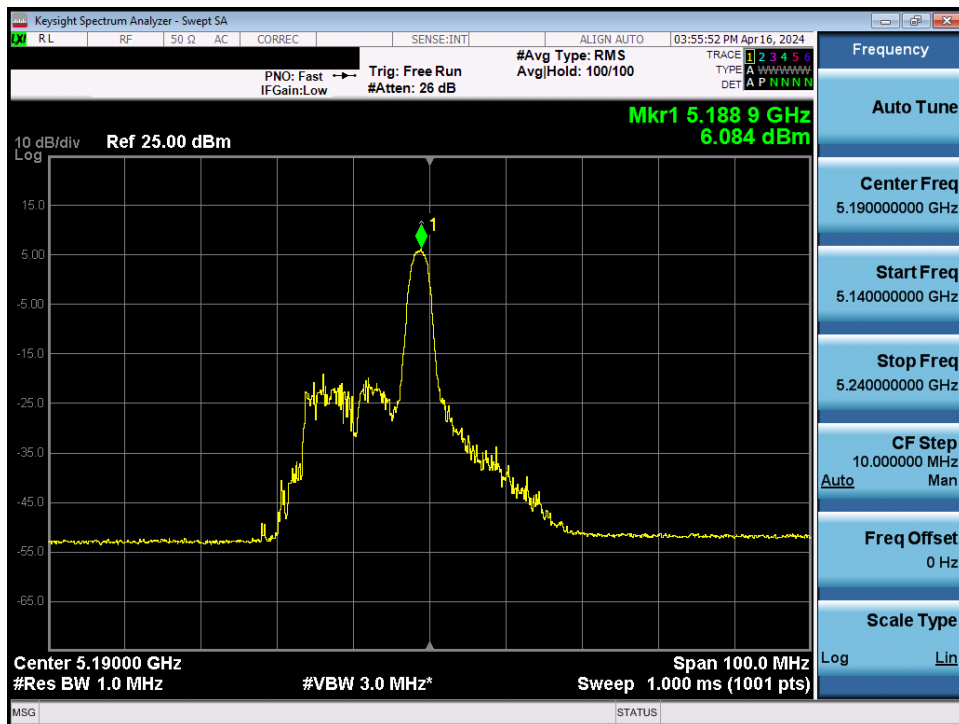
Plot 7-76. Power Spectral Density Plot MIMO ANT1 (40MHz BW 802.11be – 26 Tones (UNII Band 1) – Ch. 38)
