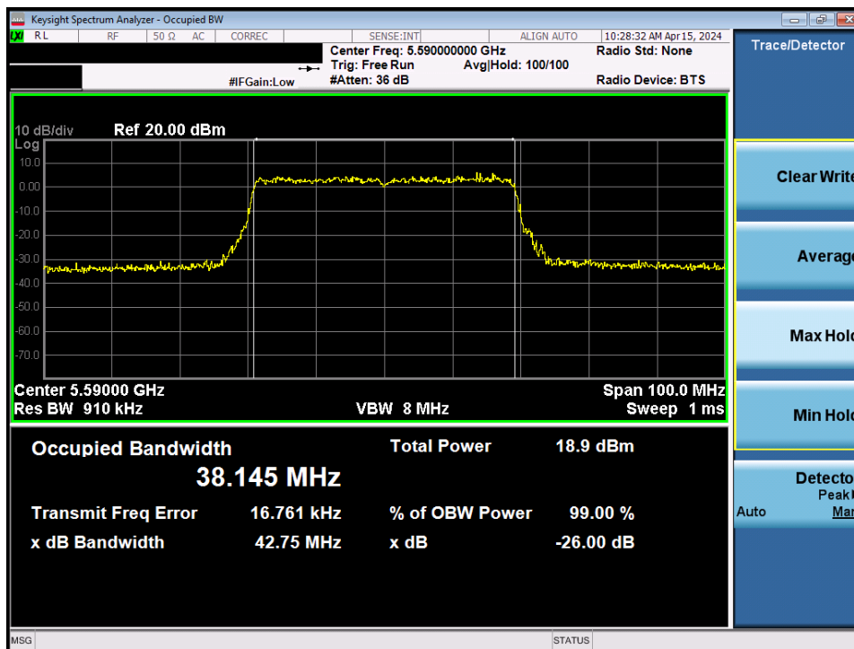
Plot 7-44. 26dB Bandwidth Plot MIMO ANT2 (40MHz BW 802.11be – 484 Tones (UNII Band 2C) – Ch. 118)
