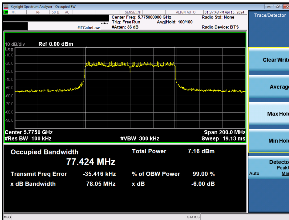
Plot 7-56. 6dB Bandwidth Plot MIMO ANT1 (80MHz BW 802.11be – 996 Tones (UNII Band 3) – Ch. 155)
