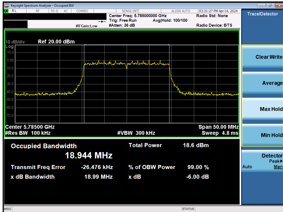
Plot 7-68. 6dB Bandwidth Plot MIMO ANT2 (20MHz BW 802.11be – 242 Tones (UNII Band 3) – Ch. 157)
