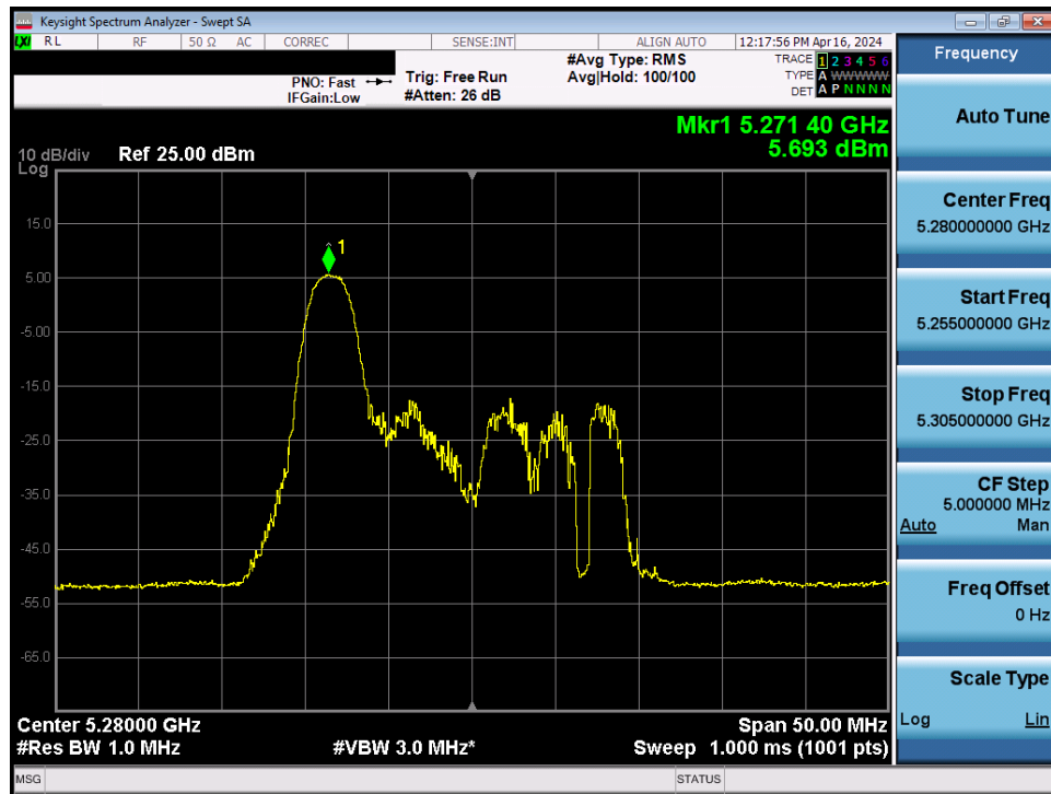
Plot 7-79. Power Spectral Density Plot MIMO ANT1 (20MHz BW 802.11be – 26 Tones (UNII Band 2A) – Ch. 56)
