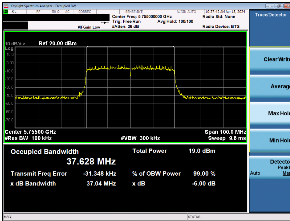
Plot 7-69. 6dB Bandwidth Plot MIMO ANT2 (40MHz BW 802.11be – 484 Tones (UNII Band 3) – Ch. 151)
