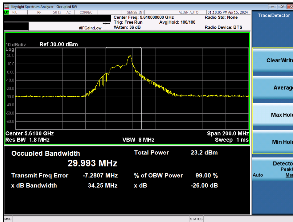
Plot 7-34. 26dB Bandwidth Plot MIMO ANT2 (80MHz BW 802.11be – 26 Tones (UNII Band 2C) – Ch. 122)
