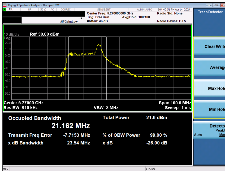
Plot 7-30. 26dB Bandwidth Plot MIMO ANT2 (40MHz BW 802.11be – 26 Tones (UNII Band 2A) – Ch. 54)
