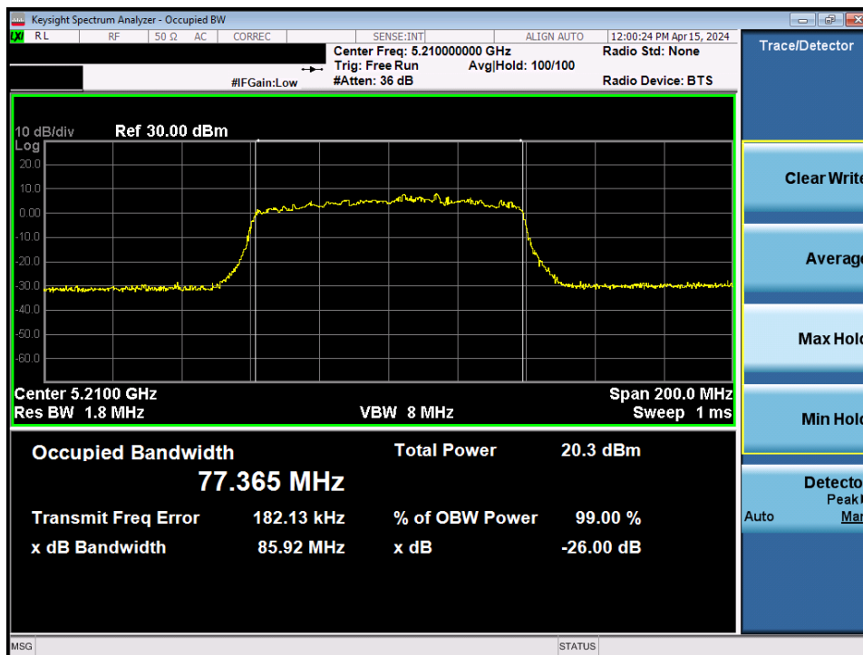
Plot 7-38. 26dB Bandwidth Plot MIMO ANT2 (80MHz BW 802.11be – 996 Tones (UNII Band 1) – Ch. 42)
