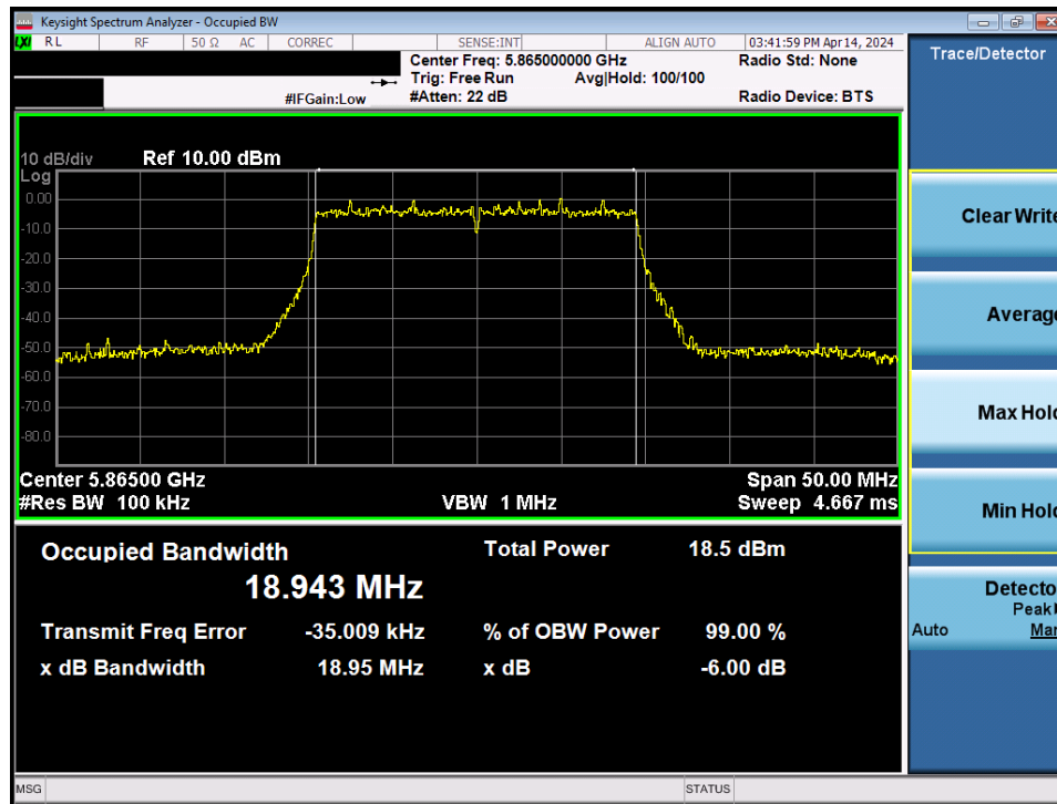
Plot 7-71. 6dB Bandwidth Plot MIMO ANT2 (20MHz BW 802.11be – 242 Tones (UNII Band 4) – Ch. 173)
