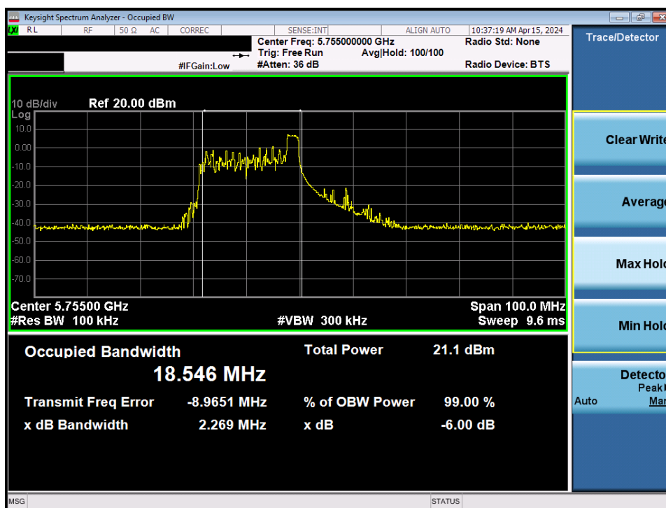
Plot 7-62. 6dB Bandwidth Plot MIMO ANT2 (40MHz BW 802.11be – 26 Tones (UNII Band 3) – Ch. 151)
