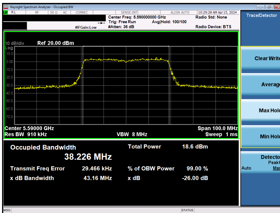
Plot 7-22. 26dB Bandwidth Plot MIMO ANT1 (40MHz BW 802.11be – 484 Tones (UNII Band 2C) – Ch. 118)
