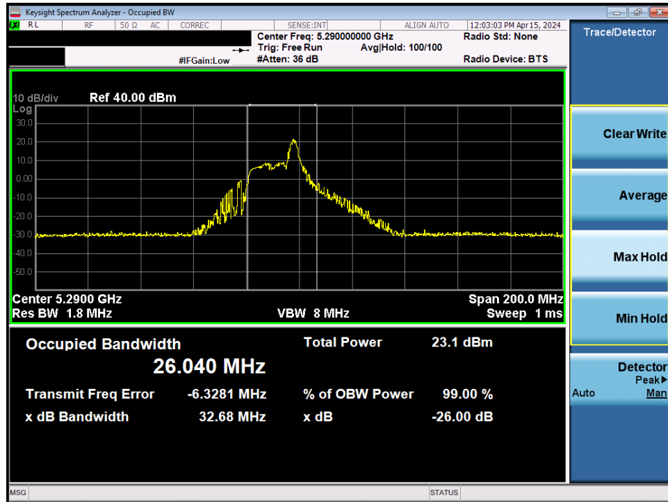
Plot 7-31. 26dB Bandwidth Plot MIMO ANT2 (80MHz BW 802.11be – 26 Tones (UNII Band 2A) – Ch. 58)
