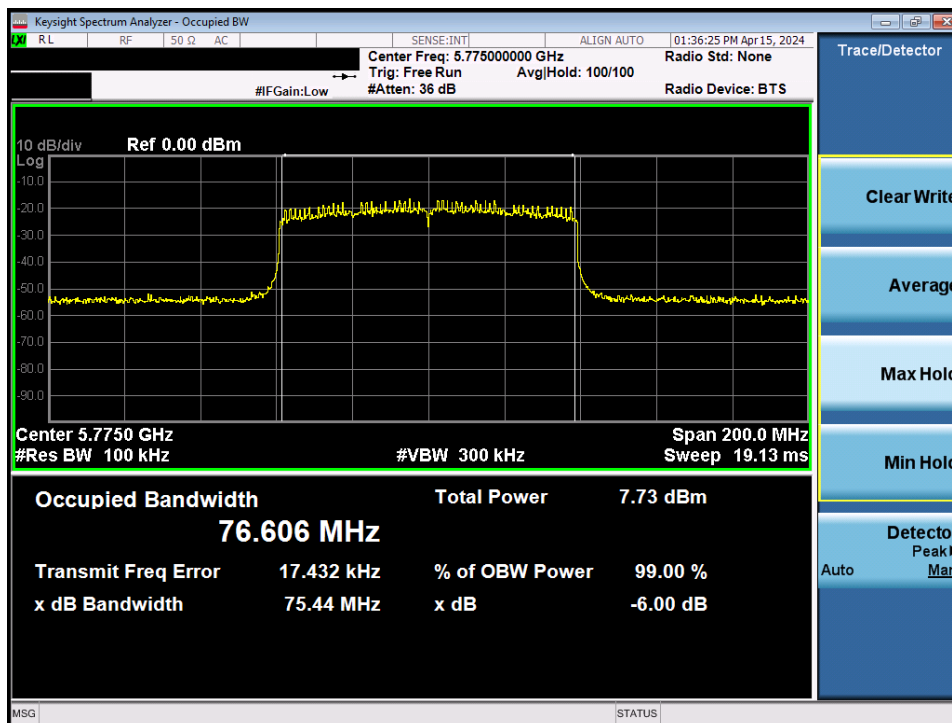
Plot 7-70. 6dB Bandwidth Plot MIMO ANT2 (80MHz BW 802.11be – 996 Tones (UNII Band 3) – Ch. 155)
