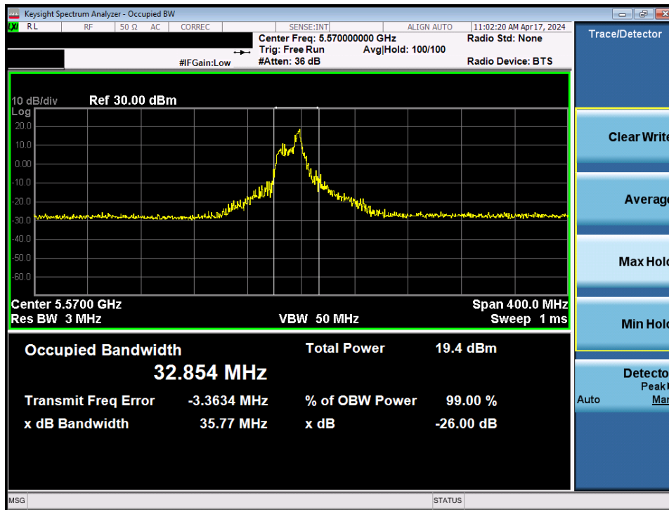
Plot 7-35. 26dB Bandwidth Plot MIMO ANT2 (160MHz BW 802.11be – 26 Tones (UNII Band 2C) – Ch. 114)
