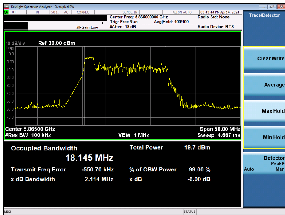
Plot 7-50. 6dB Bandwidth Plot MIMO ANT1 (20MHz BW 802.11be – 26 Tones (UNII Band 4) – Ch. 173)
