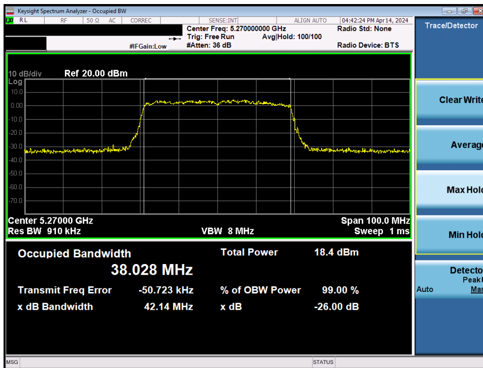
Plot 7-19. 26dB Bandwidth Plot MIMO ANT1 (40MHz BW 802.11be – 484 Tones (UNII Band 2A) – Ch. 54)
