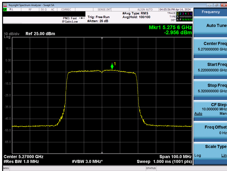
Plot 7-98. Power Spectral Density Plot MIMO ANT1 (40MHz BW 802.11be – 484 Tones (UNII Band 2A) – Ch. 54)
