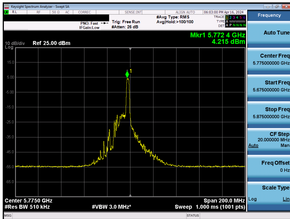
Plot 7-88. Power Spectral Density Plot MIMO ANT1 (80MHz BW 802.11be – 26 Tones (UNII Band 3) – Ch. 155)
