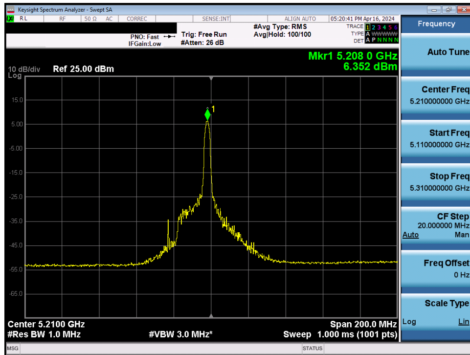
Plot 7-77. Power Spectral Density Plot MIMO ANT1 (80MHz BW 802.11be – 26 Tones (UNII Band 1) – Ch. 42)
