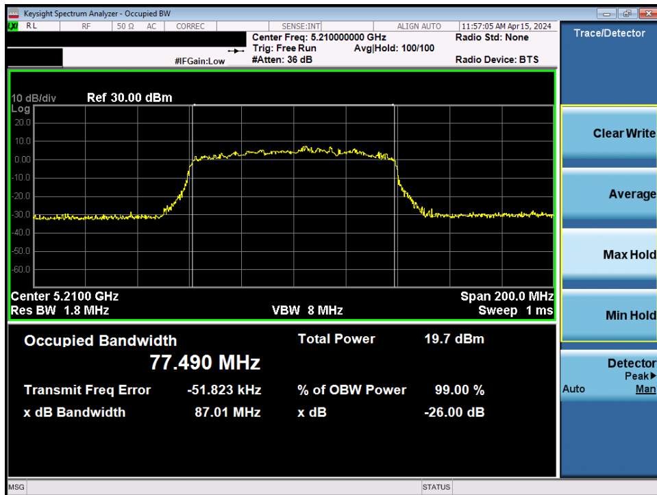
Plot 7-16. 26dB Bandwidth Plot MIMO ANT1 (80MHz BW 802.11be – 996 Tones (UNII Band 1) – Ch. 42)
