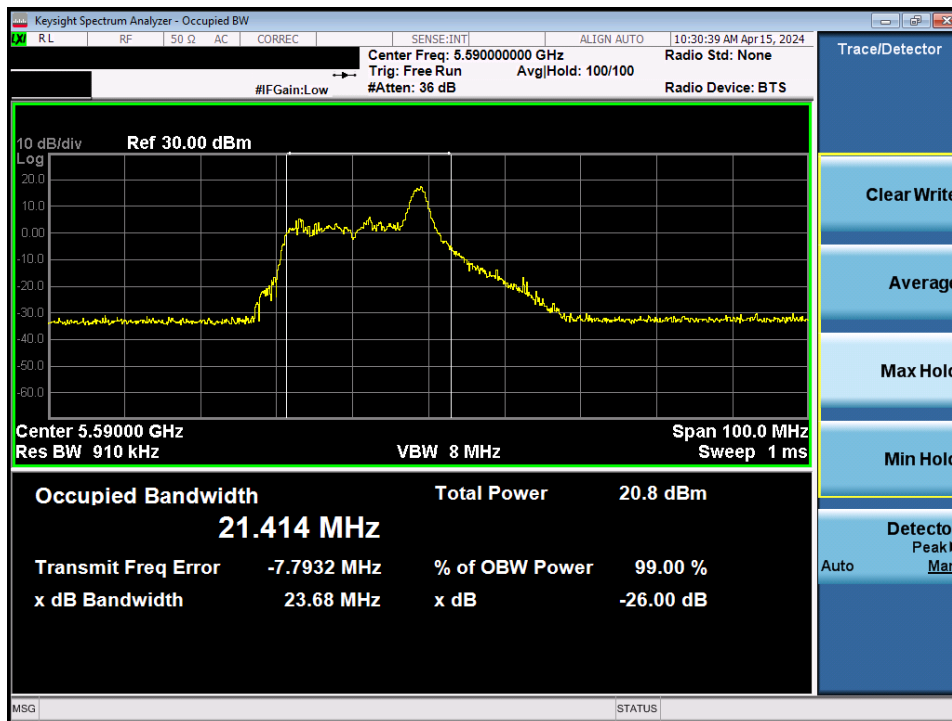
Plot 7-11. 26dB Bandwidth Plot MIMO ANT1 (40MHz BW 802.11be – 26 Tones (UNII Band 2C) – Ch. 118)
