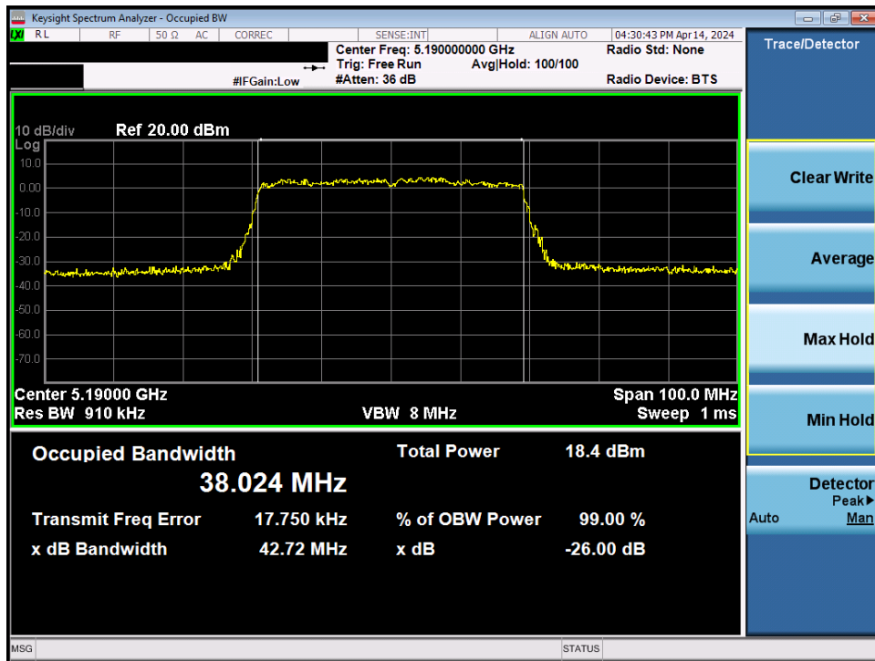
Plot 7-15. 26dB Bandwidth Plot MIMO ANT1 (40MHz BW 802.11be – 484 Tones (UNII Band 1) – Ch. 38)
