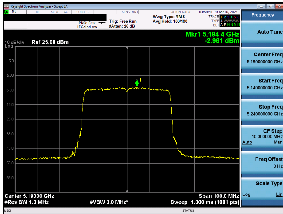
Plot 7-94. Power Spectral Density Plot MIMO ANT1 (40MHz BW 802.11be – 484 Tones (UNII Band 1) – Ch. 38)
