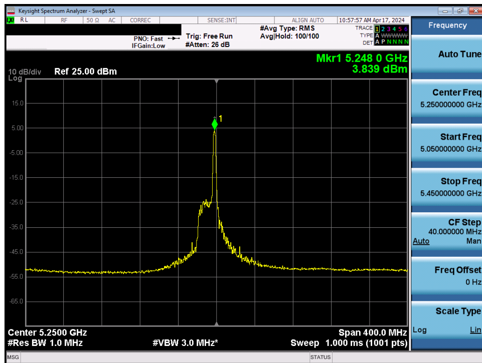
Plot 7-78. Power Spectral Density Plot MIMO ANT1 (160MHz BW 802.11be – 26 Tones (UNII Band 1/2A) – Ch. 50)
