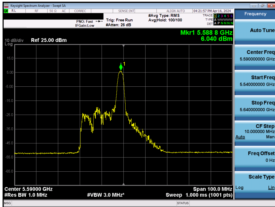
Plot 7-83. Power Spectral Density Plot MIMO ANT1 (40MHz BW 802.11be – 26 Tones (UNII Band 2C) – Ch. 118)
