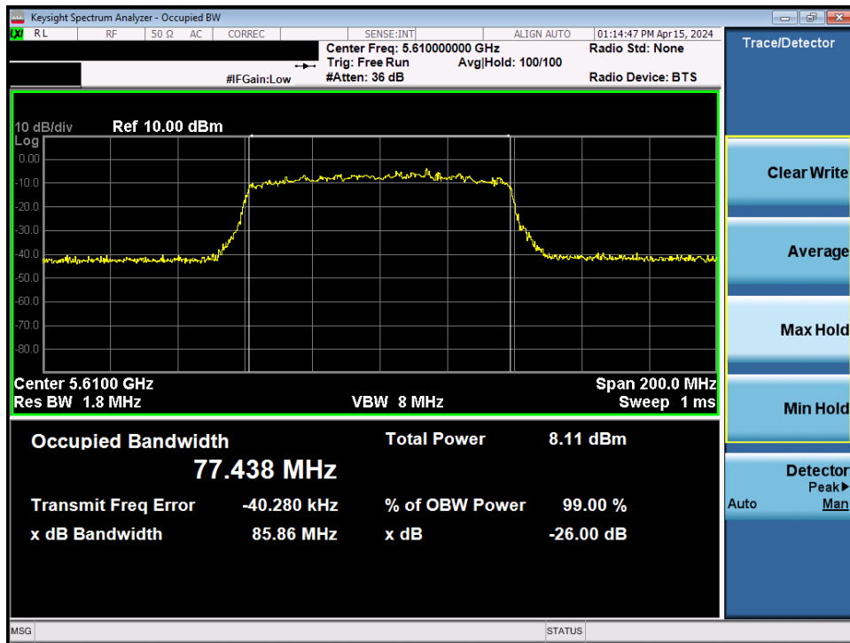
Plot 7-45. 26dB Bandwidth Plot MIMO ANT2 (80MHz BW 802.11be – 996 Tones (UNII Band 2C) – Ch. 122)
