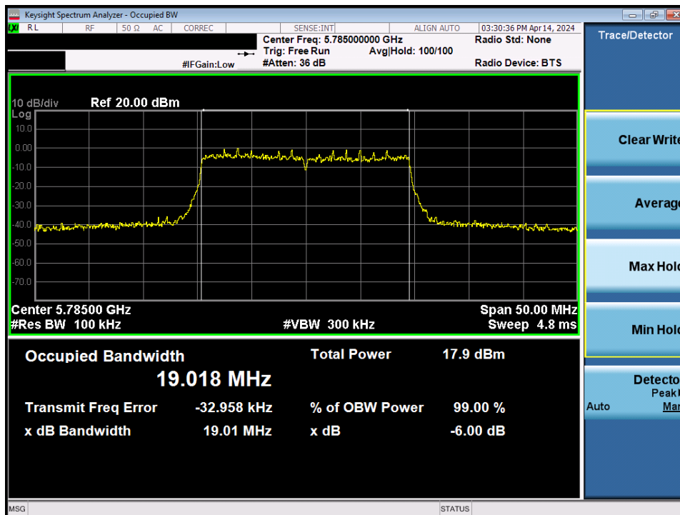
Plot 7-54. 6dB Bandwidth Plot MIMO ANT1 (20MHz BW 802.11be – 242 Tones (UNII Band 3) – Ch. 157)
