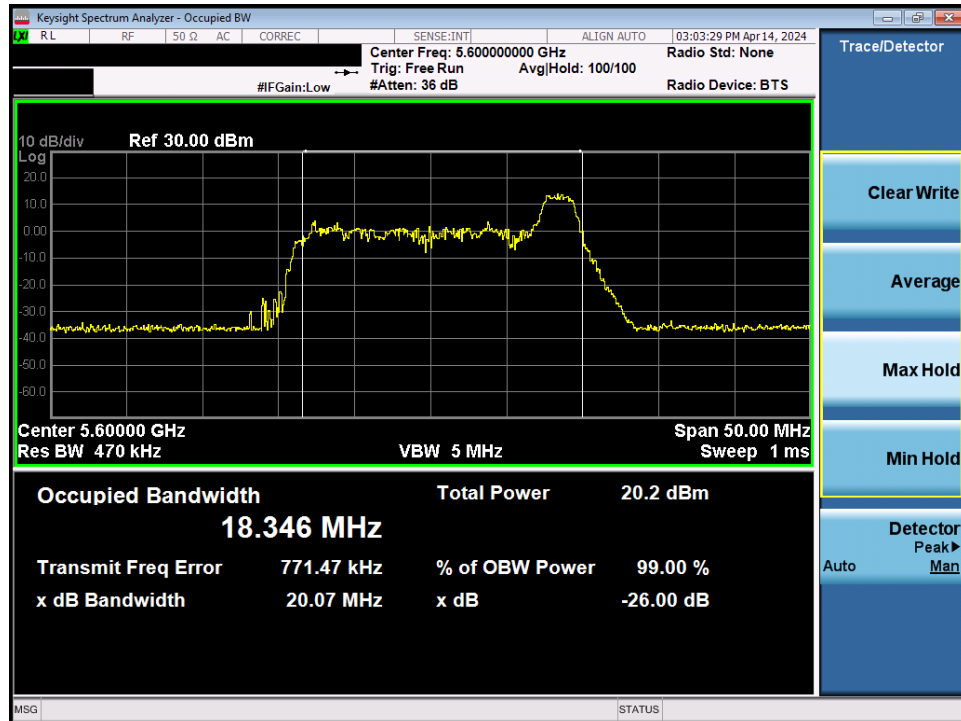
Plot 7-32. 26dB Bandwidth Plot MIMO ANT2 (20MHz BW 802.11be – 26 Tones (UNII Band 2C) – Ch. 120)
