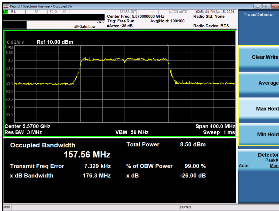
Plot 7-24. 26dB Bandwidth Plot MIMO ANT1 (160MHz BW 802.11be – 2x996 Tones (UNII Band 2C) – Ch. 114)
