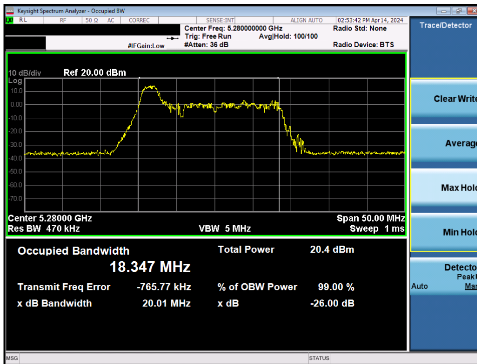
Plot 7-29. 26dB Bandwidth Plot MIMO ANT2 (20MHz BW 802.11be – 26 Tones (UNII Band 2A) – Ch. 56)
