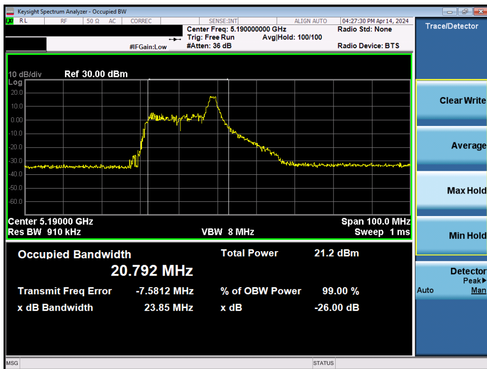
Plot 7-26. 26dB Bandwidth Plot MIMO ANT2 (40MHz BW 802.11be – 26 Tones (UNII Band 1) – Ch. 38)
