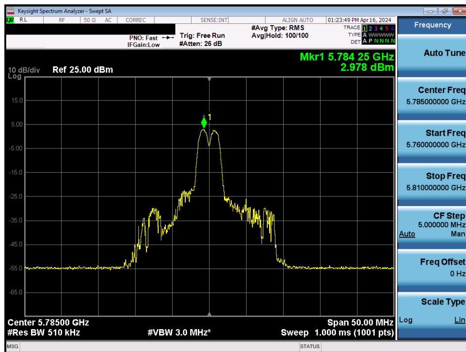
Plot 7-86. Power Spectral Density Plot MIMO ANT1 (20MHz BW 802.11be – 26 Tones (UNII Band 3) – Ch. 157)
