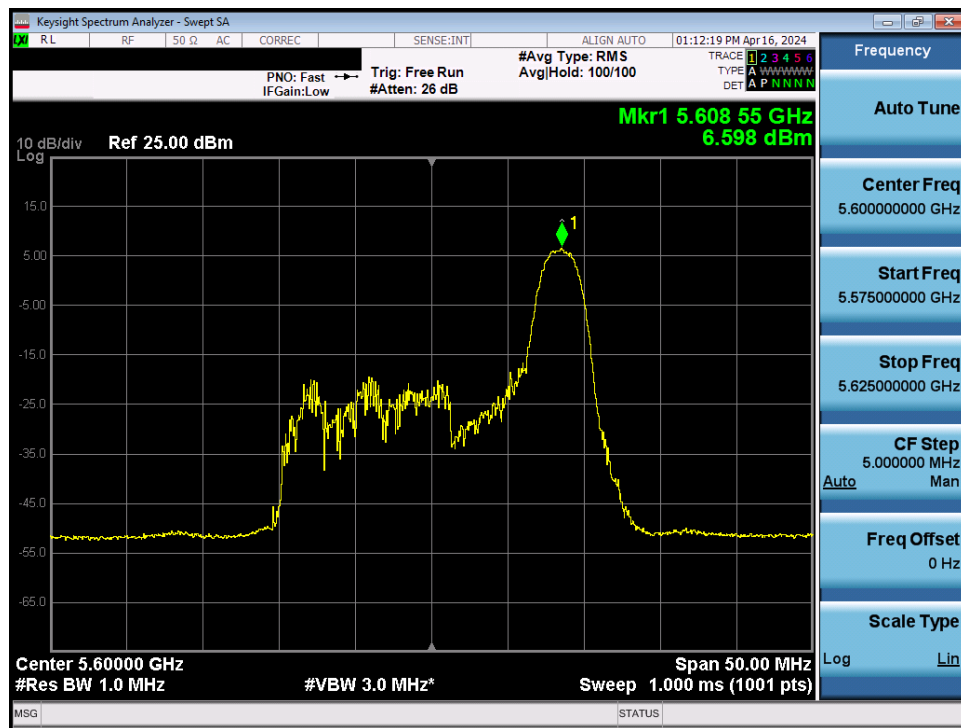
Plot 7-82. Power Spectral Density Plot MIMO ANT1 (20MHz BW 802.11be – 26 Tones (UNII Band 2C) – Ch. 120)
