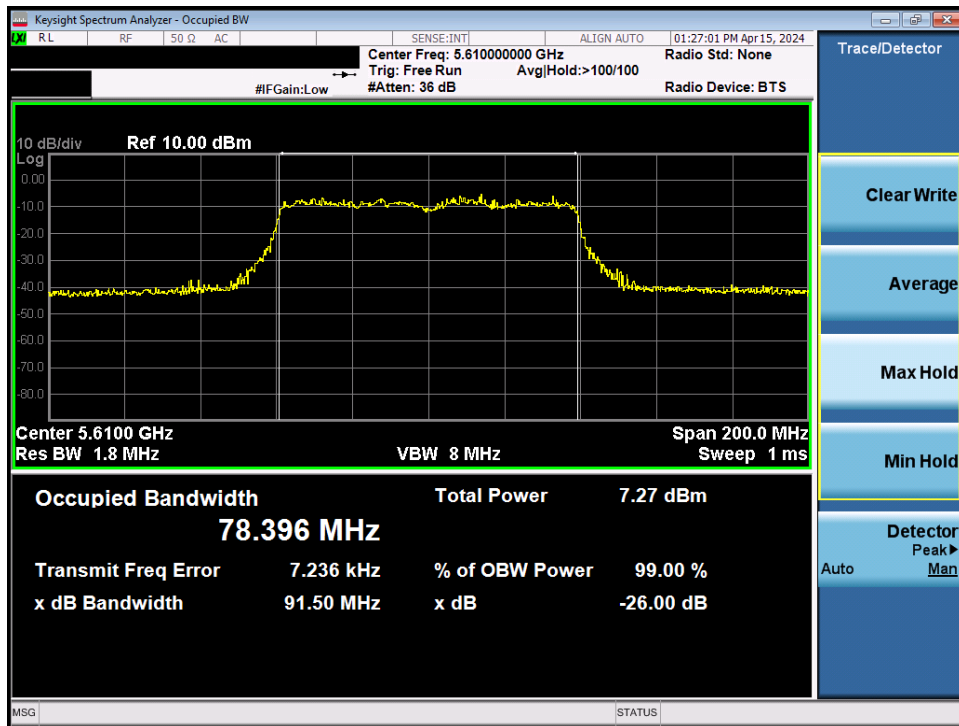
Plot 7-23. 26dB Bandwidth Plot MIMO ANT1 (80MHz BW 802.11be – 996 Tones (UNII Band 2C) – Ch. 122)
