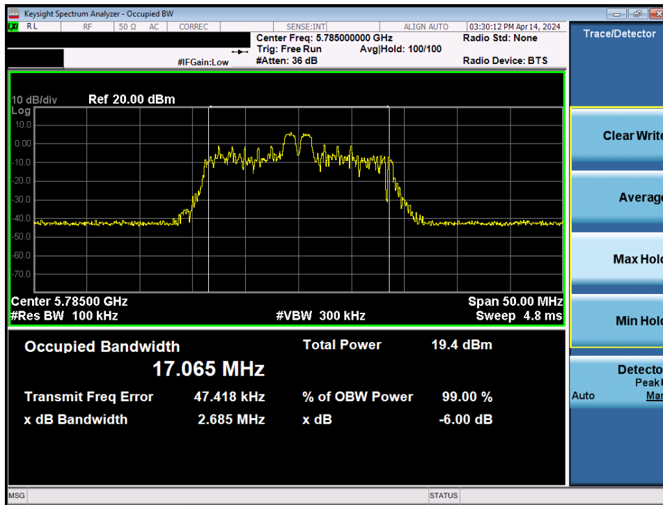
Plot 7-47. 6dB Bandwidth Plot MIMO ANT1 (20MHz BW 802.11be - 26 Tones (UNII Band 3) - Ch. 157)
