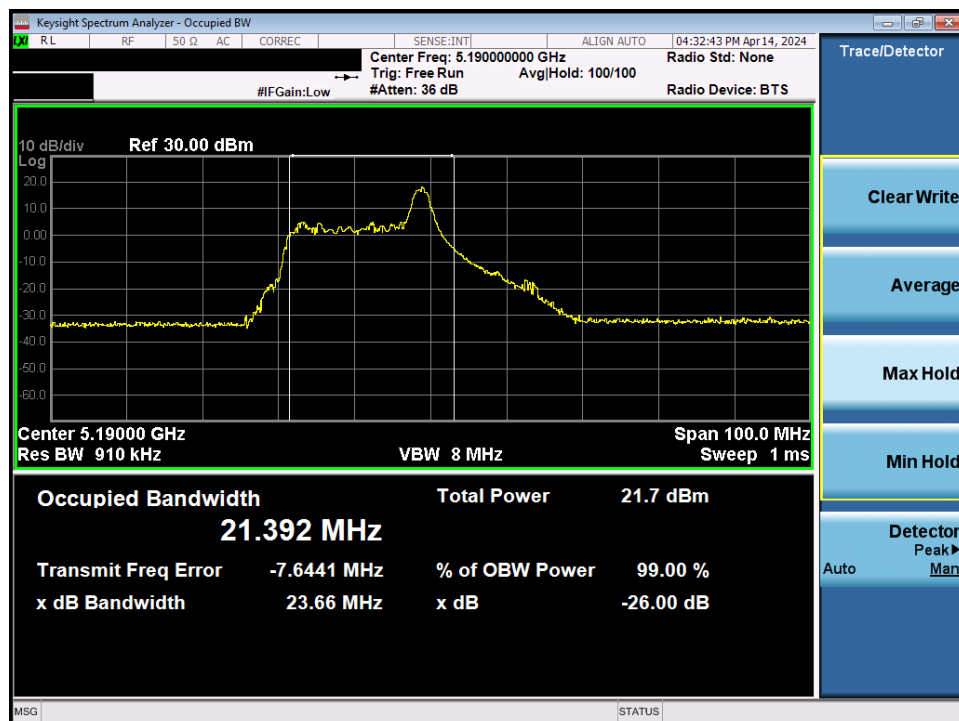
Plot 7-4. 26dB Bandwidth Plot MIMO ANT1 (40MHz BW 802.11be – 26 Tones (UNII Band 1) – Ch. 38)
