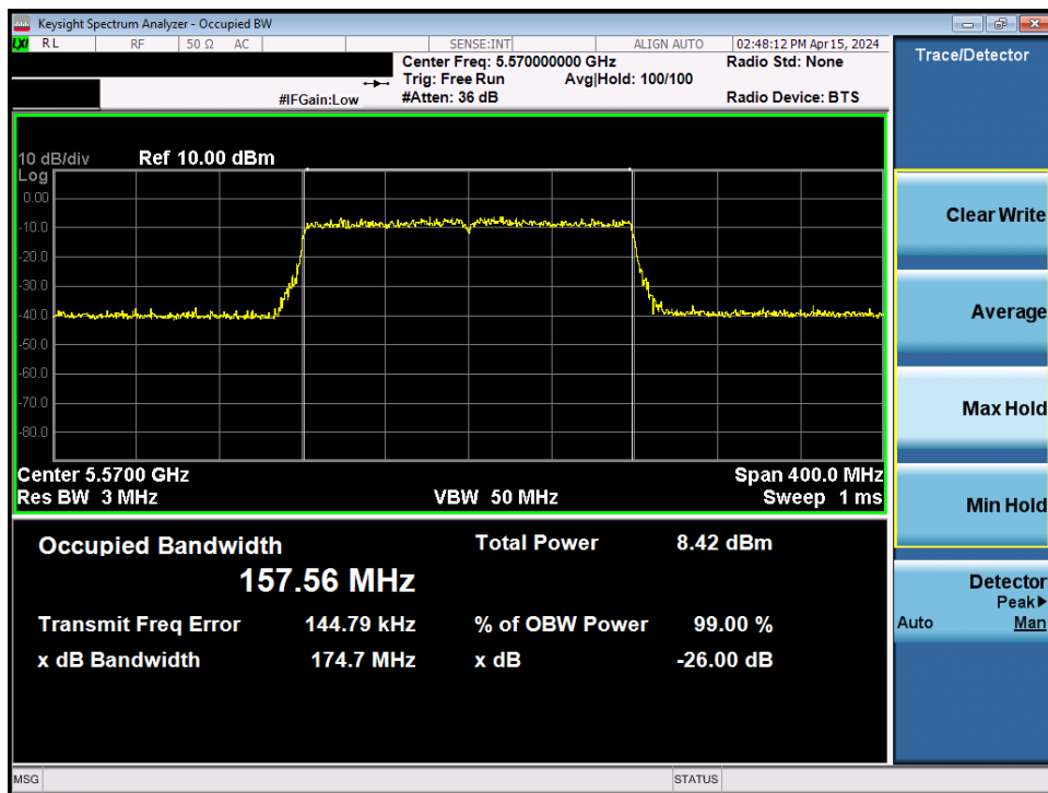
Plot 7-46. 26dB Bandwidth Plot MIMO ANT2 (160MHz BW 802.11be – 2x996 Tones (UNII Band 2C) – Ch. 114)
