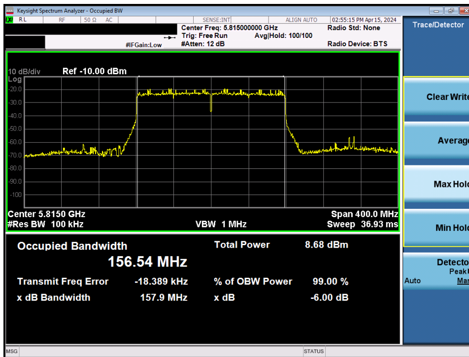
Plot 7-74. 6dB Bandwidth Plot MIMO ANT2 (160MHz BW 802.11be – 996*2 Tones (UNII Band 3/4) – Ch. 163)
