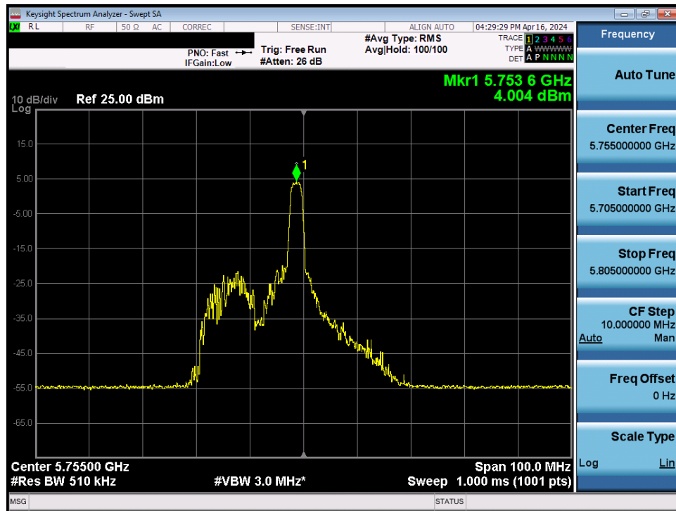
Plot 7-87. Power Spectral Density Plot MIMO ANT1 (40MHz BW 802.11be – 26 Tones (UNII Band 3) – Ch. 151)
