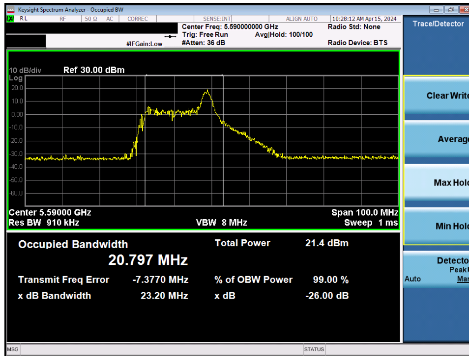
Plot 7-33. 26dB Bandwidth Plot MIMO ANT2 (40MHz BW 802.11be – 26 Tones (UNII Band 2C) – Ch. 118)
