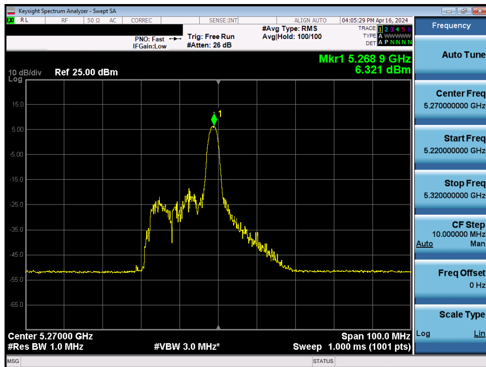
Plot 7-80. Power Spectral Density Plot MIMO ANT1 (40MHz BW 802.11be – 26 Tones (UNII Band 2A) – Ch. 54)
