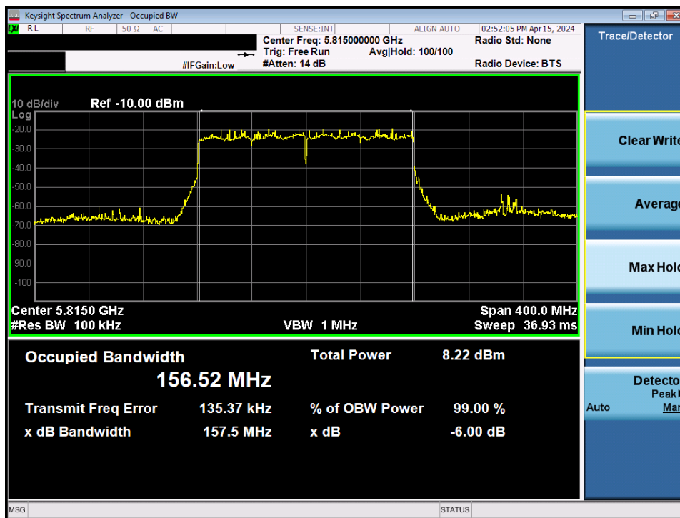
Plot 7-60. 6dB Bandwidth Plot MIMO ANT1 (160MHz BW 802.11be – 996*2 Tones (UNII Band 3/4) – Ch. 163)
