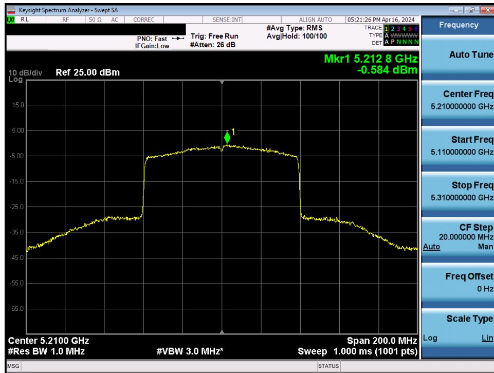
Plot 7-95. Power Spectral Density Plot MIMO ANT1 (80MHz BW 802.11be – 996 Tones (UNII Band 1) – Ch. 42)
