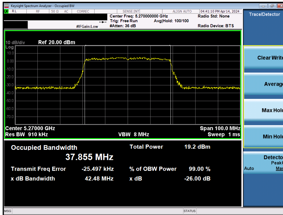
Plot 7-41. 26dB Bandwidth Plot MIMO ANT2 (40MHz BW 802.11be – 484 Tones (UNII Band 2A) – Ch. 54)
