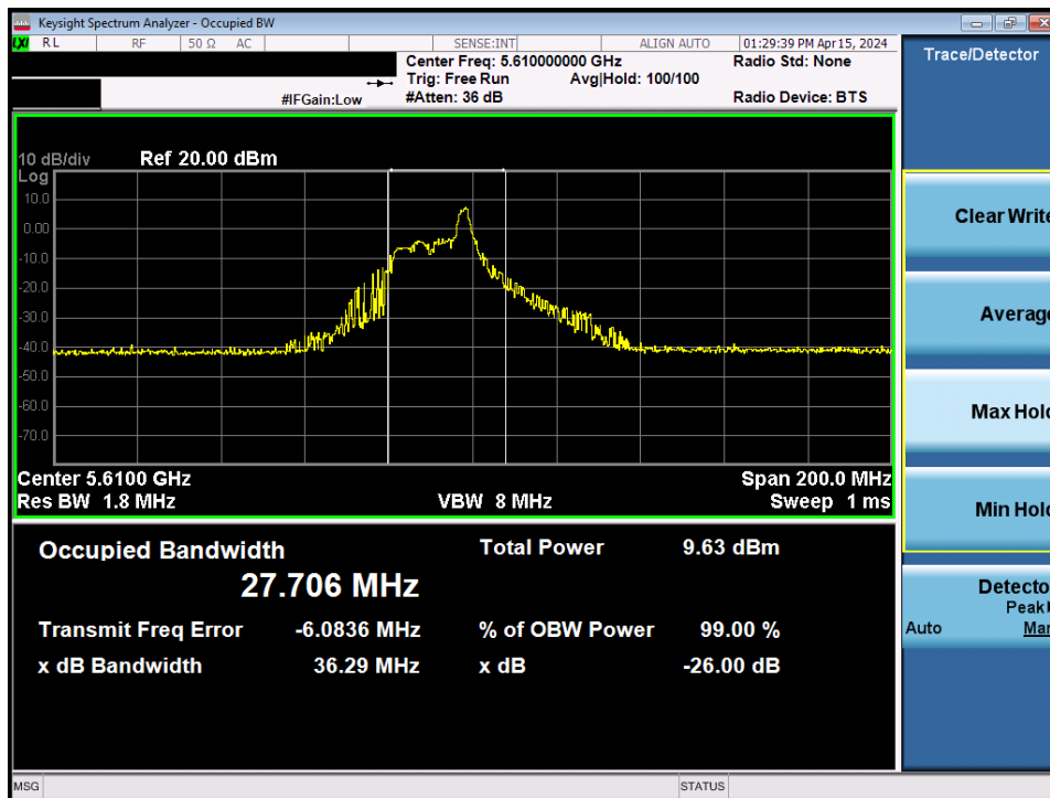
Plot 7-12. 26dB Bandwidth Plot MIMO ANT1 (80MHz BW 802.11be – 26 Tones (UNII Band 2C) – Ch. 122)
