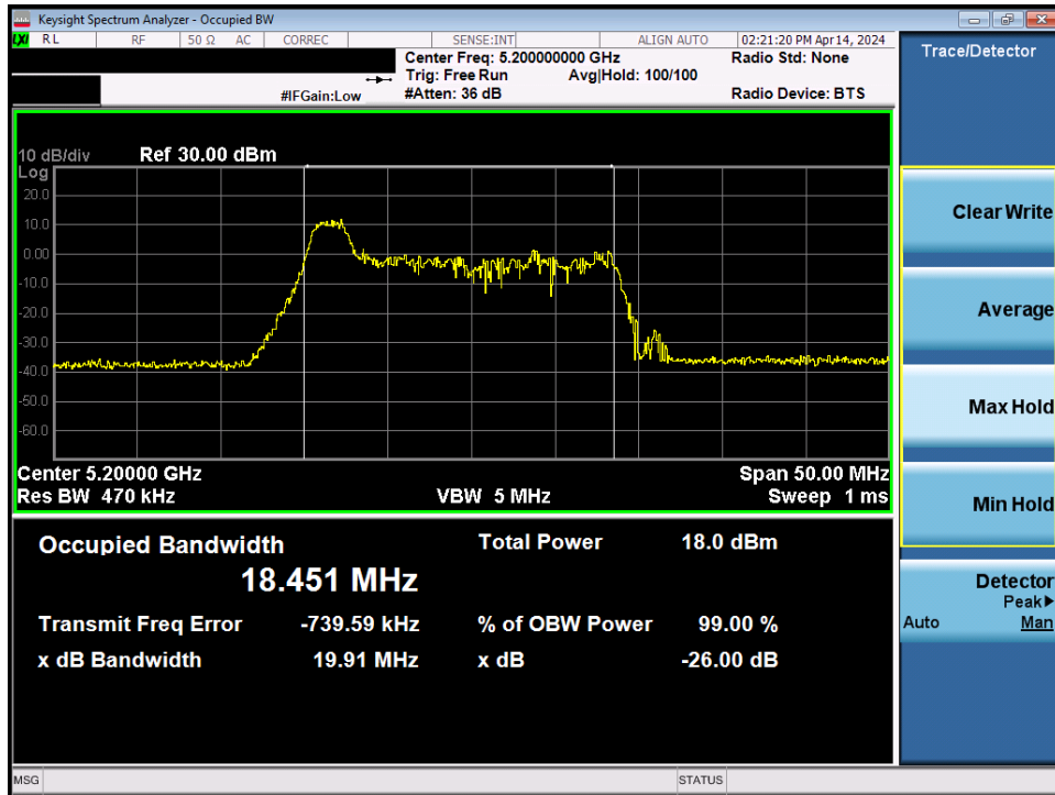
Plot 7-25. 26dB Bandwidth Plot MIMO ANT2 (20MHz BW 802.11be – 26 Tones (UNII Band 1) – Ch. 40)
