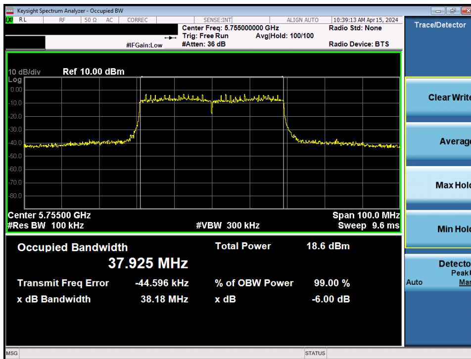
Plot 7-55. 6dB Bandwidth Plot MIMO ANT1 (40MHz BW 802.11be – 484 Tones (UNII Band 3) – Ch. 151)
