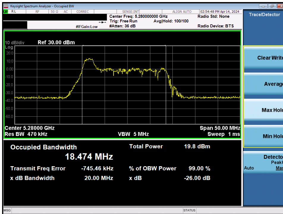
Plot 7-7. 26dB Bandwidth Plot MIMO ANT1 (20MHz BW 802.11be – 26 Tones (UNII Band 2A) – Ch. 56)
