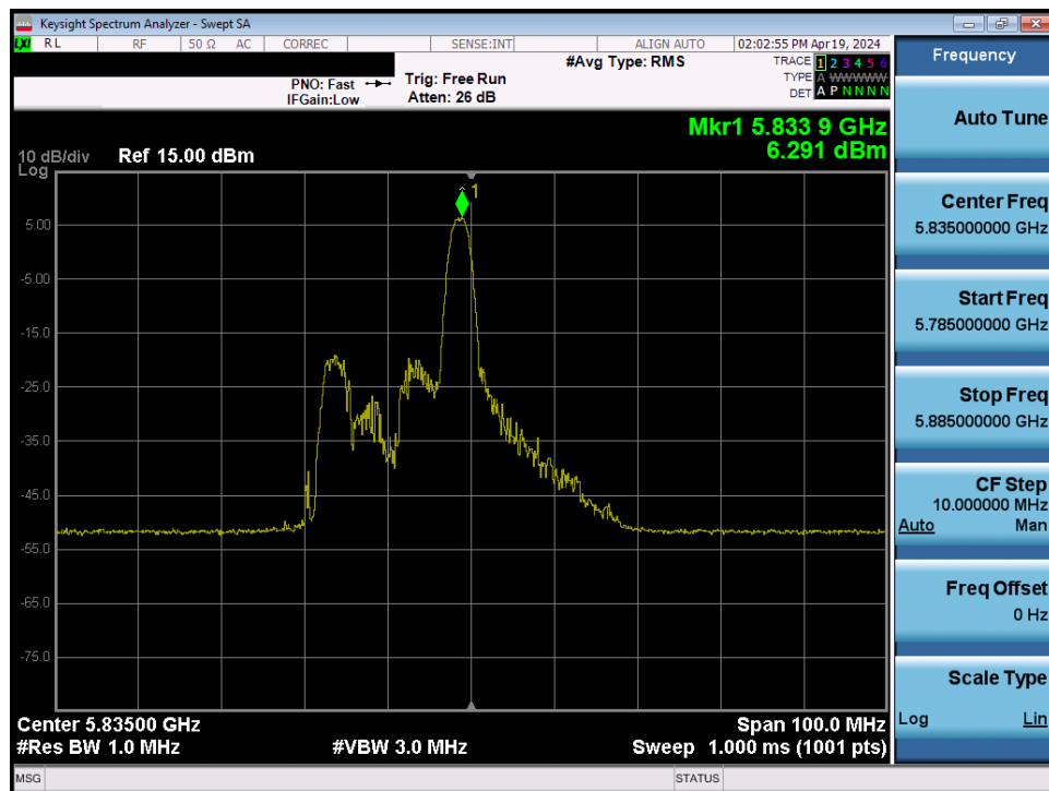
Plot 7-90. Power Spectral Density Plot MIMO ANT1 (40MHz BW 802.11be – 26 Tones (UNII Band 3/4) – Ch. 167)
