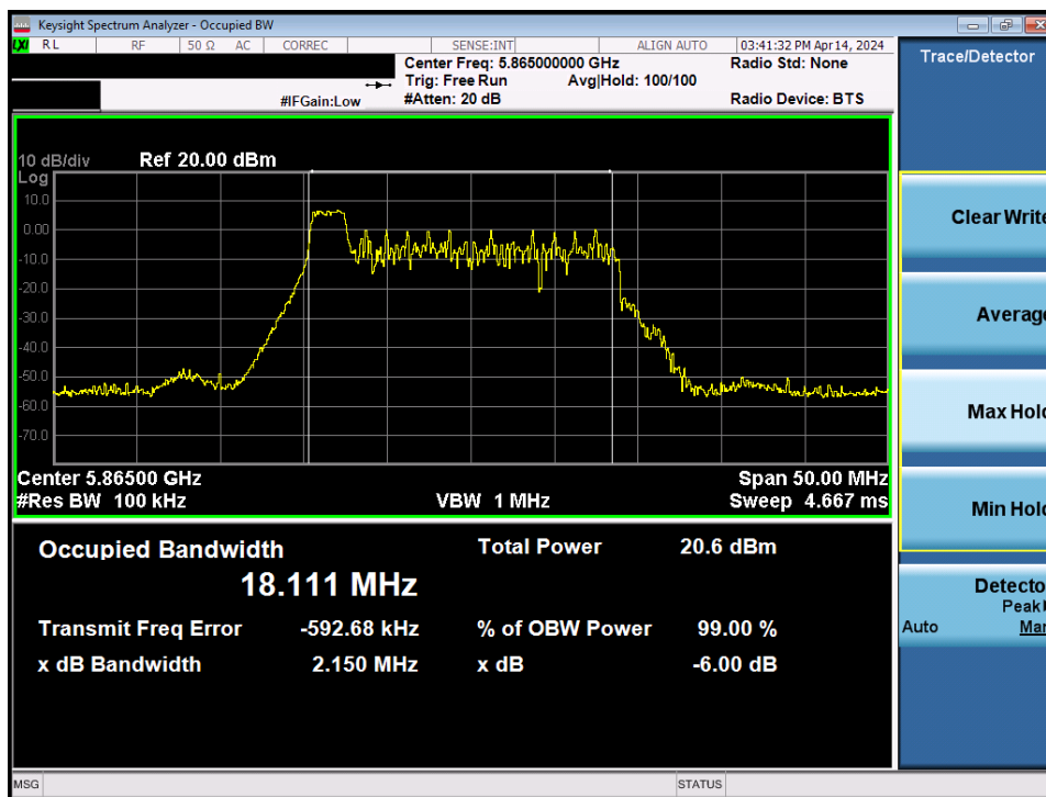
Plot 7-64. 6dB Bandwidth Plot MIMO ANT2 (20MHz BW 802.11be – 26 Tones (UNII Band 4) – Ch. 173)
