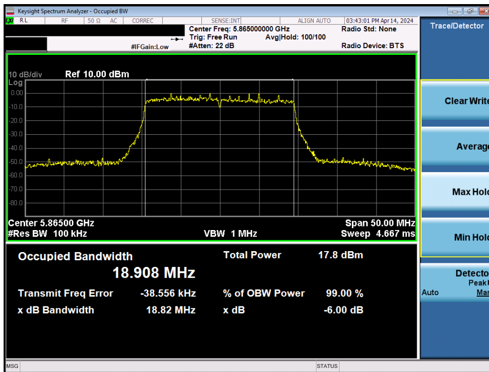
Plot 7-57. 6dB Bandwidth Plot MIMO ANT1 (20MHz BW 802.11be – 242 Tones (UNII Band 4) – Ch. 173)
