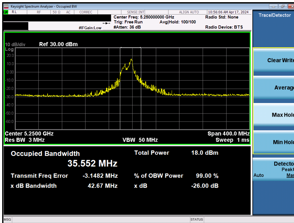
Plot 7-6. 26dB Bandwidth Plot MIMO ANT1 (160MHz BW 802.11be – 26 Tones (UNII Band 1/2A) – Ch. 50)
