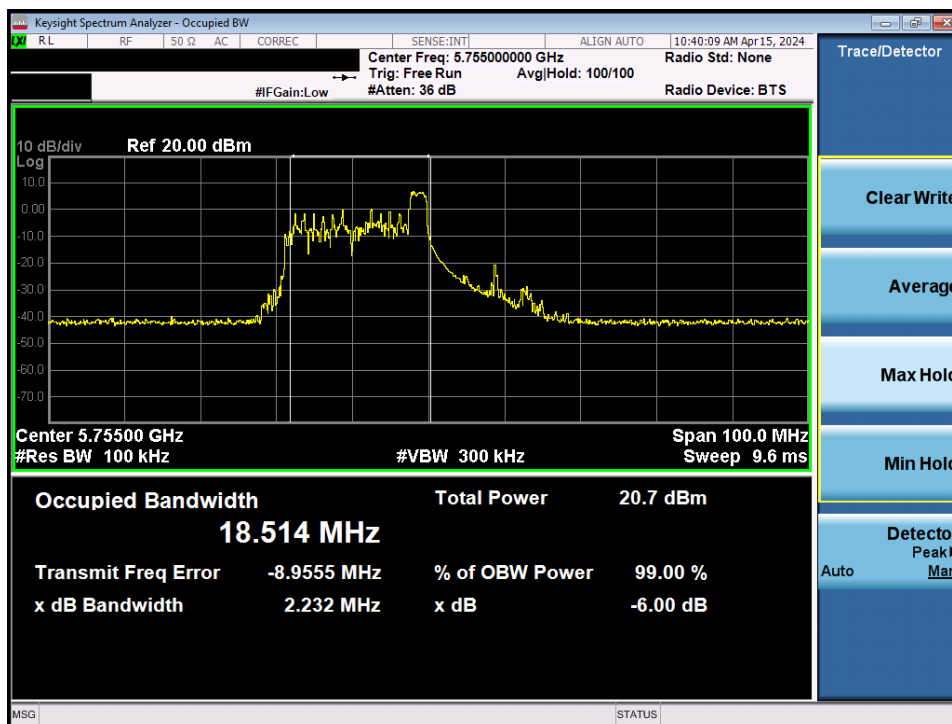
Plot 7-48. 6dB Bandwidth Plot MIMO ANT1 (40MHz BW 802.11be - 26 Tones (UNII Band 3) - Ch. 151)
