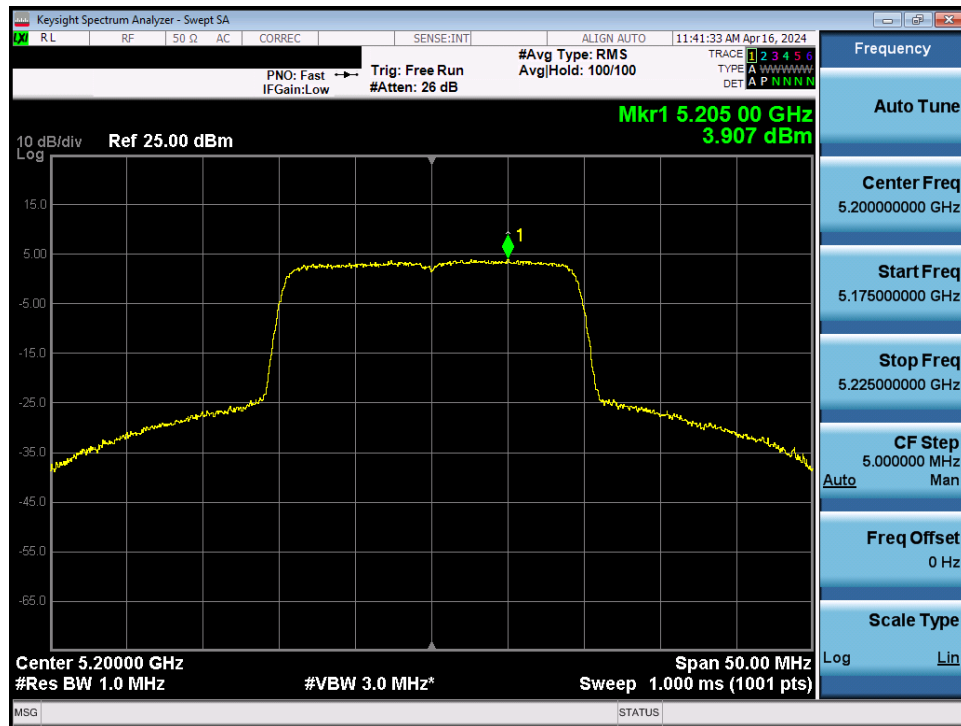
Plot 7-93. Power Spectral Density Plot MIMO ANT1 (20MHz BW 802.11be – 242 Tones (UNII Band 1) – Ch. 40)
