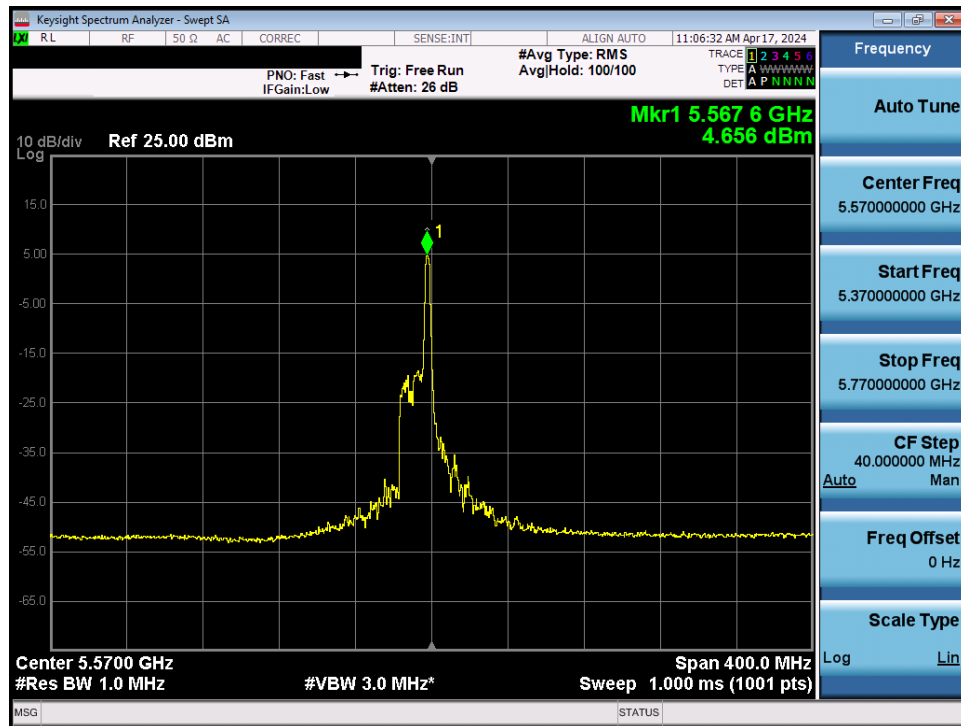
Plot 7-85. Power Spectral Density Plot MIMO ANT1 (160MHz BW 802.11be – 26 Tones (UNII Band 2C) – Ch. 114)
