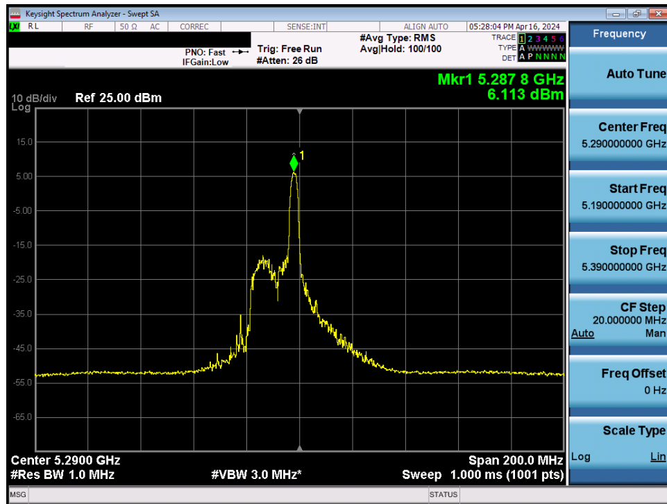
Plot 7-81. Power Spectral Density Plot MIMO ANT1 (80MHz BW 802.11be – 26 Tones (UNII Band 2A) – Ch. 58)
