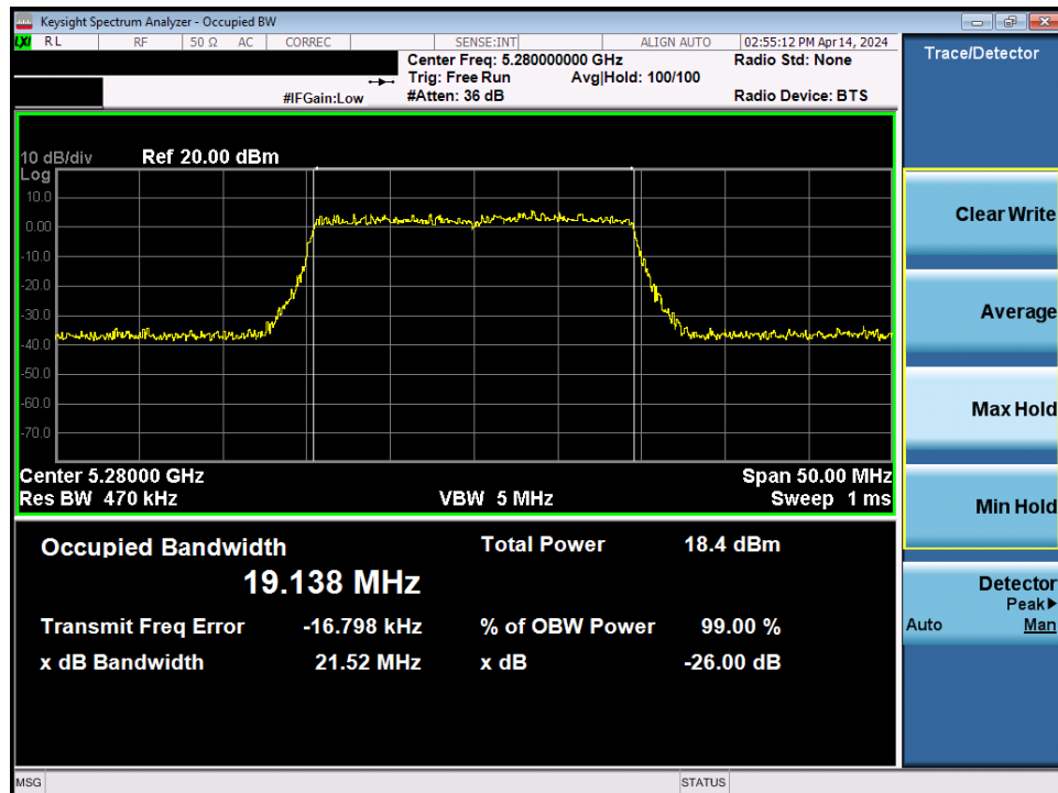
Plot 7-18. 26dB Bandwidth Plot MIMO ANT1 (20MHz BW 802.11be – 242 Tones (UNII Band 2A) – Ch. 56)
