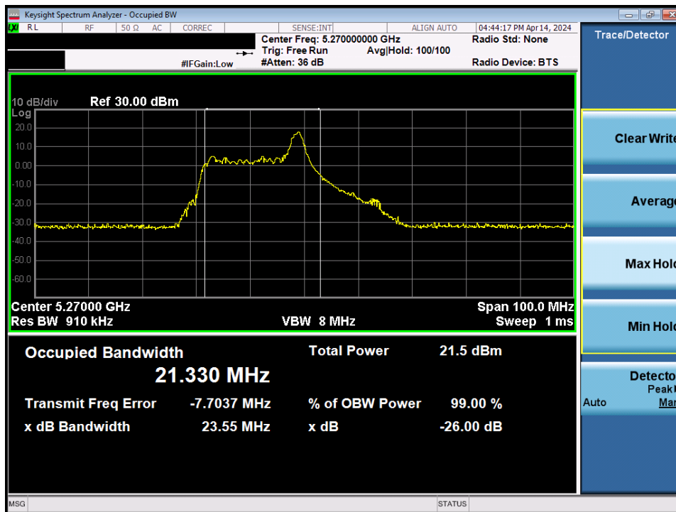
Plot 7-8. 26dB Bandwidth Plot MIMO ANT1 (40MHz BW 802.11be – 26 Tones (UNII Band 2A) – Ch. 54)
