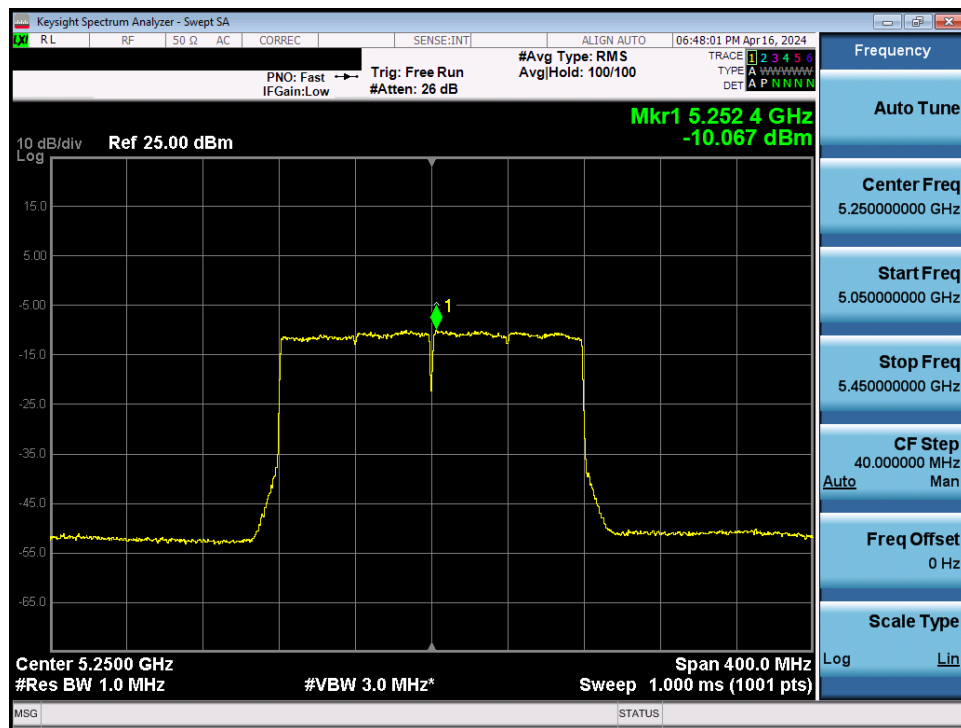
Plot 7-96. Power Spectral Density Plot MIMO ANT1 (160MHz BW 802.11be – 2x996 Tones (UNII Band 1/2A) – Ch. 50)
