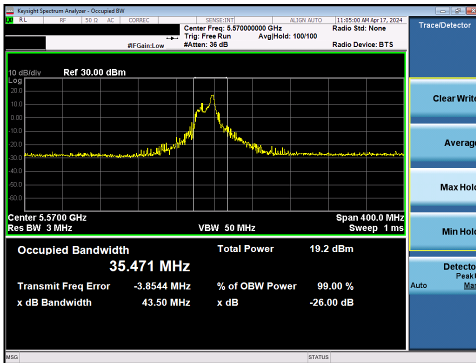
Plot 7-13. 26dB Bandwidth Plot MIMO ANT1 (160MHz BW 802.11be – 26 Tones (UNII Band 2C) – Ch. 114)
