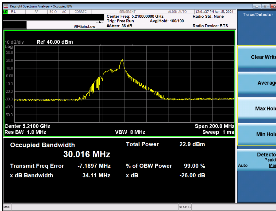
Plot 7-27. 26dB Bandwidth Plot MIMO ANT2 (80MHz BW 802.11be – 26 Tones (UNII Band 1) – Ch. 42)
