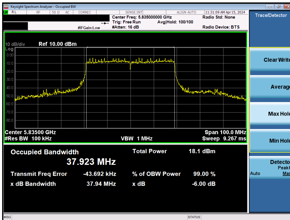
Plot 7-58. 6dB Bandwidth Plot MIMO ANT1 (40MHz BW 802.11be – 484 Tones (UNII Band 3/4) – Ch. 167)
