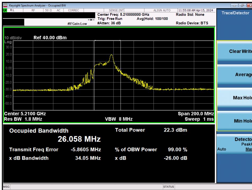
Plot 7-5. 26dB Bandwidth Plot MIMO ANT1 (80MHz BW 802.11be – 26 Tones (UNII Band 1) – Ch. 42)
