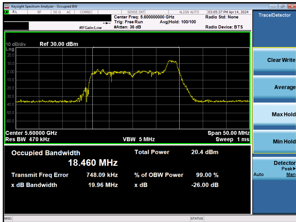
Plot 7-10. 26dB Bandwidth Plot MIMO ANT1 (20MHz BW 802.11be – 26 Tones (UNII Band 2C) – Ch. 120)
