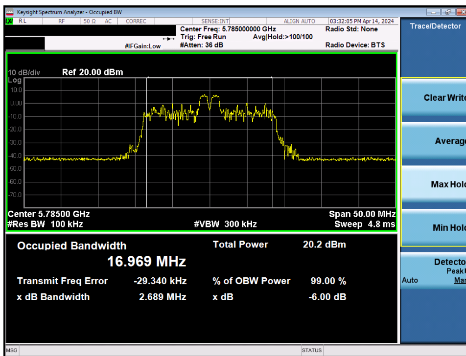
Plot 7-61. 6dB Bandwidth Plot MIMO ANT2 (20MHz BW 802.11be – 26 Tones (UNII Band 3) – Ch. 157)
