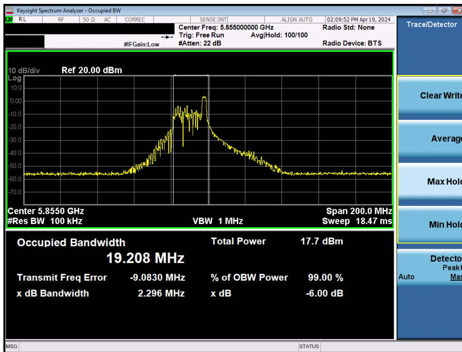
Plot 7-52. 6dB Bandwidth Plot MIMO ANT1 (80MHz BW 802.11be – 26 Tones (UNII Band 3/4) – Ch. 171)
