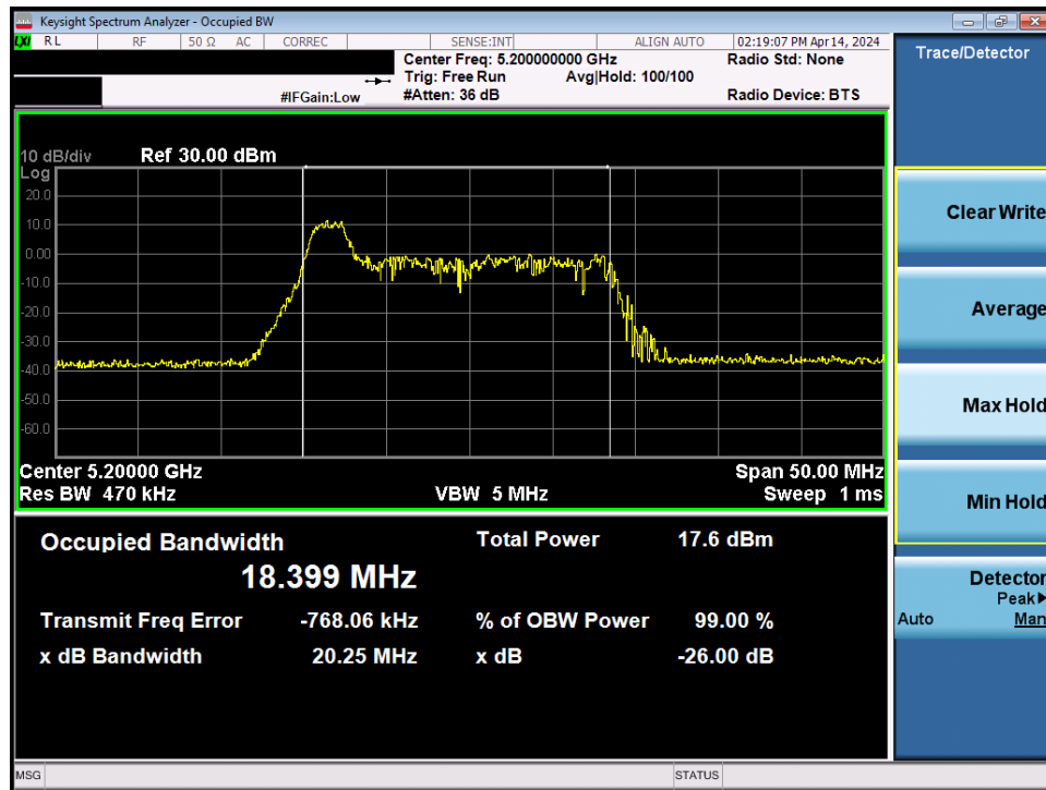
Plot 7-3. 26dB Bandwidth Plot MIMO ANT1 (20MHz BW 802.11be – 26 Tones (UNII Band 1) – Ch. 40)
