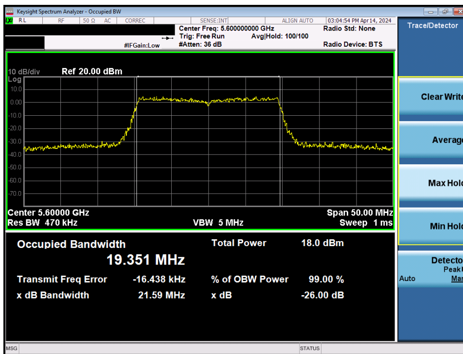
Plot 7-21. 26dB Bandwidth Plot MIMO ANT1 (20MHz BW 802.11be – 242 Tones (UNII Band 2C) – Ch. 120)
