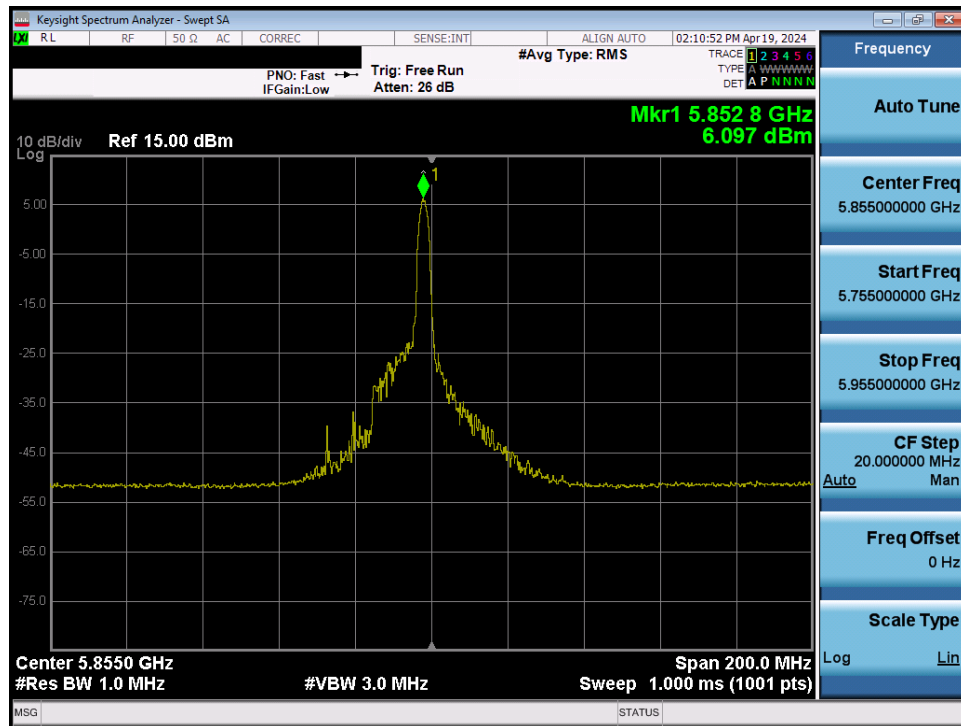
Plot 7-91. Power Spectral Density Plot MIMO ANT1 (80MHz BW 802.11be – 26 Tones (UNII Band 3/4) – Ch. 171)
