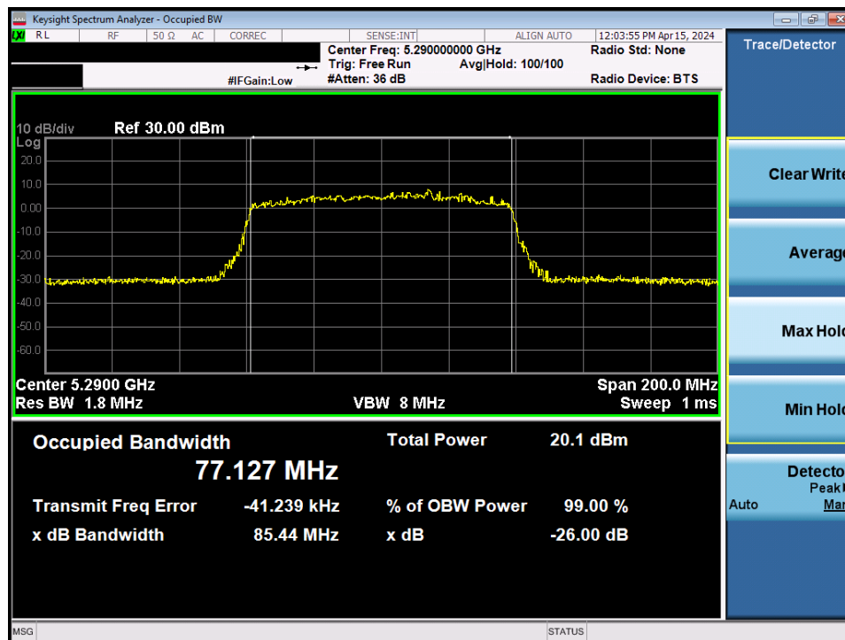
Plot 7-42. 26dB Bandwidth Plot MIMO ANT2 (80MHz BW 802.11be – 996 Tones (UNII Band 2A) – Ch. 58)
