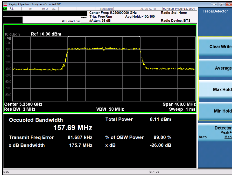
Plot 7-39. 26dB Bandwidth Plot MIMO ANT2 (160MHz BW 802.11be – 2x996 Tones (UNII Band 1/2A) – Ch. 50)
