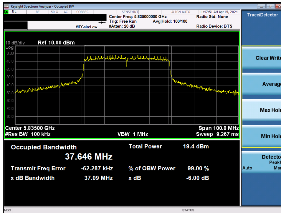
Plot 7-72. 6dB Bandwidth Plot MIMO ANT2 (40MHz BW 802.11be – 484 Tones (UNII Band 3/4) – Ch. 167)
