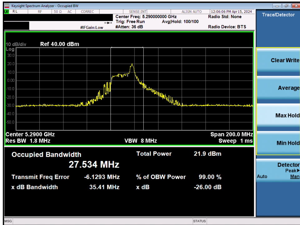
Plot 7-9. 26dB Bandwidth Plot MIMO ANT1 (80MHz BW 802.11be – 26 Tones (UNII Band 2A) – Ch. 58)
