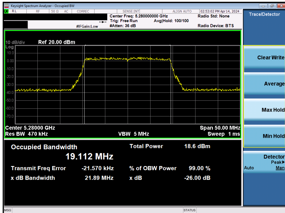
Plot 7-40. 26dB Bandwidth Plot MIMO ANT2 (20MHz BW 802.11be – 242 Tones (UNII Band 2A) – Ch. 56)
