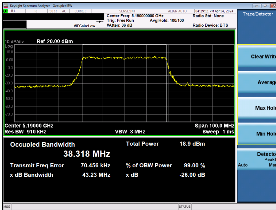
Plot 7-37. 26dB Bandwidth Plot MIMO ANT2 (40MHz BW 802.11be – 484 Tones (UNII Band 1) – Ch. 38)
