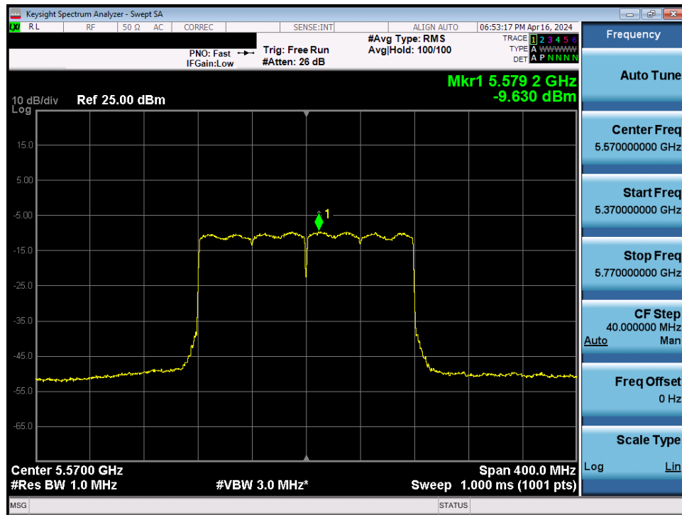
Plot 7-103. Power Spectral Density Plot MIMO ANT1 (160MHz BW 802.11be – 2x996 Tones (UNII Band 2C) – Ch. 114)
