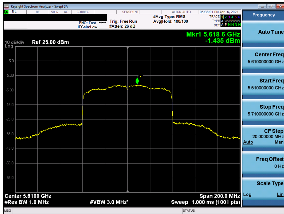
Plot 7-102. Power Spectral Density Plot MIMO ANT1 (80MHz BW 802.11be – 996 Tones (UNII Band 2C) – Ch. 122)
