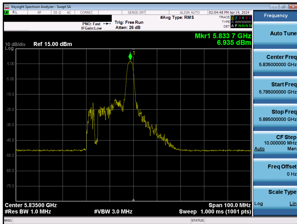
Plot 7-144. Power Spectral Density Plot MIMO ANT2 (40MHz BW 802.11be – 26 Tones (UNII Band 3/4) – Ch. 167)
