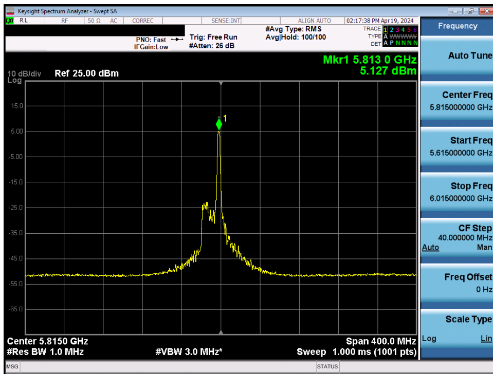
Plot 7-146. Power Spectral Density Plot MIMO ANT2 (160MHz BW 802.11be – 26 Tones (UNII Band 3/4) – Ch. 163)
