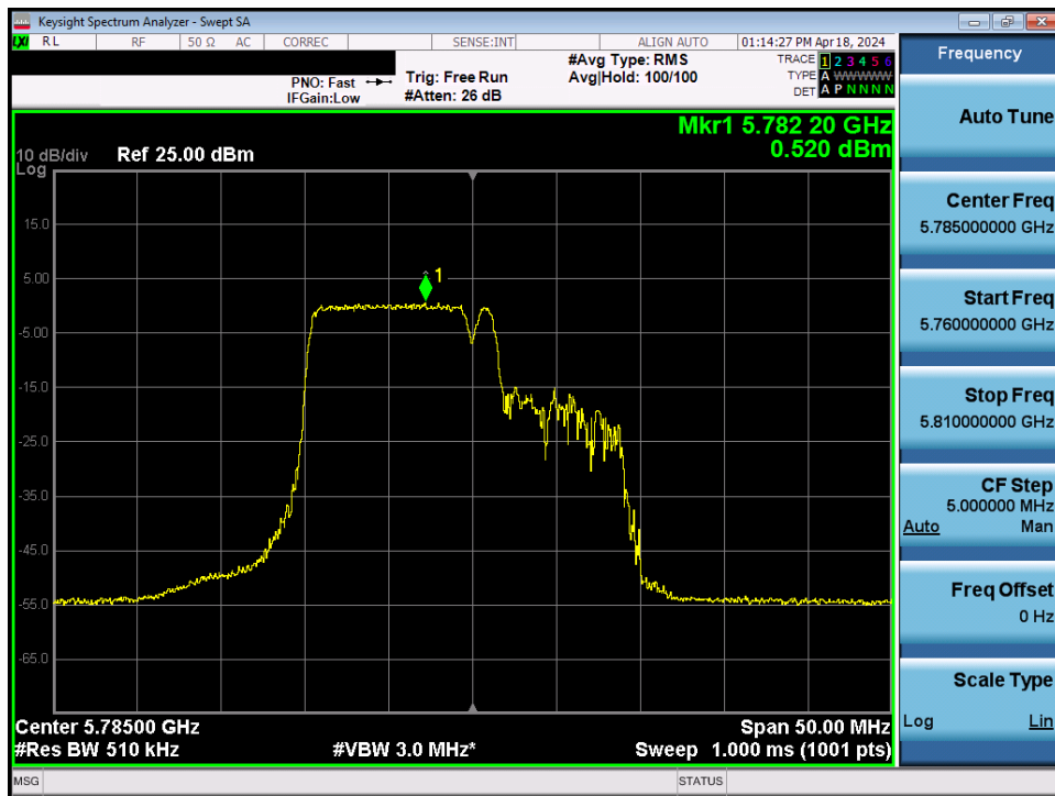
Plot 7-177. Power Spectral Density Plot MIMO ANT2 (20MHz BW 802.11be – 106+26 Tones (UNII Band 3) – Ch. 157)
