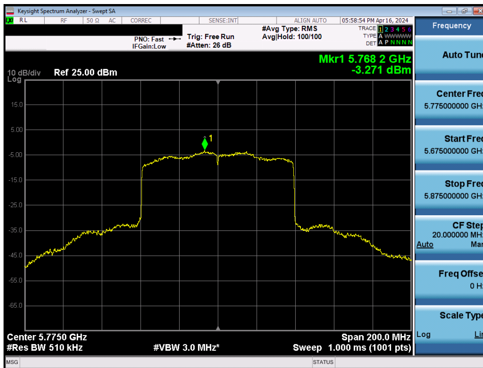
Plot 7-106. Power Spectral Density Plot MIMO ANT1 (80MHz BW 802.11be – 996 Tones (UNII Band 3) – Ch. 155)
