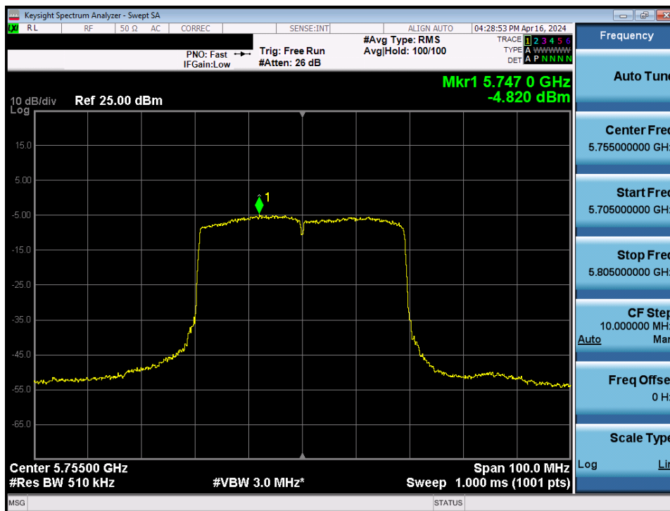
Plot 7-105. Power Spectral Density Plot MIMO ANT1 (40MHz BW 802.11be – 484 Tones (UNII Band 3) – Ch. 151)
