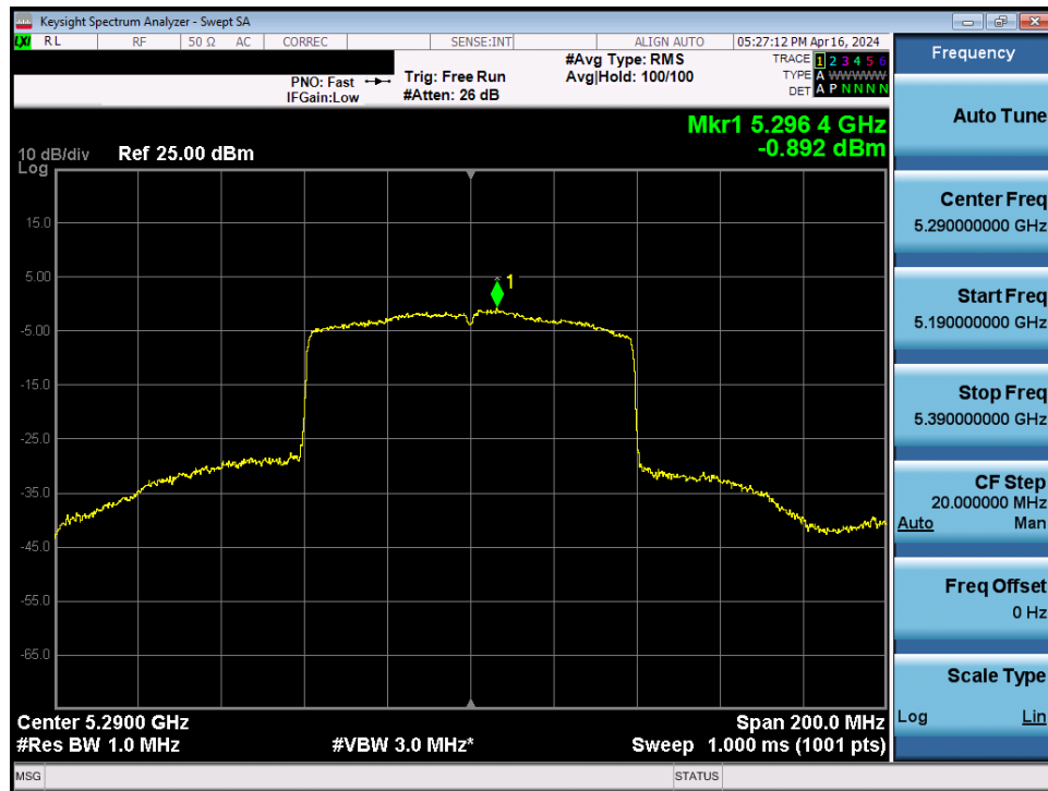
Plot 7-99. Power Spectral Density Plot MIMO ANT1 (80MHz BW 802.11be – 996 Tones (UNII Band 2A) – Ch. 58)
