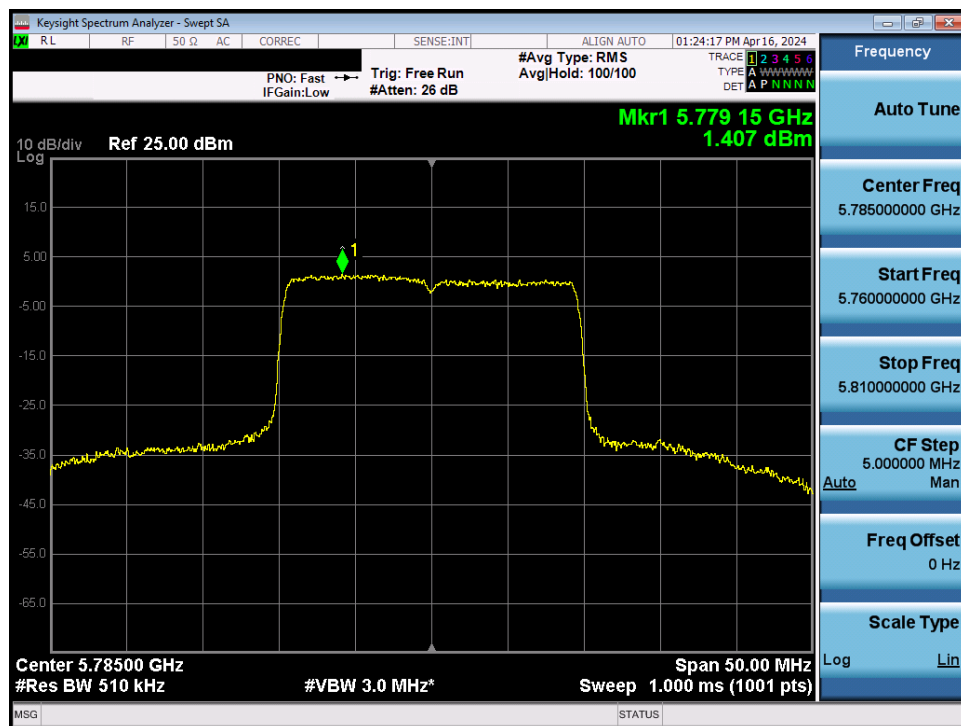
Plot 7-104. Power Spectral Density Plot MIMO ANT1 (20MHz BW 802.11be – 242 Tones (UNII Band 3) – Ch. 157)
