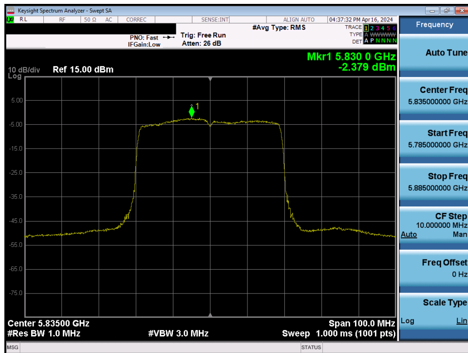
Plot 7-108. Power Spectral Density Plot MIMO ANT1 (40MHz BW 802.11be – 484 Tones (UNII Band 3/4) – Ch. 167)
