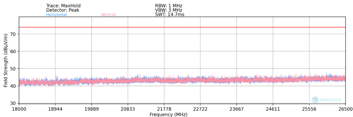
Plot 7-188. Radiated Spurious Plot 18GHz - 26.5GHz (802.11be)
