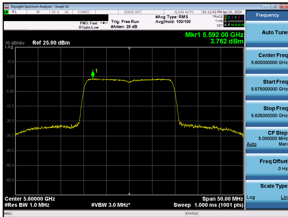
Plot 7-100. Power Spectral Density Plot MIMO ANT1 (20MHz BW 802.11be – 242 Tones (UNII Band 2C) – Ch. 120)
