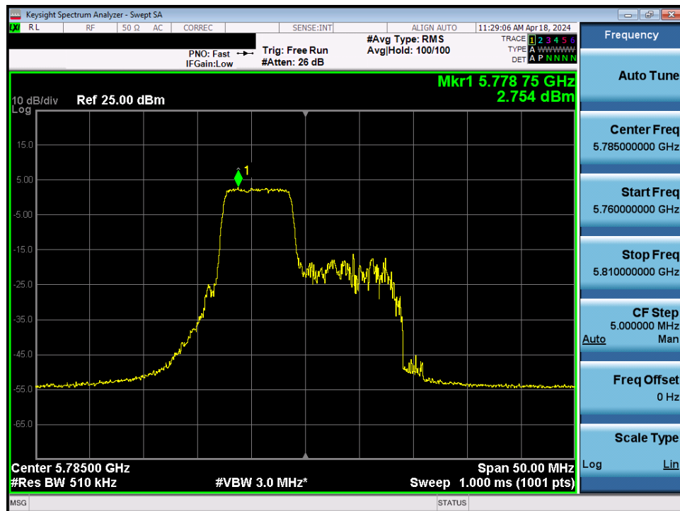
Plot 7-176. Power Spectral Density Plot MIMO ANT2 (20MHz BW 802.11be – 52+26 Tones (UNII Band 3) – Ch. 157)
