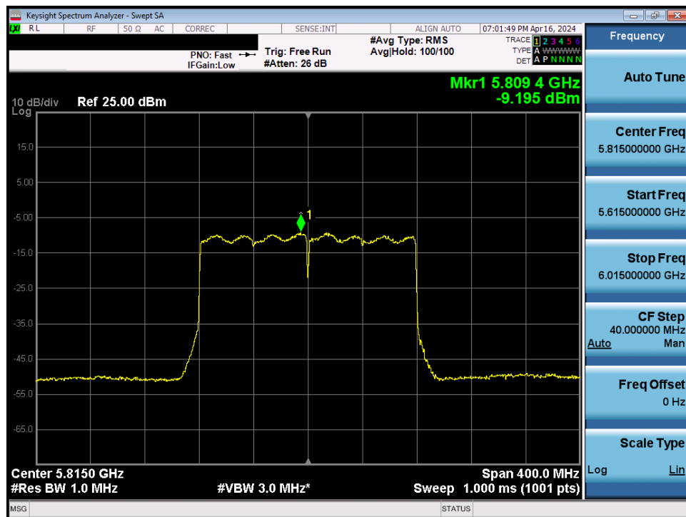
Plot 7-110. Power Spectral Density Plot MIMO ANT1 (160MHz BW 802.11be – 996*2 Tones (UNII Band 3/4) – Ch. 163)
