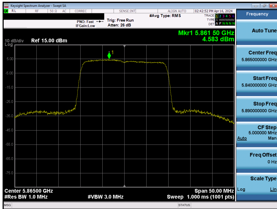
Plot 7-107. Power Spectral Density Plot MIMO ANT1 (20MHz BW 802.11be – 242 Tones (UNII Band 4) – Ch. 173)
