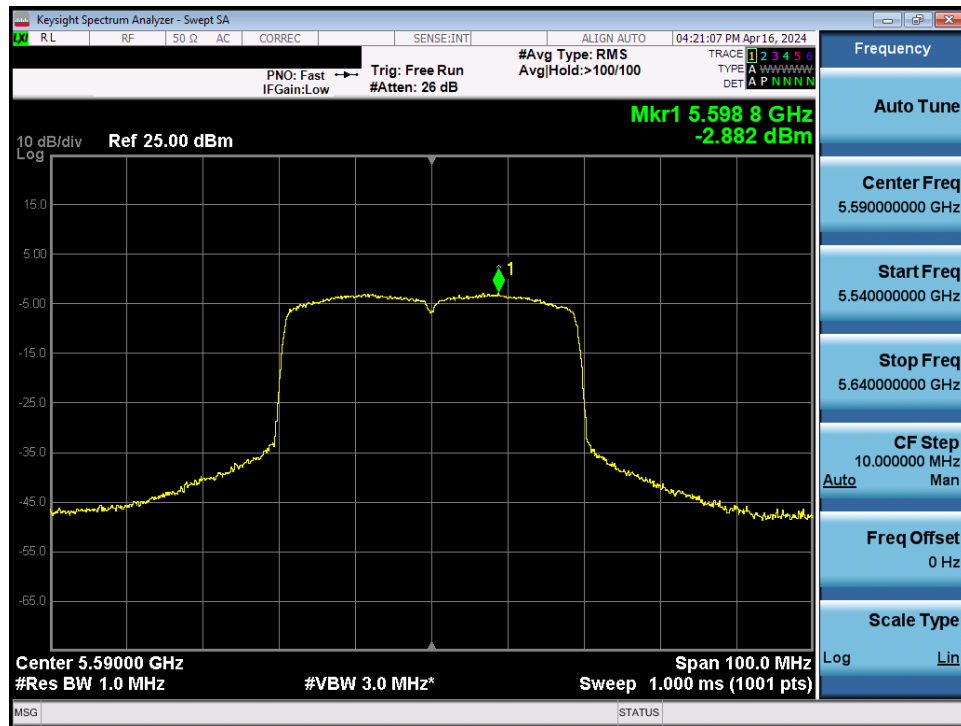
Plot 7-101. Power Spectral Density Plot MIMO ANT1 (40MHz BW 802.11be – 484 Tones (UNII Band 2C) – Ch. 118)
