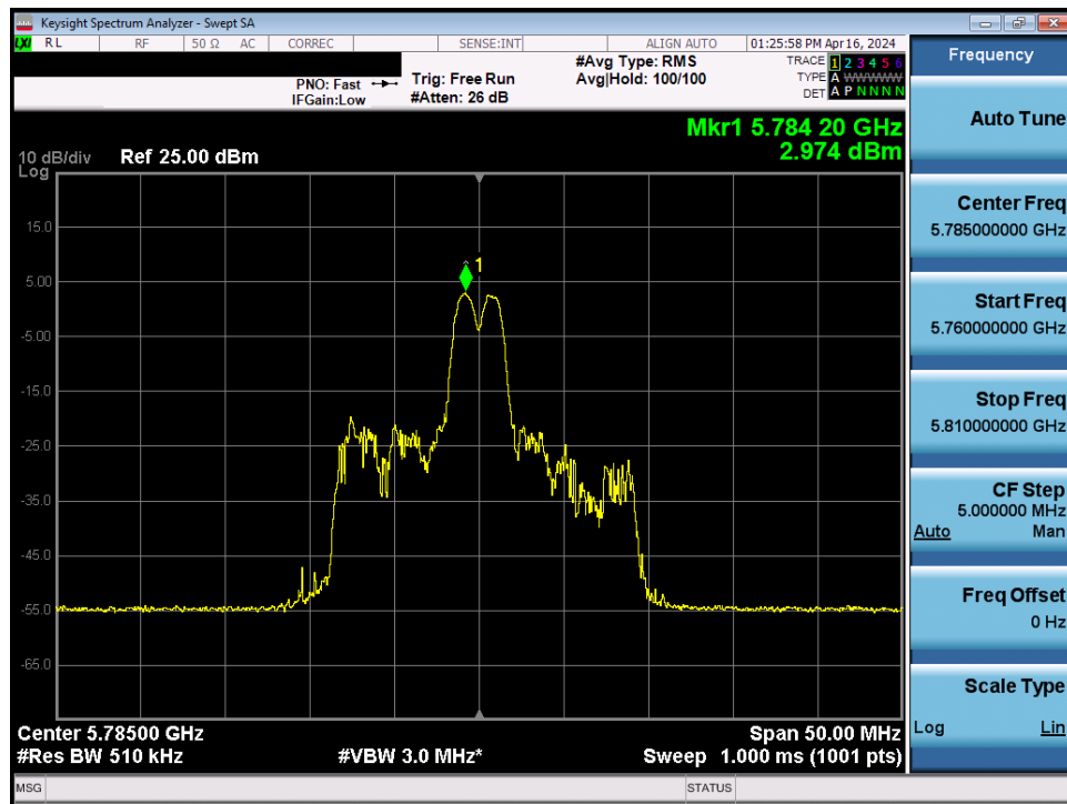
Plot 7-140. Power Spectral Density Plot MIMO ANT2 (20MHz BW 802.11be – 26 Tones (UNII Band 3) – Ch. 157)
