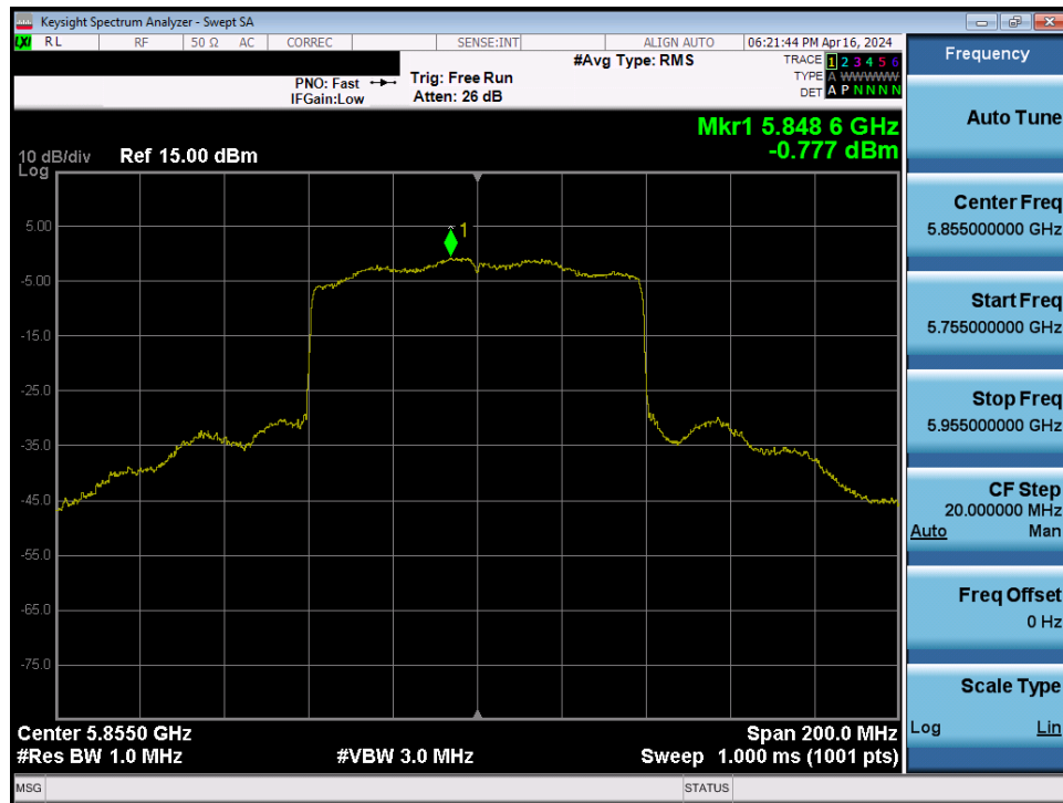
Plot 7-109. Power Spectral Density Plot MIMO ANT1 (80MHz BW 802.11be – 996 Tones (UNII Band 3/4) – Ch. 171)
