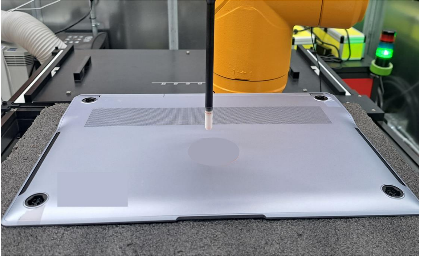
Near Field Power Density Test Setup Photo 3 – Bottom Edge at 10.02mm
