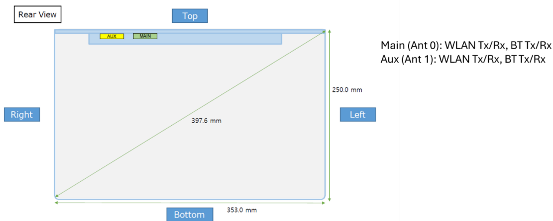
Figure H-1 DUT Antenna Locations
