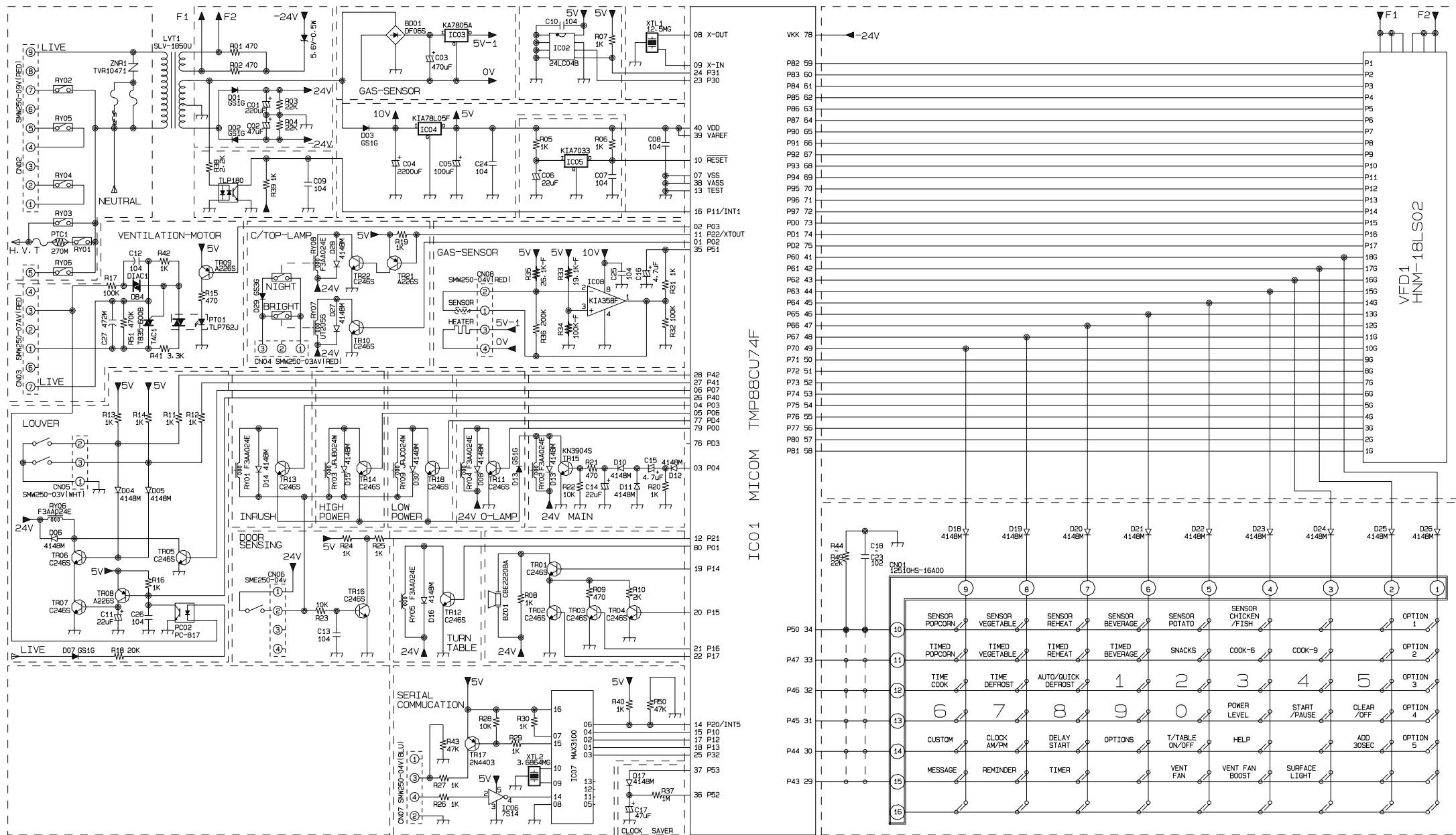
DIGRAM ELECTRIC OTR-9(1.8Cu.ft)
