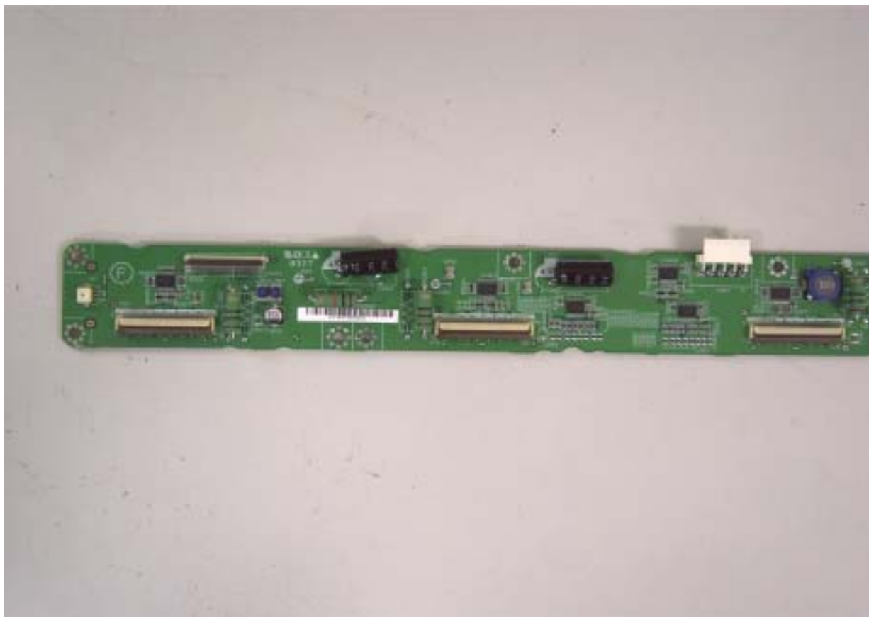
F buffer board top view
