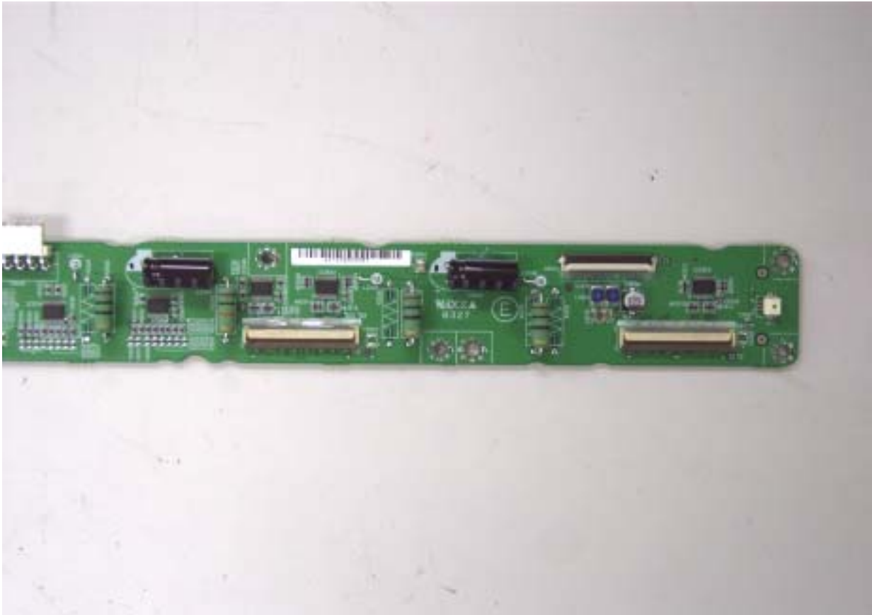
E buffer-1 board top view
