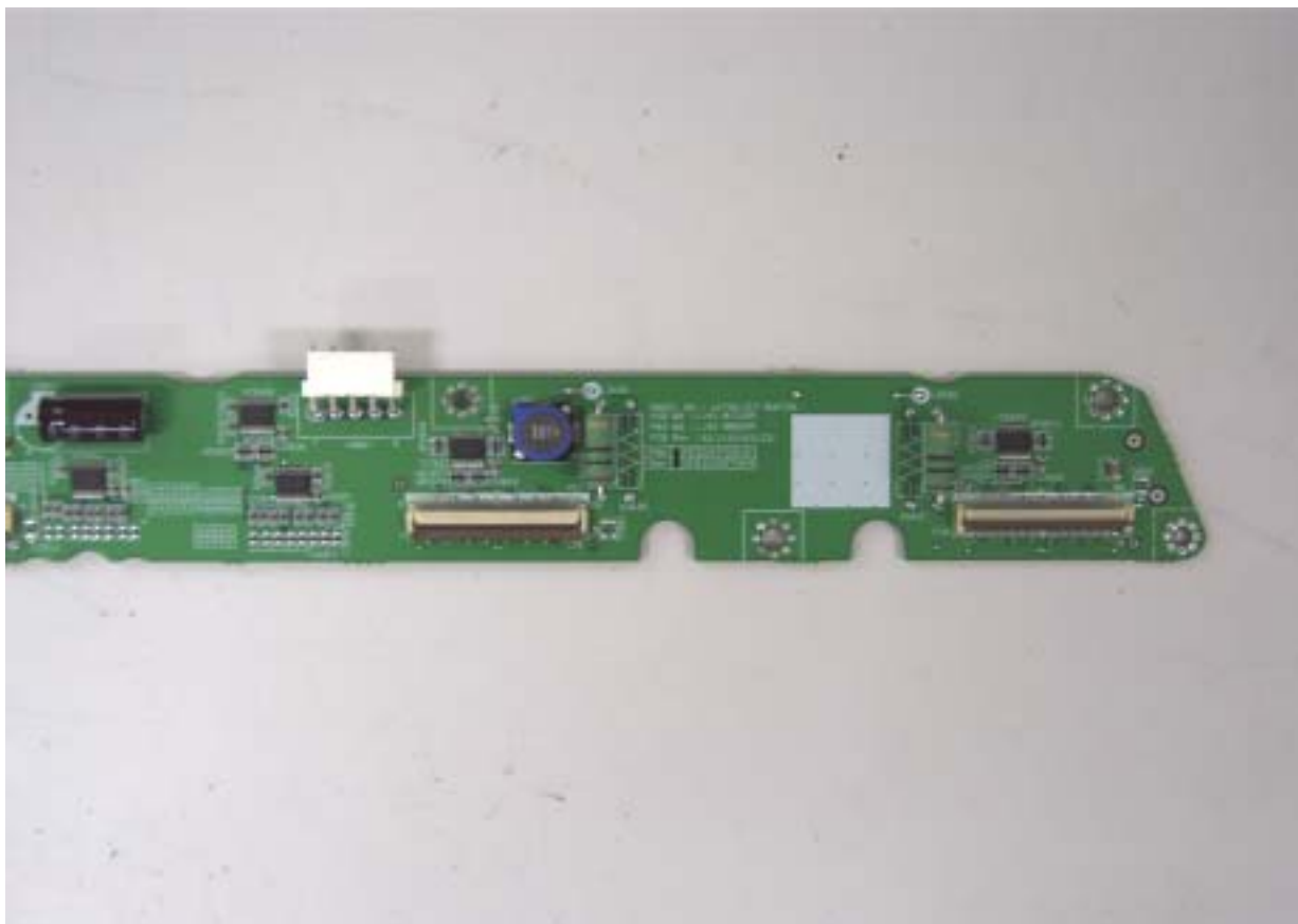
F buffer board top view
