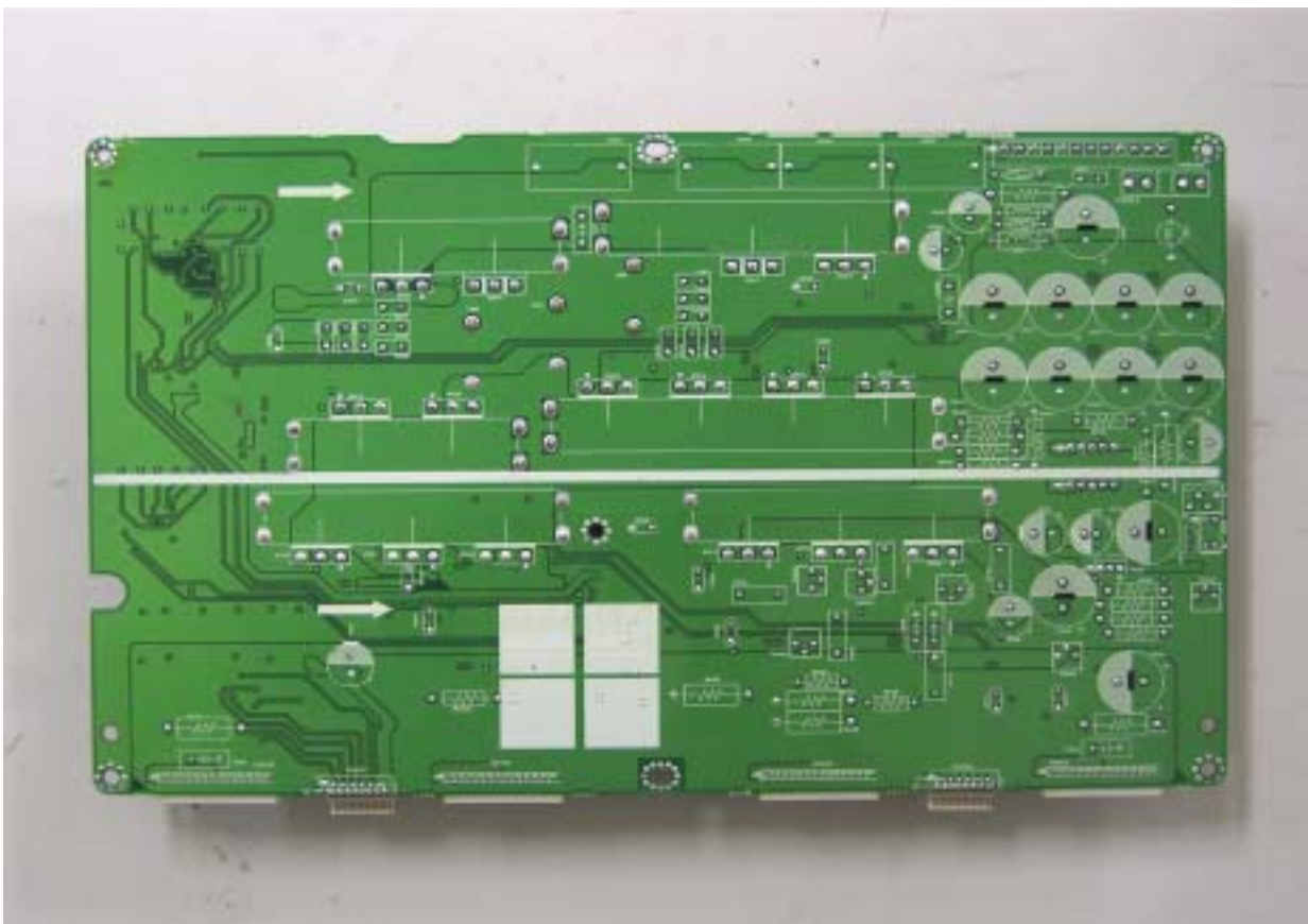
Y driver board bottom view
