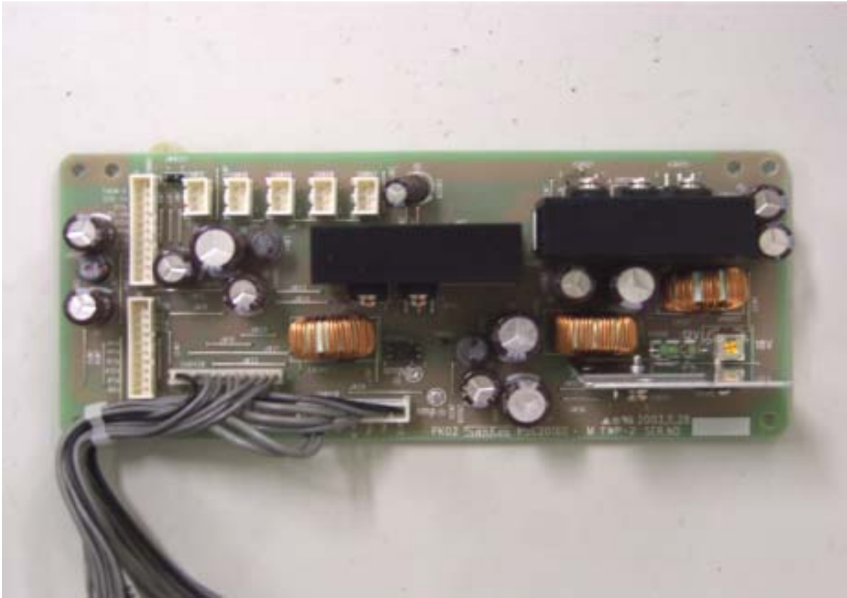
SMPS sub board top view
