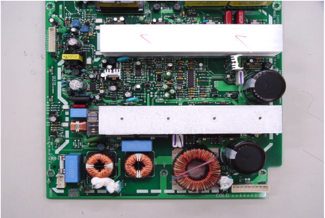
SMPS board-1 top view
