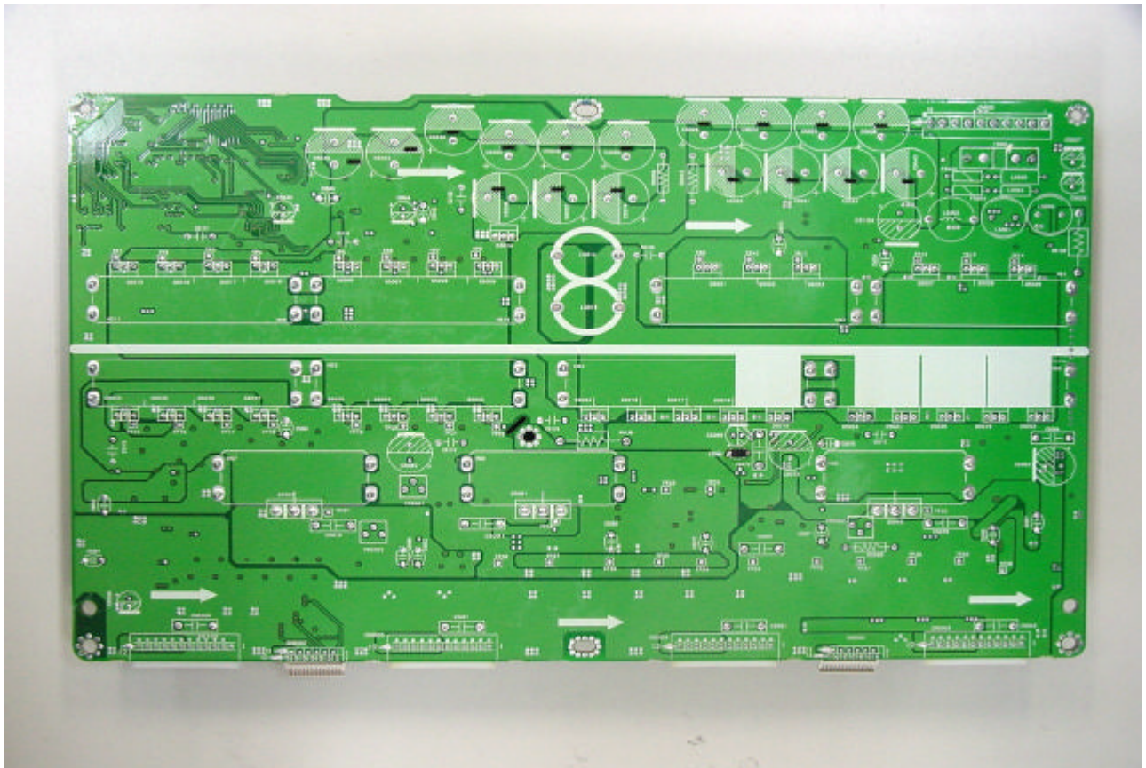
Y-driver board bottom view
