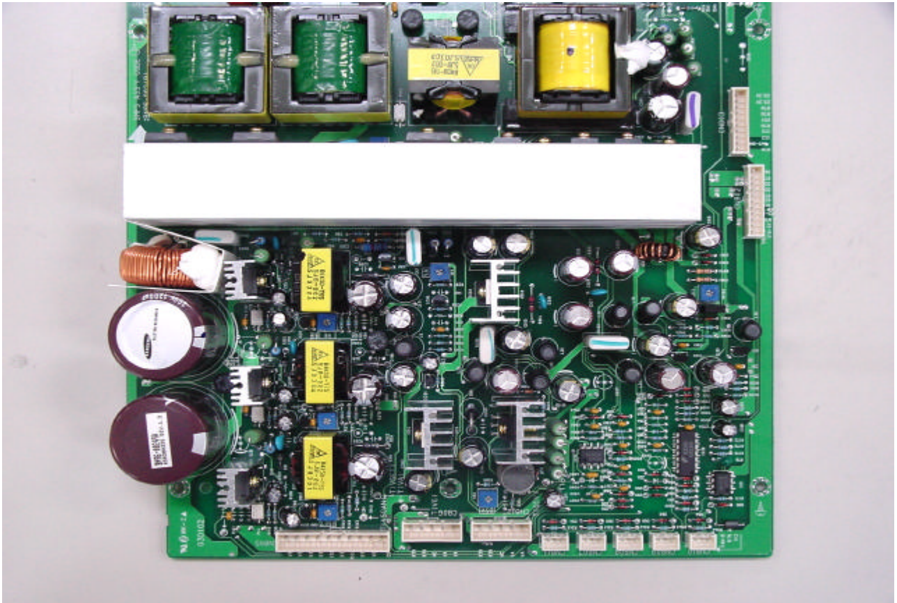
SMPS board top view
