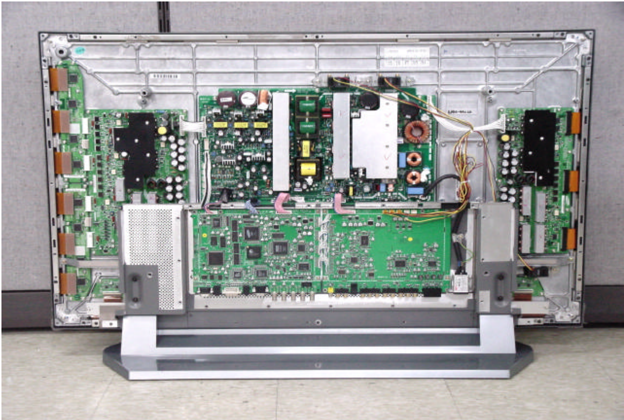
EUT interior view
