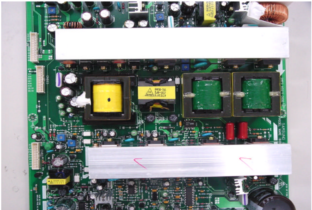
SMPS board-2 top view
