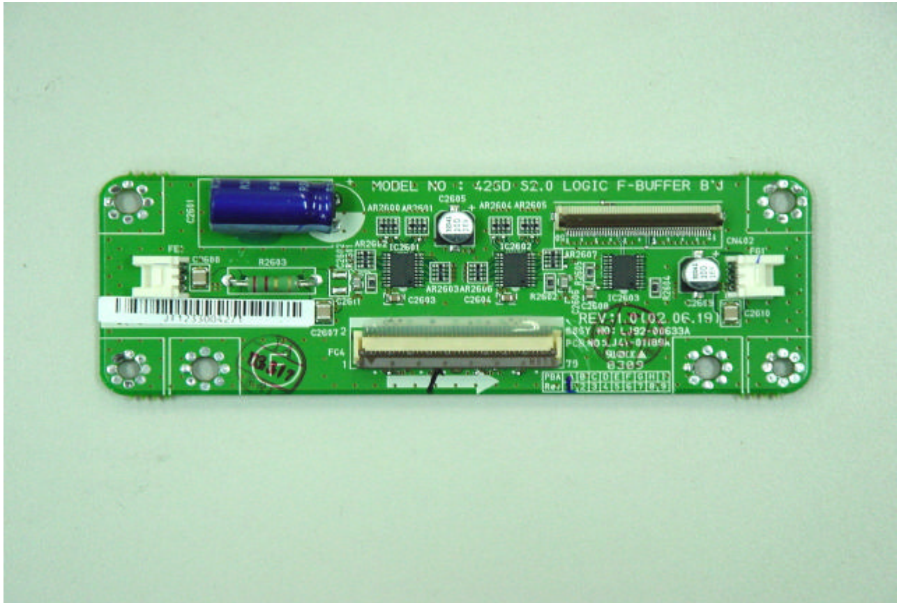
Logic-F-buffer board top view
