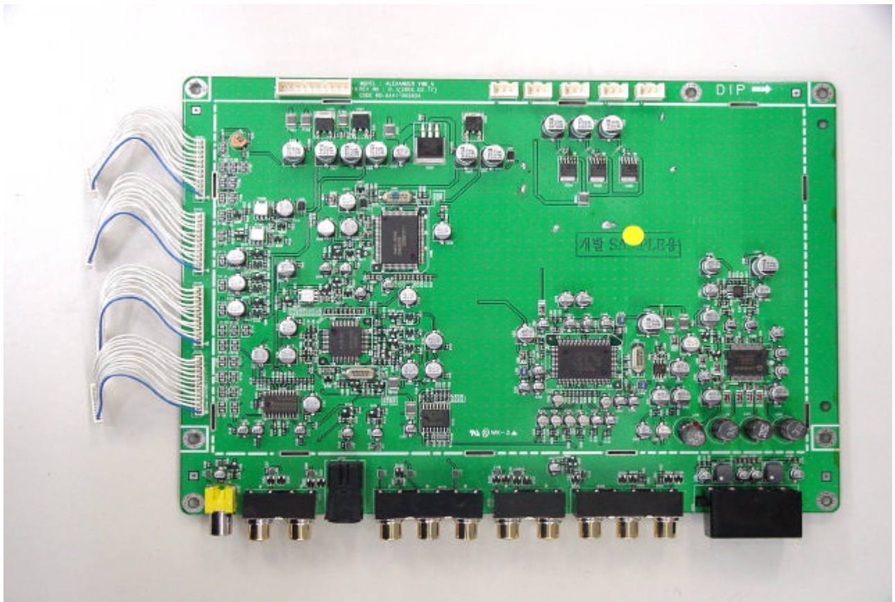
Analog visual board top view
