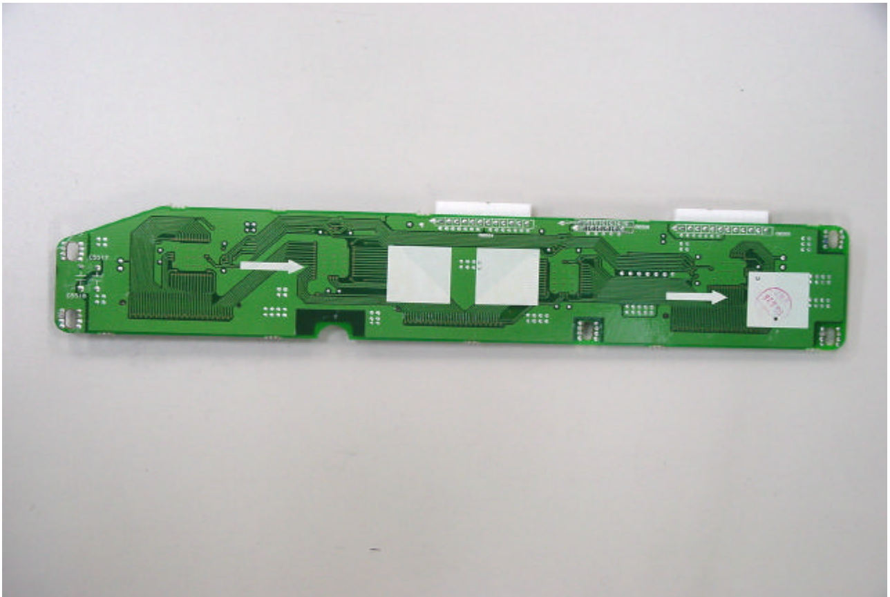
YB-lower board bottom view
