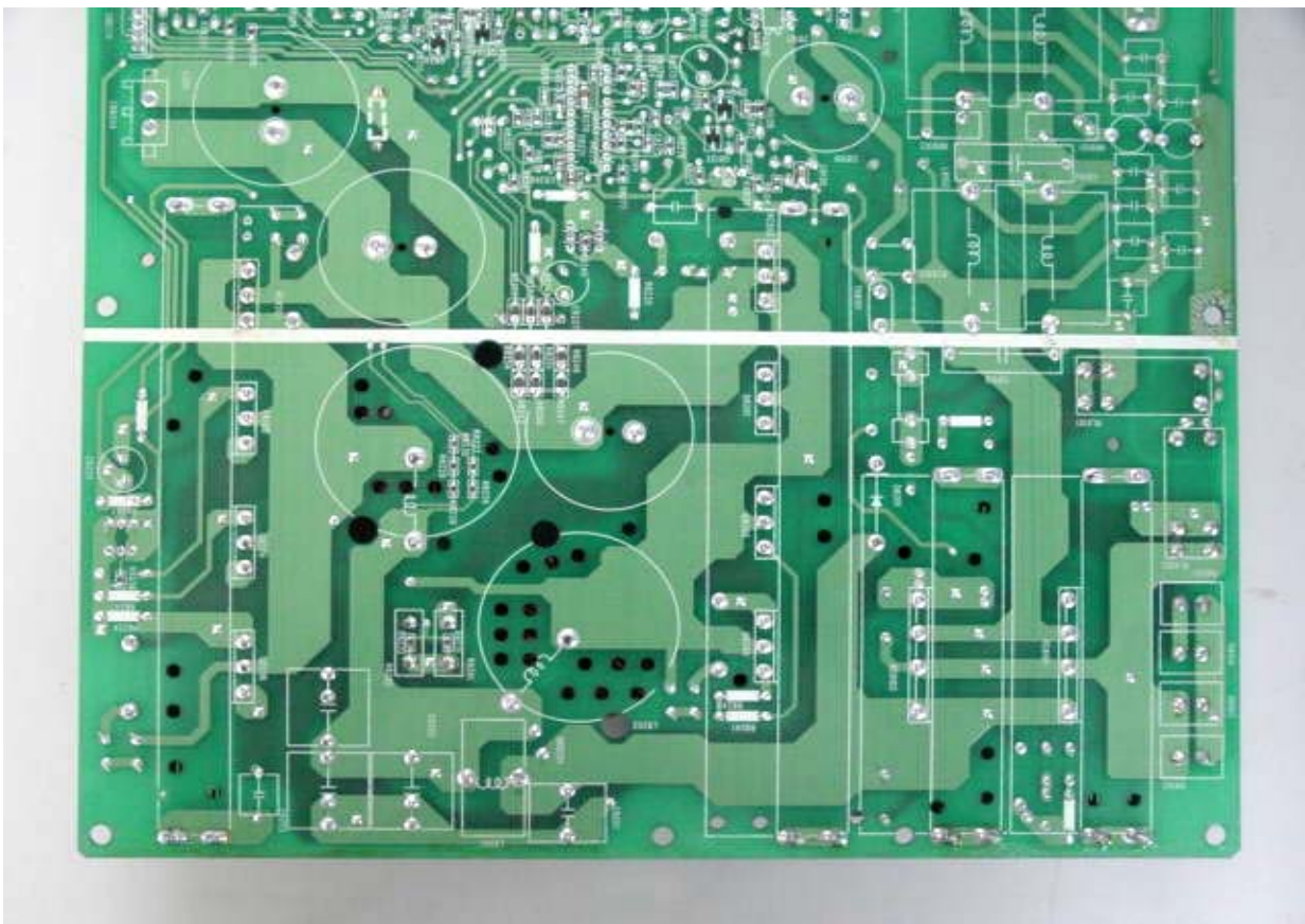
Line-filter-2 board bottom view
