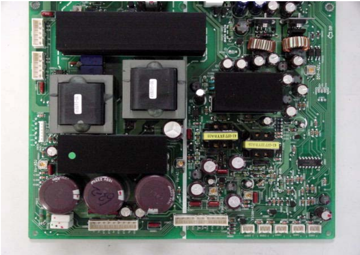
SMPS-1 board top view
