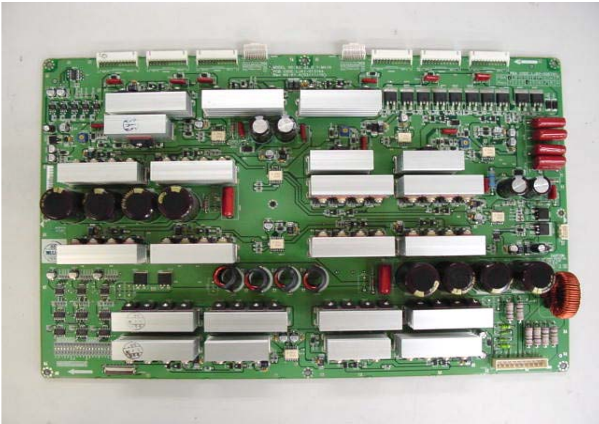
Y-driver board top view
