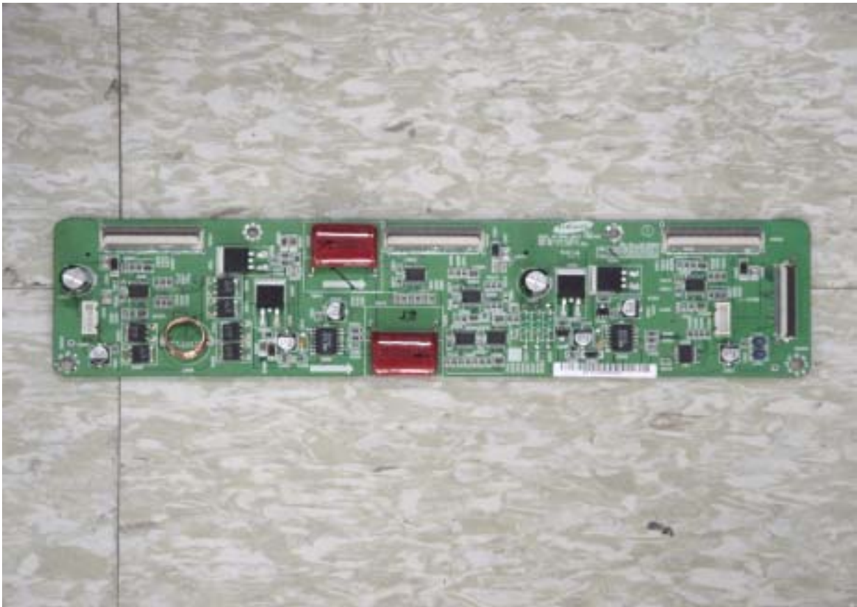
Logic-I buffer board top view
