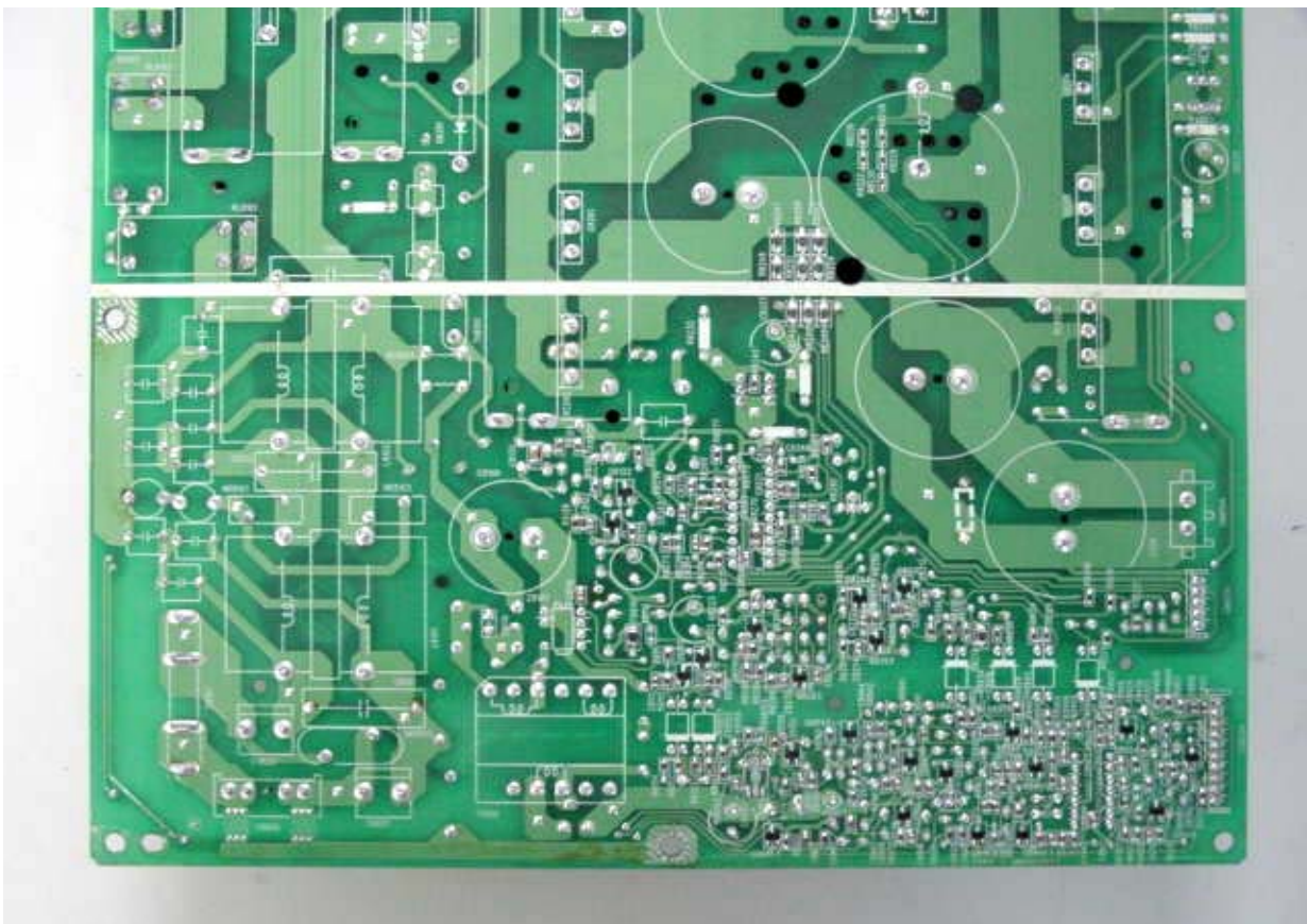
Line-filter-1 board bottom view
