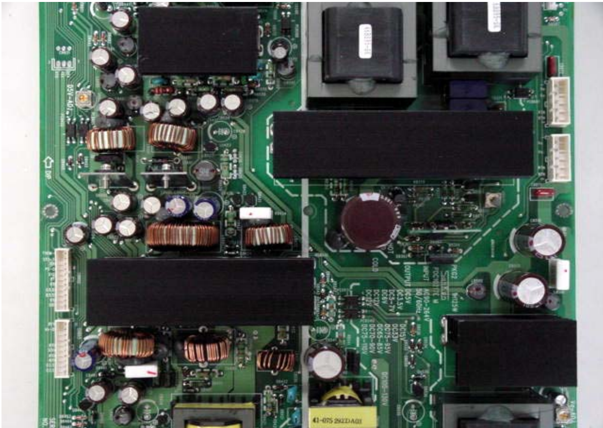
SMPS-3 board top view
