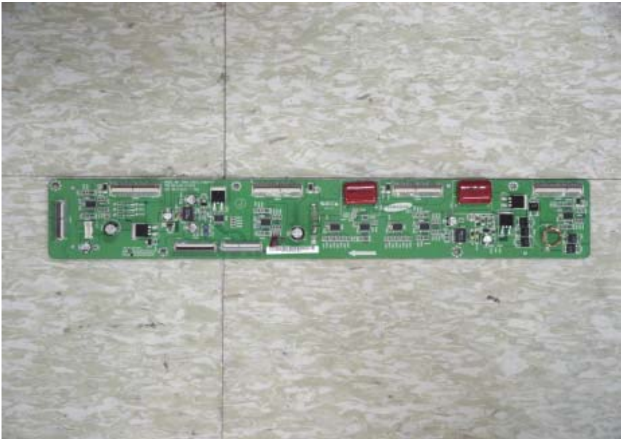
Logic-J buffer board top view
