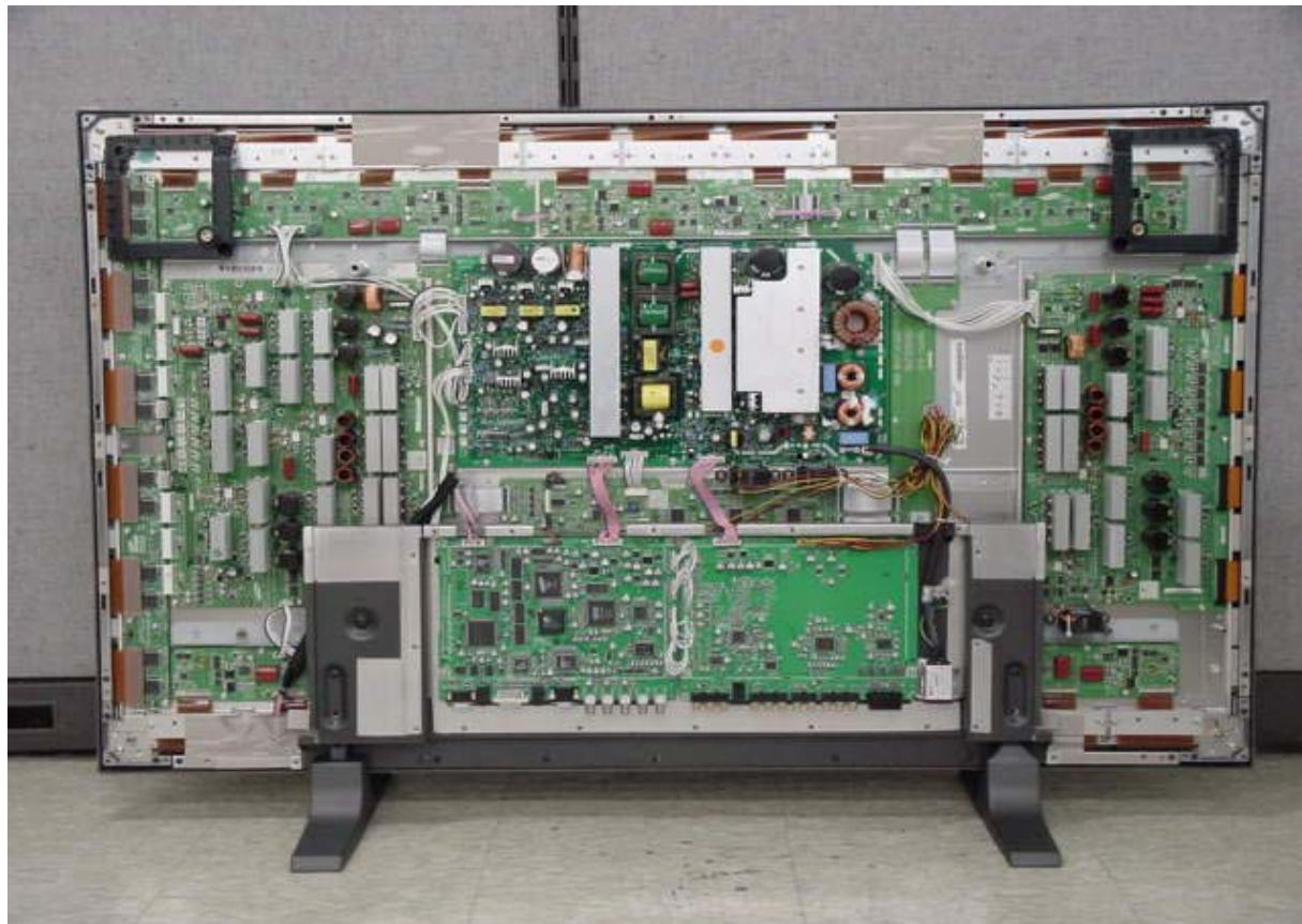
EUT interior view
