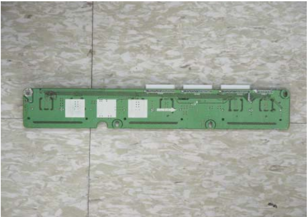
Address buffer lower bottom view
