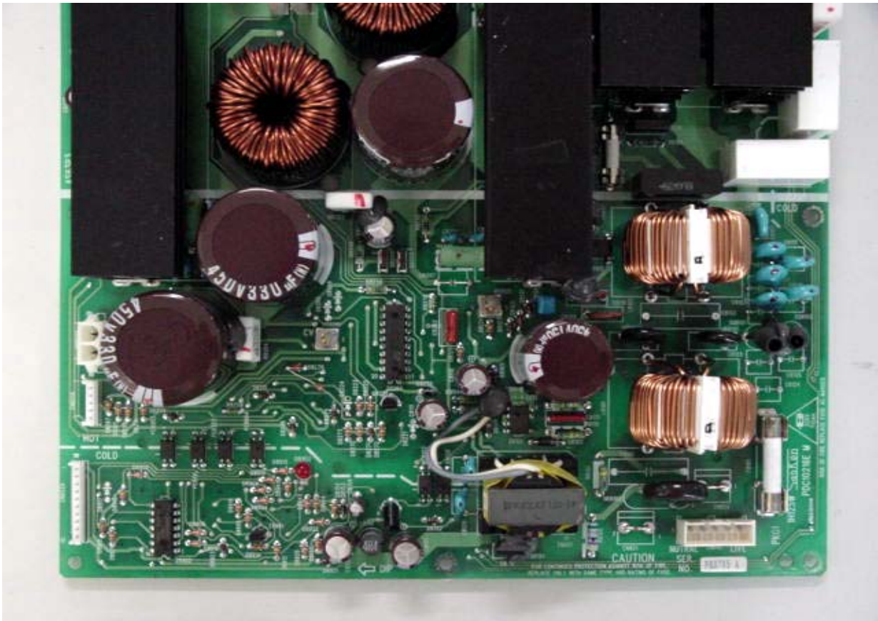
Line-filter-1 board top view
