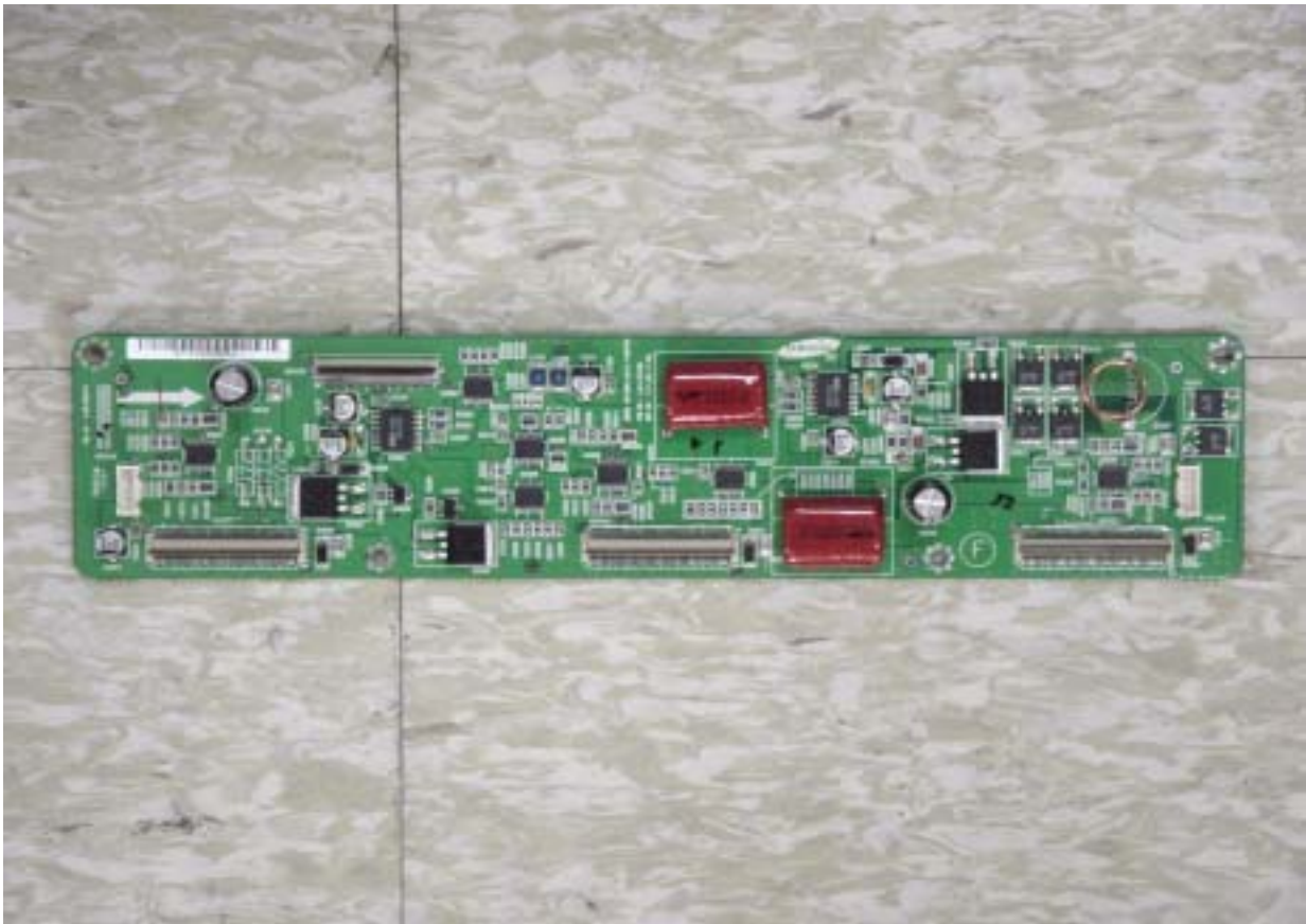
Logic-F buffer board top view
