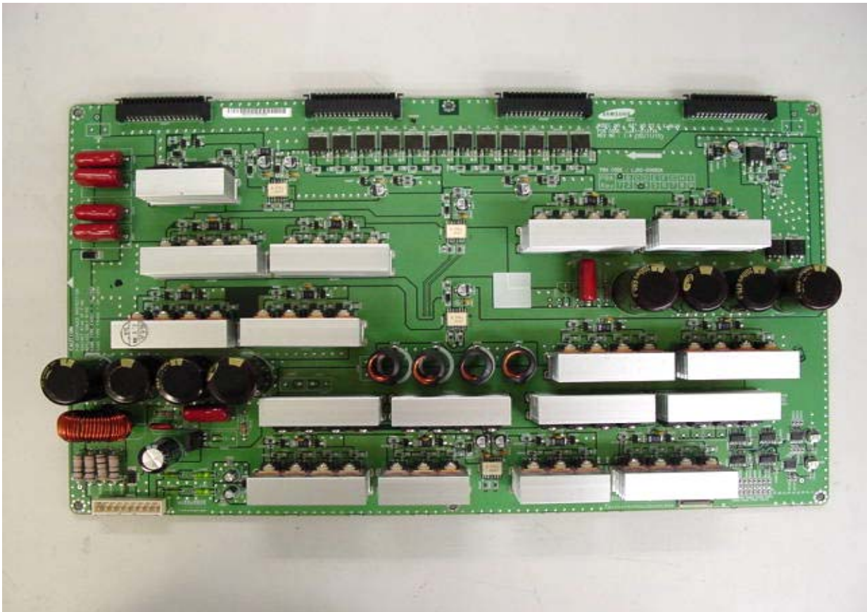
X-driver board top view
