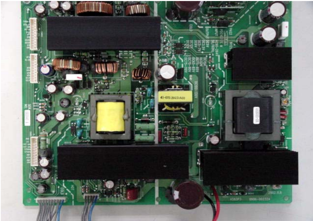
SMPS-2 board top view
