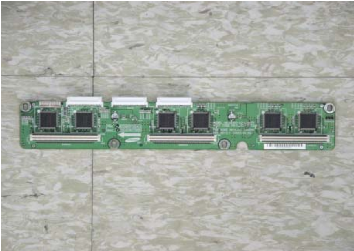
Address buffer lower top view
