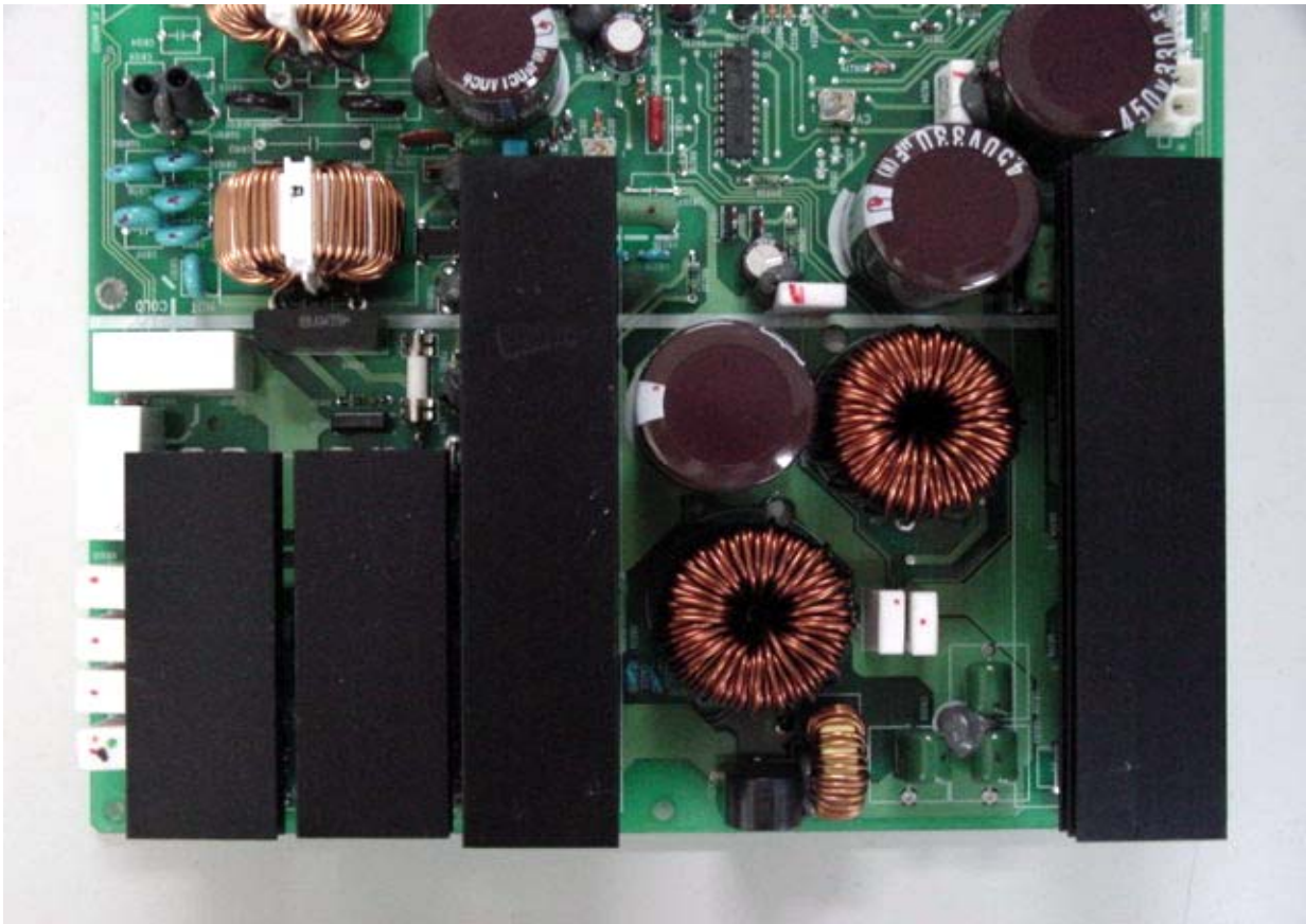
Line-filter-2 board top view
