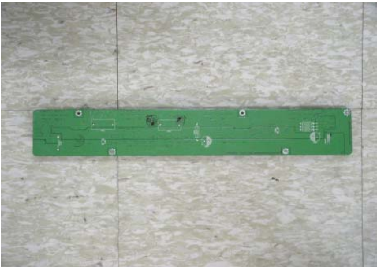
Logic-J buffer board bottom view
