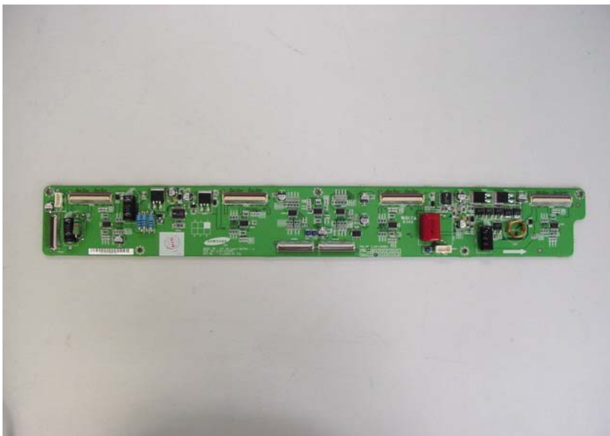
Logic buffer-J board top view
