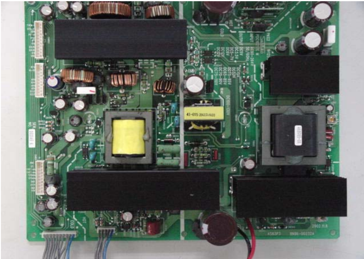
SMPS-2 board top view
