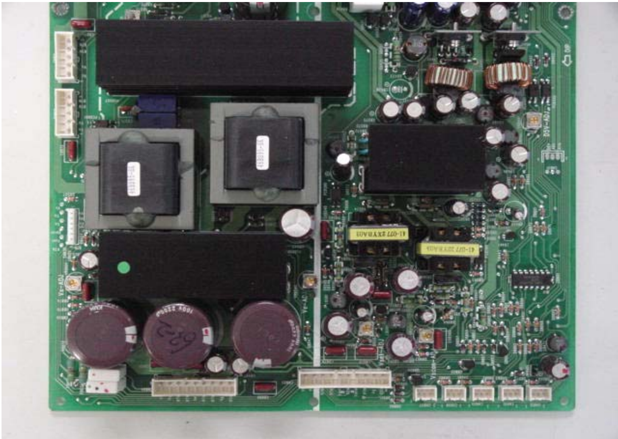
SMPS-1 board top view
