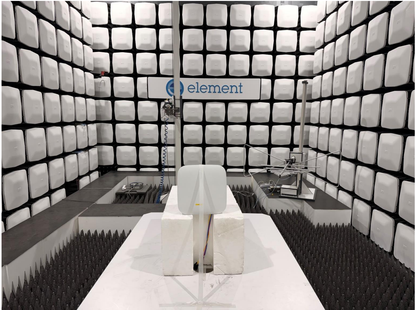
Above 1GHz radiated Test Instrument & Measurement Setup _DC Power
