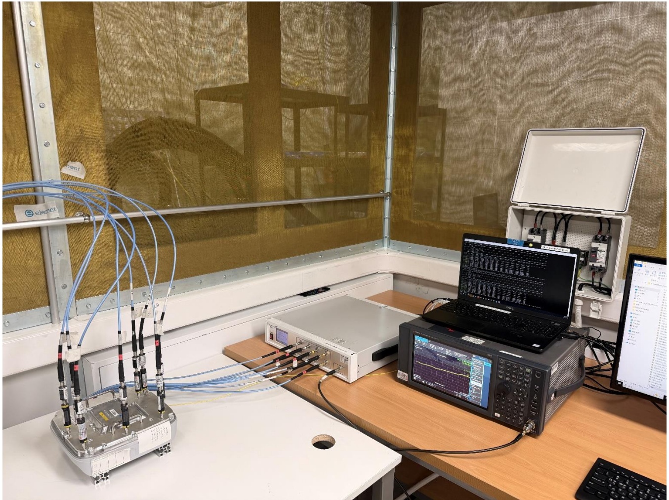
Conducted Test Instrument & Measurement Setup
