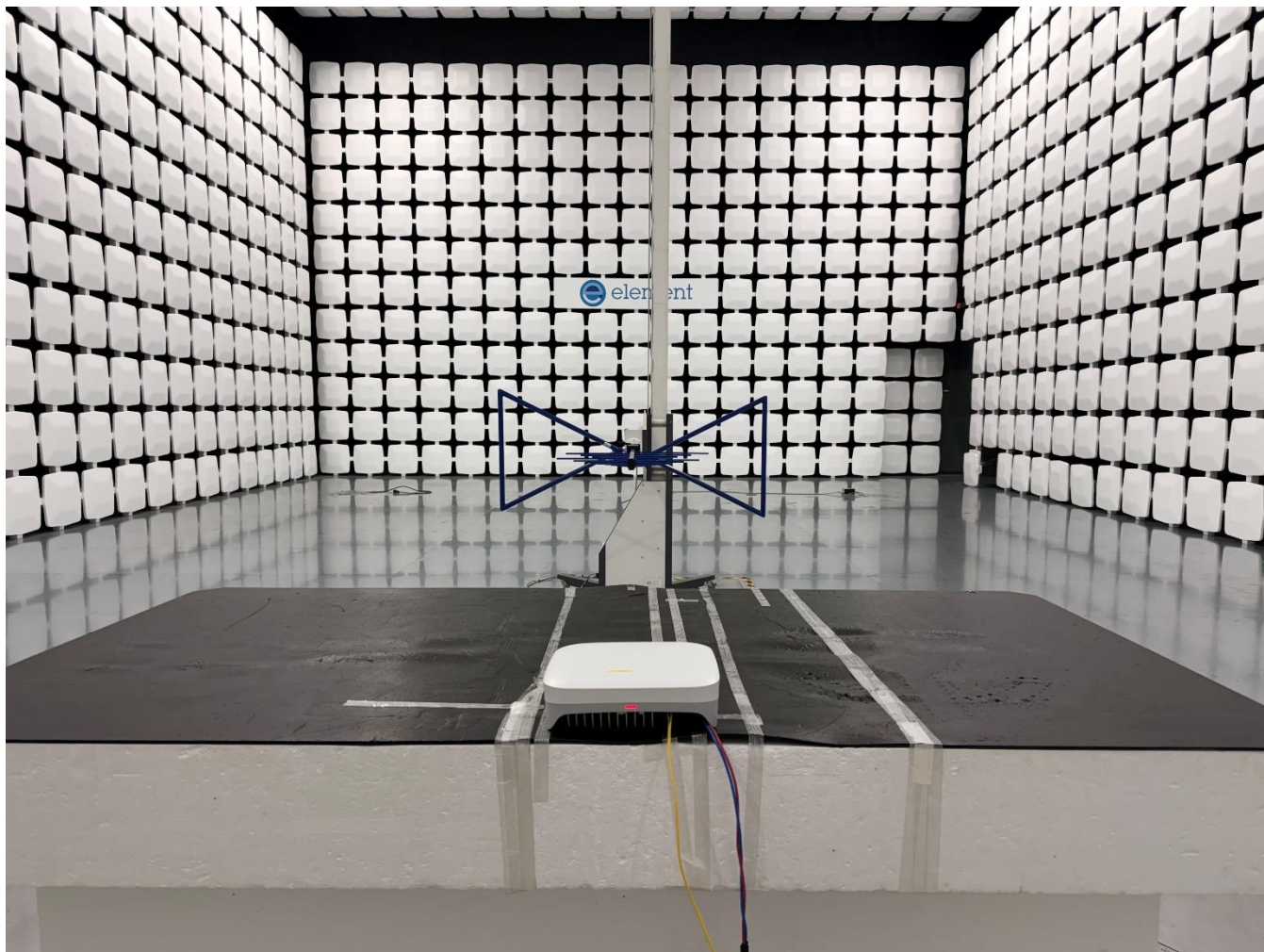
Below 1GHz radiated Test Instrument & Measurement Setup_DC Power
