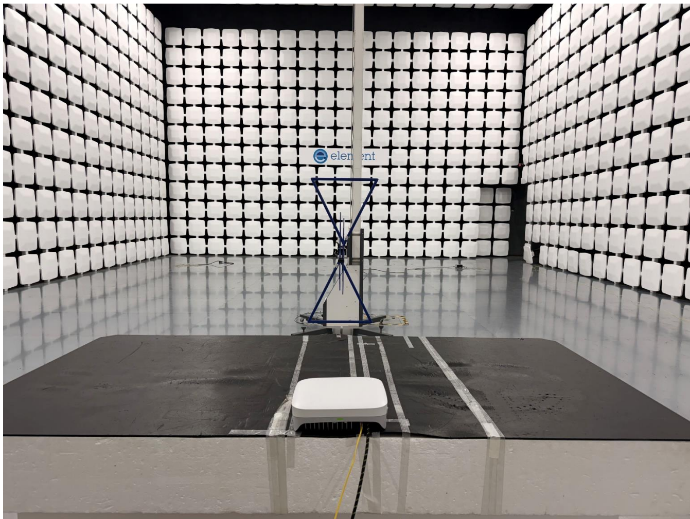
Below 1GHz radiated Test Instrument & Measurement Setup_PoE Power
