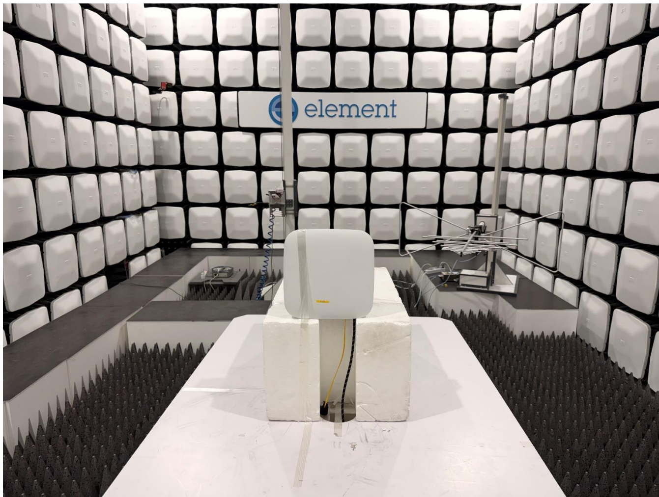
Above 1GHz radiated Test Instrument & Measurement Setup _PoE Power
