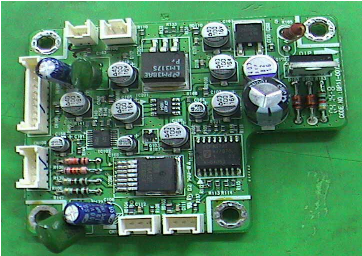
Sub detect board top view
