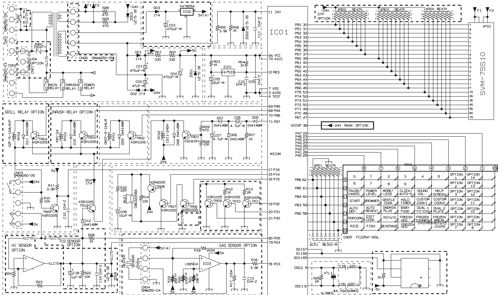
W3USA SCHEMATIC
