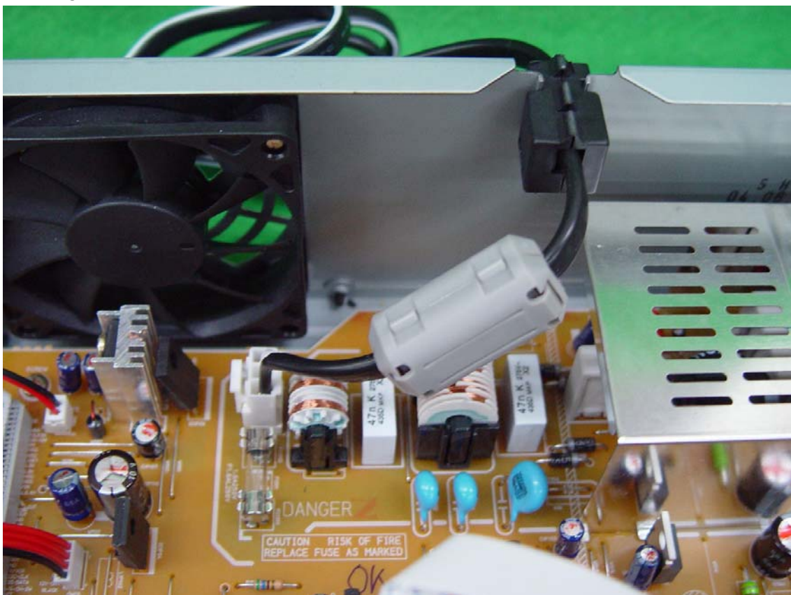
Shielding 4
