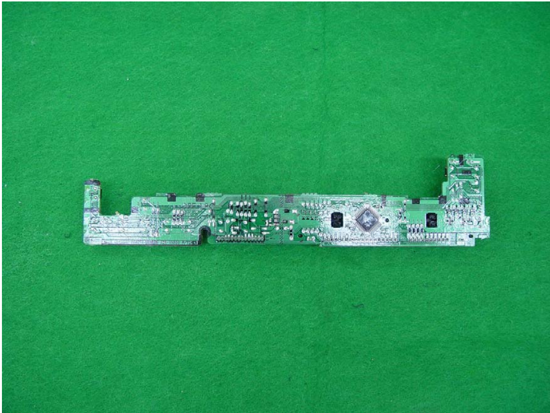
Bottom of Front PCB View
