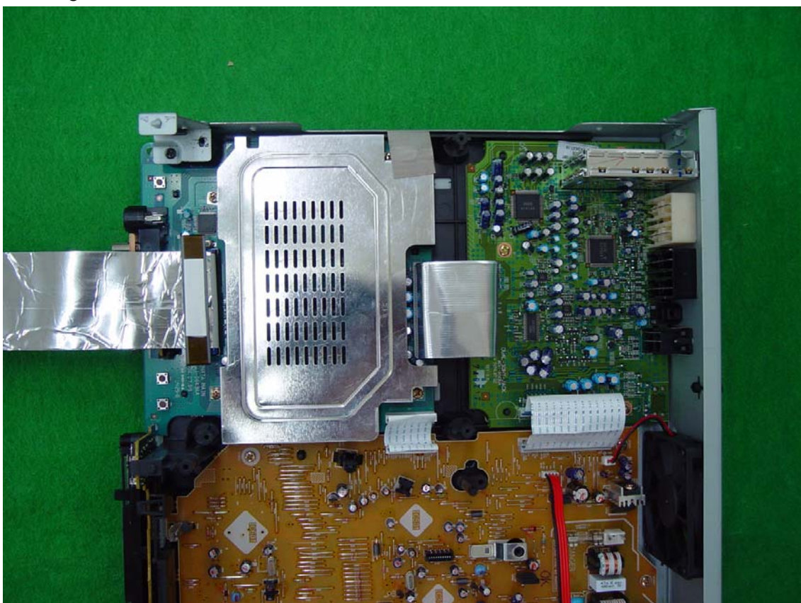
Shielding 2
