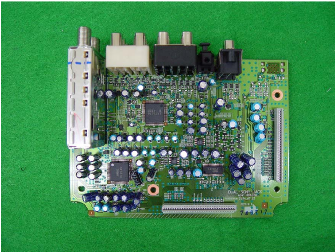
Top of DVD PCB 1 View
