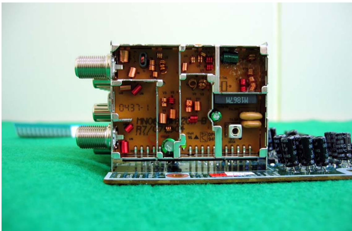
TM Block View (Top & Cover Open)
