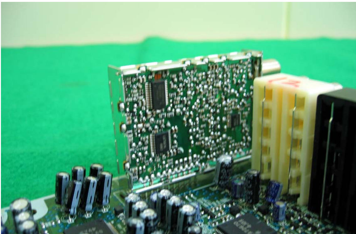
TM Block View (Bottom & Cover Open)
