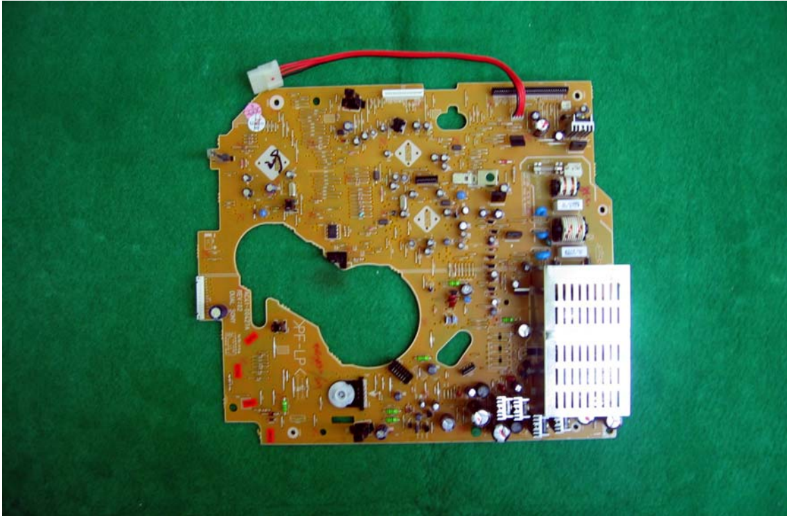
Main PCB View (Top)
