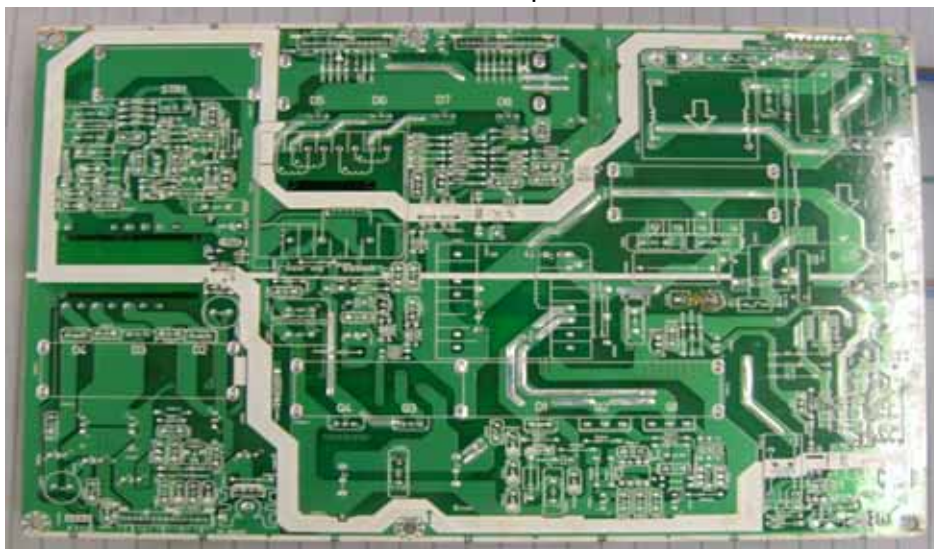
SMPS board top view
