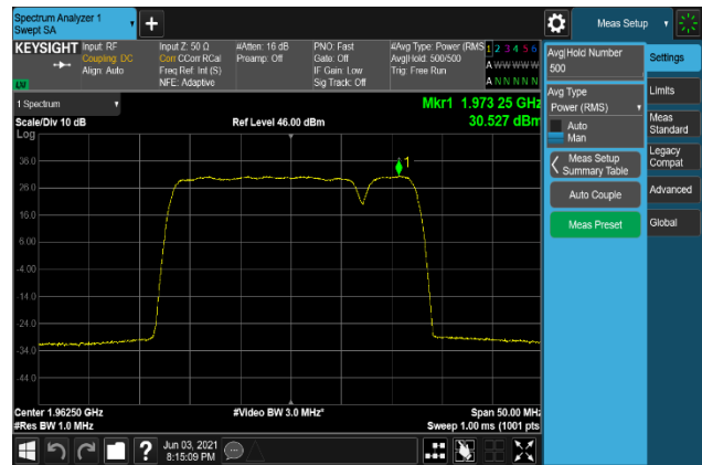
Plot 7-366. Peak To Average Power Ratio Plot (B2_20M+5M_16QAM - Middle Channel, Port 0)
