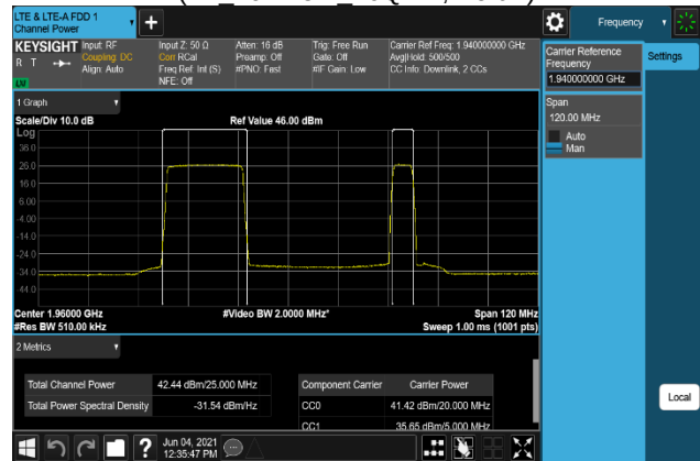
Plot 7-332. Conducted Average Output Power Plot (B2_20M+5M_256QAM, Port 2)
