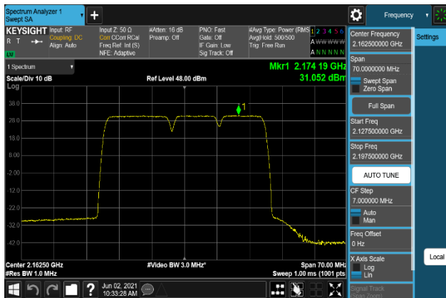
Plot 7-345. Peak To Average Power Radio Plot (B66_15M+10M+10M_QPSK - High Channel, Port 0)
