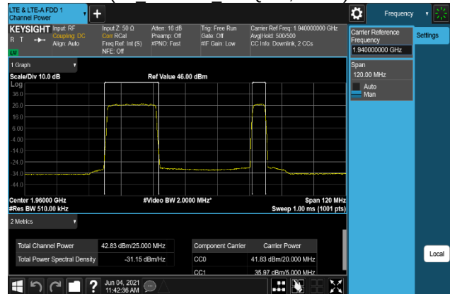
Plot 7-326. Conducted Average Output Power Plot (B2_20M+5M_16QAM, Port 1)
