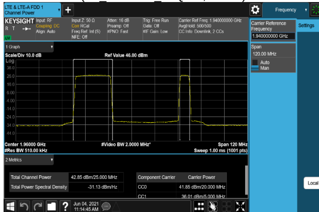
Plot 7-325. Conducted Average Output Power Plot (B2_20M+5M_QPSK, Port 1)
