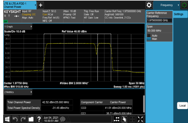
Plot 7-316. Conducted Average Output Power Plot (B2_20M+5M_256QAM - High Channel, Port 2)
