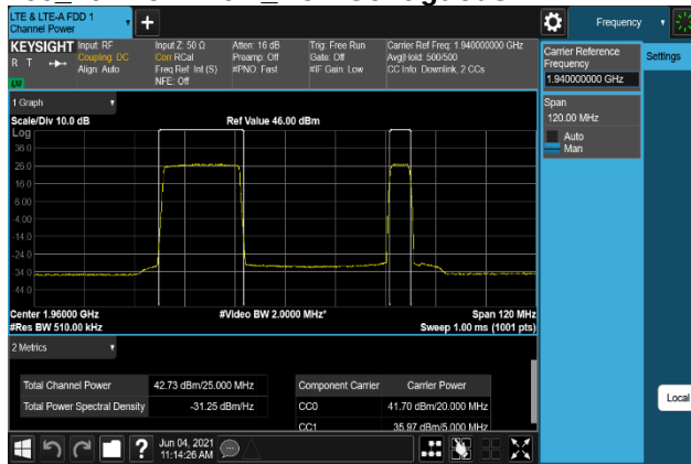
Plot 7-321. Conducted Average Output Power Plot (B2 20M+5M QPSK, Port 0)
