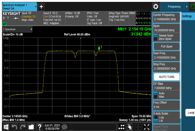
Plot 7-341. Peak To Average Power Ratio Plot (B66_15M+10M+10M_QPSK - Middle Channel, Port 0)
