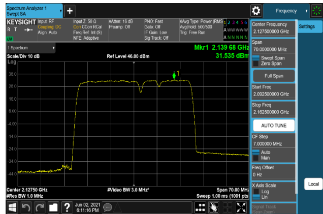
Plot 7-350. Peak To Average Power Ratio Plot (B66_20M+5M+10M_16QAM - Low Channel, Port 1)
