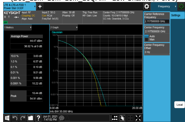
Plot 7-376. Peak To Average Power Ratio Plot (B66_15M+10M+10M_256QAM - Low Channel, Port 0)
