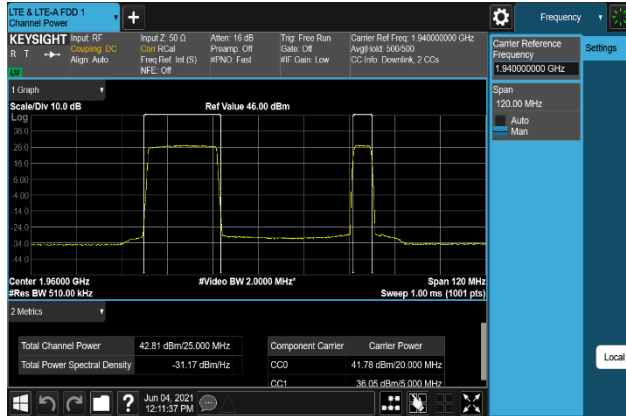
Plot 7-327. Conducted Average Output Power Plot (B2_20M+5M_64QAM, Port 1)
