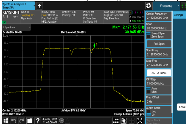
Plot 7-347. Peak To Average Power Radio Plot (B66_15M+10M+10M_64QAM - High Channel, Port 0)
