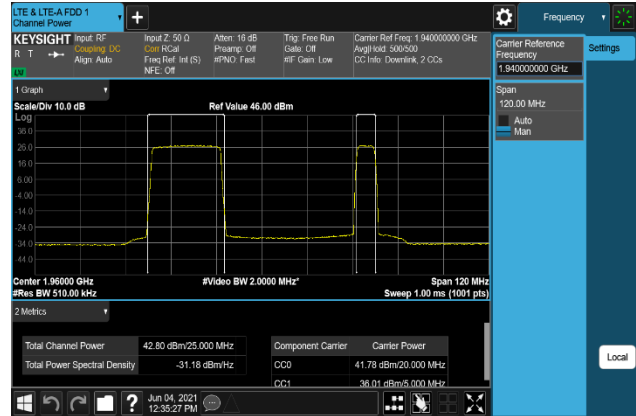
Plot 7-328. Conducted Average Output Power Plot (B2_20M+5M_256QAM, Port 1)
