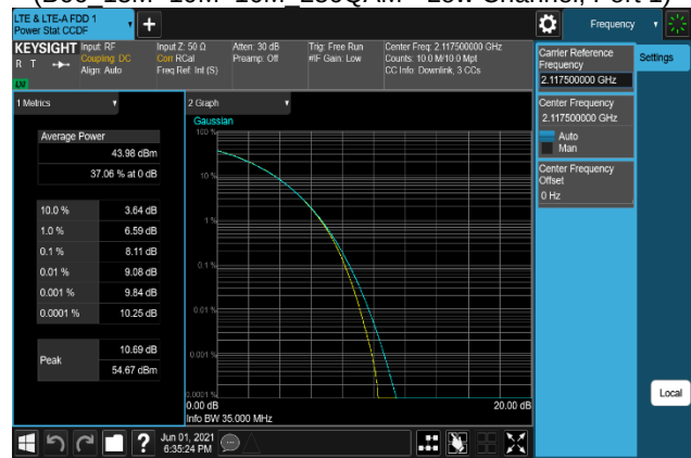
Plot 7-382. Peak To Average Power Ratio Plot (B66_15M+10M+10M_16QAM - Low Channel, Port 2)
