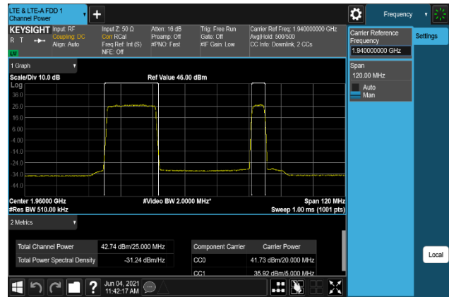
Plot 7-322. Conducted Average Output Power Plot (B2 20M+5M 16QAM, Port 0)
