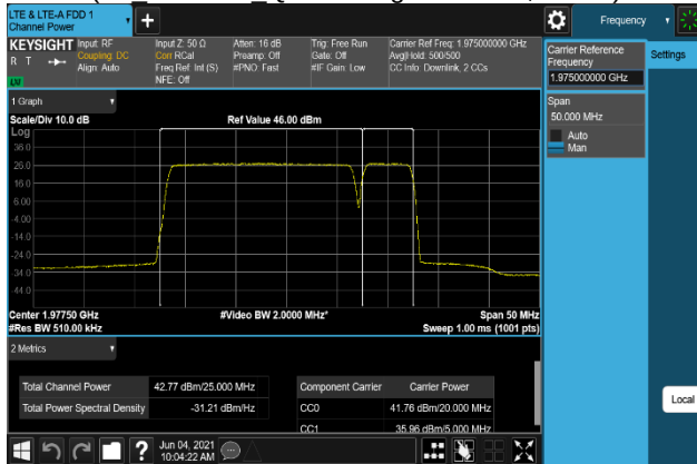
Plot 7-319. Conducted Average Output Power Plot (B2_20M+5M_64QAM - High Channel, Port 3)
