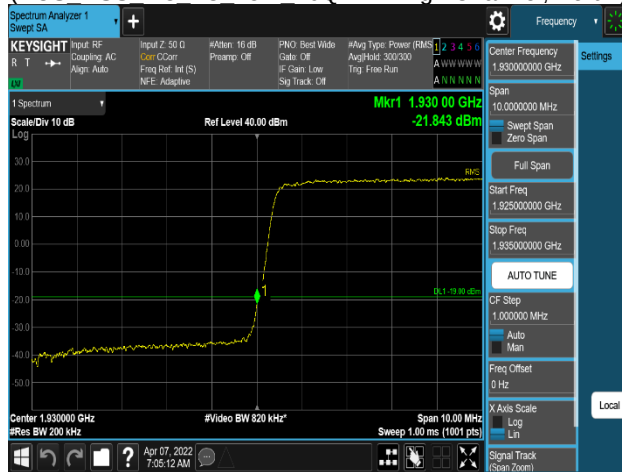
Plot 8-240. Band Edge Emission Plot (PCS_DSS_2:8_1C_20M_64QAM - Low Channel, Port 3)
