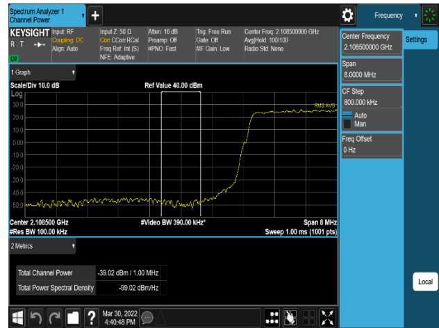
Plot 8-258. Band Edge Emission Plot (AWS NR 1C 10M QPSK - High Channel, Port 2)
