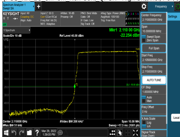
Plot 8-252. Band Edge Emission Plot (AWS_NR_1C_5M_64QAM - Low Channel, Port 1)
