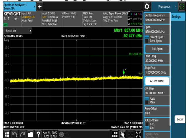
Plot 8-353. Conducted Spurious Emission Plot 30 MHz to 1 GHz (AWS_DSS_1C_15M + LTE_1C_5M_Non-Contiguous_QPSK - Mid Channel, Port 0)
