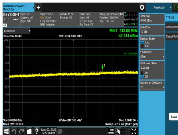
Plot 8-360. Conducted Spurious Emission Plot 30 MHz to 1 GHz (PCS_NR_1C_5M + AWS_NR_1C_5M_Inter CA_QPSK - Mid Channel, Port 0)
