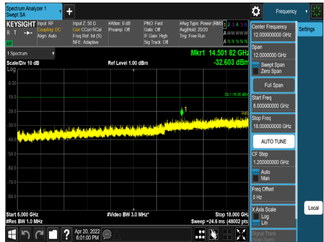
Plot 8-349. Conducted Spurious Emission Plot 6 GHz to 18 GHz (AWS_NR_2C_15M + 20M_QPSK - Mid Channel, Port 0)
