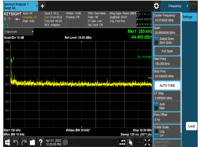
Plot 8-331. Conducted Spurious Emission Plot 150 kHz to 30 MHz (AWS NR 1C 20M 64QAM - Low Channel, Port 3)
