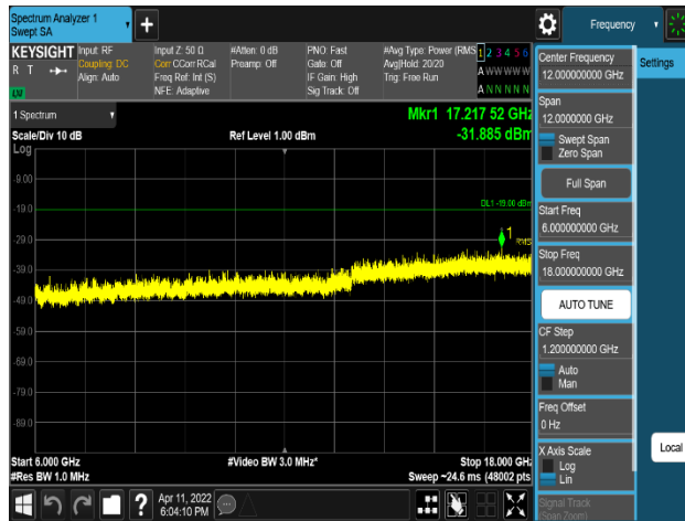
Plot 8-342. Conducted Spurious Emission Plot 6 GHz to 18 GHz (AWS_DSS_Ratio_5:5_1C_20M_256QAM - High Channel, Port 2)
