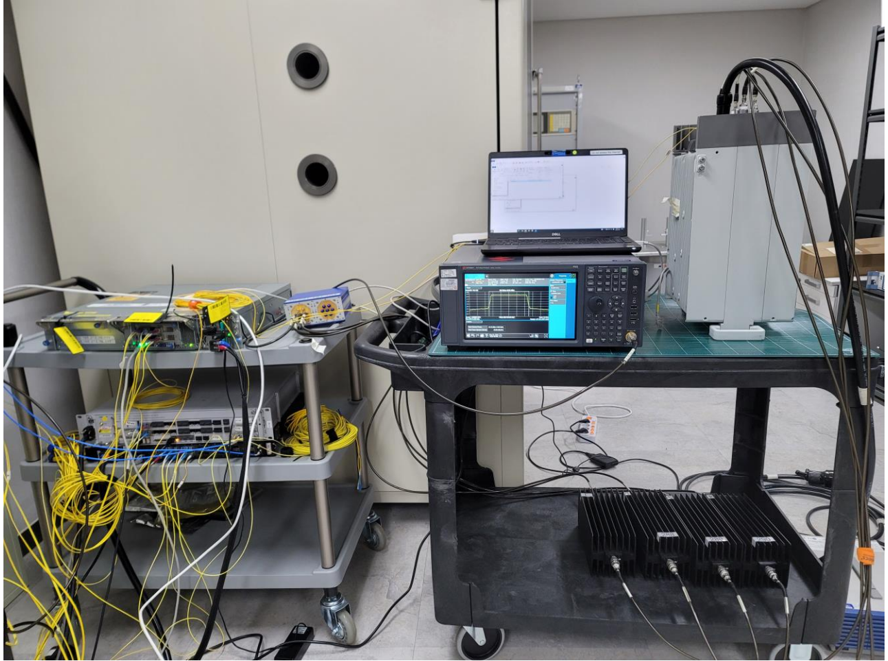
Test Instrument & Measurement Setup Photo
