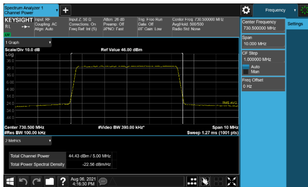
Plot 7-51. Conducted Average Output Power Plot (B85 LTE 1C 5M – Low Channel, 256QAM, Port 0)
