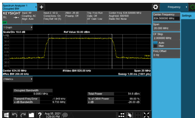
Plot 7-1. Occupied Bandwidth Plot (B71 LTE 1C 10M – Mid Channel, QPSK, Port 3)
