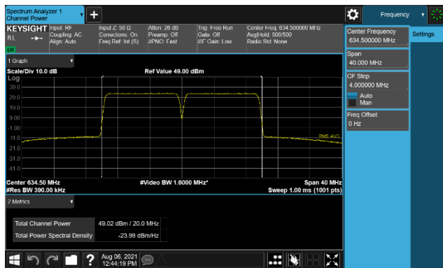
Plot 7-43. Conducted Average Output Power Plot (B71 LTE 2C 10M+10M Conti – Mid Channel, QPSK, Port 0)
