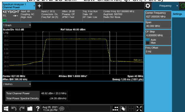
Plot 7-41. Conducted Average Output Power Plot (B71 LTE 1C 20M – Low Channel, QPSK, Port 2)
