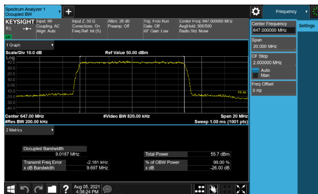
Plot 7-2. Occupied Bandwidth Plot (B71 LTE 1C 10M – High Channel, 16QAM, Port 2)
