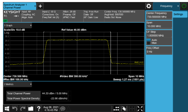
Plot 7-52. Conducted Average Output Power Plot (B85 LTE 1C 5M – Low Channel, 256QAM, Port 1)
