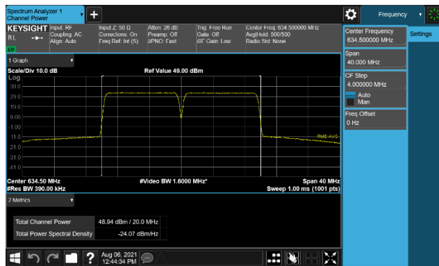
Plot 7-44. Conducted Average Output Power Plot (B71 LTE 2C 10M+10M Conti – Mid Channel, QPSK, Port 1)
