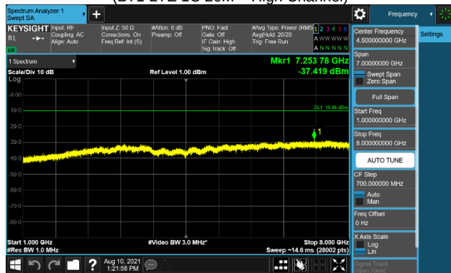
Plot 7-146. Conducted Spurious Emission Plot (1GHz to 8GHz) (B71 LTE 1C 20M – High Channel)
