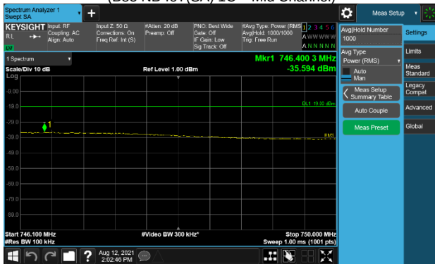
Plot 7-198. Conducted Spurious Emission Plot (746.1MHz to 750MHz) (B85 NB-IoT(SA) 1C – Mid Channel)
