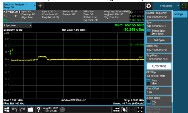
Plot 7-145. Conducted Spurious Emission Plot (652.1MHz to 1GHz) (B71 LTE 1C 20M – High Channel)
