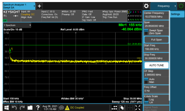
Plot 7-143. Conducted Spurious Emission Plot (150kHz to 30MHz) (B71 LTE 1C 20M – High Channel)
