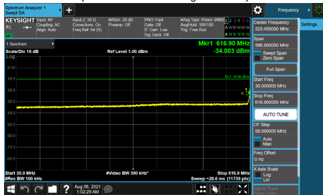
Plot 7-144. Conducted Spurious Emission Plot (30MHz to 616.9MHz) (B71 LTE 1C 20M – High Channel)
