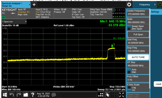
Plot 7-211. Conducted Spurious Emission Plot (30MHz to 720MHz) (B85 NB-IoT(SA) 2C Conti – Low Channel)
