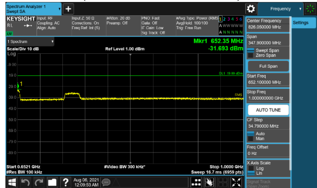
Plot 7-140. Conducted Spurious Emission Plot (652.1MHz to 1GHz) (B71 LTE 1C 20M – Mid Channel)
