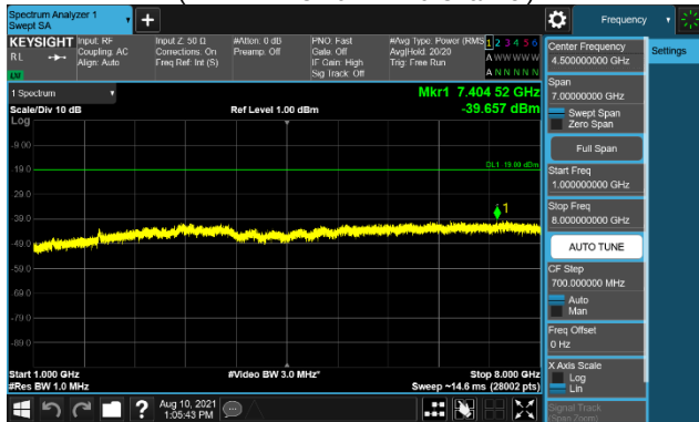
Plot 7-141. Conducted Spurious Emission Plot (1GHz to 8GHz) (B71 LTE 1C 20M – Mid Channel)
