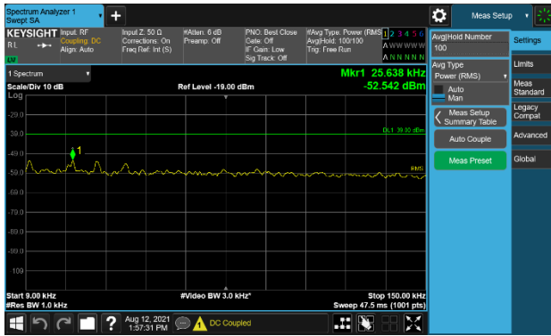
Plot 7-194. Conducted Spurious Emission Plot (9kHz to 150kHz) (B85 NB-IoT(SA) 1C – Mid Channel)
