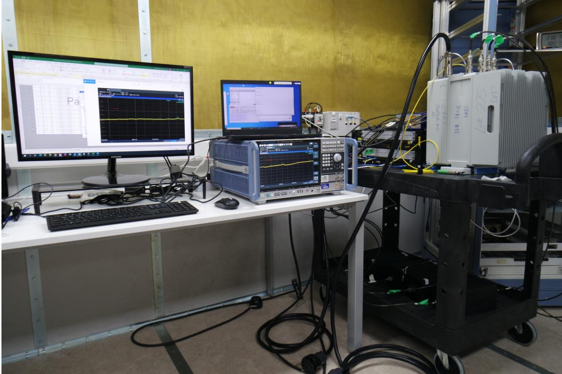
Conducted Test Measurement Setup Photo
