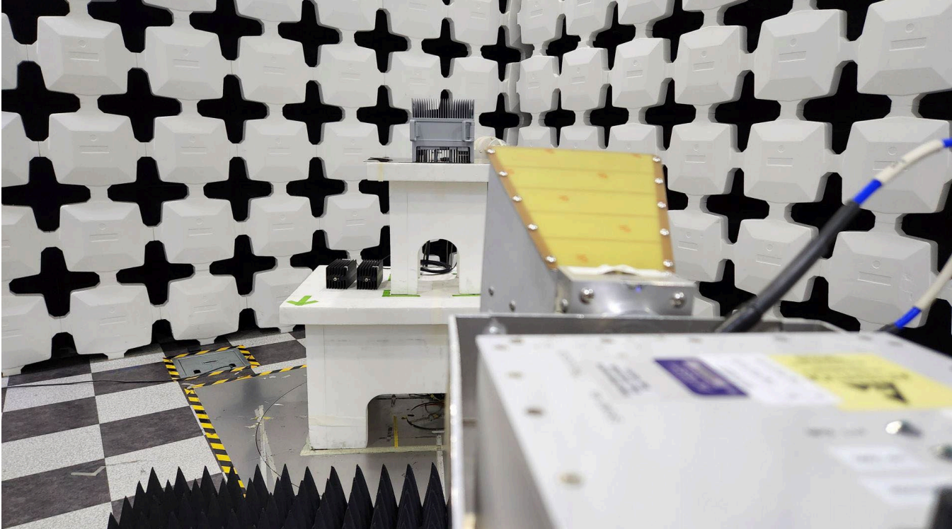
Above 1GHz Test Instrument & Measurement Setup
