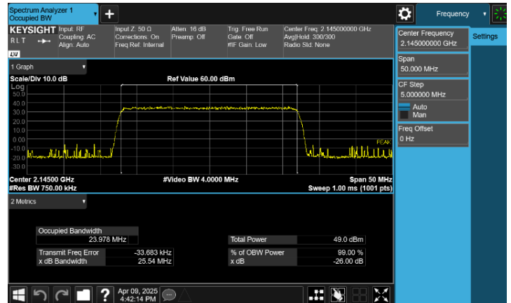
Plot 8-8. Occupied Bandwidth Plot (n66(n4)_NR_1C_25M_64QAM - Mid Channel, Port 1)
