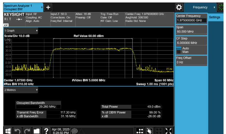
Plot 8-6. Occupied Bandwidth Plot (B/n25(B/n2)_NR_1C_25M+LTE_1C_5M_16QAM - High Channel, Port 0)
