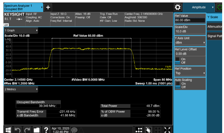
Plot 8-12. Occupied Bandwidth Plot (n66(n4)_NR_3C_5M+10M+25M_16QAM - Mid Channel, Port 2)
