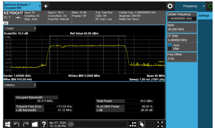
Plot 8-4. Occupied Bandwidth Plot (n25(n2)_NR_2C_5M+25M_16QAM - Low Channel, Port 3)
