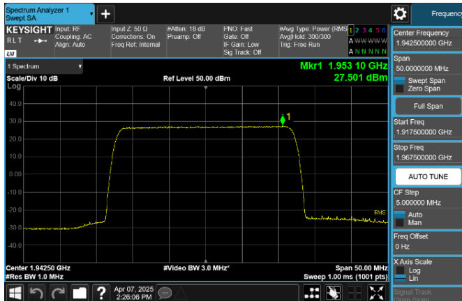
Plot 8-23. Equivalent Radiated Power Plot (n25(n2)_NR_1C_25M_256QAM - Low Channel, Port 0)
