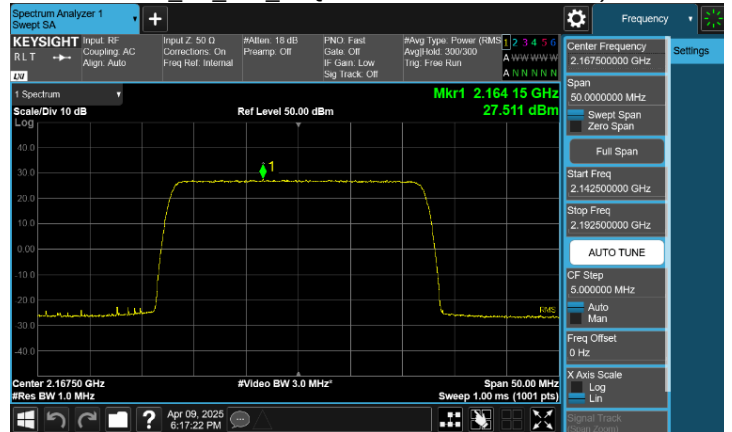
Plot 8-26. Equivalent Radiated Power Plot (n66(n4)_NR_1C_25M_16QAM - High Channel, Port 3)
