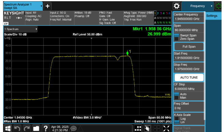
Plot 8-24. Equivalent Radiated Power Plot (n25(n2)_NR_1C_25M +LTE_1C_5M_16QAM - Low Channel, Port 3)
