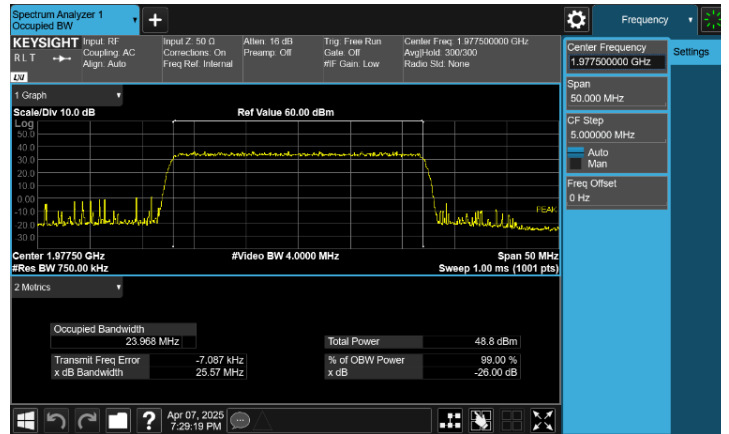
Plot 8-2. Occupied Bandwidth Plot (n25(n2)_NR_1C_25M_16QAM - High Channel, Port 2)
