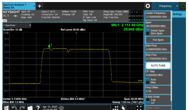
Plot 8-28. Equivalent Radiated Power Plot (n66(n4)_NR_3C_5M+10M+25M_QPSK - Low Channel, Port 3)
