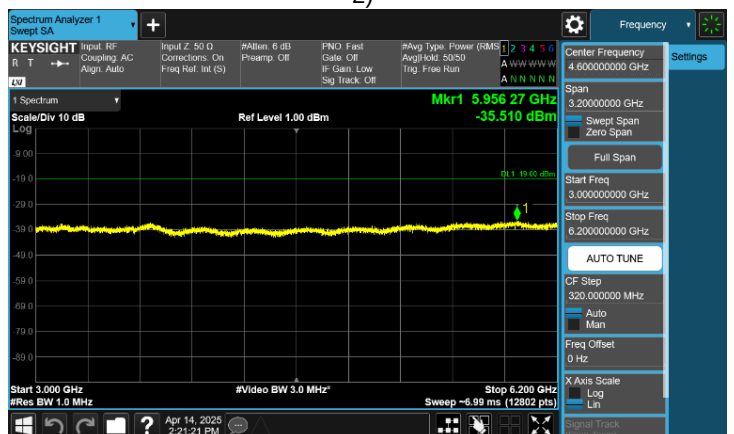
Plot 8-129. Conducted Spurious Emission Plot 3 GHz to 6.2 GHz (B/n66(B/n4)_NC_NR_1C_25M+LTE_2C_10M+5M - QPSK, Port 2)
