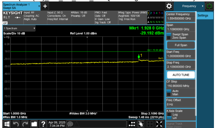
Plot 8-89. Conducted Spurious Emission Plot 1 GHz to 2.109 GHz
