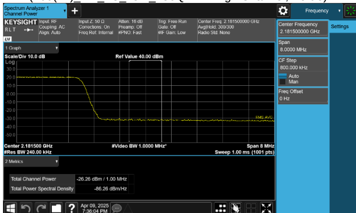
Plot 8-90. Conducted Spurious Emission Plot 2.181 GHz to 2.182 GHz
