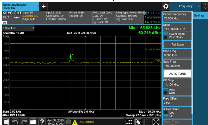
Plot 8-76. Conducted Spurious Emission Plot 9 kHz to 150 kHz (n25(n2)_NR_2NC_5M+25M_QPSK, Port 1)
