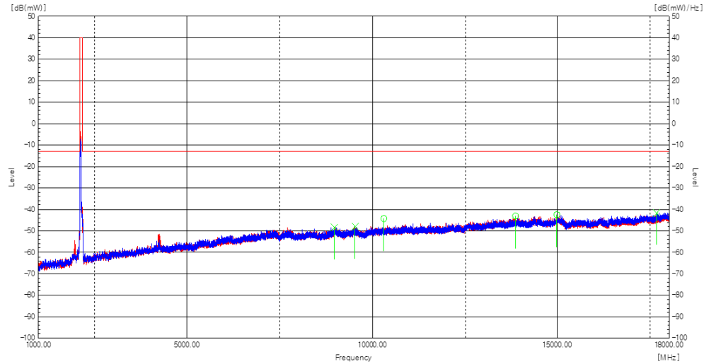
Plot 8-190. Radiated spurious emission Plot_1 GHz to 18 GHz (B/n66(B/n4)_NR_1C_25M+DSS_1C_15M_Mid Channel)
