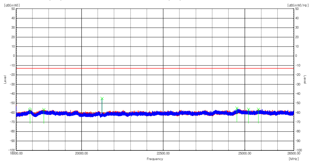
Plot 8-195. Radiated spurious emission Plot_18 GHz to 26.5 GHz (Multi-Band_n25(n2)_NR_3C_5M+5M+20M+n66(n4)_NR_3C_5M+15M+20M_Mid Channel)
