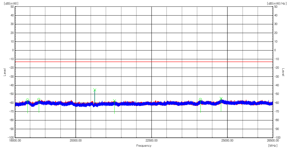
Plot 8-175. Radiated spurious emission Plot_18 GHz to 26.5 GHz (n25(n2)_NR_1C_25M_Mid Channel)
