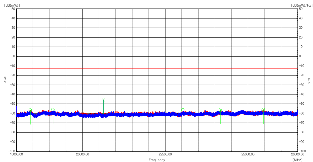
Plot 8-189. Radiated spurious emission Plot_18 GHz to 26.5 GHz (n66(n4)_NR_3C_5M+10M+25M_Mid Channel)
