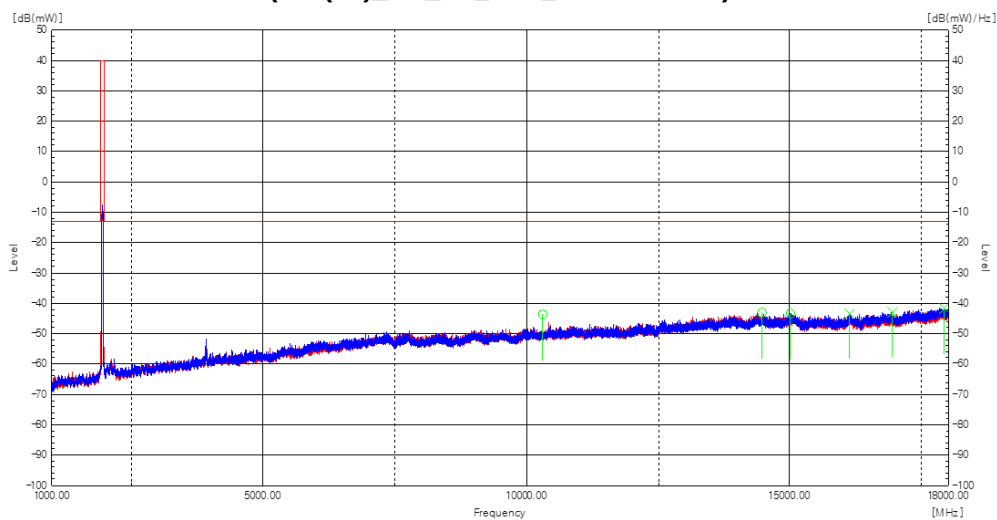
Plot 8-174. Radiated spurious emission Plot_1 GHz to 18 GHz (n25(n2)_NR_1C_25M_Mid Channel)
