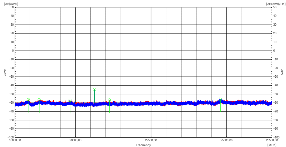
Plot 8-179. Radiated spurious emission Plot_18 GHz to 26.5 GHz (n25(n2)_NR_2C_5M+25M_Low)
