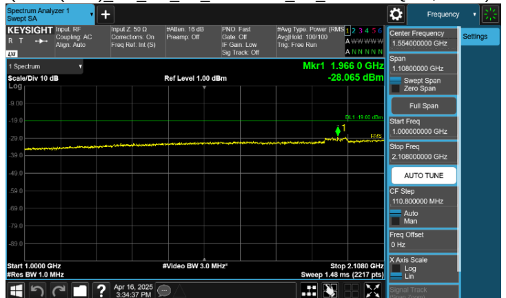
Plot 8-135. Conducted Spurious Emission Plot 1 GHz to 2.108 GHz (B/n66(B/n4)_NC_NR_1C_25M+DSS_1C_15M - 16QAM, Port 3)
