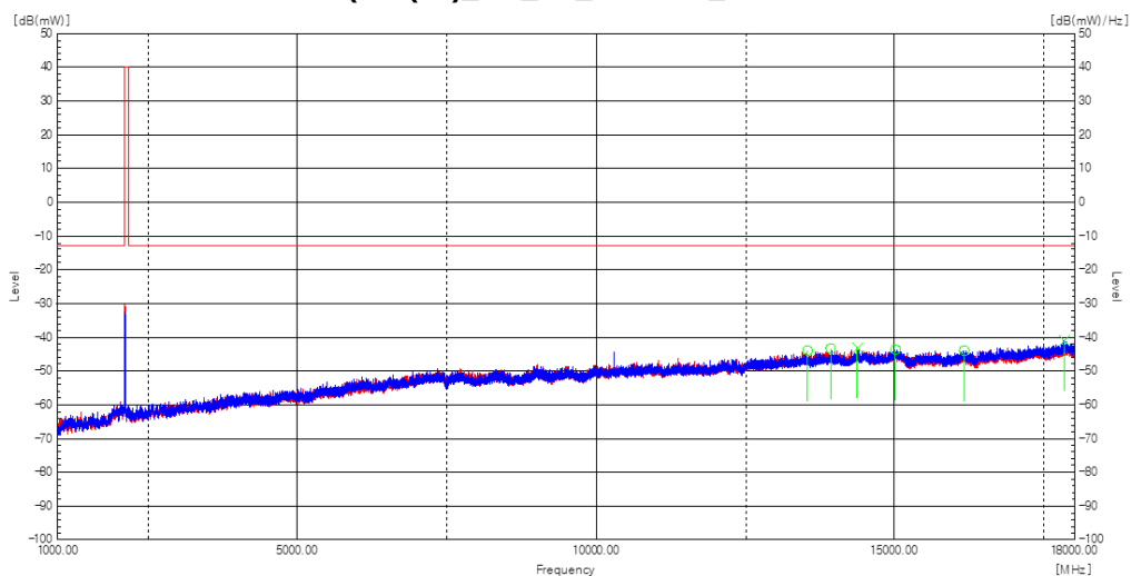
Plot 8-180. Radiated spurious emission Plot_1 GHz to 18 GHz (n66(n4)_NR_1C_25M_Low Channel)
