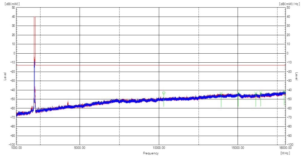
Plot 8-188. Radiated spurious emission Plot_1 GHz to 18 GHz (n66(n4)_NR_3C_5M+10M+25M_Mid Channel)
