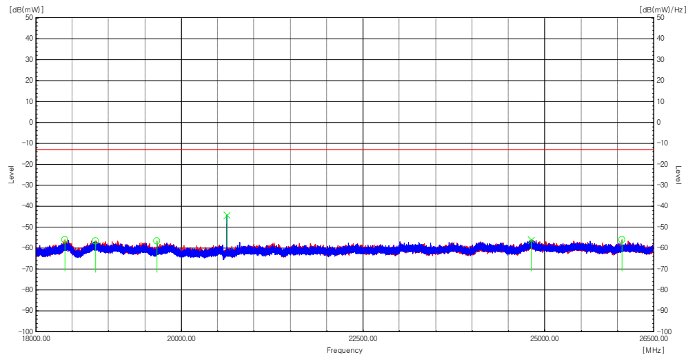
Plot 8-191. Radiated spurious emission Plot_18 GHz to 26.5 GHz (B/n66(B/n4)_NR_1C_25M+DSS_1C_15M_Mid Channel)
