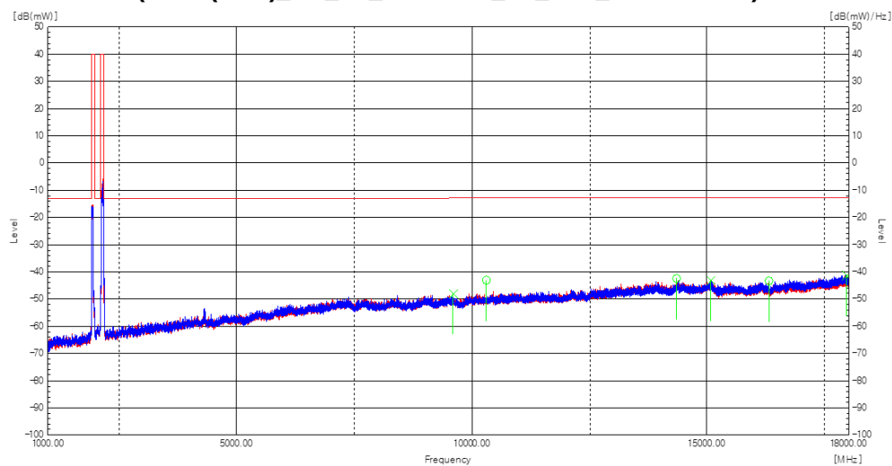
Plot 8-192. Radiated spurious emission Plot_1 GHz to 18 GHz (Multi-Band_n25(n2)_NR_2C_5M+25M+n66(n4)_NR_3C_5M+10M+25M_Mid Channel)
