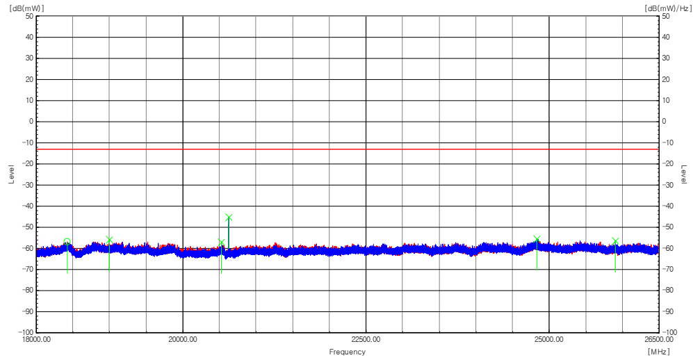
Plot 8-181. Radiated spurious emission Plot_18 GHz to 26.5 GHz (n66(n4)_NR_1C_25M_Low Channel)
