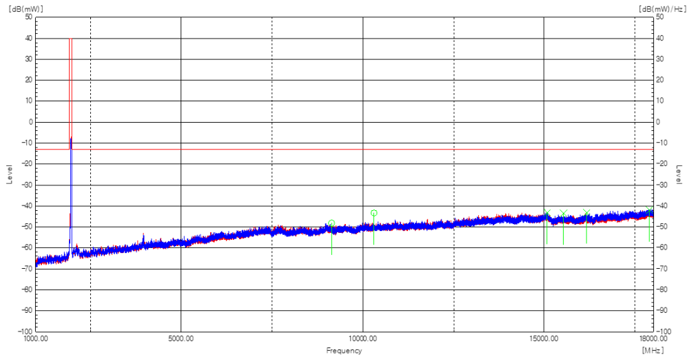
Plot 8-176. Radiated spurious emission Plot_1 GHz to 18 GHz (n25(n2)_NR_1C_25M_High Channel)
