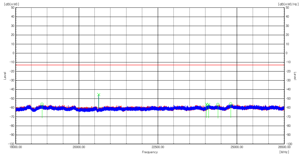
Plot 8-173. Radiated spurious emission Plot_18 GHz to 26.5 GHz (n25(n2)_NR_1C_25M_Low Channel)
