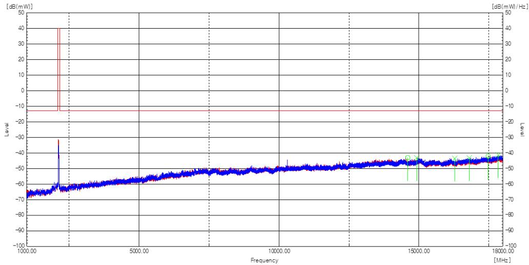
Plot 8-182. Radiated spurious emission Plot_1 GHz to 18 GHz (n66(n4)_NR_1C_25M_Mid Channel)
