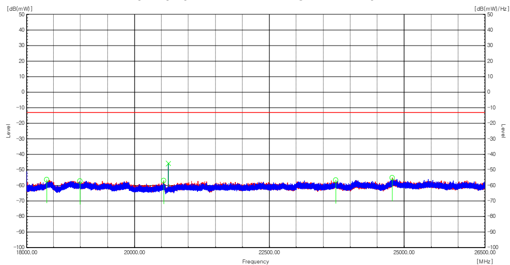
Plot 8-177. Radiated spurious emission Plot_18 GHz to 26.5 GHz (n25(n2)_NR_1C_25M_High Channel)
