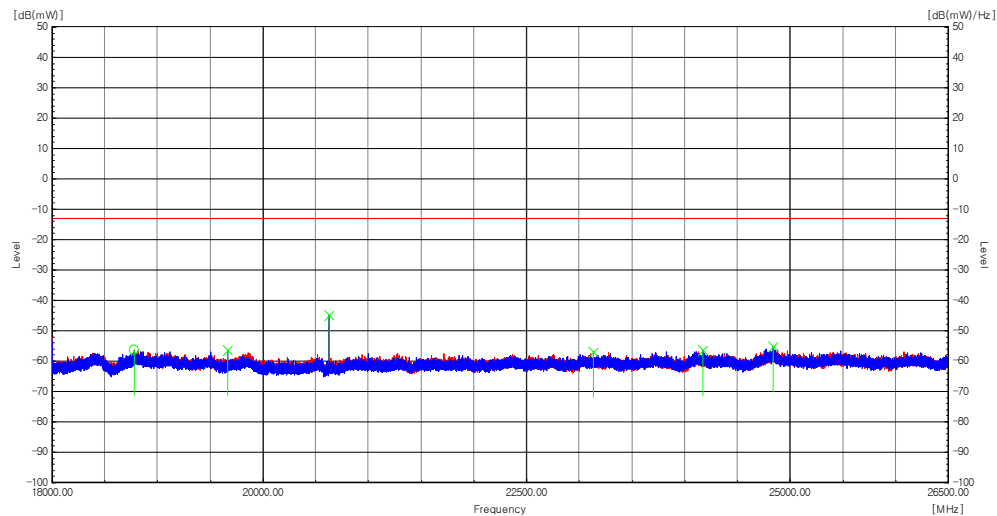
Plot 8-183. Radiated spurious emission Plot_18 GHz to 26.5 GHz (n66(n4)_NR_1C_25M_Mid Channel)
