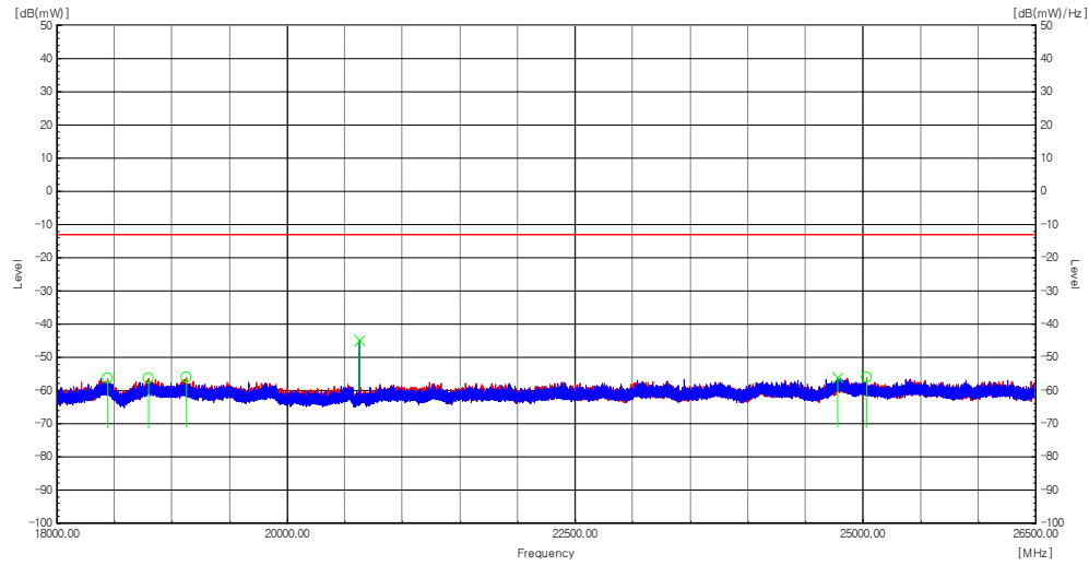
Plot 8-187. Radiated spurious emission Plot_18 GHz to 26.5 GHz (n66(n4)_NR_1C_30M_Low Channel)
