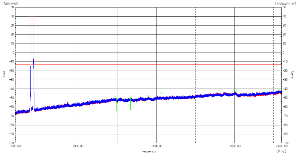
Plot 8-194. Radiated spurious emission Plot_1 GHz to 18 GHz (Multi-Band_n25(n2)_NR_3C_5M+5M+20M+n66(n4)_NR_3C_5M+15M+20M_Mid Channel)
