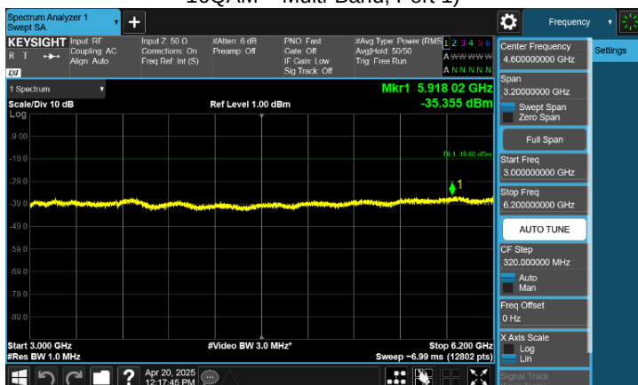
Plot 8-152. Conducted Spurious Emission Plot 3 GHz to 6.2 GHz (n25(n2)_NR_3C_5M+5M+20M+B/n66(B/n4)_NR_2C_10M+30M_16QAM – Multi-Band, Port 1)
