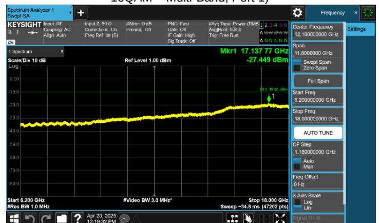
Plot 8-153. Conducted Spurious Emission Plot 6.2 GHz to 18 GHz (n25(n2)_NR_3C_5M+5M+20M+B/n66(B/n4)_NR_2C_10M+30M_16QAM – Multi-Band, Port 1)
