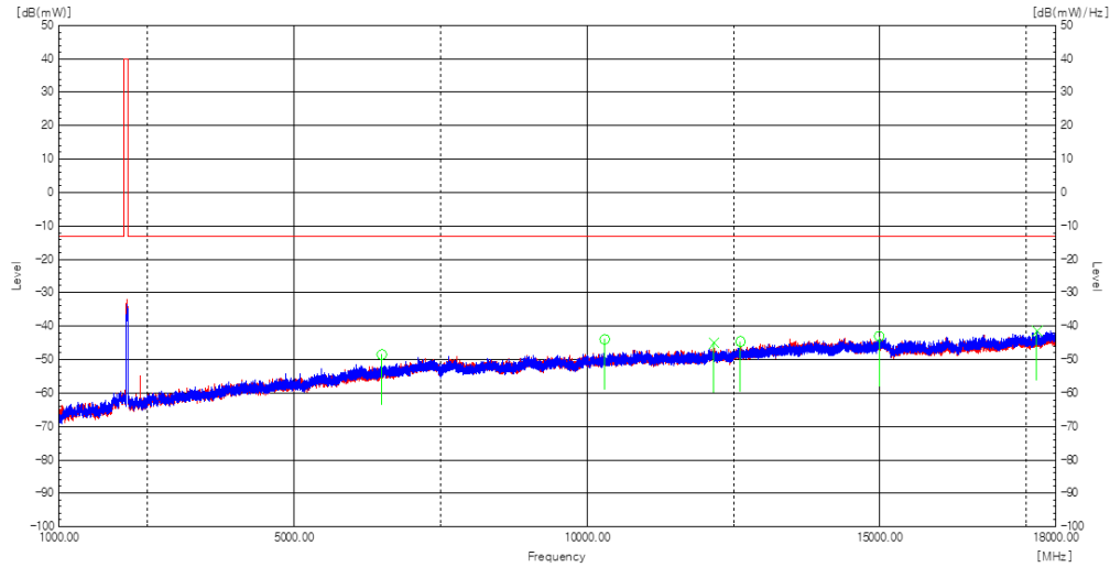
Plot 8-184. Radiated spurious emission Plot_1 GHz to 18 GHz (n66(n4)_NR_1C_25M_High Channel)
