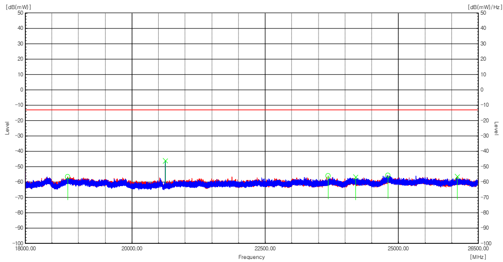
Plot 8-185. Radiated spurious emission Plot_18 GHz to 26.5 GHz (n66(n4)_NR_1C_25M_High Channel)
