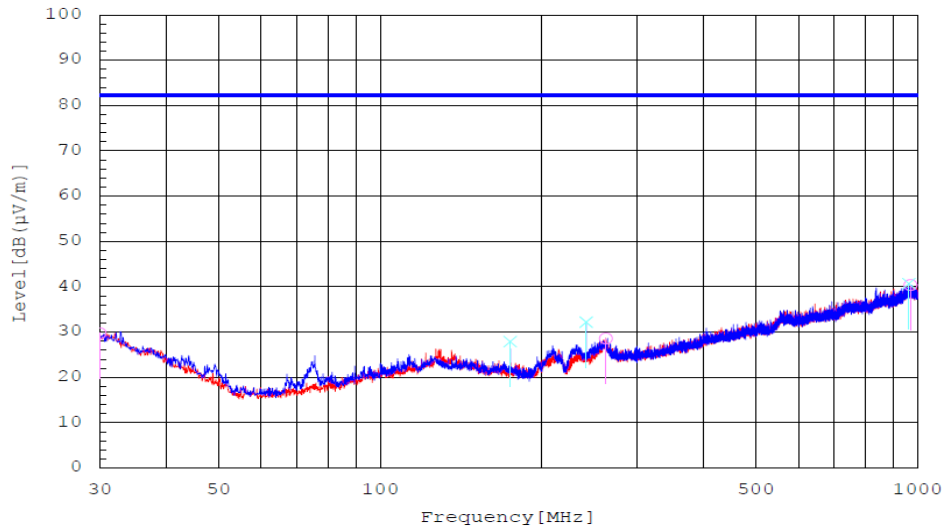
Plot 8-171. Radiated spurious emission Plot_30 MHz to 1000 MHz (B/n66(B/n4)_NR_1C_30M+DSS_1C_10M+LTE_1C_5M_High Channel)
