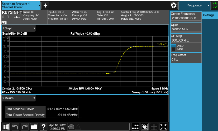
Plot 8-136. Conducted Spurious Emission Plot 2.108 GHz to 2.109 GHz
