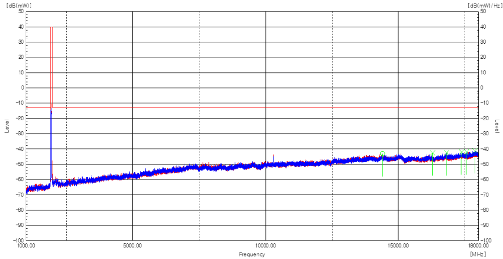
Plot 8-172. Radiated spurious emission Plot_1 GHz to 18 GHz (n25(n2)_NR_1C_25M_Low Channel)
