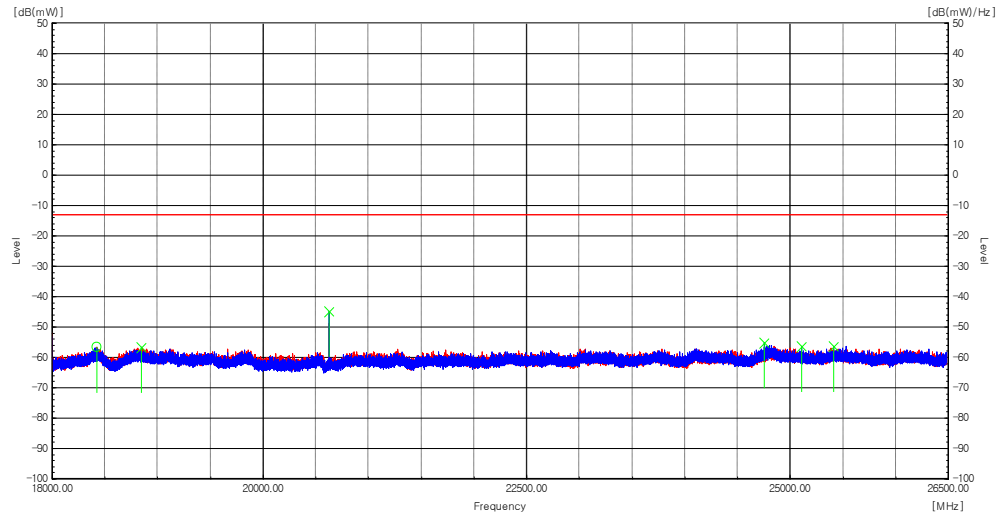
Plot 8-193. Radiated spurious emission Plot_18 GHz to 26.5 GHz (Multi-Band_n25(n2)_NR_2C_5M+25M+n66(n4)_NR_3C_5M+10M+25M_Mid Channel)
