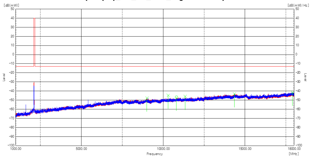
Plot 8-186. Radiated spurious emission Plot_1 GHz to 18 GHz (n66(n4)_NR_1C_30M_Low Channel)
