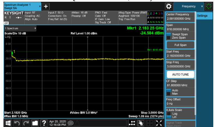
Plot 8-151. Conducted Spurious Emission Plot 2.182 GHz to 3 GHz (n25(n2)_NR_3C_5M+5M+20M+B/n66(B/n4)_NR_2C_10M+30M_16QAM – Multi-Band, Port 1)
