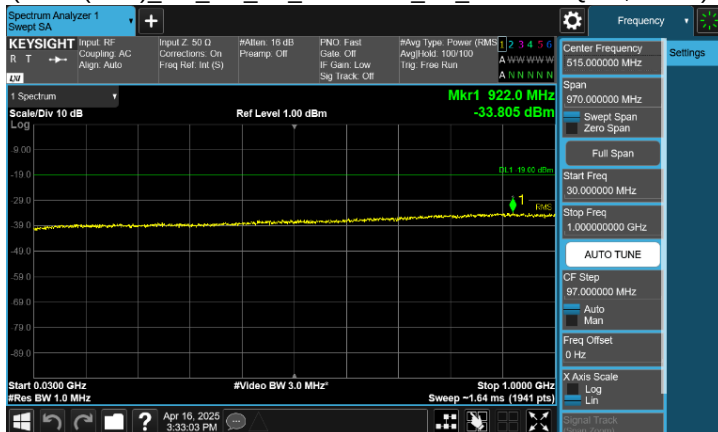
Plot 8-134. Conducted Spurious Emission Plot 30 MHz to 1 GHz (B/n66(B/n4)_NC_NR_1C_25M+DSS_1C_15M - 16QAM, Port 3)
