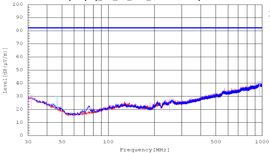
Plot 8-169. Radiated spurious emission Plot_30 MHz to 1000 MHz (B/n25(B/n2)_NR_1C_25M+LTE_1C_5M_High Channel)
