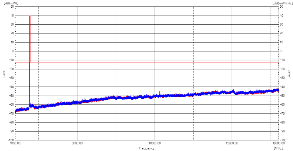
Plot 8-178. Radiated spurious emission Plot_1 GHz to 18 GHz (n25(n2)_NR_2C_5M+25M_Low Channel)
