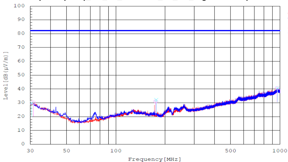
Plot 8-170. Radiated spurious emission Plot_30 MHz to 1000 MHz (n66(n4)_NR_1C_30M_Mid Channel)
