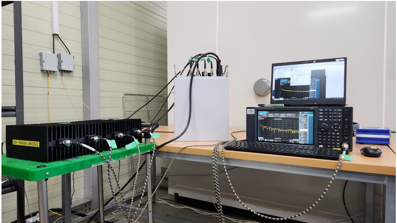
Conducted Test Instrument & Measurement Setup
