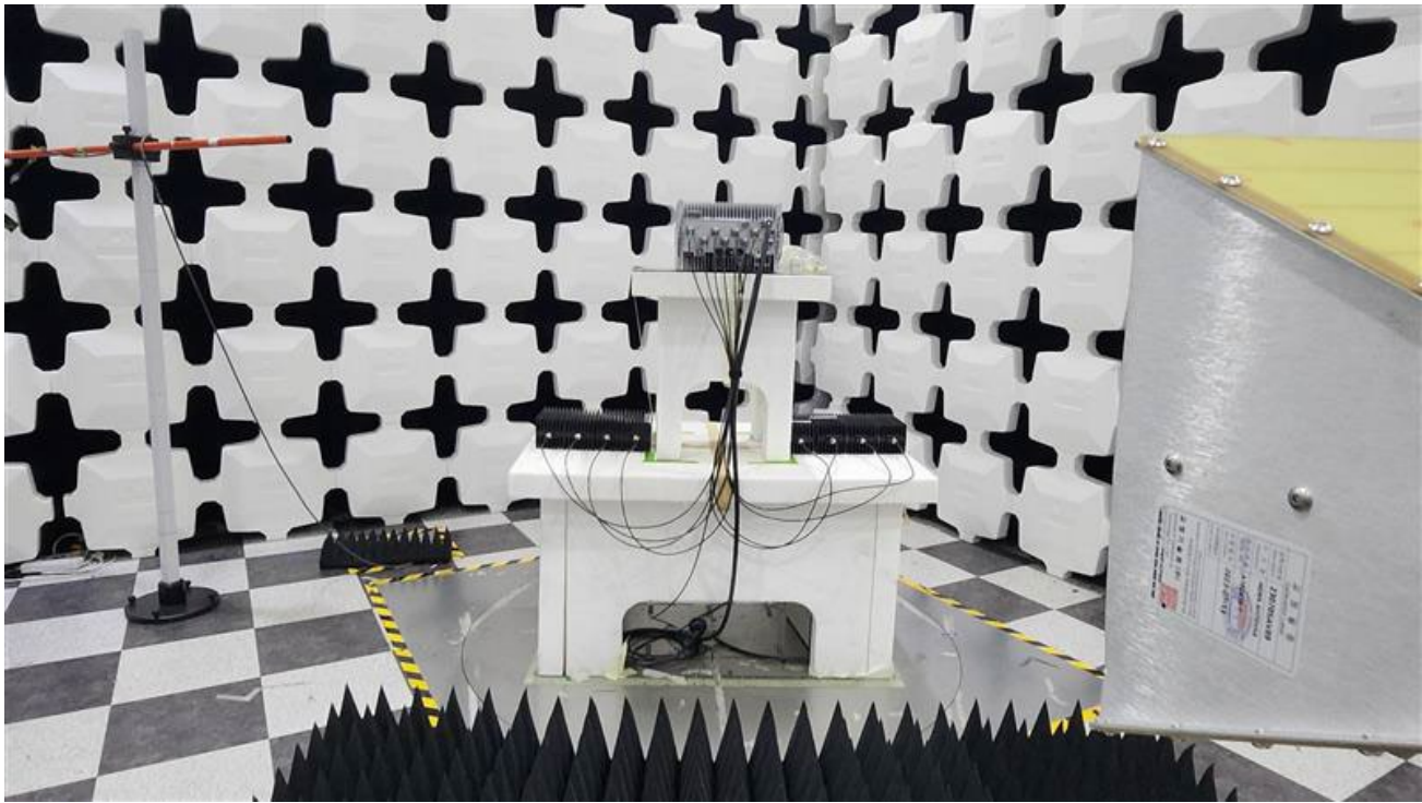
Above 1GHz Test Instrument & Measurement Setup > 1GHz
