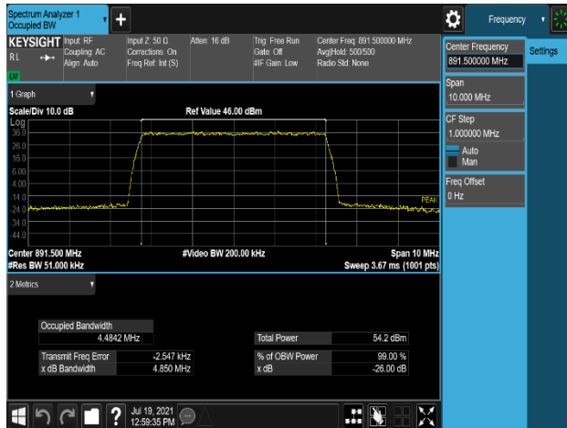
Plot 7-9. Occupied Bandwidth Plot (B5_5M_1C_QPSK - High Channel, Port 1)
