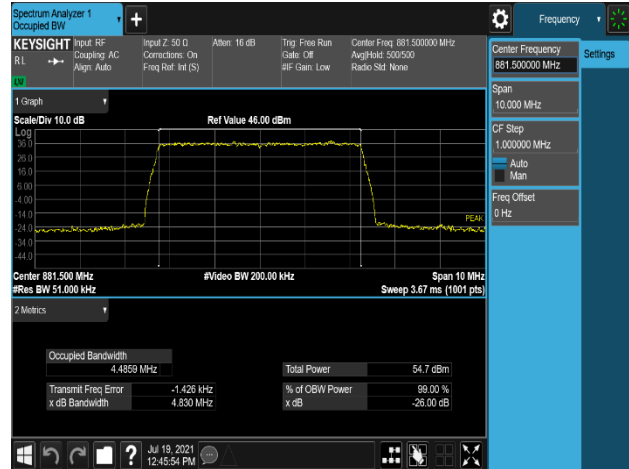
Plot 7-8. Occupied Bandwidth Plot (B5_5M_1C_256QAM - Mid Channel, Port 0)
