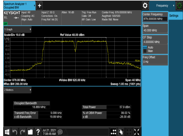
Plot 7-62. Occupied Bandwidth Plot (B5_10M+10M_2C_16QAM - Low Channel, Port 0)
