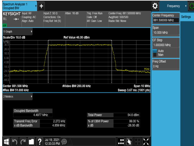
Plot 7-7. Occupied Bandwidth Plot (B5_5M_1C_64QAM - Mid Channel, Port 0)
