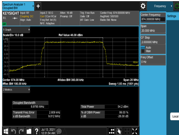
Plot 7-39. Occupied Bandwidth Plot (B5_10M_1C_64QAM - Low Channel, Port 1)
