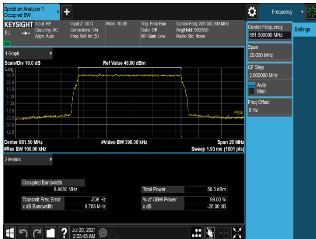
Plot 7-17. Occupied Bandwidth Plot (B5_10M_1C_QPSK - Mid Channel, Port 0)
