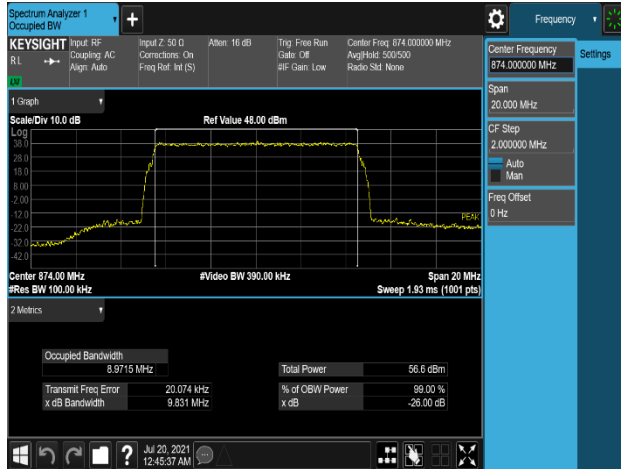
Plot 7-13. Occupied Bandwidth Plot (B5_10M_1C_QPSK - Low Channel, Port 1)
