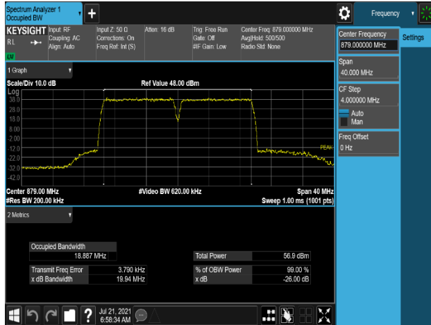
Plot 7-61. Occupied Bandwidth Plot (B5_10M+10M_2C_QPSK - Low Channel, Port 0)
