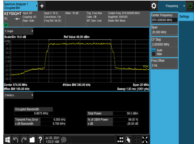
Plot 7-14. Occupied Bandwidth Plot (B5_10M_1C_16QAM - Low Channel, Port 0)
