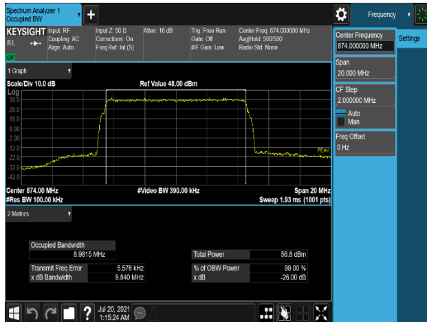
Plot 7-15. Occupied Bandwidth Plot (B5_10M_1C_64QAM - Low Channel, Port 0)
