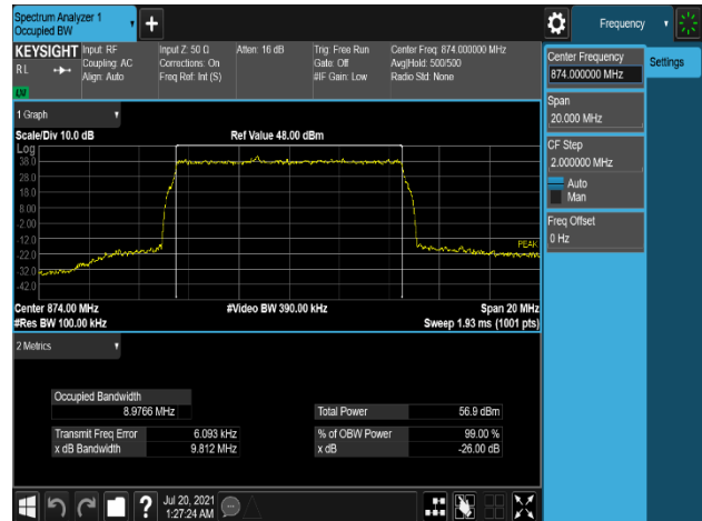
Plot 7-16. Occupied Bandwidth Plot (B5_10M_1C_256QAM - Low Channel, Port 0)
