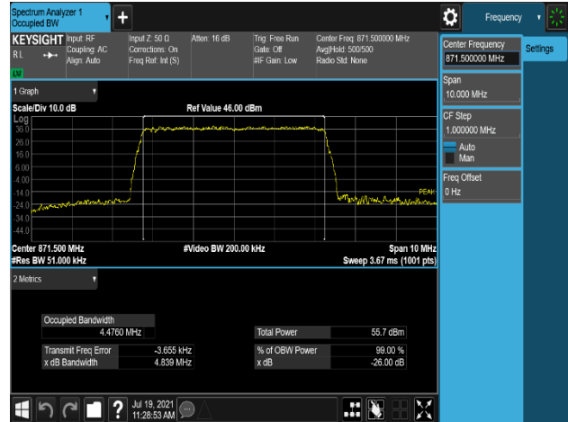
Plot 7-2. Occupied Bandwidth Plot (B5_5M_1C_16QAM - Low Channel, Port 0)
