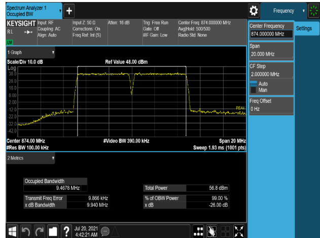
Plot 7-52. Occupied Bandwidth Plot (B5_5M+5M_2C_256QAM - Low Channel, Port 0)
