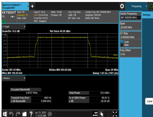
Plot 7-41. Occupied Bandwidth Plot (B5_10M_1C_QPSK - Mid Channel, Port 2)
