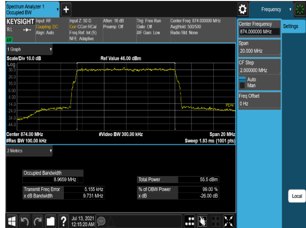
Plot 7-38. Occupied Bandwidth Plot (B5_10M_1C_16QAM - Low Channel, Port 2)
