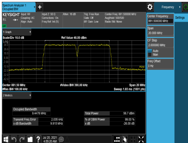
Plot 7-53. Occupied Bandwidth Plot (B5_5M+5M_2C_QPSK - Mid Channel, Port 0)
