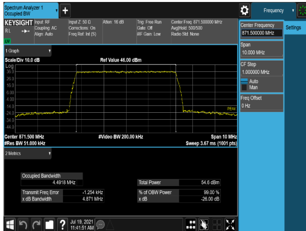
Plot 7-3. Occupied Bandwidth Plot (B5_5M_1C_64QAM - Low Channel, Port 0)
