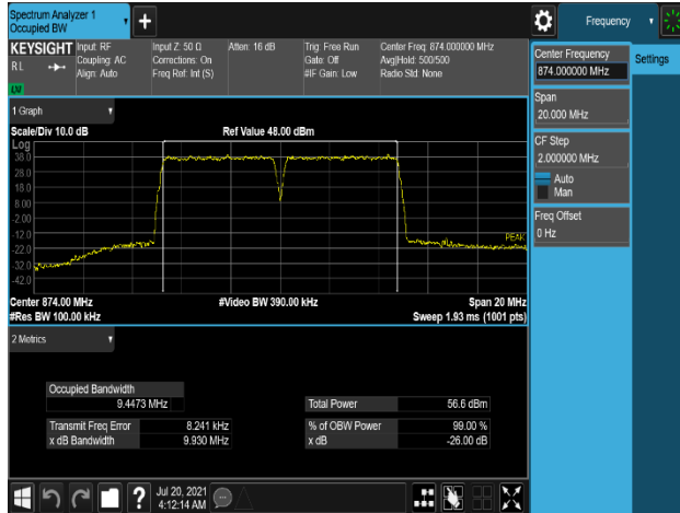
Plot 7-49. Occupied Bandwidth Plot (B5_5M+5M_2C_QPSK - Low Channel, Port 0)
