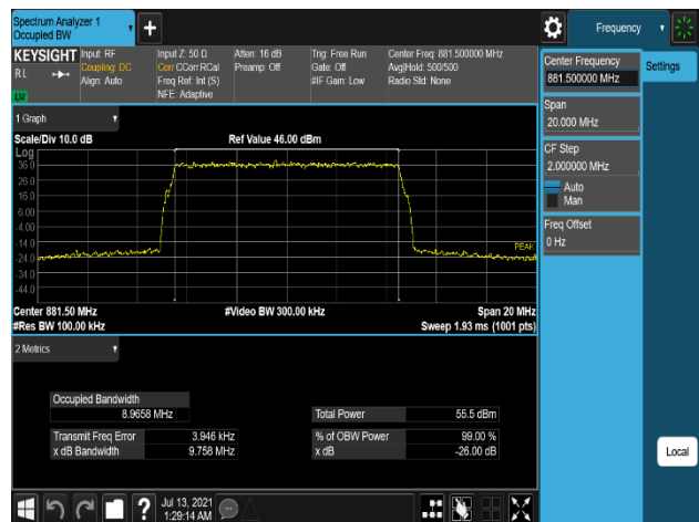
Plot 7-42. Occupied Bandwidth Plot (B5_10M_1C_16QAM - Mid Channel, Port 2)
