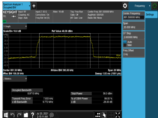
Plot 7-18. Occupied Bandwidth Plot (B5_10M_1C_16QAM - Mid Channel, Port 0)
