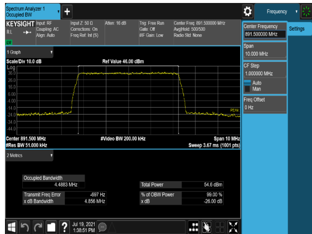
Plot 7-12. Occupied Bandwidth Plot (B5_5M_1C_256QAM - High Channel, Port 1)
