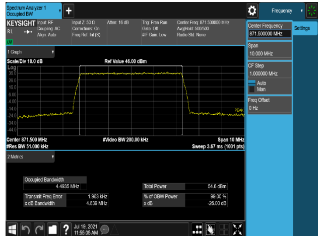
Plot 7-4. Occupied Bandwidth Plot (B5_5M_1C_256QAM - Low Channel, Port 1)
