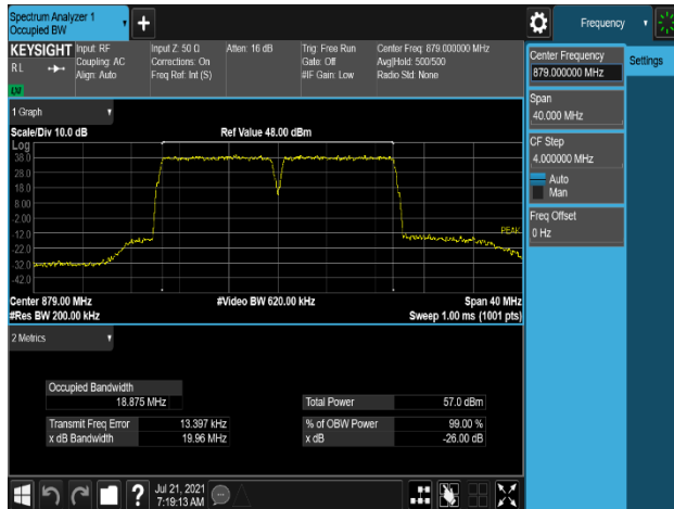
Plot 7-63. Occupied Bandwidth Plot (B5_10M+10M_2C_64QAM - Low Channel, Port 1)
