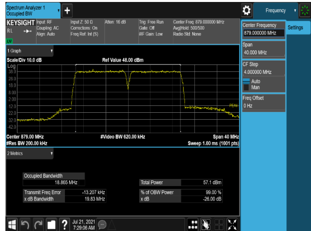
Plot 7-64. Occupied Bandwidth Plot (B5_10M+10M_2C_256QAM - Low Channel, Port 0)
