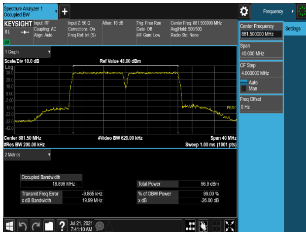
Plot 7-65. Occupied Bandwidth Plot (B5_10M+10M_2C_QPSK - Mid Channel, Port 0)
