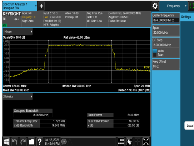
Plot 7-37. Occupied Bandwidth Plot (B5_10M_1C_QPSK - Low Channel, Port 0)
