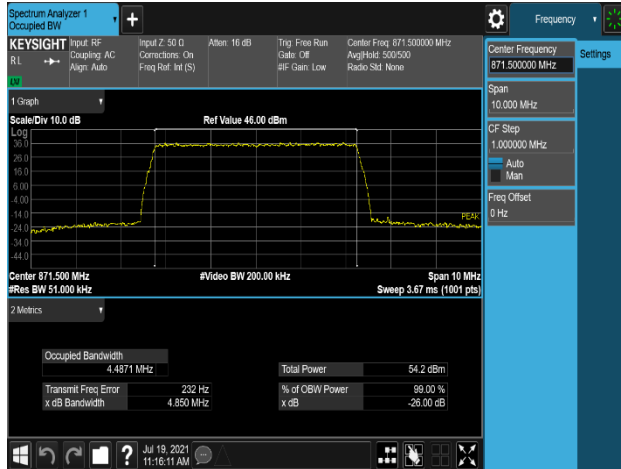
Plot 7-1. Occupied Bandwidth Plot (B5_5M_1C_QPSK - Low Channel, Port 1)
