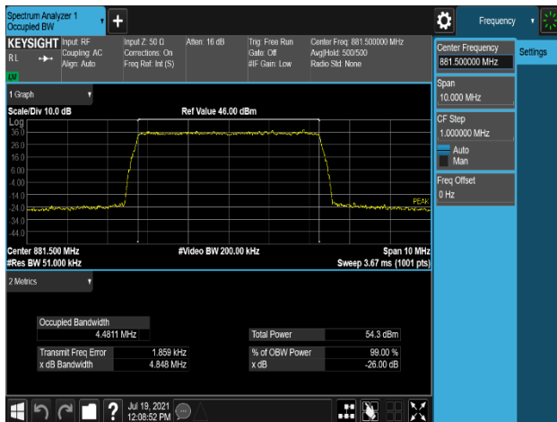
Plot 7-5. Occupied Bandwidth Plot (B5_5M_1C_QPSK - Mid Channel, Port 0)
