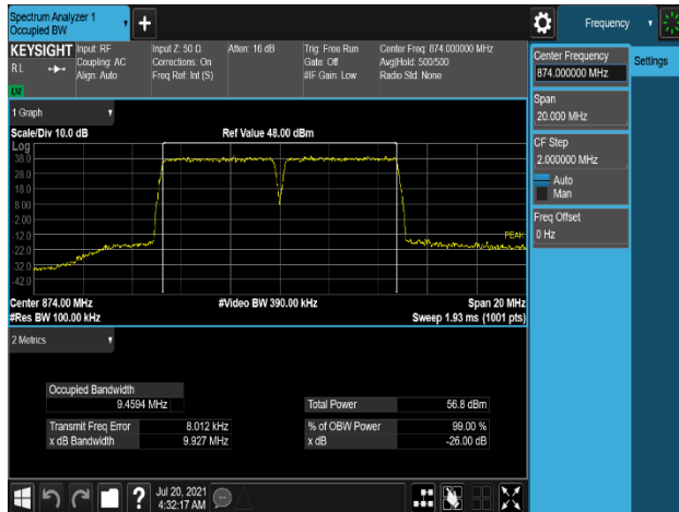
Plot 7-51. Occupied Bandwidth Plot (B5_5M+5M_2C_64QAM - Low Channel, Port 0)
