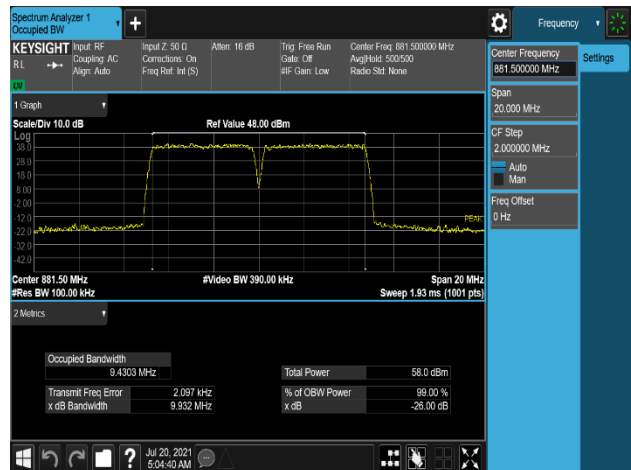
Plot 7-54. Occupied Bandwidth Plot (B5_5M+5M_2C_16QAM - Mid Channel, Port 0)
