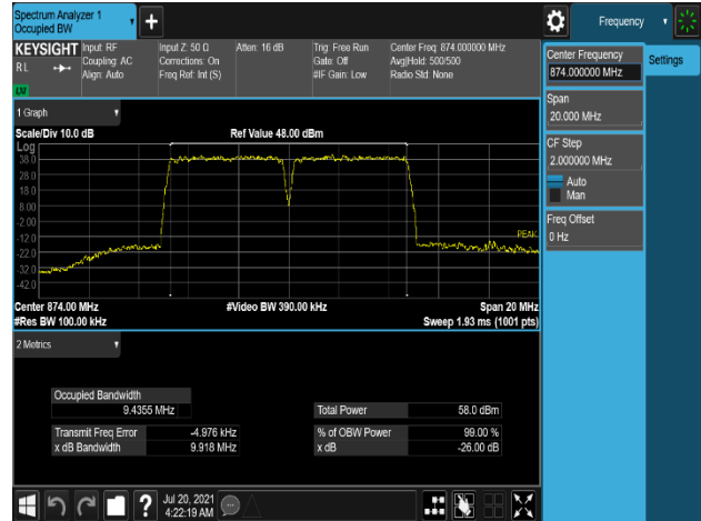
Plot 7-50. Occupied Bandwidth Plot (B5_5M+5M_2C_16QAM - Low Channel, Port 0)
