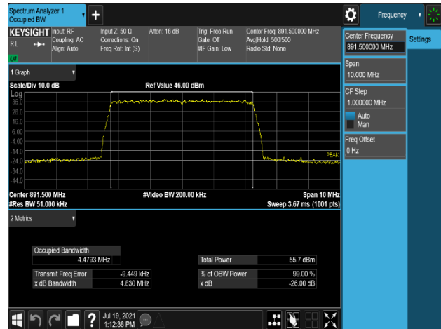
Plot 7-10. Occupied Bandwidth Plot (B5_5M_1C_16QAM - High Channel, Port 1)
