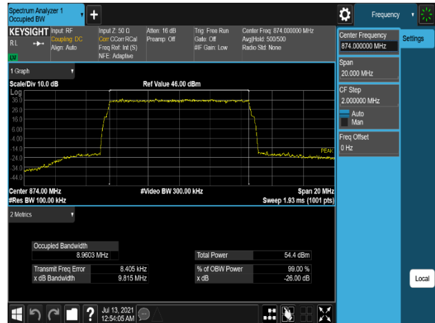
Plot 7-40. Occupied Bandwidth Plot (B5_10M_1C_256QAM - Low Channel, Port 2)
