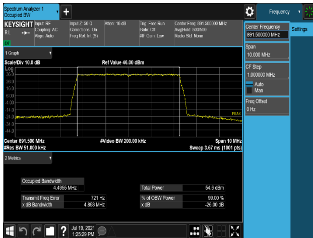
Plot 7-11. Occupied Bandwidth Plot (B5_5M_1C_64QAM - High Channel, Port 0)
