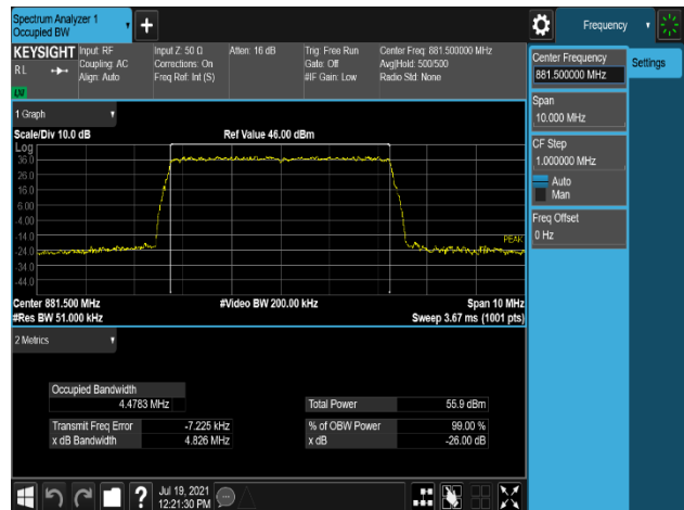
Plot 7-6. Occupied Bandwidth Plot (B5_5M_1C_16QAM - Mid Channel, Port 1)
