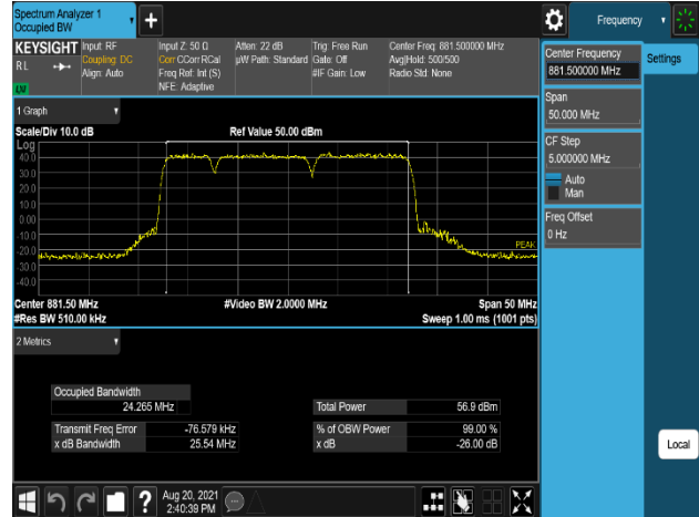
Plot 7-232. Occupied Bandwidth Plot (B5_10M(DSS)+10M+5M_3C_16QAM - Port 0)
