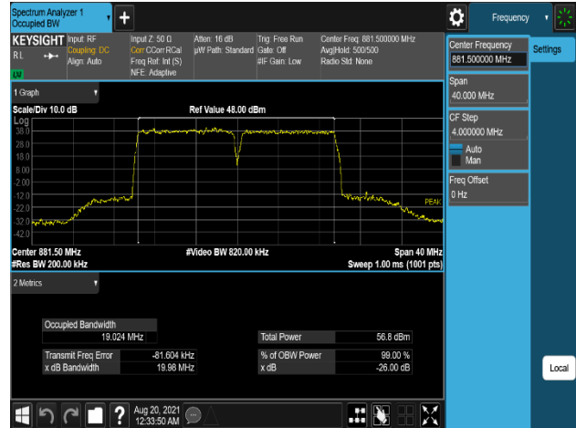
Plot 7-222. Occupied Bandwidth Plot (B5_10M(DSS)+10M_2C_256QAM - Mid Channel, Port 0)
