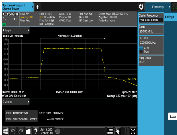
Plot 7-269. Conducted Average Output Power Plot (B5_10M_1C_QPSK – High Channel, Port 2)
