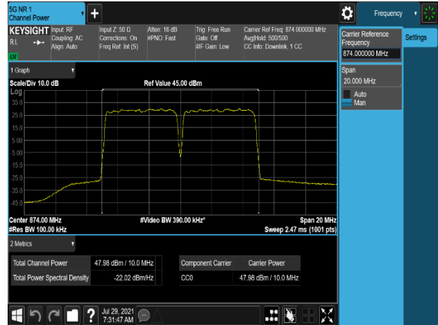
Plot 7-272. Conducted Average Output Power Plot (B5_5M+5M_2C_16QAM - Low Channel, Port 1)
