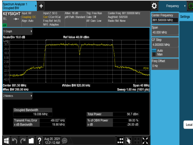
Plot 7-221. Occupied Bandwidth Plot (B5_10M(DSS)+10M_2C_64QAM - Mid Channel, Port 0)
