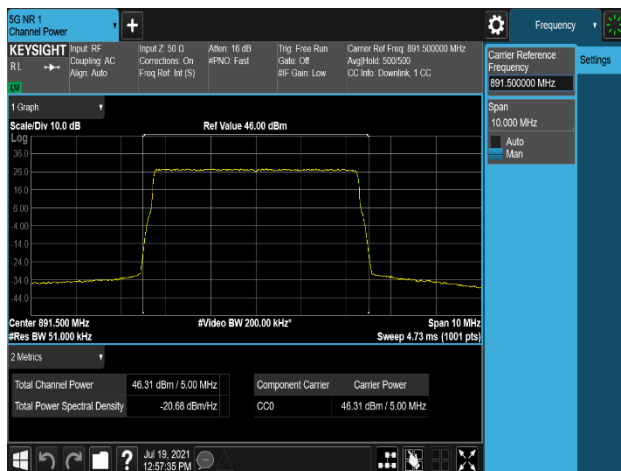
Plot 7-239. Conducted Average Output Power Plot (B5_5M_1C_QPSK - High Channel, Port 0)
