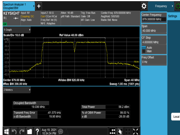
Plot 7-215. Occupied Bandwidth Plot (B5_10M(DSS)+10M_2C_QPSK - Low Channel, Port 1)
