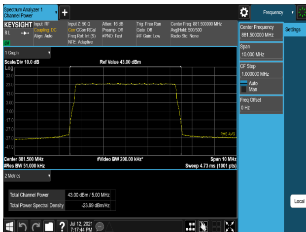
Plot 7-251. Conducted Average Output Power Plot (B5_5M_1C_256QAM - Mid Channel, Port 0)
