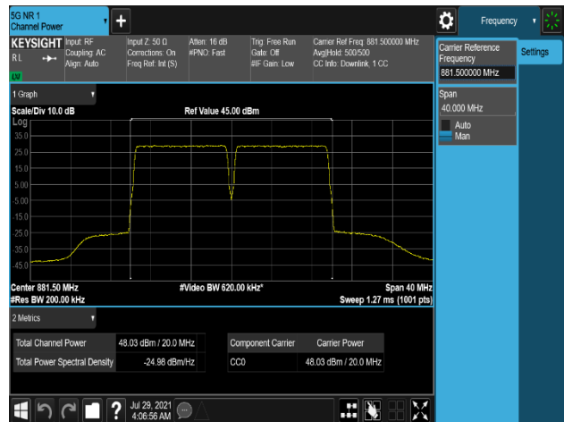
Plot 7-280. Conducted Average Output Power Plot (B5_10M+10M_2C_QPSK - Mid Channel, Port 1)
