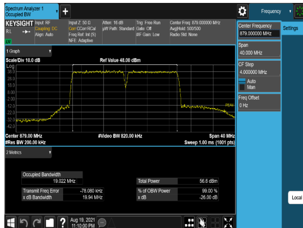
Plot 7-217. Occupied Bandwidth Plot (B5_10M(DSS)+10M_2C_64QAM - Low Channel, Port 0)
