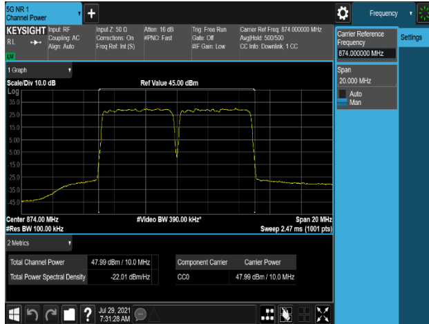
Plot 7-271. Conducted Average Output Power Plot (B5_5M+5M_2C_16QAM - Low Channel, Port 0)
