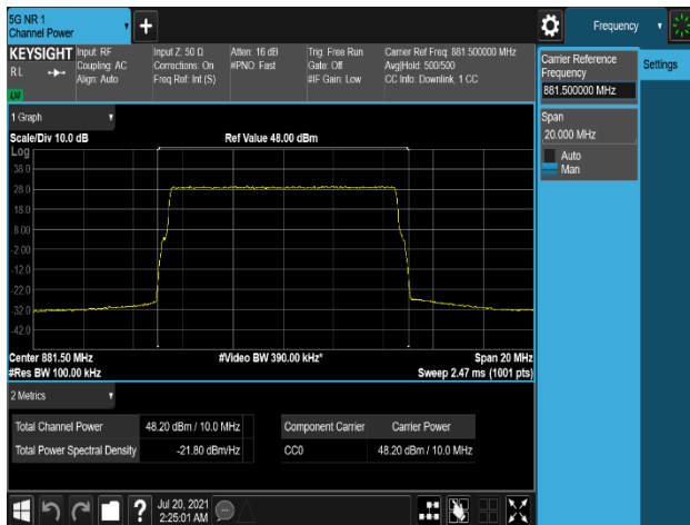
Plot 7-243. Conducted Average Output Power Plot (B5_10M_1C_64QAM - Mid Channel, Port 0)
