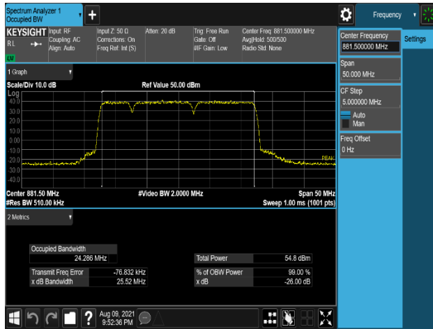
Plot 7-227. Occupied Bandwidth Plot (B5_10M(DSS)+10M+5M_3C_QPSK - Port 0)
