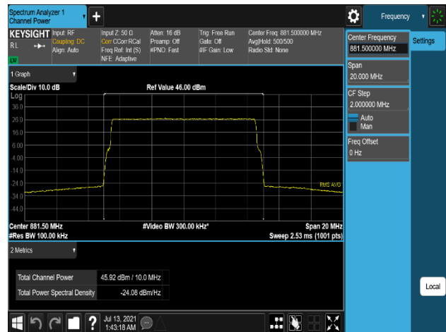
Plot 7-266. Conducted Average Output Power Plot (B5_10M_1C_64QAM – Mid Channel, Port 3)
