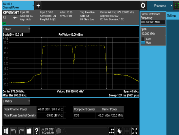
Plot 7-277. Conducted Average Output Power Plot (B5_10M+10M_2C_QPSK - Low Channel, Port 0)
