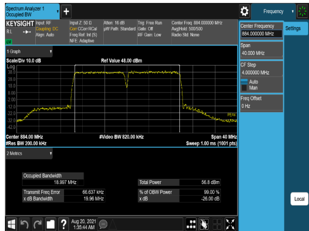
Plot 7-226. Occupied Bandwidth Plot (B5_10M(DSS)+10M_2C_256QAM - High Channel, Port 0)
