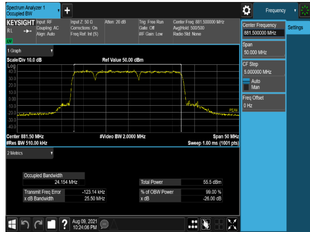
Plot 7-228. Occupied Bandwidth Plot (B5_10M(DSS)+10M+5M_3C_16QAM - Port 2)
