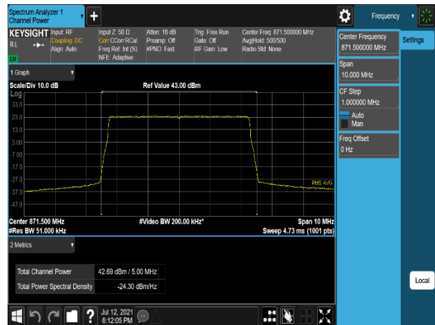
Plot 7-250. Conducted Average Output Power Plot (B5_5M_1C_256QAM - Low Channel, Port 3)
