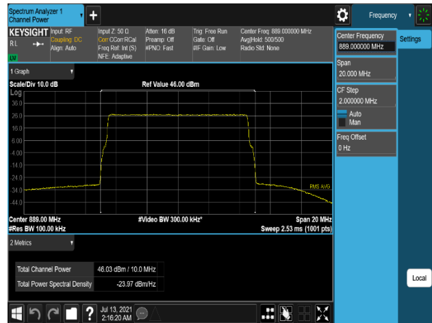
Plot 7-268. Conducted Average Output Power Plot (B5_10M_1C_QPSK – High Channel, Port 1)
