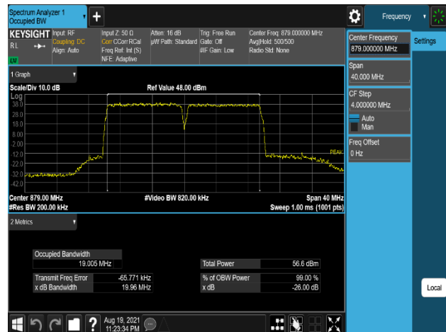
Plot 7-218. Occupied Bandwidth Plot (B5_10M(DSS)+10M_2C_256QAM - Low Channel, Port 0)
