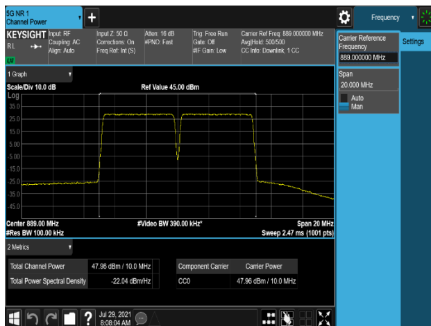
Plot 7-275. Conducted Average Output Power Plot (B5_5M+5M_2C_QPSK - High Channel, Port 0)
