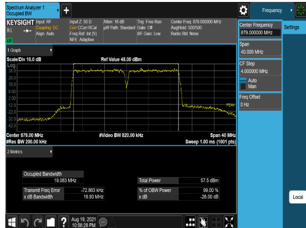
Plot 7-216. Occupied Bandwidth Plot (B5_10M(DSS)+10M_2C_16QAM - Low Channel, Port 0)
