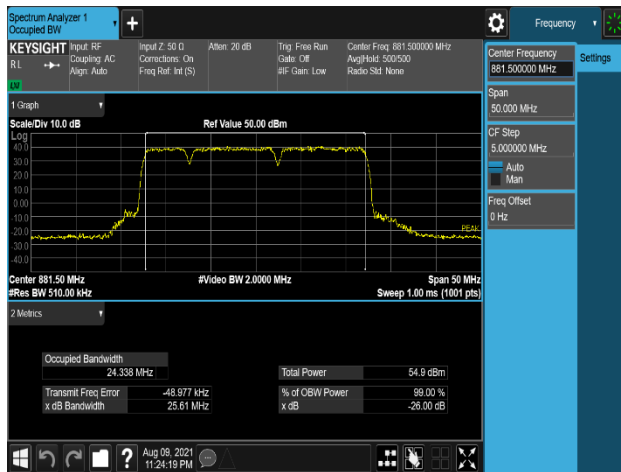
Plot 7-229. Occupied Bandwidth Plot (B5_10M(DSS)+10M+5M_3C_64QAM - Port 0)
