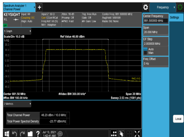
Plot 7-264. Conducted Average Output Power Plot (B5_10M_1C_64QAM - Mid Channel, Port 1)
