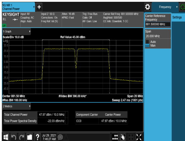
Plot 7-273. Conducted Average Output Power Plot (B5_5M+5M_2C_QPSK - Mid Channel, Port 0)
