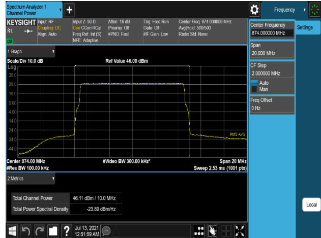
Plot 7-260. Conducted Average Output Power Plot (B5_10M_1C_256QAM - Low Channel, Port 1)
