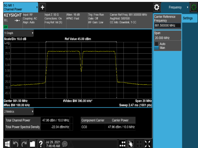
Plot 7-274. Conducted Average Output Power Plot (B5_5M+5M_2C_QPSK - Mid Channel, Port 1)
