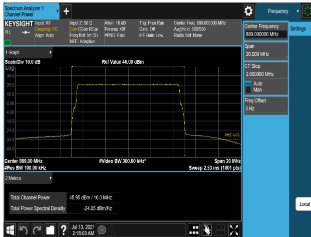
Plot 7-267. Conducted Average Output Power Plot (B5_10M_1C_QPSK – High Channel, Port 0)
