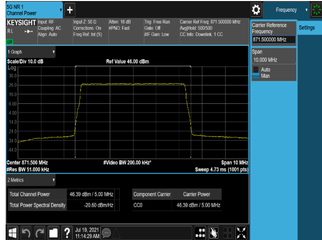
Plot 7-236. Conducted Average Output Power Plot (B5_5M_1C_QPSK - Low Channel, Port 1)
