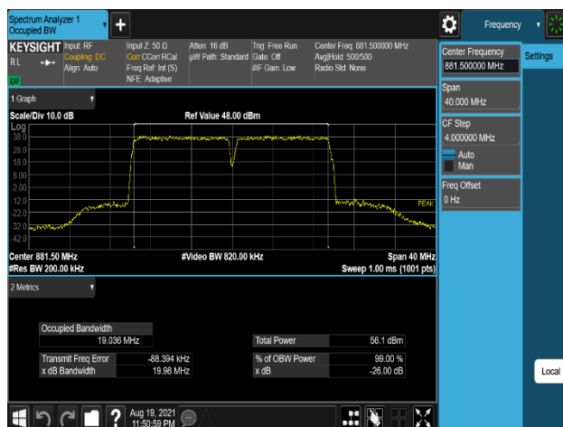
Plot 7-219. Occupied Bandwidth Plot (B5_10M(DSS)+10M_2C_QPSK - Mid Channel, Port 0)
