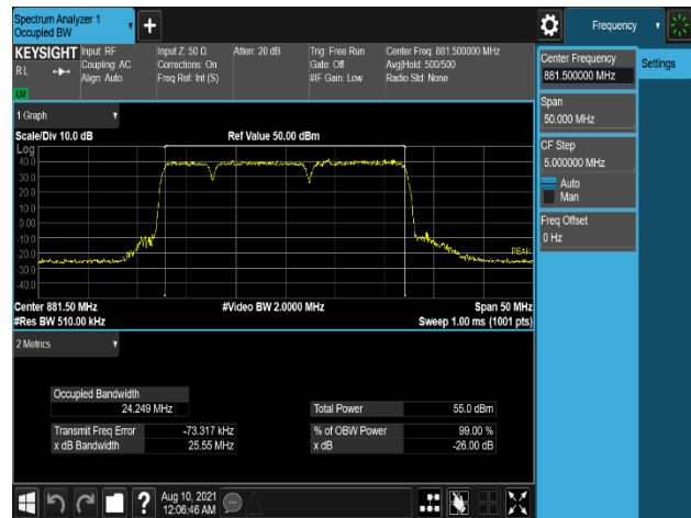
Plot 7-230. Occupied Bandwidth Plot (B5_10M(DSS)+10M+5M_3C_256QAM - Port 1)
