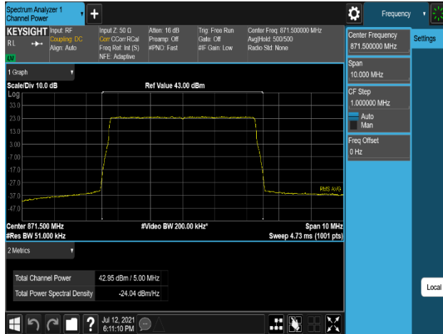
Plot 7-247. Conducted Average Output Power Plot (B5_5M_1C_256QAM - Low Channel, Port 0)
