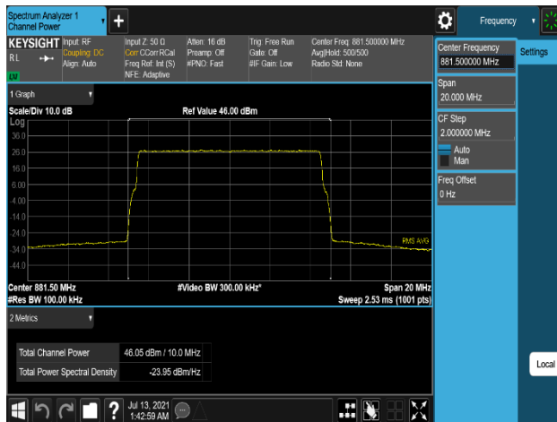
Plot 7-265. Conducted Average Output Power Plot (B5_10M_1C_64QAM – Mid Channel, Port 2)
