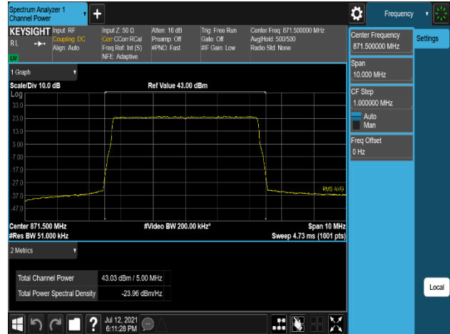
Plot 7-248. Conducted Average Output Power Plot (B5_5M_1C_256QAM - Low Channel, Port 1)
