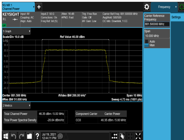
Plot 7-237. Conducted Average Output Power Plot (B5_5M_1C_256QAM - Mid Channel, Port 0)
