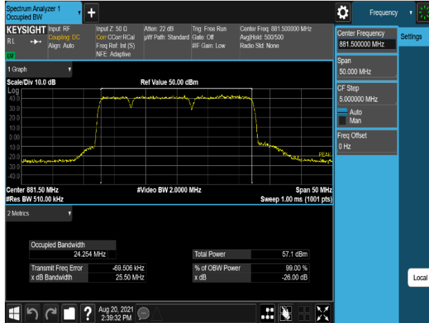
sPlot 7-231. Occupied Bandwidth Plot (B5_10M(DSS)+10M+5M_3C_QPSK - Port 1)
