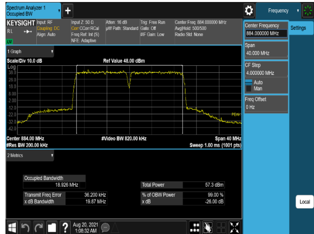
Plot 7-224. Occupied Bandwidth Plot (B5_10M(DSS)+10M_2C_16QAM - High Channel, Port 0)
