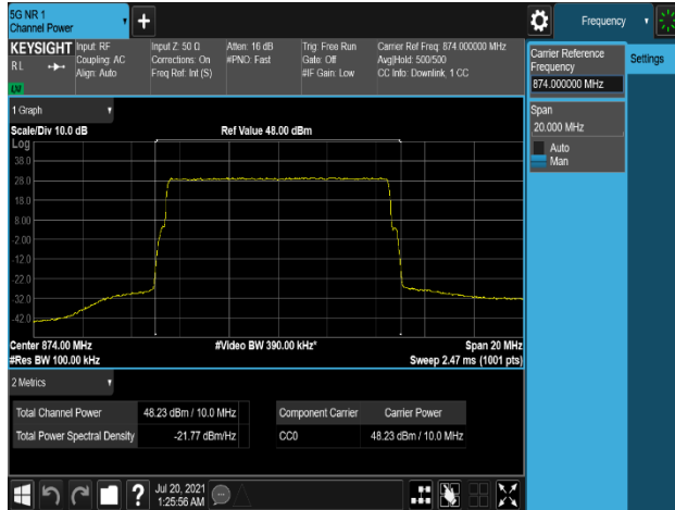
Plot 7-241. Conducted Average Output Power Plot (B5_10M_1C_256QAM - Low Channel, Port 0)
