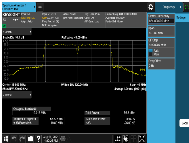
Plot 7-225. Occupied Bandwidth Plot (B5_10M(DSS)+10M_2C_64QAM - High Channel, Port 1)
