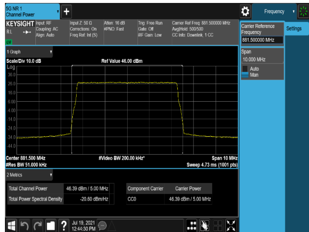
Plot 7-238. Conducted Average Output Power Plot (B5_5M_1C_256QAM - Mid Channel, Port 1)
