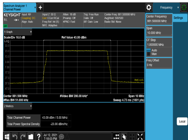
Plot 7-252. Conducted Average Output Power Plot (B5_5M_1C_256QAM - Mid Channel, Port 1)
