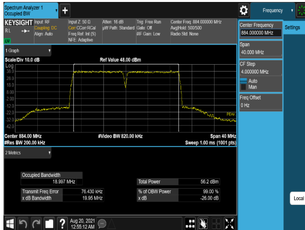
Plot 7-223. Occupied Bandwidth Plot (B5_10M(DSS)+10M_2C_QPSK - High Channel, Port 1)
