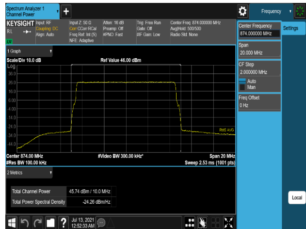
Plot 7-262. Conducted Average Output Power Plot (B5_10M_1C_256QAM - Low Channel, Port 3)
