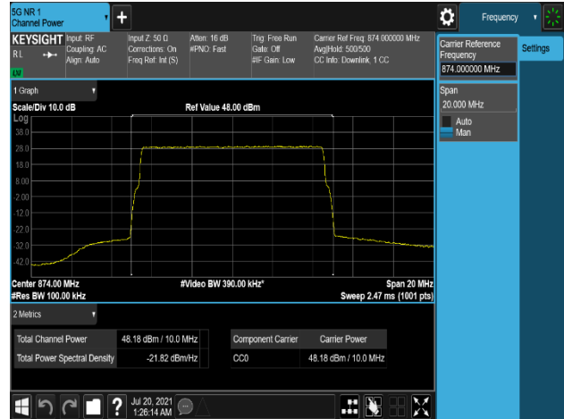
Plot 7-242. Conducted Average Output Power Plot (B5_10M_1C_256QAM - Low Channel, Port 1)
