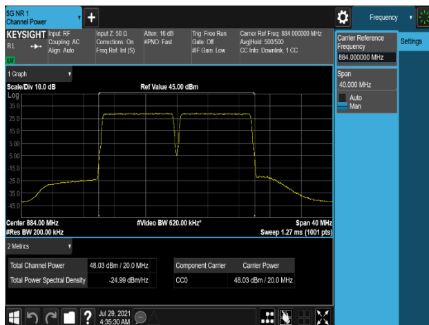
Plot 7-281. Conducted Average Output Power Plot (B5_10M+10M_2C_64QAM - High Channel, Port 0)
