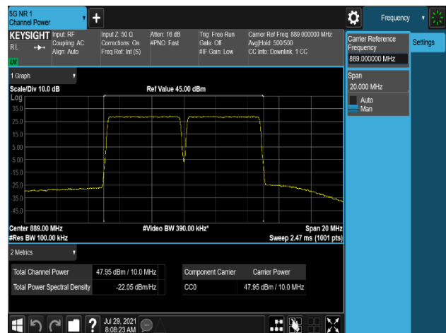
Plot 7-276. Conducted Average Output Power Plot (B5_5M+5M_2C_QPSK - High Channel, Port 1)
