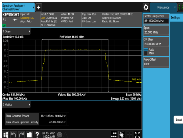
Plot 7-263. Conducted Average Output Power Plot (B5_10M_1C_64QAM - Mid Channel, Port 0)
