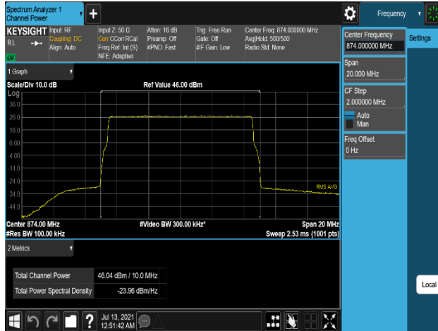
Plot 7-259. Conducted Average Output Power Plot (B5_10M_1C_256QAM - Low Channel, Port 0)
