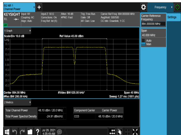
Plot 7-282. Conducted Average Output Power Plot (B5_10M+10M_2C_64QAM - High Channel, Port 1)
