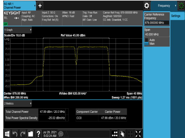
Plot 7-278. Conducted Average Output Power Plot (B5_10M+10M_2C_QPSK - Low Channel, Port 1)
