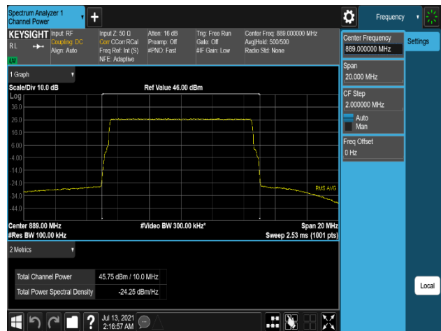
Plot 7-270. Conducted Average Output Power Plot (B5_10M_1C_QPSK – High Channel, Port 3)
