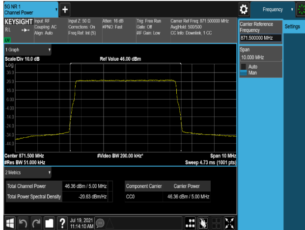
Plot 7-235. Conducted Average Output Power Plot (B5_5M_1C_QPSK - Low Channel, Port 0)
