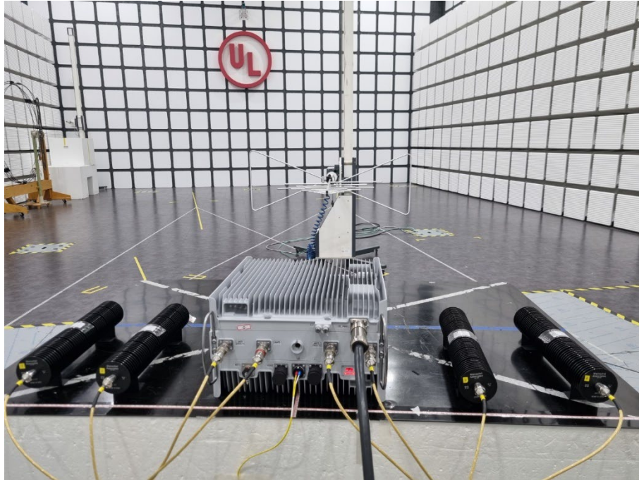
RSE TEST PHOTO (Below 1 GHz)
