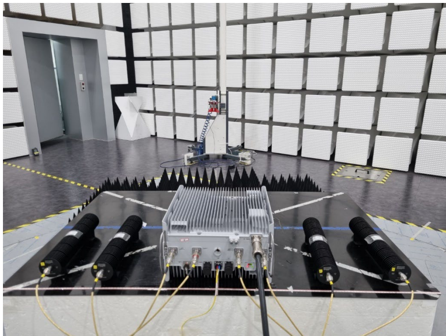
RSE TEST PHOTO (Above 1 GHz)
