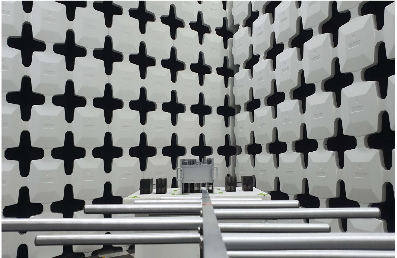
Below 1GHz Test Instrument & Measurement Setup
