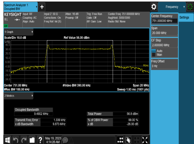
Plot 8-46. Occupied Bandwidth Plot (LTE B13_1C_10M+NB-IoT(2GB)_QPSK - Mid Channel_2T, Port 0)
