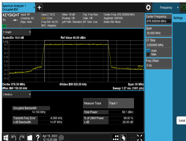
Plot 8-17. Occupied Bandwidth Plot (NR n5_1C_15M_QPSK - Low Channel_2T, Port 0)
