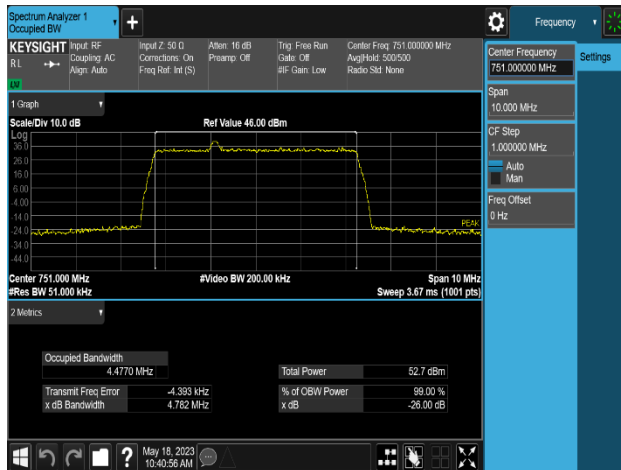
Plot 8-45. Occupied Bandwidth Plot (LTE B13_1C_5M+NB-IoT(1B)_QPSK - Mid Channel_2T, Port 0)
