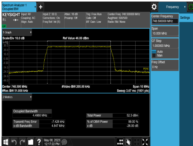
Plot 8-39. Occupied Bandwidth Plot (LTE B13_1C_5M_QPSK - Low Channel_2T, Port 1)
