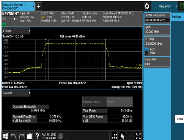
Plot 8-49. Occupied Bandwidth Plot (LTE B5_1C_10M_QPSK - Low Channel_4T, Port 2)
