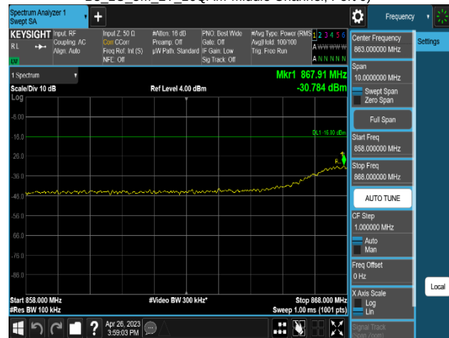
Plot 8-558. Conducted Spurious Emission Plot 858 MHz to 868 MHz (MSR 3C_DSS B(n)5_1C_10M+NR n5_1C_5M+LTE B5_1C_5M_2T_16QAM-Middle Channel, Port 0)
