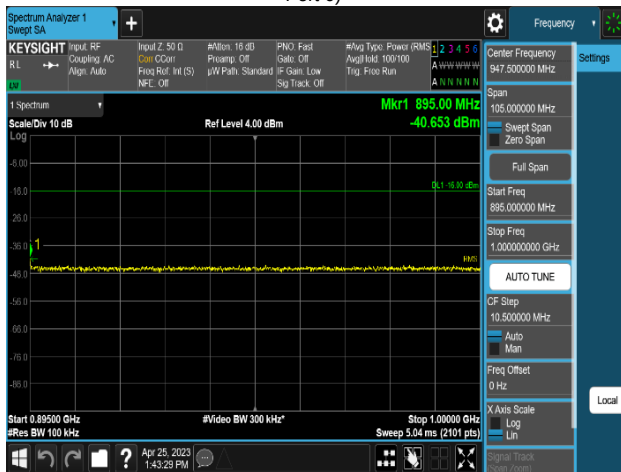
Plot 8-523. Conducted Spurious Emission Plot 895 MHz to 1 GHz
