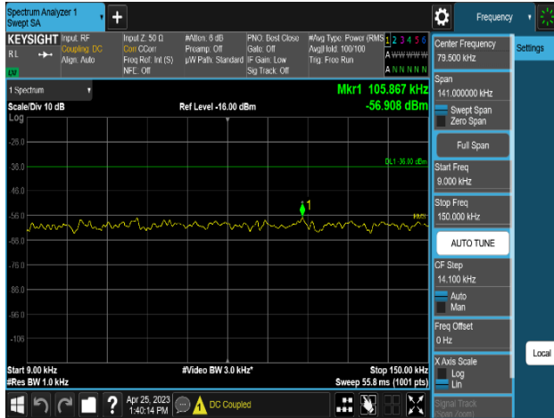
Plot 8-519. Conducted Spurious Emission Plot 9 kHz to 150 kHz
