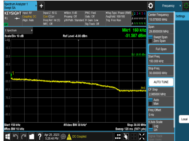
Plot 8-544. Conducted Spurious Emission Plot 150 kHz to 30 MHz (MSR 2C_DSS B(n)5_1C_10M+NR n5_1C_15M_2T_16QAM-Low Channel, Port 0)
