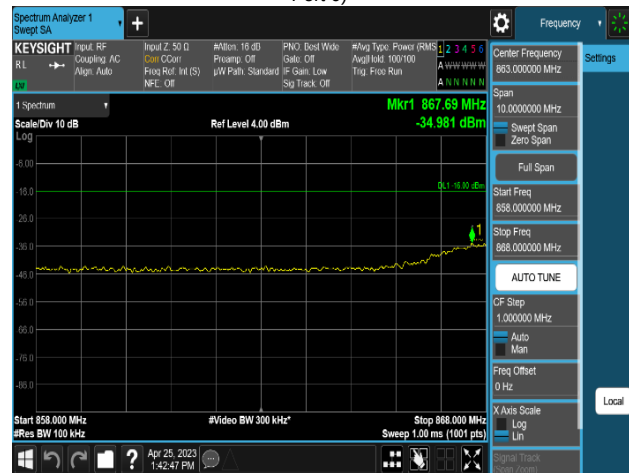
Plot 8-522. Conducted Spurious Emission Plot 858 MHz to 868 MHz
