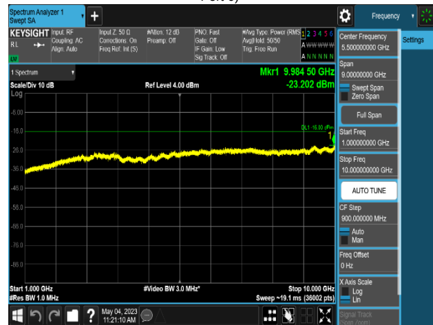
Plot 8-524. Conducted Spurious Emission Plot 1 GHz to 10 GHz
