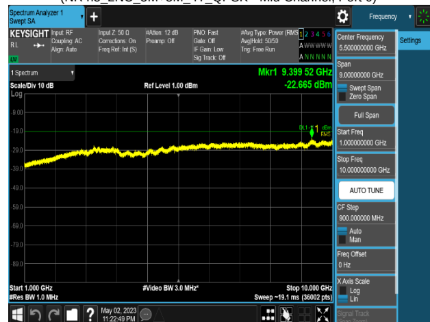
Plot 8-693. Conducted Spurious Emission Plot 1 GHz to 10 GHz (NR n5_2NC_5M+5M_4T_QPSK - Mid Channel, Port 0)
