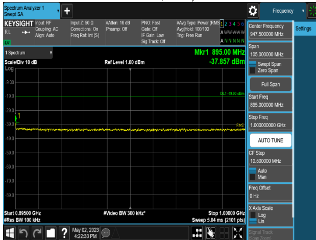
Plot 8-740. Conducted Spurious Emission Plot 895 MHz to 1 GHz (MSR 2C_DSS B(n)5_1C_10M+NR n5_1C_15M_4T_16QAM - Middle Channel, Port 0)
