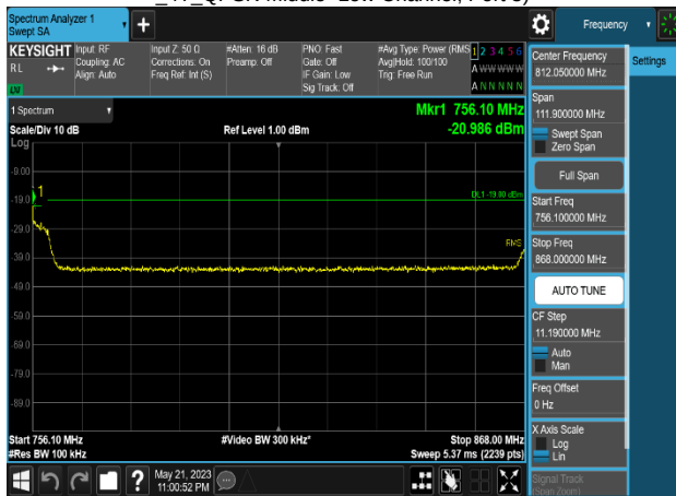
Plot 8-800. Conducted Spurious Emission Plot 756.1 MHz to 868 MHz (Multi-Band_LTE B13_1C_10M+NB-IoT(2GB)+LTE B5_1C_10M _4T_QPSK-Middle+Low Channel, Port 3)
