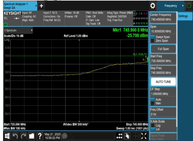
Plot 8-799. Conducted Spurious Emission Plot 735 MHz to 745.9 MHz (Multi-Band_LTE B13_1C_10M+NB-IoT(2GB)+LTE B5_1C_10M _4T_QPSK-Middle+Low Channel, Port 3)
