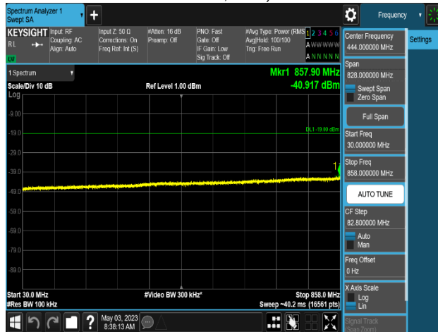
Plot 8-744. Conducted Spurious Emission Plot 30 MHz to 858 MHz (MSR 2NC_DSS B(n)5_1C_10M+NR n5_1C_5M_4T_QPSK - Middle Channel, Port 0)
