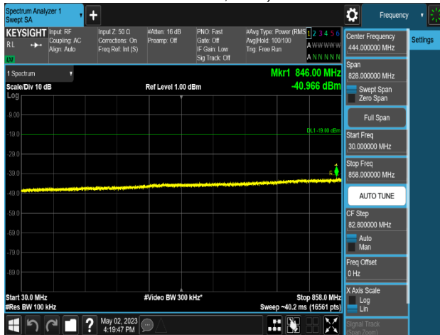
Plot 8-738. Conducted Spurious Emission Plot 30 MHz to 858 MHz (MSR 2C_DSS B(n)5_1C_10M+NR n5_1C_15M_4T_16QAM - Middle Channel, Port 0)
