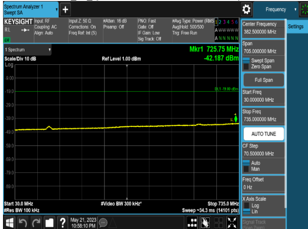
Plot 8-798. Conducted Spurious Emission Plot 30 MHz to 735 MHz (Multi-Band_LTE B13_1C_10M+NB-IoT(2GB)+LTE B5_1C_10M _4T_QPSK-Middle+Low Channel, Port 3)
