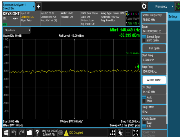
Plot 8-784. Conducted Spurious Emission Plot 9 kHz to 150 kHz
