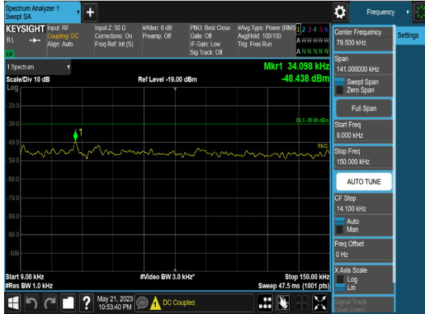
Plot 8-796. Conducted Spurious Emission Plot 9 kHz to 150 kHz (Multi-Band_LTE B13_1C_10M+NB-IoT(2GB)+LTE B5_1C_10M _4T_QPSK-Middle+Low Channel, Port 3)
