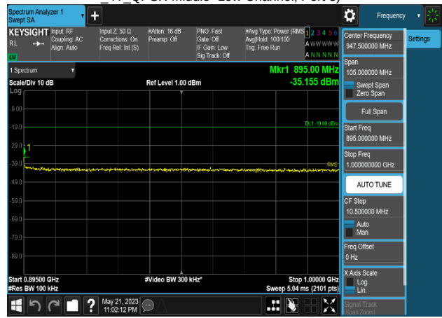
Plot 8-801. Conducted Spurious Emission Plot 895 MHz to 1 GHz (Multi-Band_LTE B13_1C_10M+NB-IoT(2GB)+LTE B5_1C_10M _4T_QPSK-Middle+Low Channel, Port 3)
