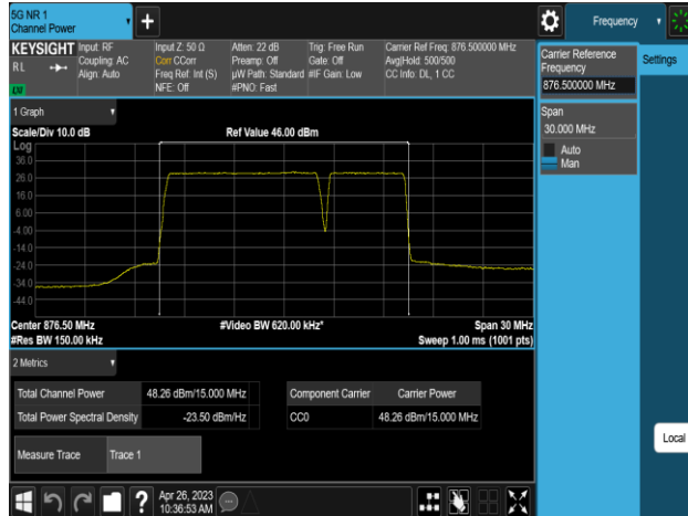
Plot 8-123. Conducted Average Output Power Plot (MSR 2C_DSS B(n)5_1C_10M+NR n5_1C_5M_2T_QPSK - Low Channel, Port 1)
