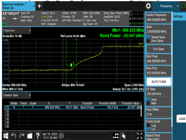
Plot 8-311. Band Edge Emission Summary Data Plot (NR n5_1C_10M_16QAM - Low Channel_2T, Port 1)
