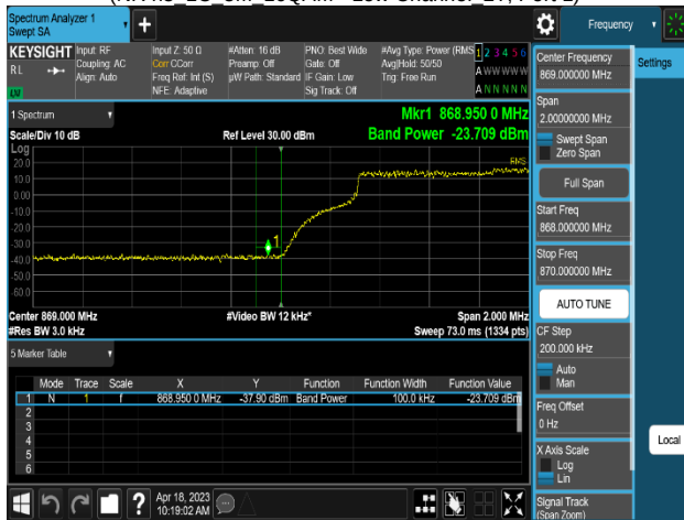
Plot 8-309. Band Edge Emission Summary Data Plot (NR n5_1C_5M_16QAM - Low Channel_2T, Port 1)
