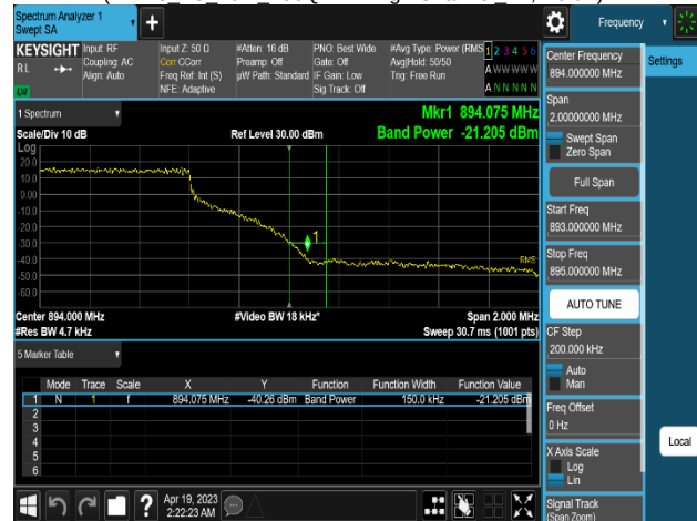
Plot 8-312. Band Edge Emission Summary Data Plot (NR n5_1C_10M_256QAM - High Channel_2T, Port 1)
