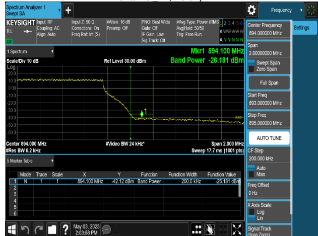
Plot 8-408. Band Edge Emission Summary Data Plot (MSR 3NC_DSS B(n)5_1C_10M+NR n5_1C_5M+LTE B5_1C_5M_QPSK - High Channel 4T, Port 2)
