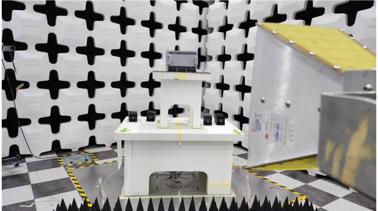
Above 1GHz Test Instrument & Measurement Setup > 1GHz
