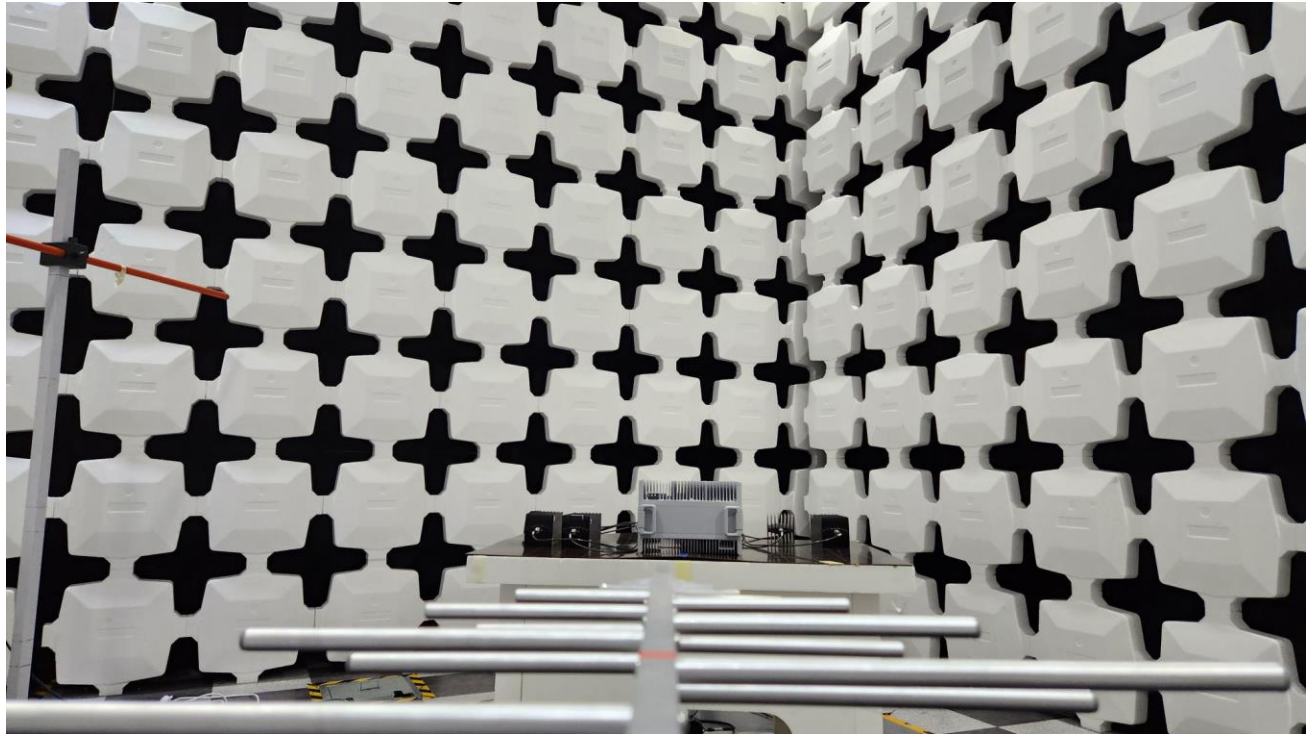
Below 1GHz Test Instrument & Measurement Setup
