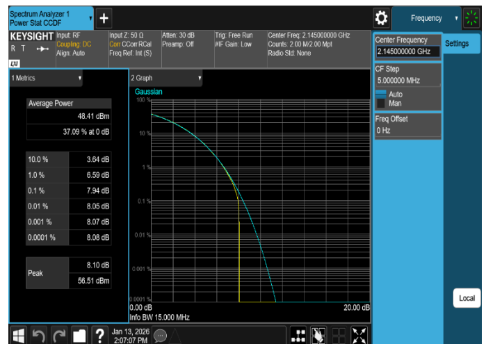
Plot 8-19. Peak To Average Power Ratio Plot (MSR_B/n66_2C_DSS_10M+LTE_5M_QPSK - Mid Channel, Port 2)
