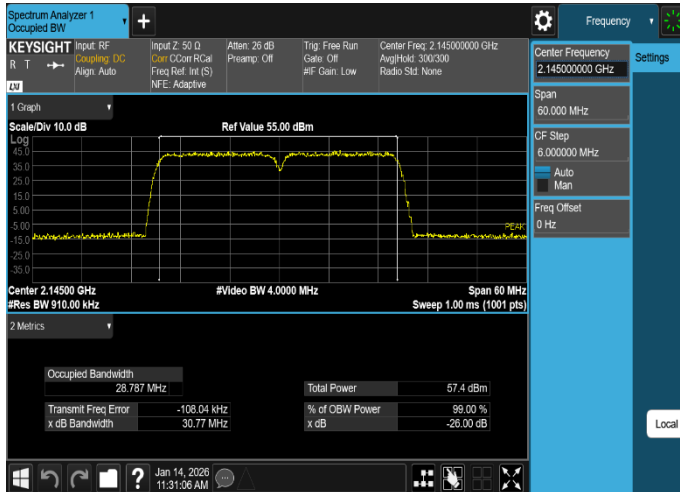
Plot 8-9. Occupied Bandwidth Plot (MSR_B/n66_2C_DSS_15M+LTE_15M_QPSK - Mid Channel, Port 0)
