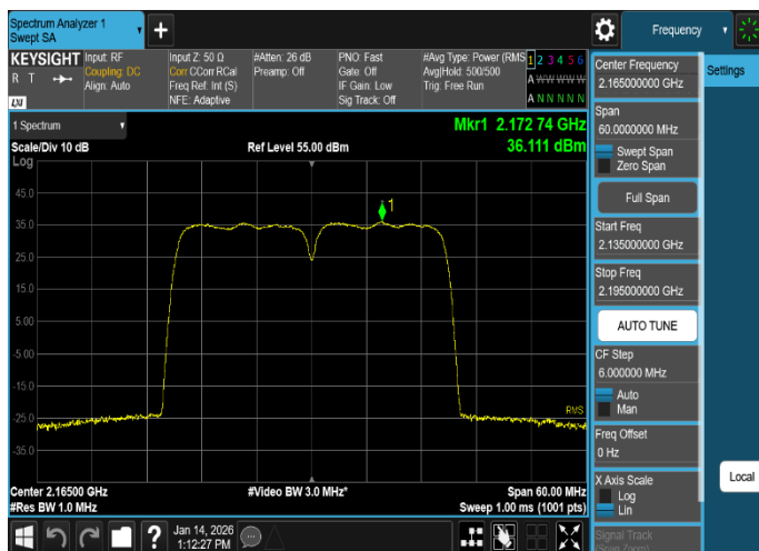
Plot 8-15. Equivalent Isotropically Radiated Power Plot (MSR_B/n66_2C_DSS_15M+LTE_15M_16QAM - High Channel, Port 3)
