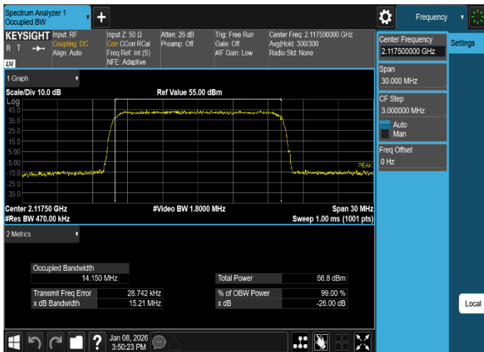
Plot 8-3. Occupied Bandwidth Plot (DSS_B/n66_1C_15M_QPSK - Low Channel, Port 1)
