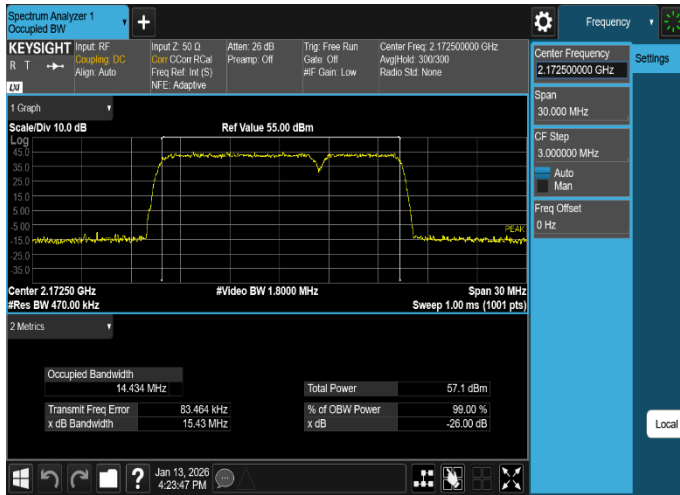
Plot 8-7. Occupied Bandwidth Plot (MSR_B/n66_2C_DSS_10M+LTE_5M_QPSK - High Channel, Port 0)
