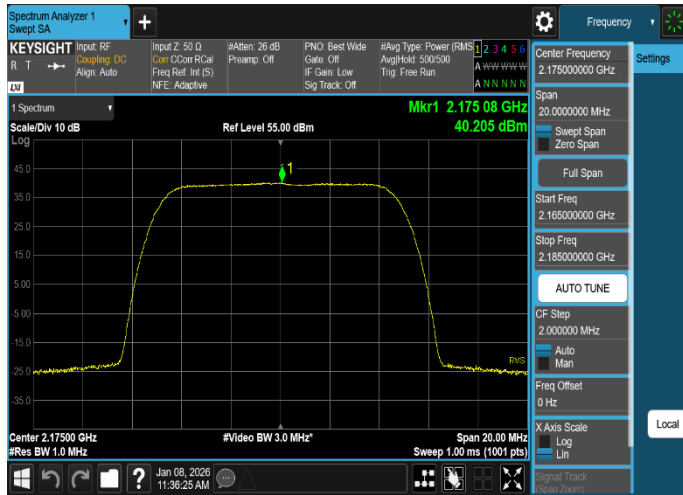
Plot 8-11. Equivalent Isotropically Radiated Power Plot (DSS_B/n66_1C_10M_16QAM - High Channel, Port 3)
