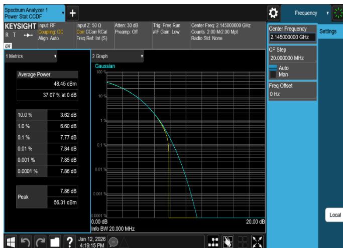
Plot 8-18. Peak To Average Power Ratio Plot (DSS_B/n66_1C_20M_QPSK - Mid Channel, Port 3)
