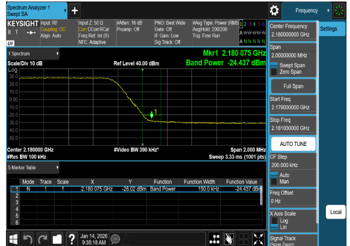
Plot 8-29. Band Edge Emission Summary Data Plot (MSR_B/n66_2NC_DSS_10M+LTE_5M_QPSK - High Edge, Port 3)
