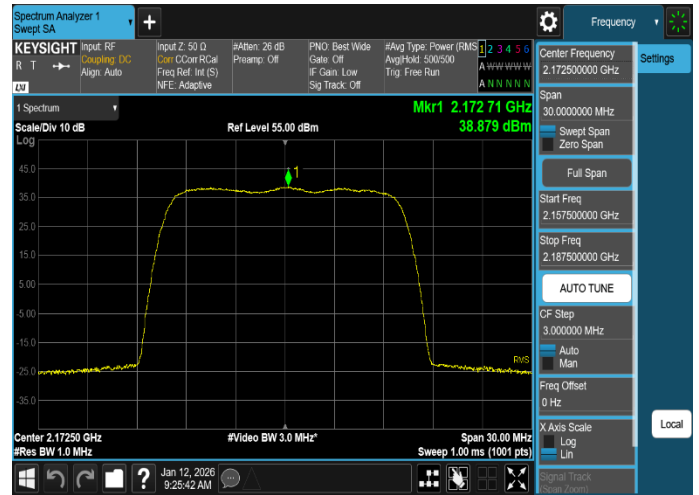
Plot 8-12. Equivalent Isotropically Radiated Power Plot (DSS_B/n66_1C_15M_16QAM - High Channel, Port 0)
