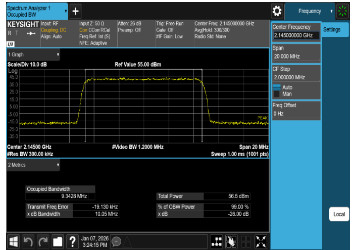
Plot 8-2. Occupied Bandwidth Plot (DSS_B/n66_1C_10M_64QAM - Mid Channel, Port 1)
