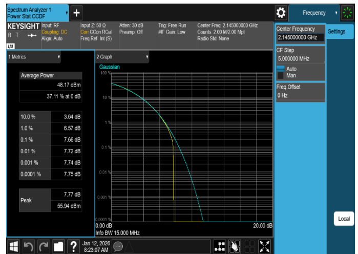
Plot 8-17. Peak To Average Power Ratio Plot (DSS_B/n66_1C_15M_256QAM - Mid Channel, Port 1)
