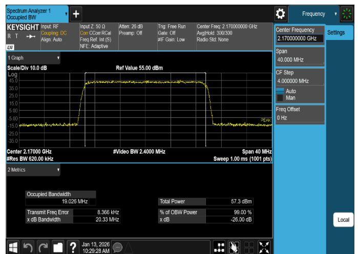
Plot 8-6. Occupied Bandwidth Plot (DSS_B/n66_1C_20M_64QAM - High Channel, Port 0)
