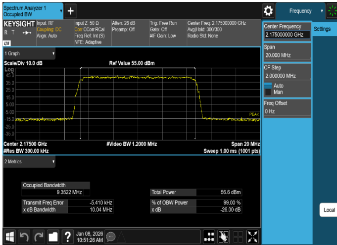
Plot 8-1. Occupied Bandwidth Plot (DSS_B/n66_1C_10M_QPSK - High Channel, Port 0)
