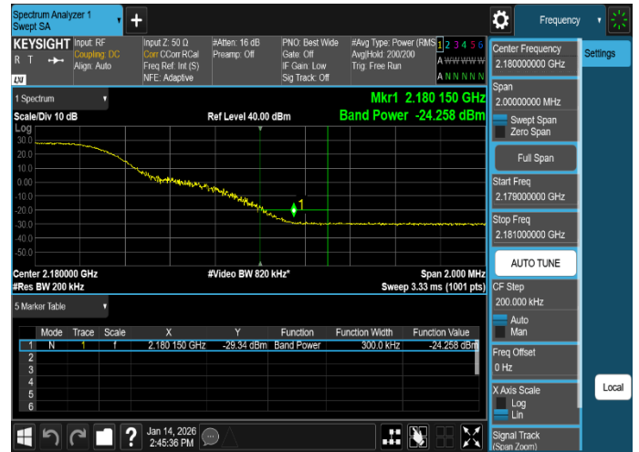
Plot 8-27. Band Edge Emission Summary Data Plot (MSR_B/n66_2C_DSS_15M+LTE_15M_QPSK - High Edge, Port 3)
