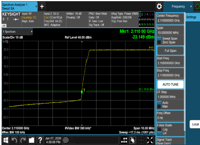
Plot 8-20. Band Edge Emission Summary Data Plot (DSS_B/n66_1C_10M_QPSK - Low Edge, Port 3)
