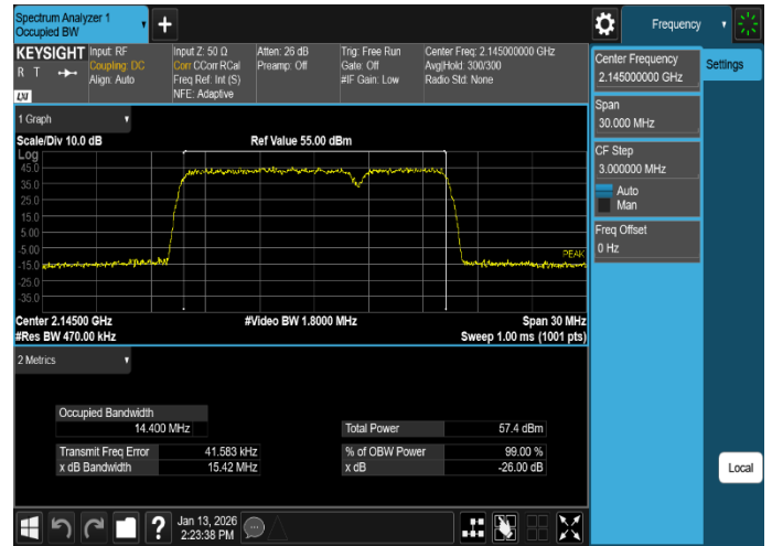
Plot 8-8. Occupied Bandwidth Plot (MSR_B/n66_2C_DSS_10M+LTE_5M_16QAM - Mid Channel, Port 1)
