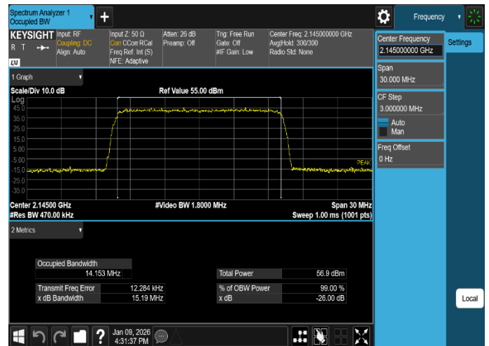
Plot 8-4. Occupied Bandwidth Plot (DSS_B/n66_1C_15M_64QAM - Mid Channel, Port 2)
