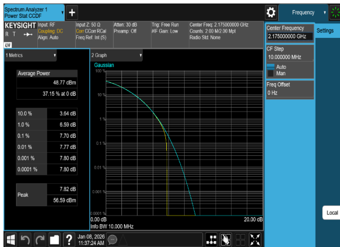
Plot 8-16. Peak To Average Power Ratio Plot (DSS_B/n66_1C_10M_16QAM - High Channel, Port 3)
