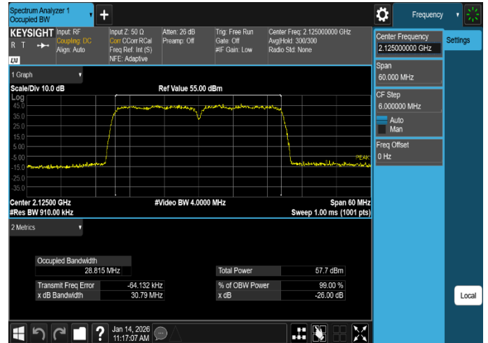
Plot 8-10. Occupied Bandwidth Plot (MSR_B/n66_2C_DSS_15M+LTE_15M_16QAM - Low Channel, Port 0)
