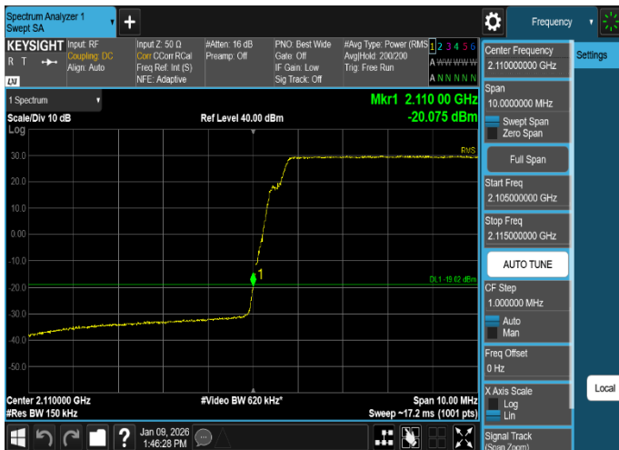
Plot 8-22. Band Edge Emission Summary Data Plot (DSS_B/n66_1C_15M_64QAM - Low Edge, Port 3)
