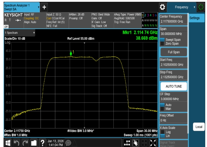
Plot 8-14. Equivalent Isotropically Radiated Power Plot (MSR_B/n66_2C_DSS_10M+LTE_5M_16QAM - Low Channel, Port 3)
