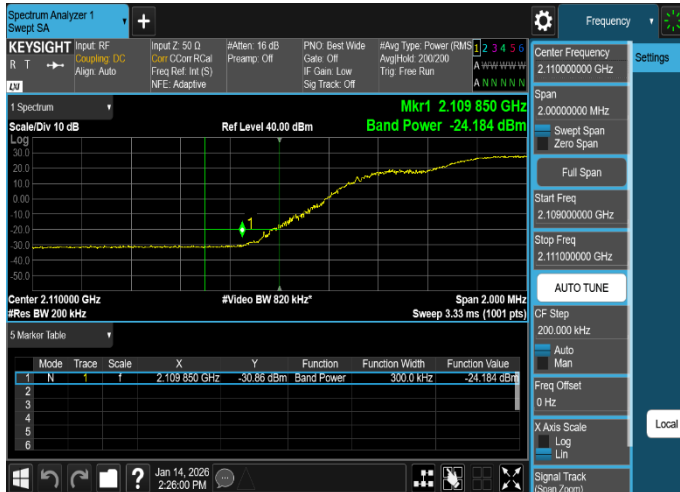
Plot 8-28. Band Edge Emission Summary Data Plot (MSR_B/n66_2NC_DSS_15M+LTE_15M_QPSK - Low Edge, Port 3)
