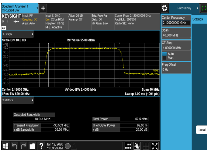
Plot 8-5. Occupied Bandwidth Plot (DSS_B/n66_1C_20M_QPSK - Low Channel, Port 3)
