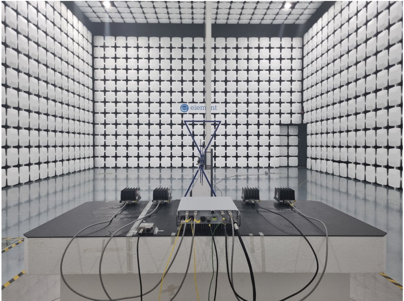
Below 1GHz radiated Test Instrument & Measurement Setup
