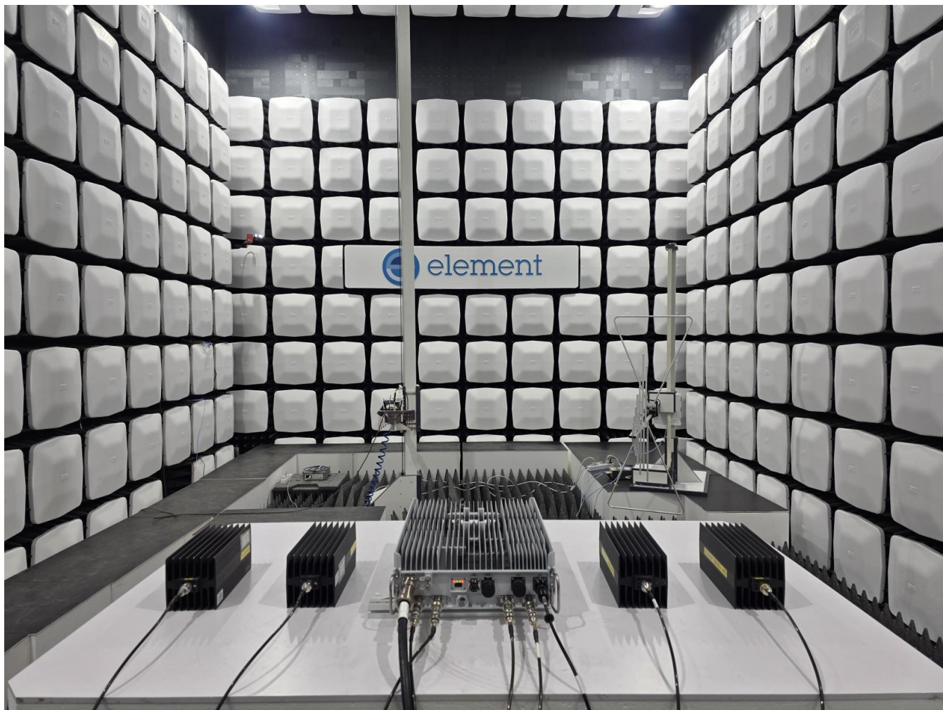
Above 1GHz radiated Test Instrument & Measurement Setup
