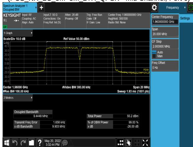
Plot 8-15. Occupied Bandwidth Plot (PCS_NR_1C_5M+LTE_1C_5M_2TX_QPSK - Mid Channel, Port 0)
