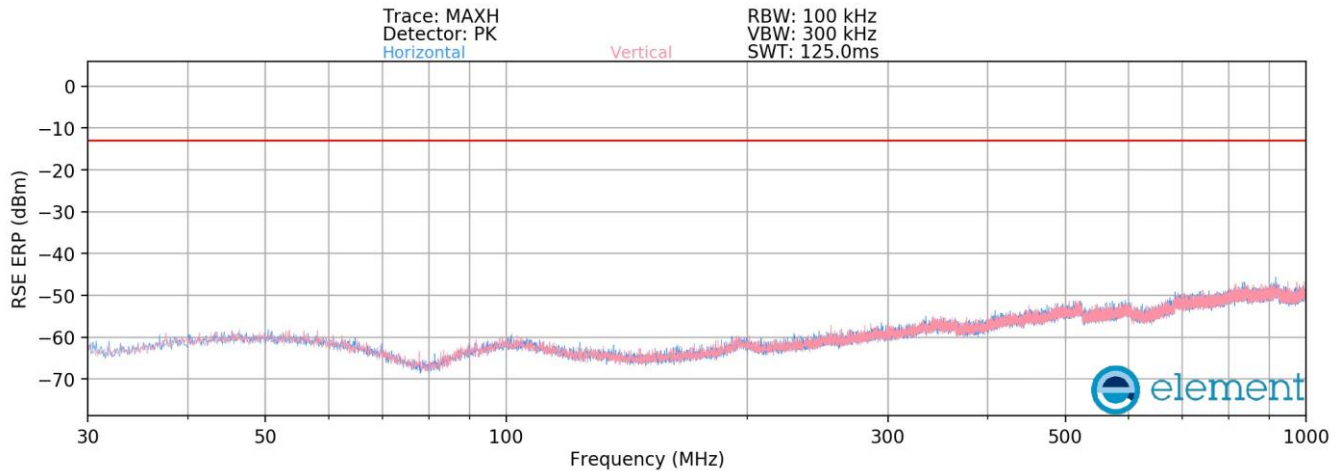
Plot 8-473. Radiated spurious emission 30 MHz to 1000 MHz (AWS_NR_1C_5M_Mid Channel_2TX)
