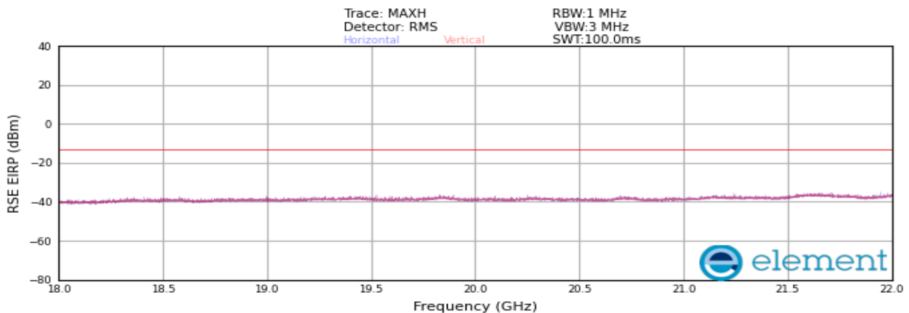
Plot 8-475. Radiated spurious emission Plot_18 GHz to 22 GHz (AWS_NR_1C_5M_Mid Channel_2TX)
