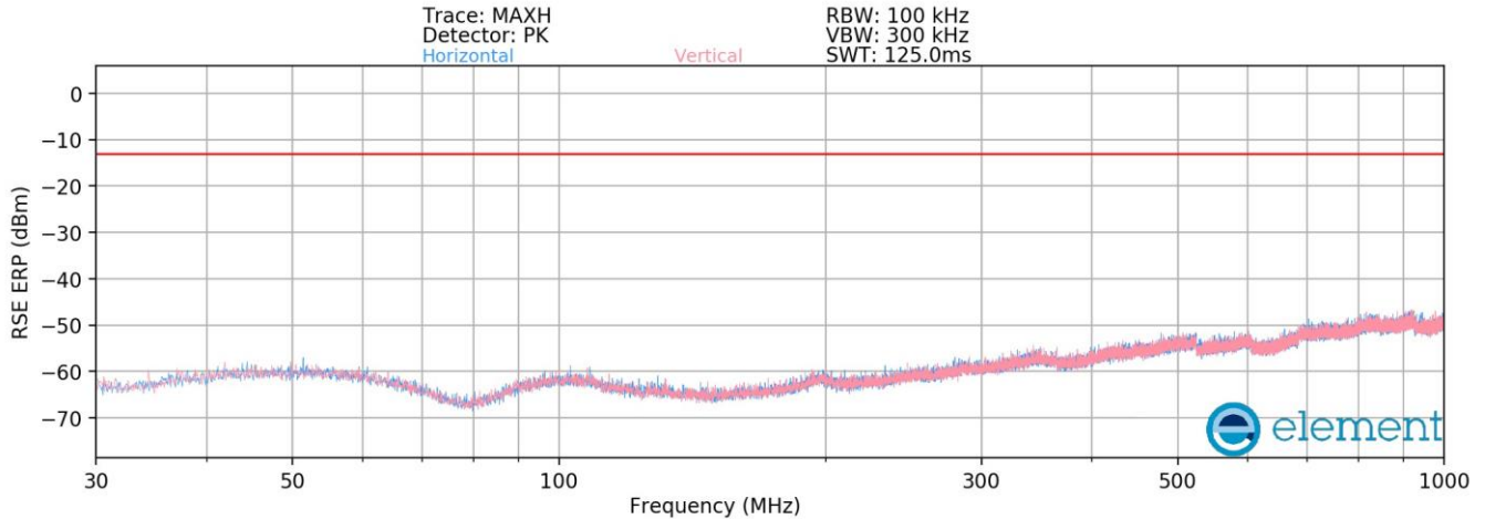
Plot 8-482. Radiated spurious emission 30 MHz to 1000 MHz (AWS_DSS_1C_20M + NR_1C_10M + LTE_1C_5M_Mid Channel_4TX_Non-Contiguous)
