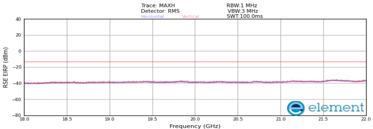
Plot 8-469. Radiated spurious emission Plot_18 GHz to 22 GHz (PCS_DSS_1C_20M + NR_1C_5M_Mid Channel_4TX)
