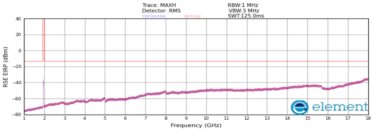
Plot 8-468. Radiated spurious emission Plot_1 GHz to 18 GHz (PCS_DSS_1C_20M + NR_1C_5M_Mid Channel_4TX)
