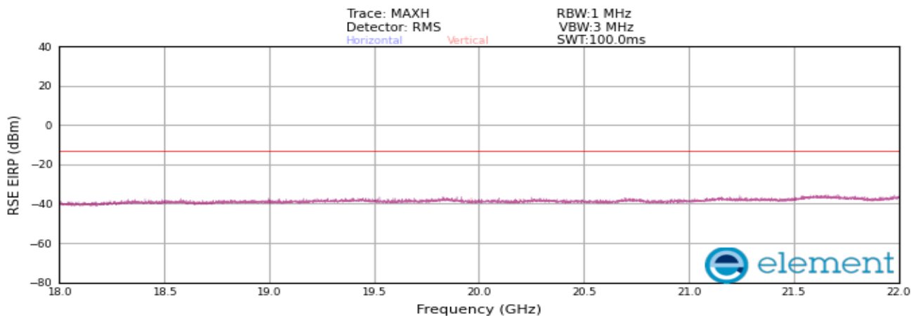
Plot 8-478. Radiated spurious emission Plot_18 GHz to 22 GHz (AWS_NR_1C_5M_Mid Channel_4TX)
