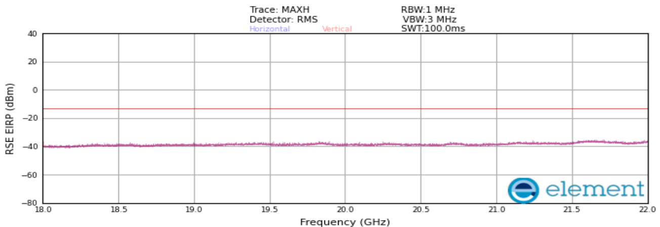
Plot 8-484. Radiated spurious emission Plot_18 GHz to 22 GHz (AWS_DSS_1C_20M + NR_1C_10M + LTE_1C_5M_Mid Channel_4TX_Non-Contiguous)
