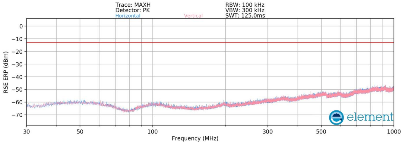
Plot 8-470. Radiated spurious emission 30 MHz to 1000 MHz (PCS_DSS_1C_20M + NR_1C_5M_Mid Channel_4TX_Non-Contiguous)
