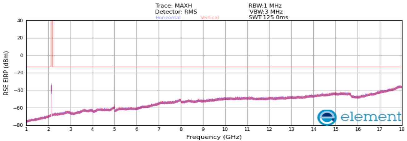
Plot 8-480. Radiated spurious emission Plot_1 GHz to 18 GHz (AWS_DSS_1C_20M + NR_1C_10M + LTE_1C_5M_Mid Channel_4TX)
