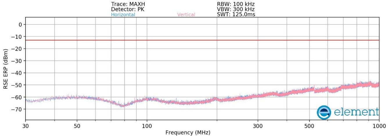
Plot 8-479. Radiated spurious emission 30 MHz to 1000 MHz (AWS_DSS_1C_20M + NR_1C_10M + LTE_1C_5M_Mid Channel_4TX)
