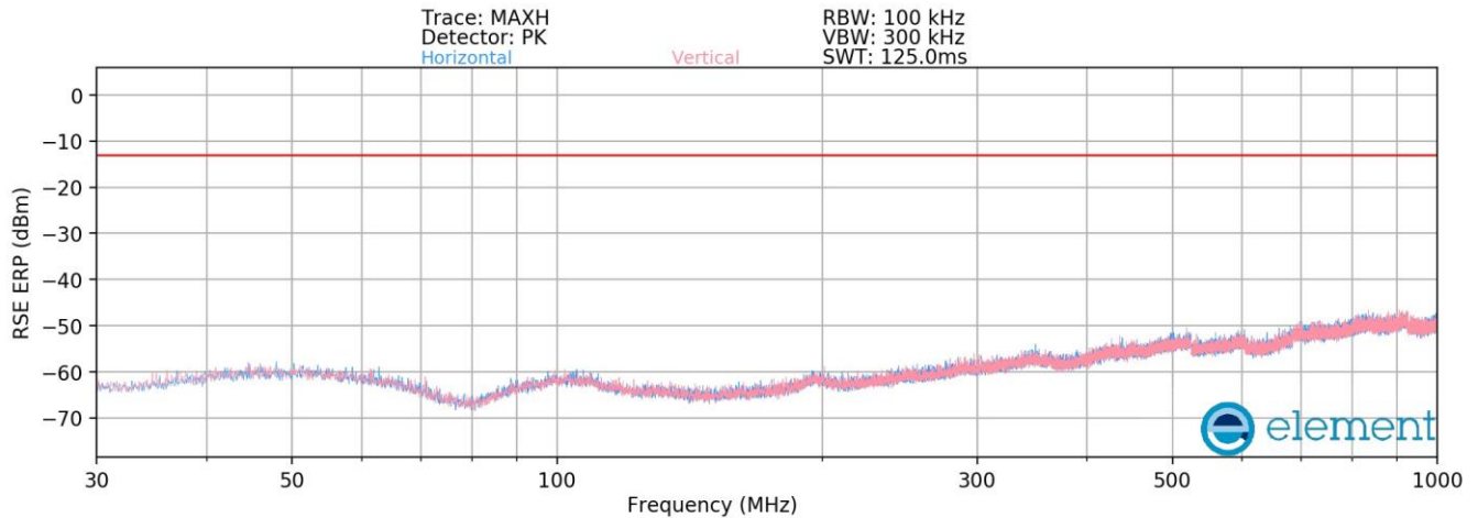
Plot 8-464. Radiated spurious emission 30 MHz to 1000 MHz (PCS_NR_1C_5M_Mid Channel_4TX)
