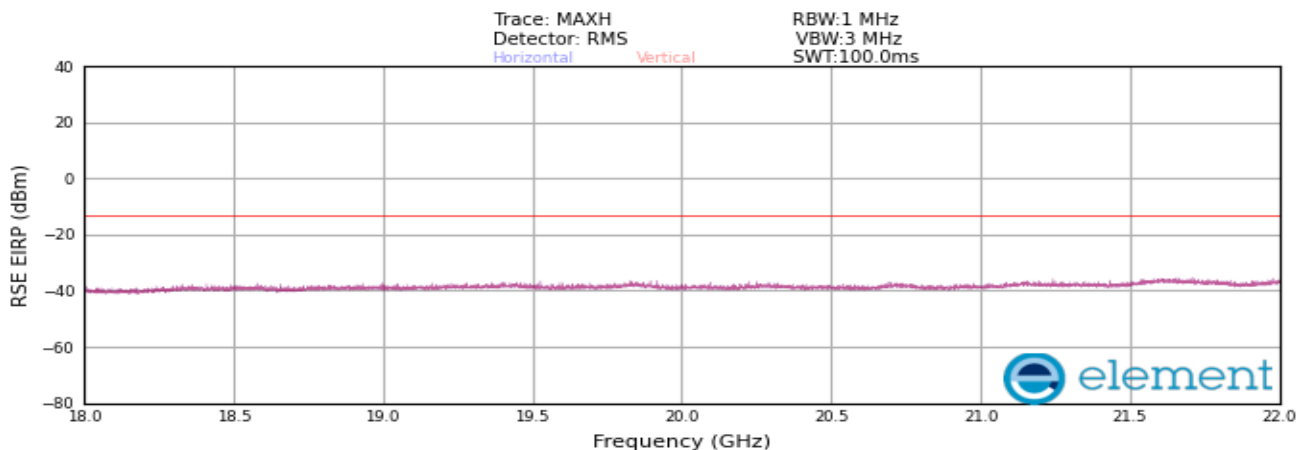
Plot 8-463. Radiated spurious emission_18 GHz to 22 GHz (PCS_NR_1C_5M_Mid Channel_2TX)
