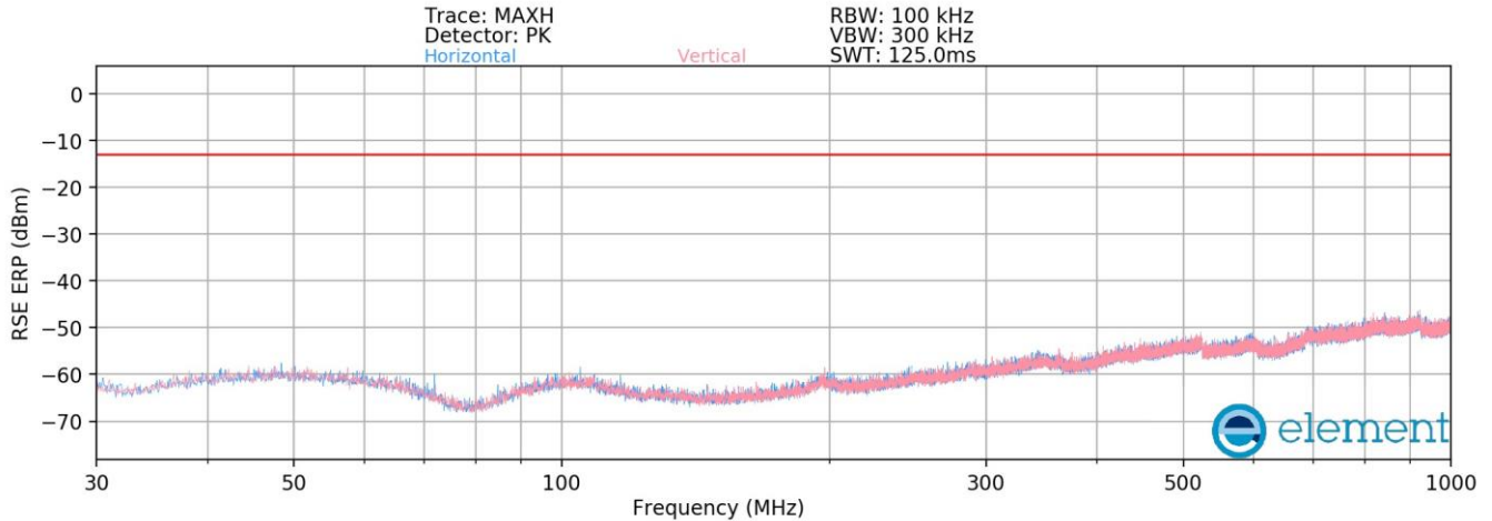
Plot 8-467. Radiated spurious emission 30 MHz to 1000 MHz (PCS_DSS_1C_20M + NR_1C_5M_Mid Channel_4TX)
