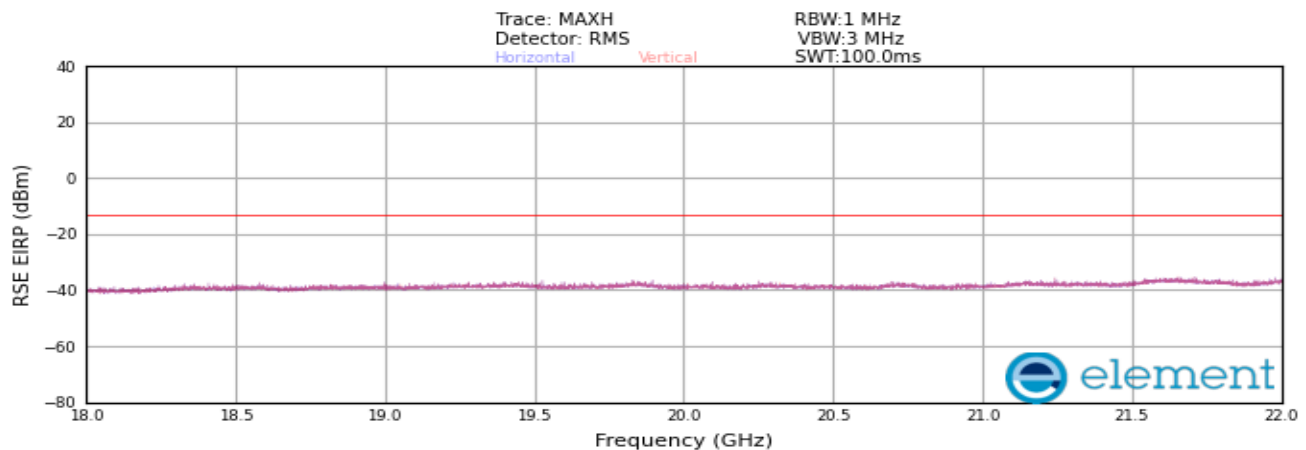
Plot 8-472. Radiated spurious emission Plot_18 GHz to 22 GHz (PCS_DSS_1C_20M + NR_1C_5M_Mid Channel_4TX_Non-Contiguous)
