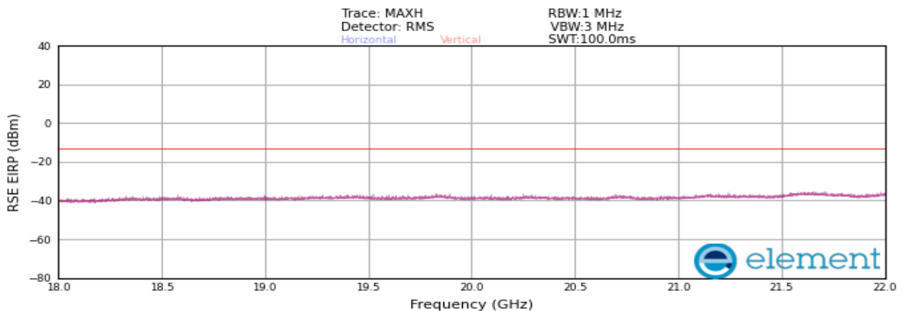
Plot 8-481. Radiated spurious emission Plot_18 GHz to 22 GHz (AWS_DSS_1C_20M + NR_1C_10M + LTE_1C_5M_Mid Channel_4TX)
