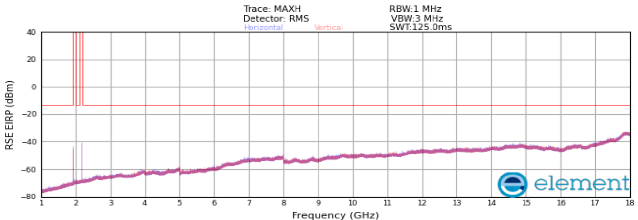
Plot 8-486. Radiated spurious emission Plot_1 GHz to 18 GHz (PCS_NR_1C_5M_Low Channel + AWS_1C_5M_High Channel_Simultaneous Operation)
