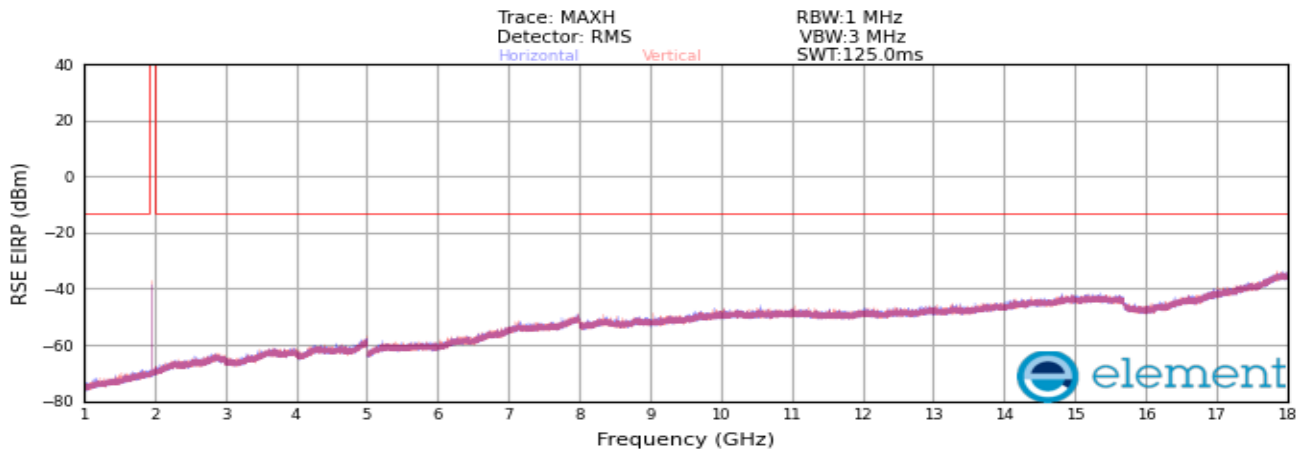
Plot 8-462. Radiated spurious emission_1 GHz to 18 GHz (PCS_NR_1C_5M_Mid Channel_2TX)
