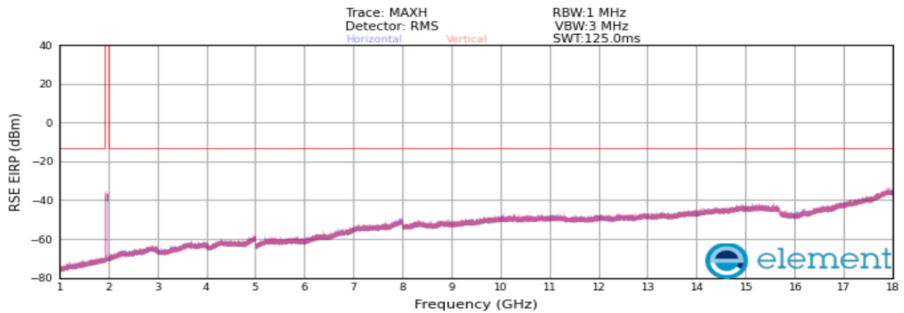
Plot 8-471. Radiated spurious emission Plot_1 GHz to 18 GHz (PCS_DSS_1C_20M + NR_1C_5M_Mid Channel_4TX_Non-Contiguous)
