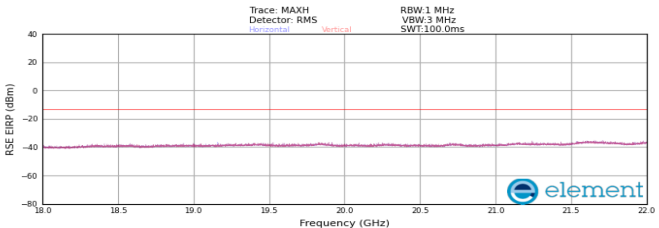
Plot 8-487. Radiated spurious emission Plot_18 GHz to 22 GHz (PCS_NR_1C_5M_Low Channel + AWS_1C_5M_High Channel_Simultaneous Operation)
