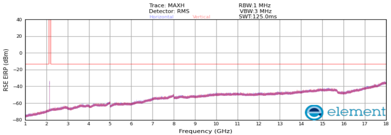
Plot 8-477. Radiated spurious emission Plot_1 GHz to 18 GHz (AWS_NR_1C_5M_Mid Channel_4TX)
