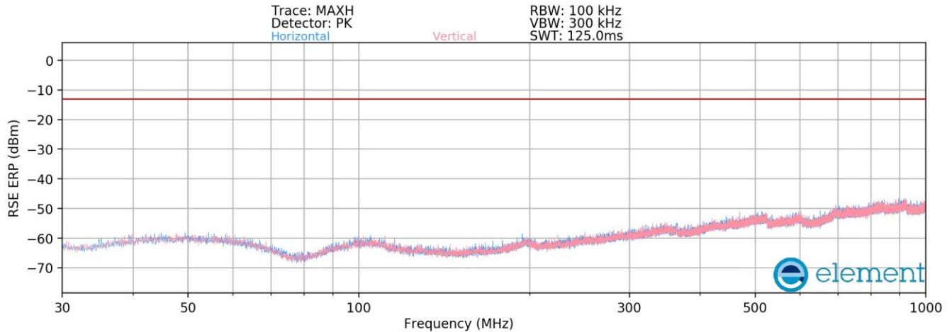
Plot 8-461. Radiated spurious emission_30 MHz to 1000 MHz (PCS_NR_1C_5M_Mid Channel_2TX)
