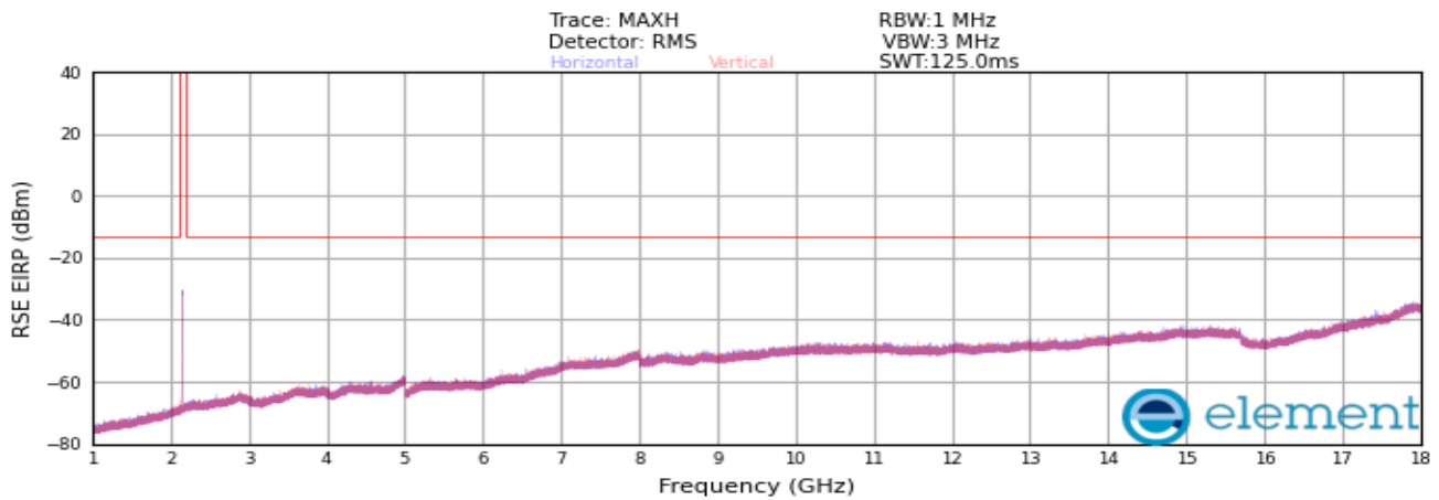
Plot 8-474. Radiated spurious emission Plot_1 GHz to 18 GHz (AWS_NR_1C_5M_Mid Channel_2TX)
