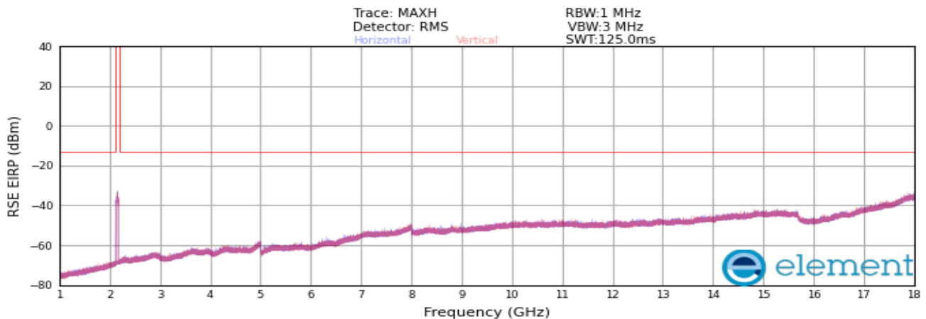
Plot 8-483. Radiated spurious emission Plot_1 GHz to 18 GHz (AWS_DSS_1C_20M + NR_1C_10M + LTE_1C_5M_Mid Channel_4TX_Non-Contiguous)
