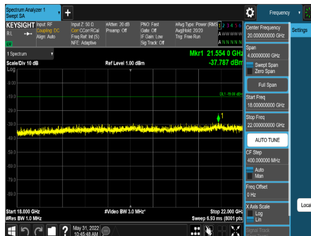
Plot 8-460. Conducted Spurious Emission Plot 18 GHz to 22 GHz (AWS_DSS_2C_10M+10M_2TX_Non-Cont_QPSK - Mid Channel, Port 0)
