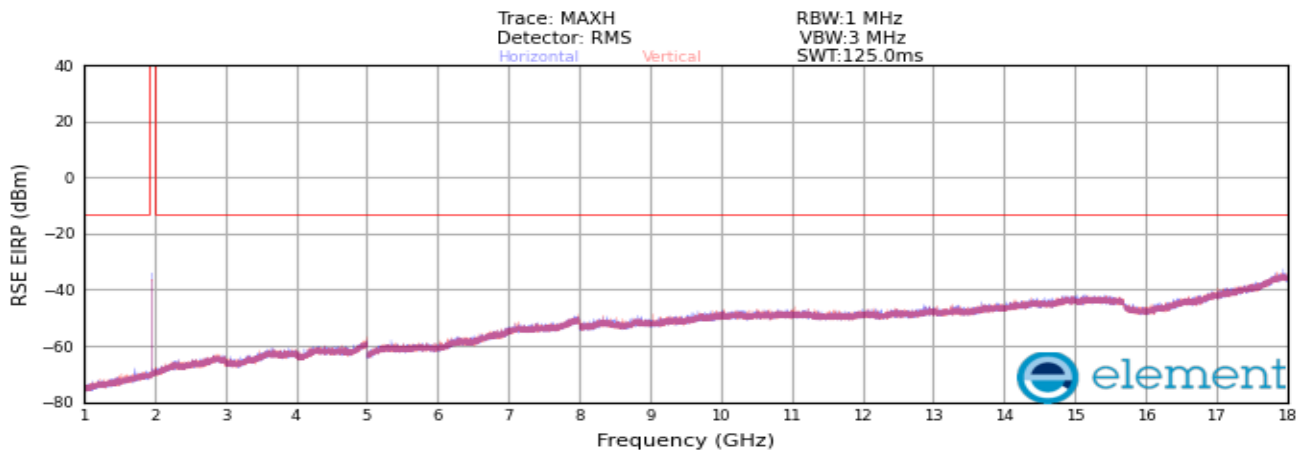
Plot 8-465. Radiated spurious emission Plot_1 GHz to 18 GHz (PCS_NR_1C_5M_Mid Channel_4TX)
