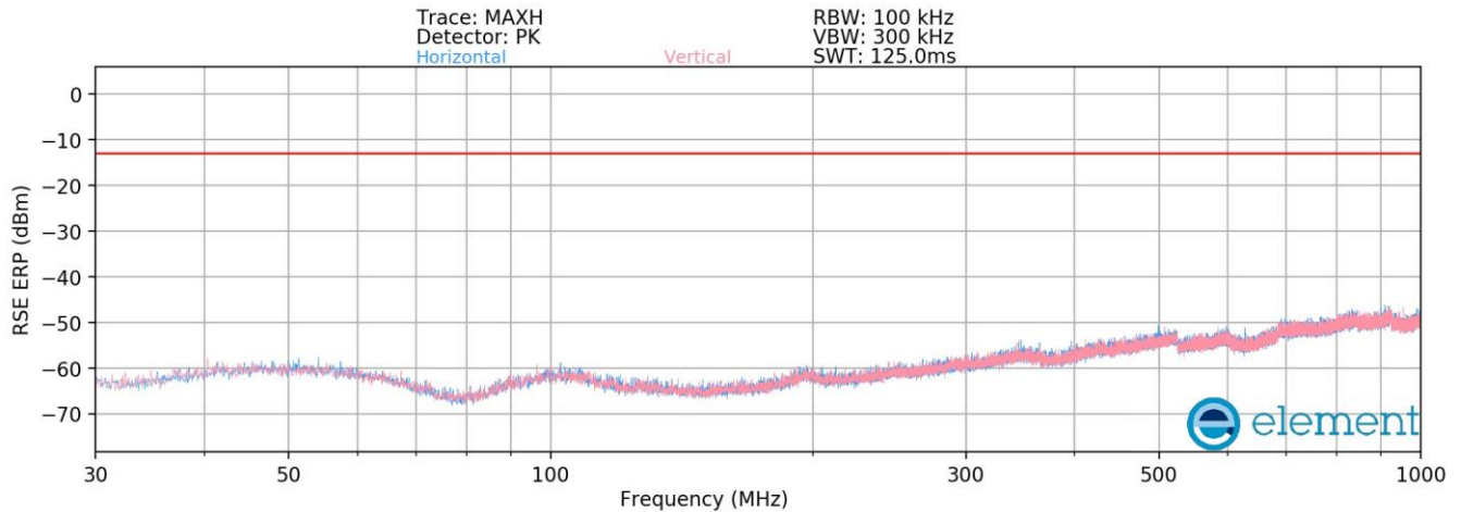
Plot 8-476. Radiated spurious emission 30 MHz to 1000 MHz (AWS_NR_1C_5M_Mid Channel_4TX)
