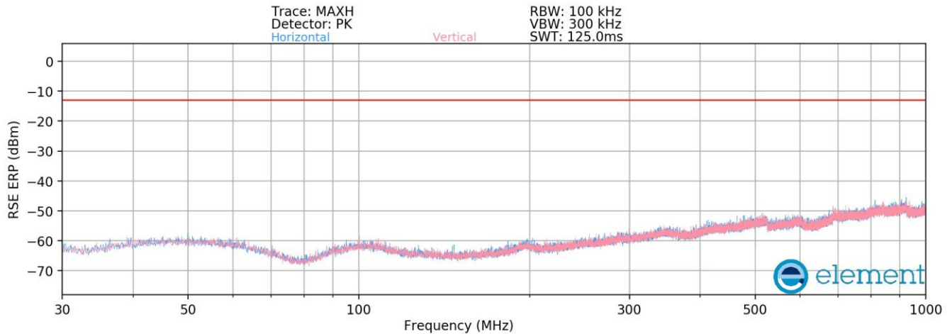
Plot 8-485. Radiated spurious emission 30 MHz to 1000 MHz (PCS_NR_1C_5M_Low Channel + AWS_1C_5M_High Channel_Simultaneous Operation)
