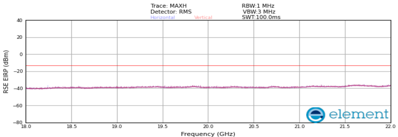
Plot 8-466. Radiated spurious emission Plot_18 GHz to 22 GHz (PCS_NR_1C_5M_Mid Channel_4TX)
