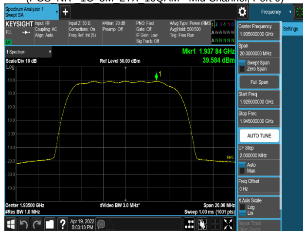
Plot 8-67. Power Spectral Density Plot (PCS_NR_1C_10M_2TX_16QAM - Low Channel, Port 0)
