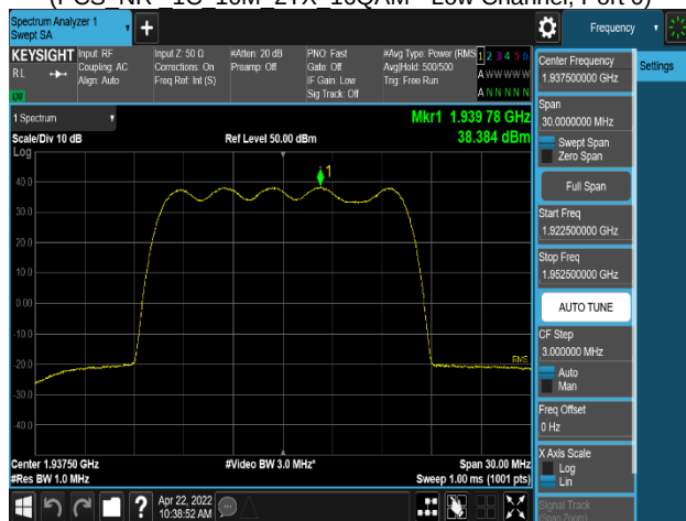
Plot 8-69. Power Spectral Density Plot (PCS_NR_1C_15M_2TX_16QAM - Low Channel, Port 0)
