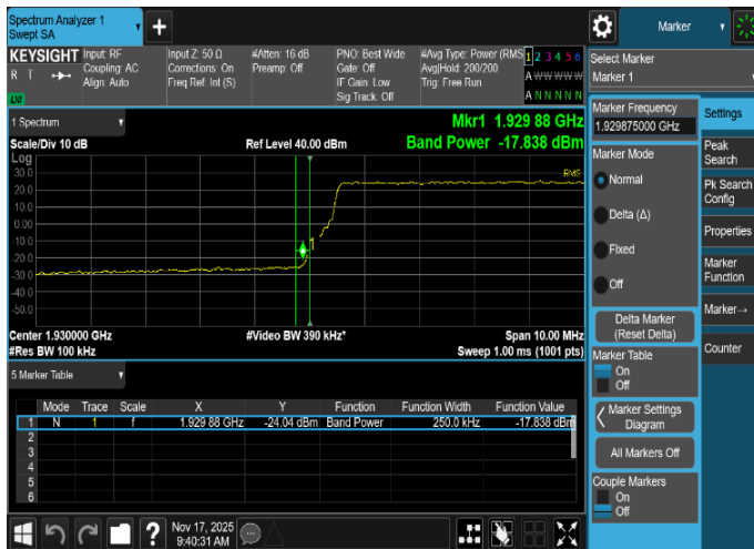
Plot 8-79. Band Edge Emission Summary Data Plot (NR_n2_1C_25M_2T_256QAM - Low Edge, Port 4)
