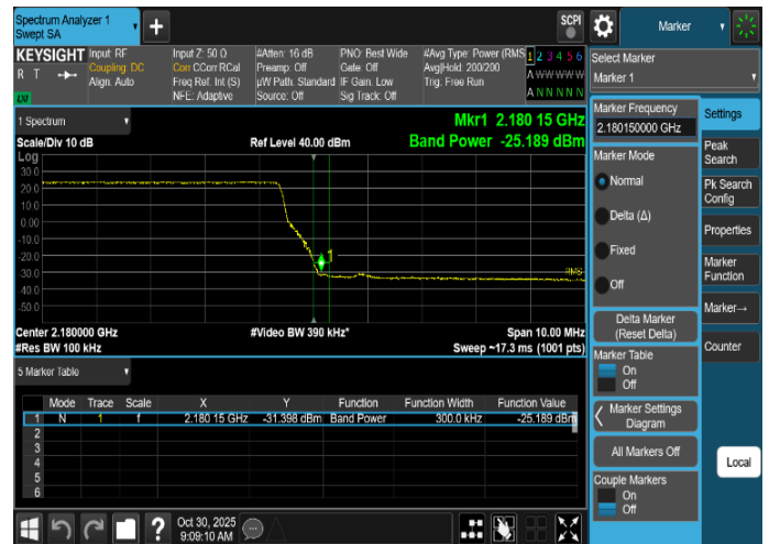
Plot 8-56. Band Edge Emission Summary Data Plot (NR_n66_1C_30M_4T_64QAM - High Edge, Port 1)
