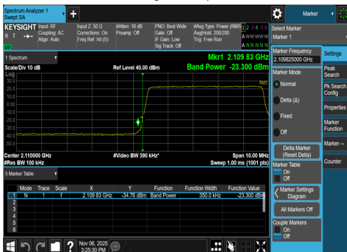
Plot 8-63. Band Edge Emission Summary Data Plot (MSR_B/n66_3NC_NR 5M+NR 25M+LTE 5M_4T_QPSK - Low Edge, Port 0)
