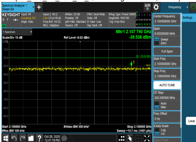
Plot 8-85. Conducted Spurious Emission Plot 2.1 GHz to 2.109 GHz (NR_n66_1C_25M_4T_QPSK - High Channel, Port 2)
