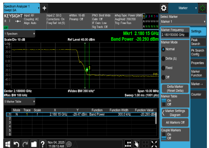
Plot 8-58. Band Edge Emission Summary Data Plot (NR_n66_2C_5M+25M_4T_QPSK - High Edge, Port 2)
