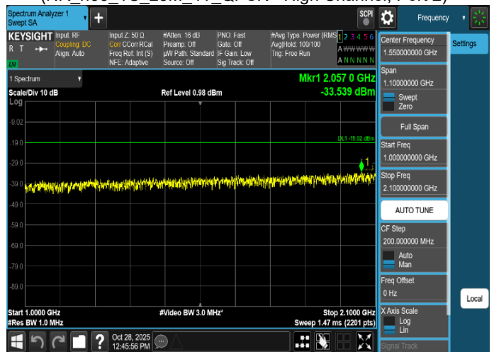
Plot 8-84. Conducted Spurious Emission Plot 1 GHz to 2.1 GHz
