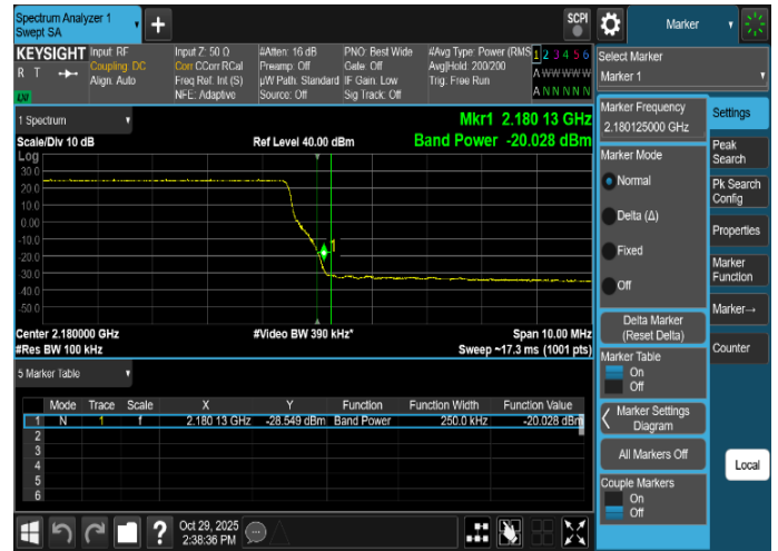
Plot 8-54. Band Edge Emission Summary Data Plot (NR_n66_1C_25M_4T_QPSK - High Edge, Port 0)
