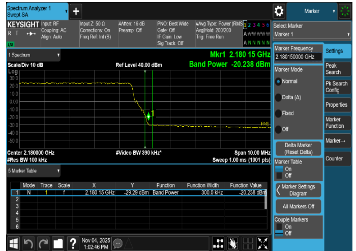
Plot 8-60. Band Edge Emission Summary Data Plot (NR_n66_2NC_5M+25M_4T_QPSK - High Edge, Port 3)
