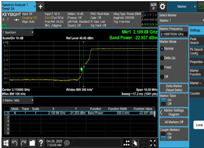
Plot 8-53. Band Edge Emission Summary Data Plot (NR_n66_1C_25M_4T_16QAM - Low Edge, Port 0)
