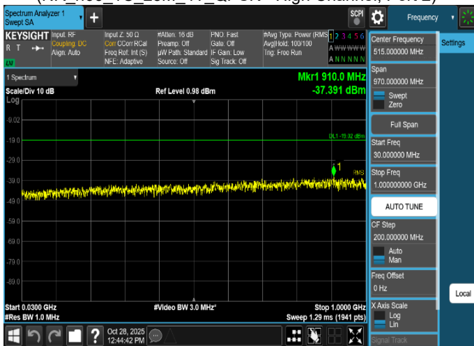
Plot 8-83. Conducted Spurious Emission Plot 30 MHz to 1 GHz (NR_n66_1C_25M_4T_QPSK - High Channel, Port 2)
