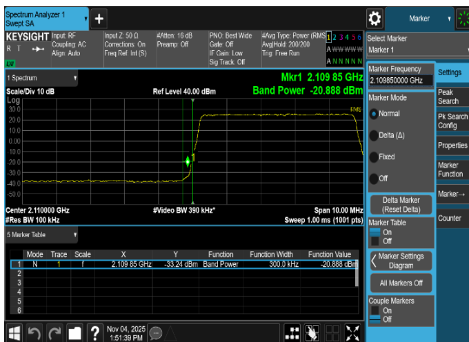
Plot 8-69. Band Edge Emission Summary Data Plot (NR_n66_2C_5M+25M_2T_QPSK - Low Edge, Port 0)
