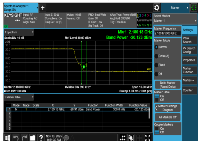
Plot 8-64. Band Edge Emission Summary Data Plot (MSR_B/n66_2NC_DSS 10M+NR 25M_4T_QPSK - High Edge, Port 0)
