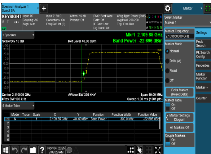
Plot 8-57. Band Edge Emission Summary Data Plot (NR_n66_2C_5M+25M_4T_QPSK - Low Edge, Port 0)
