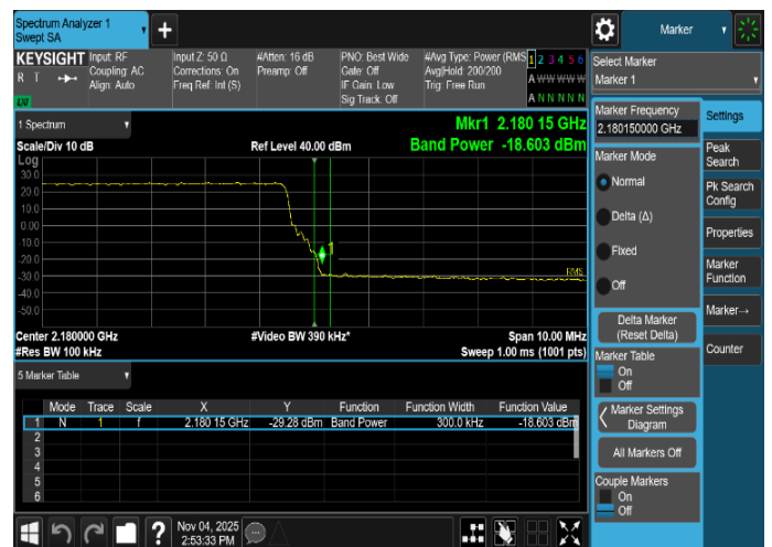
Plot 8-70. Band Edge Emission Summary Data Plot (NR_n66_2C_5M+25M_2T_QPSK - High Edge, Port 1)
