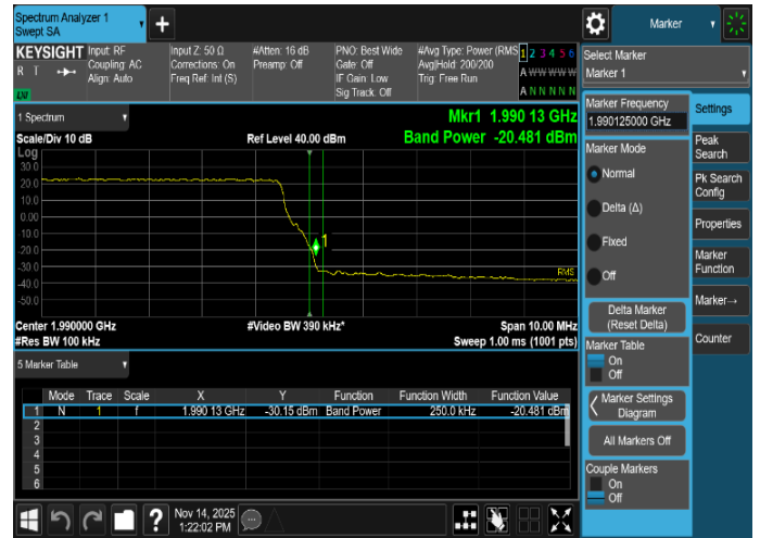
Plot 8-78. Band Edge Emission Summary Data Plot (NR_n2_1C_25M_4T_16QAM - High Edge, Port 7)
