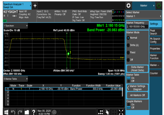
Plot 8-62. Band Edge Emission Summary Data Plot (MSR_B/n66_2C_NR 25M+LTE 5M_4T_QPSK - High Edge, Port 2)
