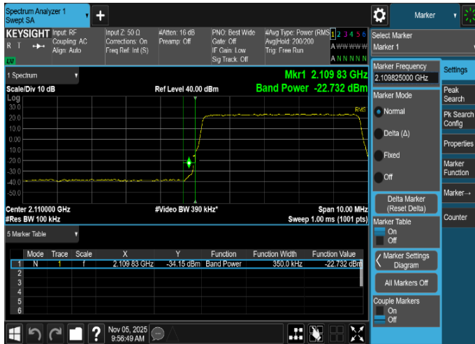
Plot 8-59. Band Edge Emission Summary Data Plot (NR_n66_3NC_5M+5M+25M_4T_QPSK - Low Edge, Port 0)
