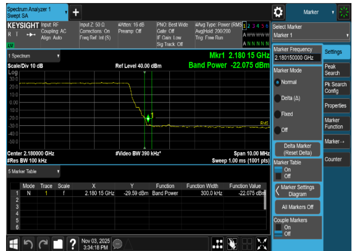
Plot 8-68. Band Edge Emission Summary Data Plot (NR_n66_1C_30M_2T_256QAM - High Edge, Port 0)
