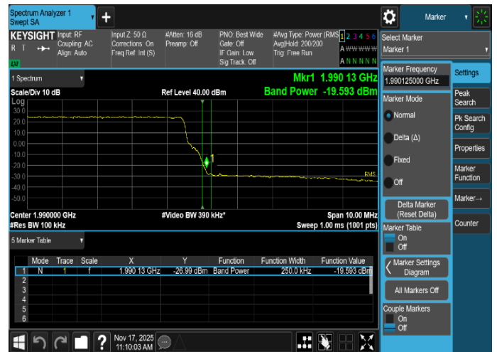
Plot 8-80. Band Edge Emission Summary Data Plot (NR_n2_1C_25M_2T_16QAM - High Edge, Port 4)
