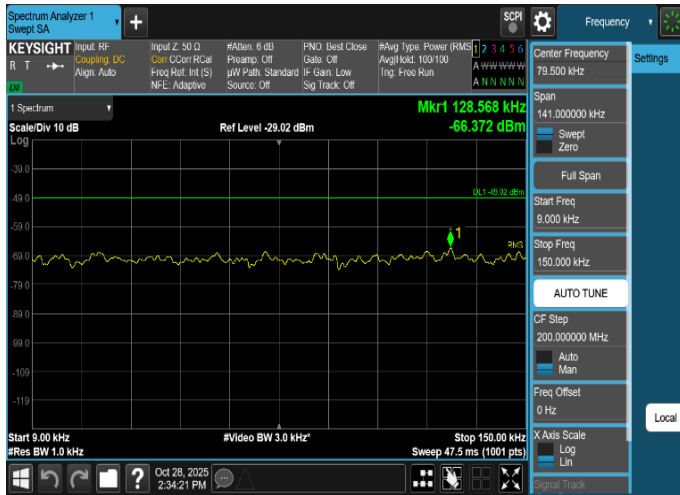
Plot 8-81. Conducted Spurious Emission Plot 9 kHz to 150 kHz
