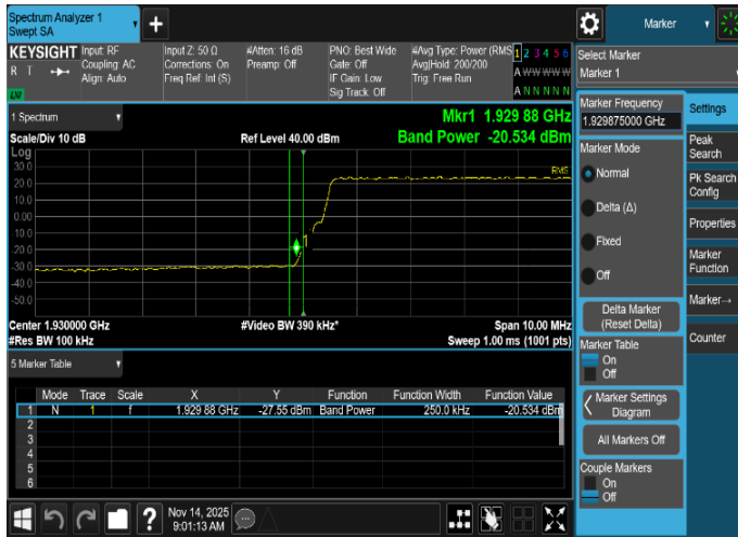
Plot 8-77. Band Edge Emission Summary Data Plot (NR_n2_1C_25M_4T_16QAM - Low Edge, Port 4)
